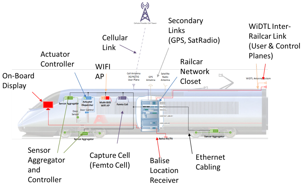
Figure 7. Proposed power car networking architecture
