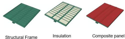
Figure 2. ABAQUS model showing component geometry of Design 2
