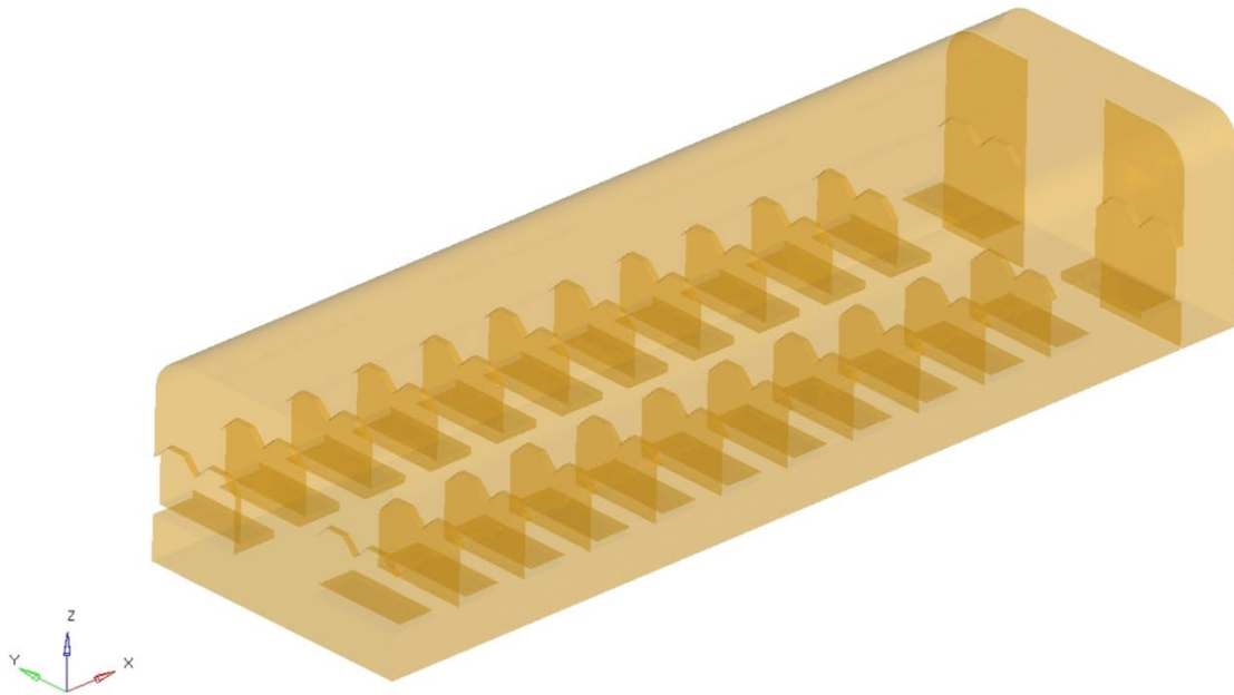
Figure 3-2. Finite element model for air volume only (233,338 nodes, 1,172,792 elements) seats shown for location
