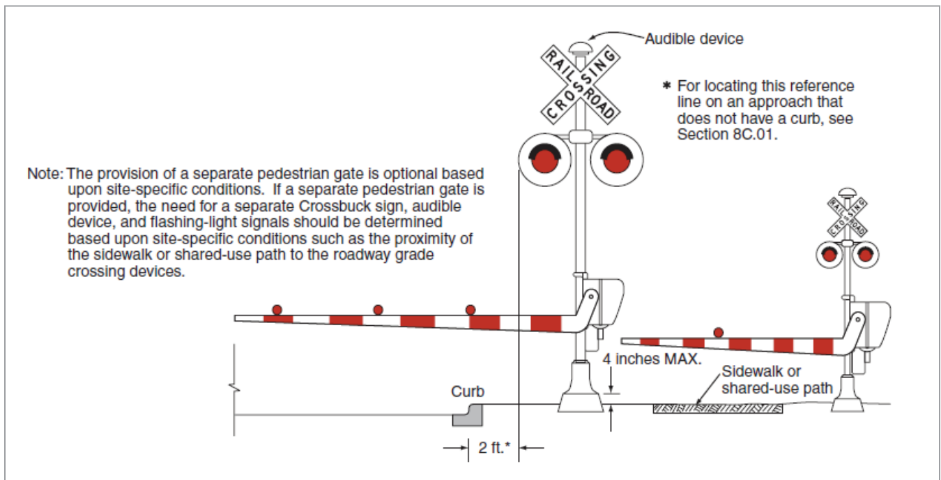
Figure 31: Example of a Separate Pedestrian Gate (MUTCD 2009 Fig. 8C-6)
