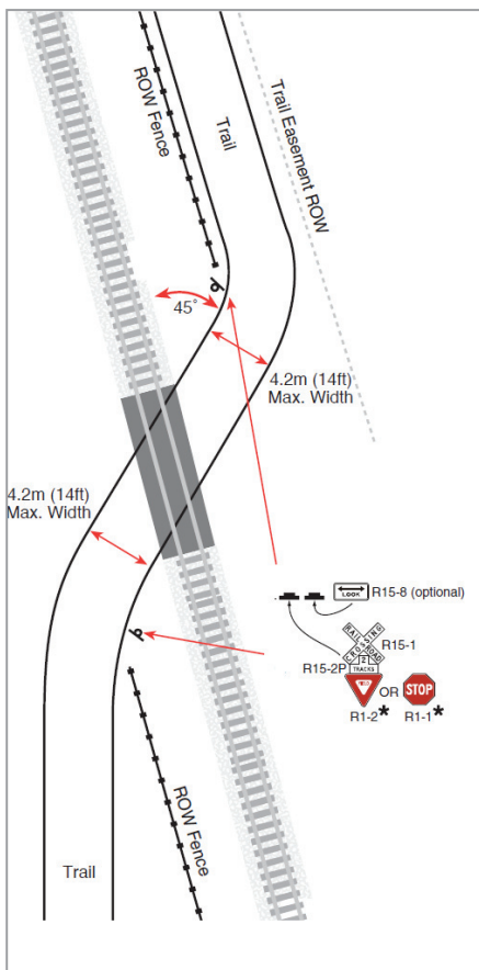
Figure 22: 45° Trail-Rail Crossing
