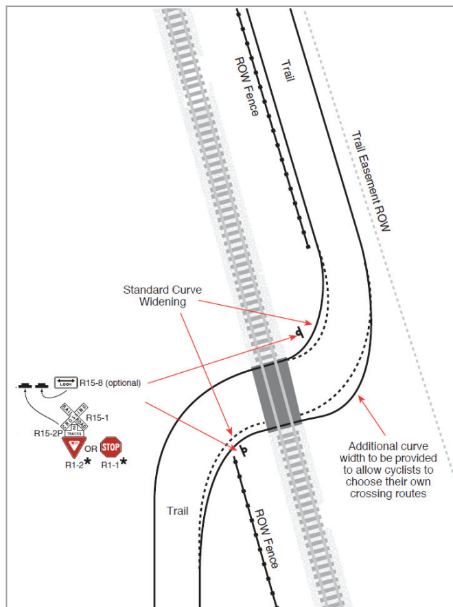
Figure 23: 90° Trail-Rail Crossing
