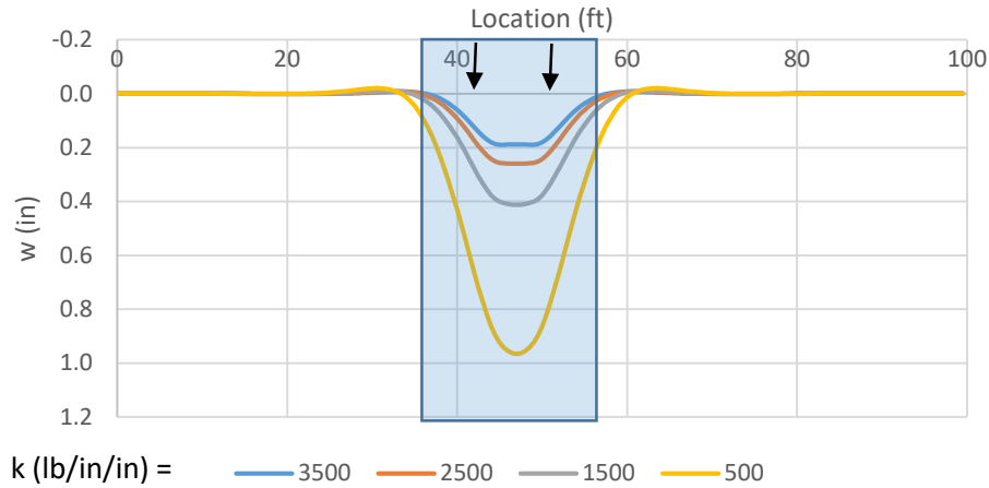
Figure 12. Deflection “plot” for a two-wheel bogie with varying soft spot track modulus
