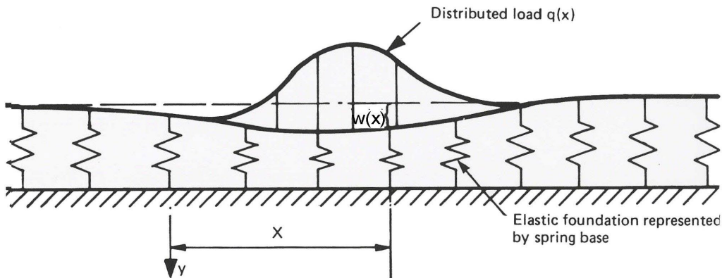
Figure 9. BOEF model
