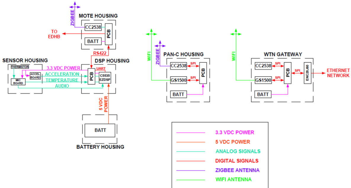
Figure 16 Wireless Train Network Components
