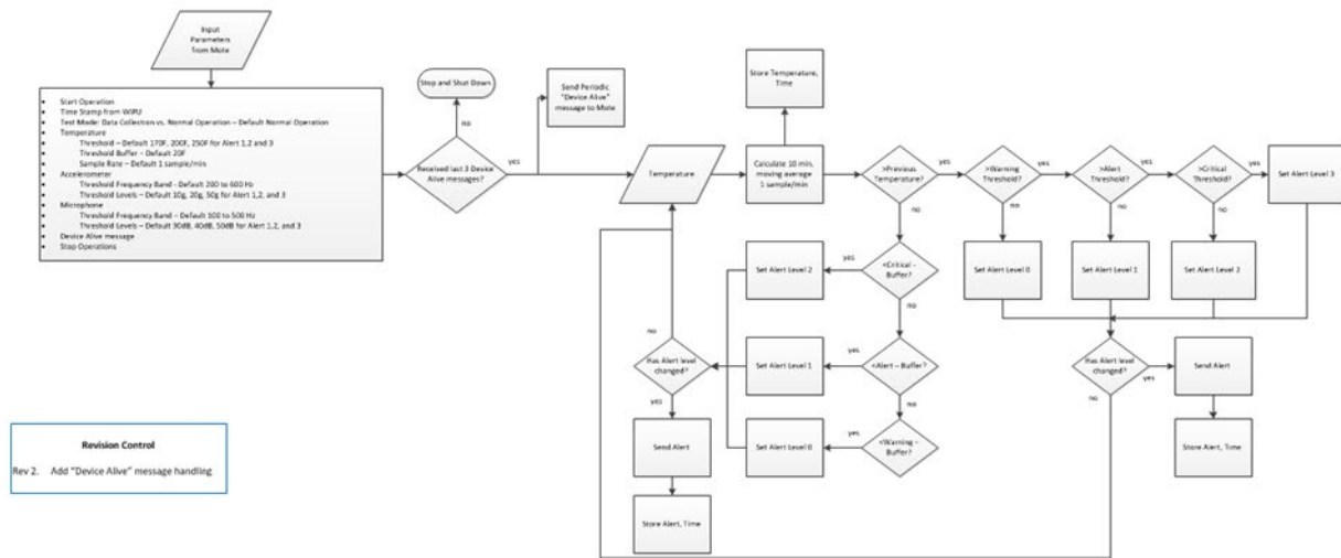
Figure 29 Thermistor Implementation Logic
