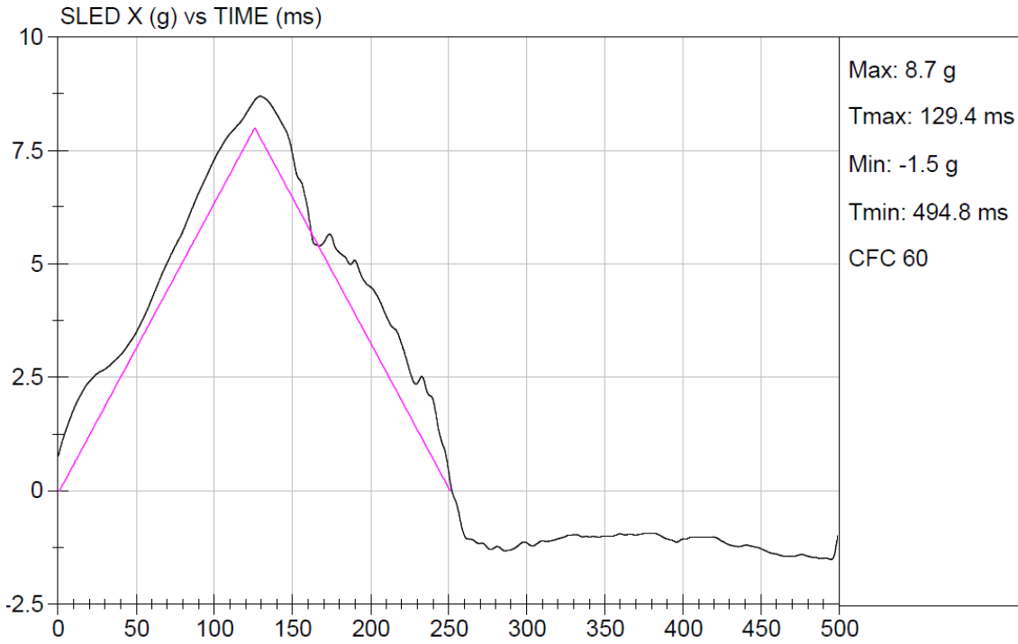
Figure 9: Test 1 Crash Pulse
