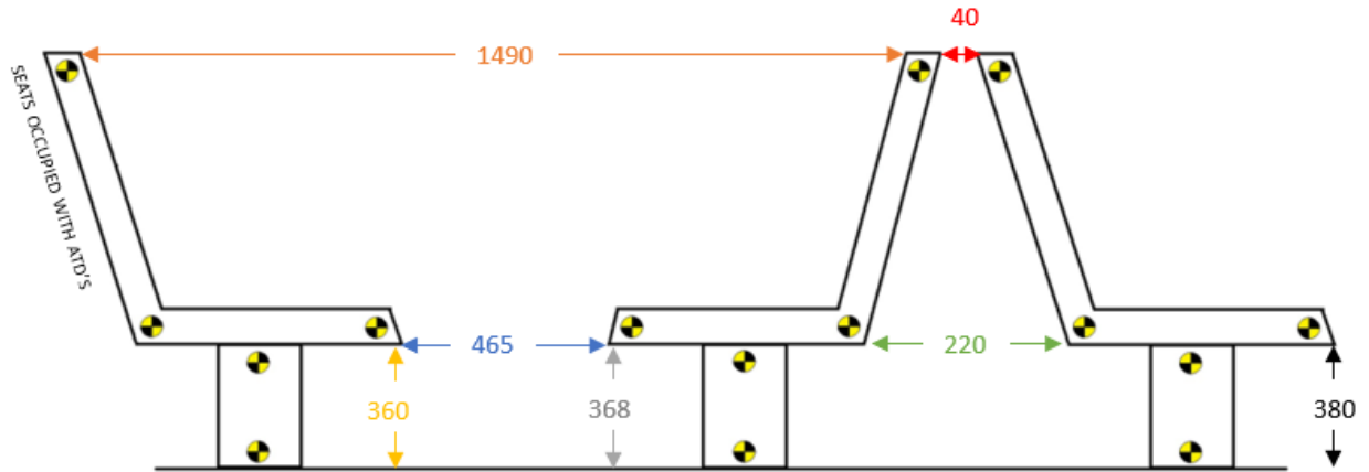
Figure 14: Test 1 Right Hand (Wall) Seat Pre-Test Measurements
