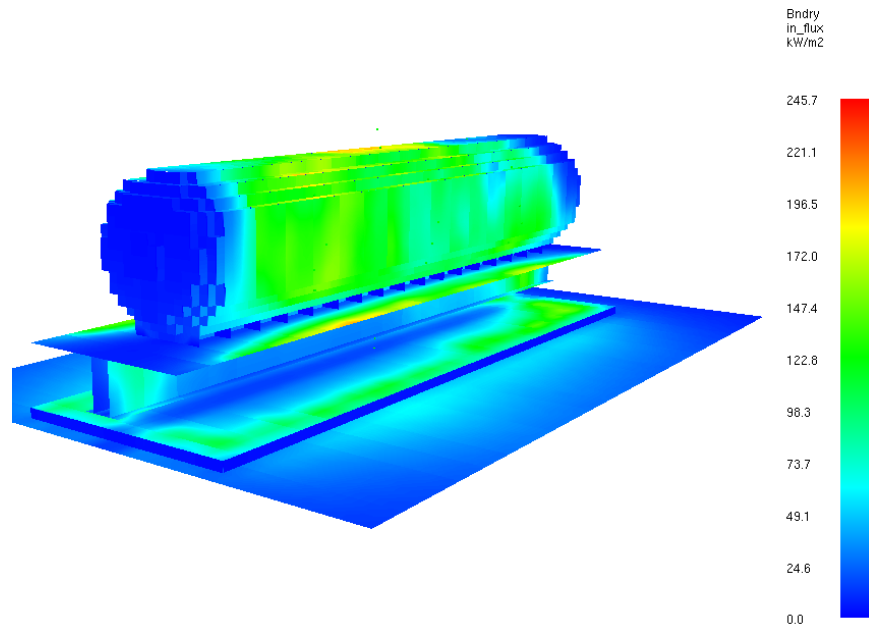
Figure 54. Incident heat flux on tank exterior in the HIGH pool fire only configuration
