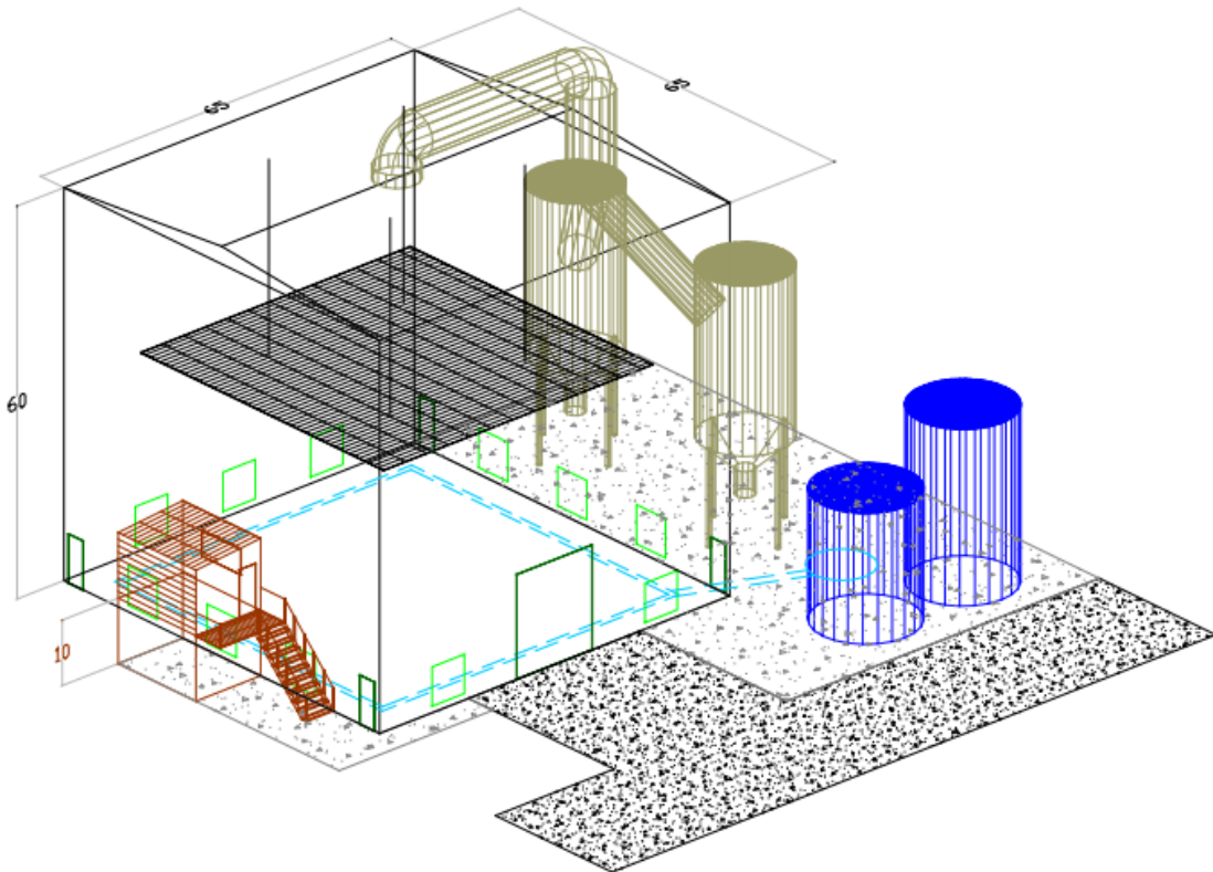
Figure 31. Large-scale fire engineering and research facility layout
