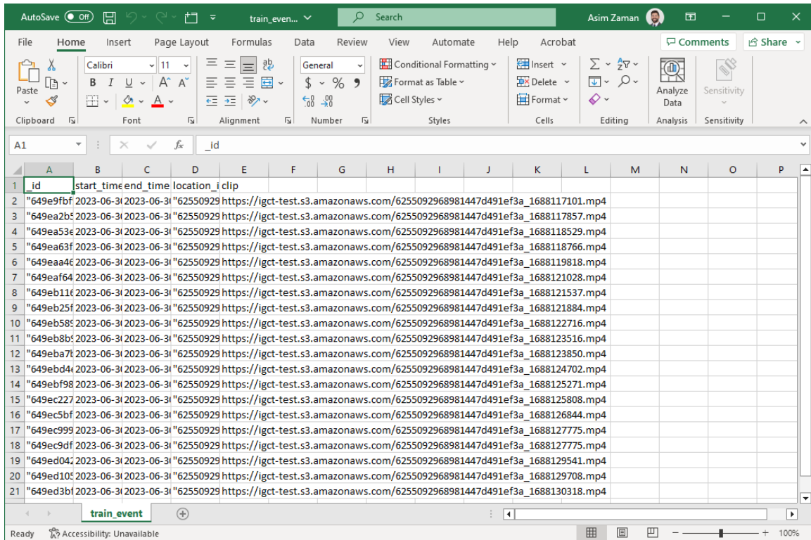
Figure 36. Example train_event.csv
