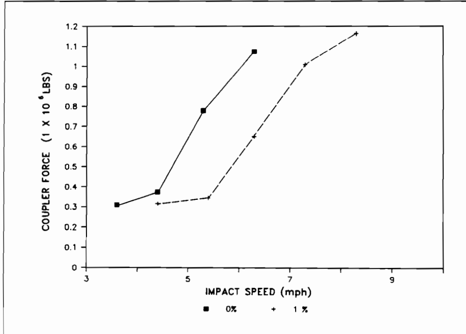
Figure 30. Coupler Force vs Impact Speed, 0% Outage, A-end Impacted
