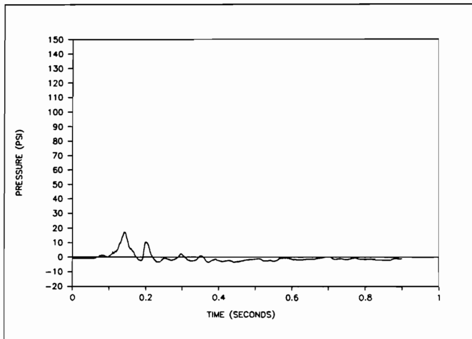
Figure 26. Surge Pressure in 2 1/2" Nozzle with SPR, 0% Outage, B-end Impacted at 5 mph
