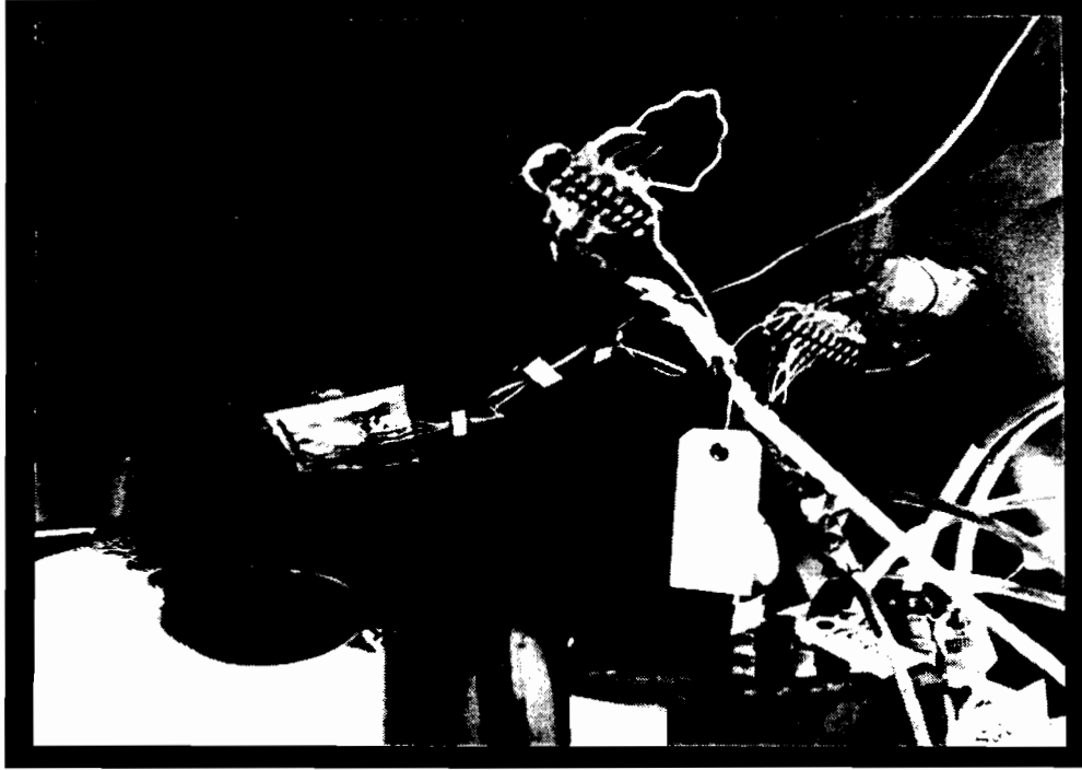
Figure 4. View of Strain Gage Rosette 2 (Location is on Middle Cross Section of Car)
