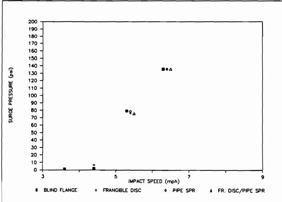
Figure 22. Surge Pressure in 4 1/2" Nozzle 0% Outage, A-end Impacted
