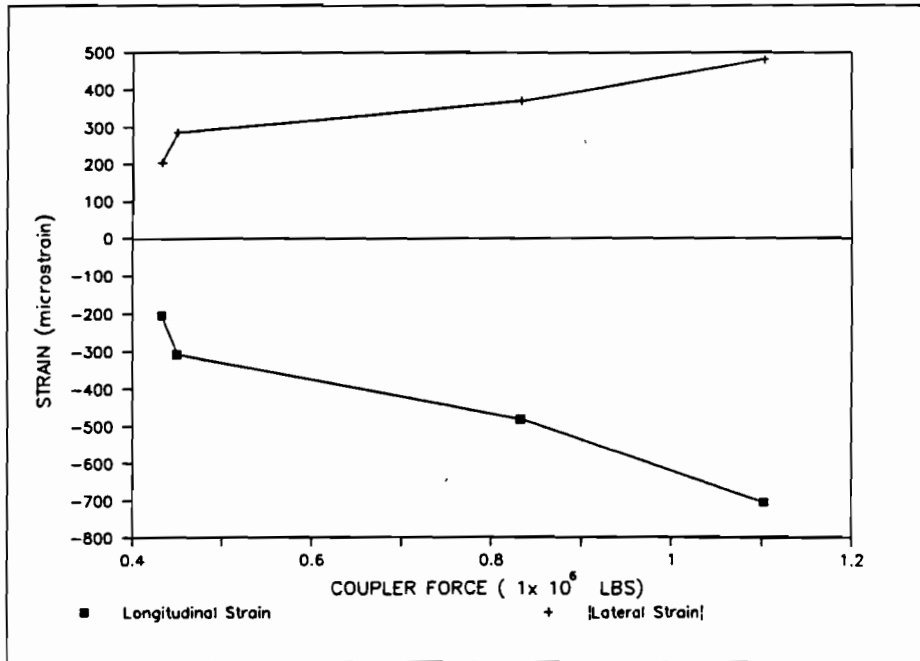
Figure 31. Longitudinal and Lateral Strains vs Coupler Force
