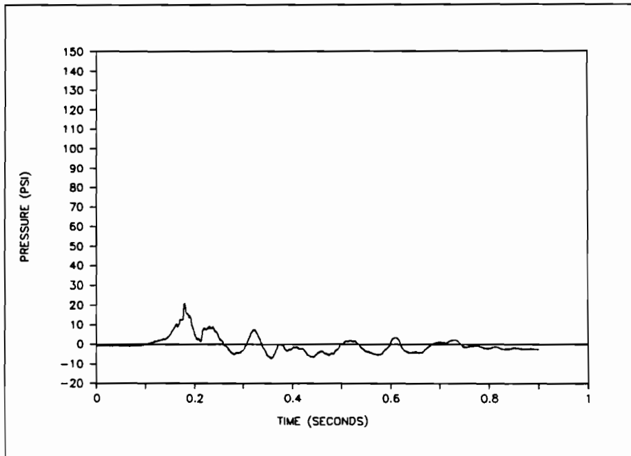
Figure 28. Surge Pressure in 6 1/2" Nozzle with SPR, 0% Outage, A-end Impacted at 5 mph
