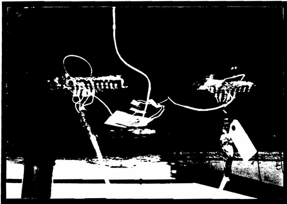
Figure 3. View of Strain Gage Rosette (9' 3/8" from B-end)
