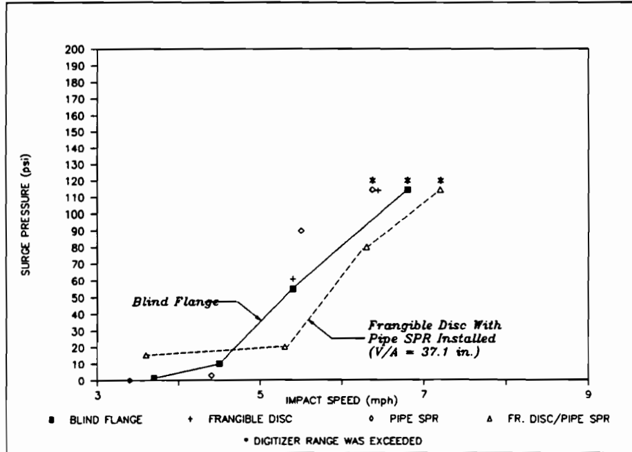
Figure 21. Surge Pressure in 4 1/2" Nozzle 0% Outage, B-end Impacted
