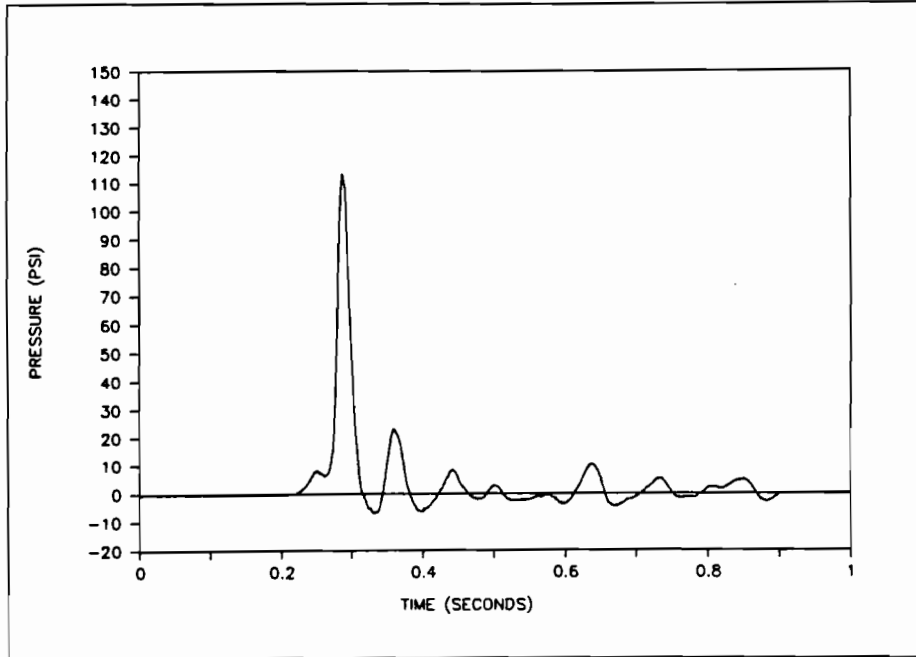
Figure 27. Surge Pressure in 6 1/2" Nozzle without SPR, 0% Outage, A-end Impacted at 5 mph
