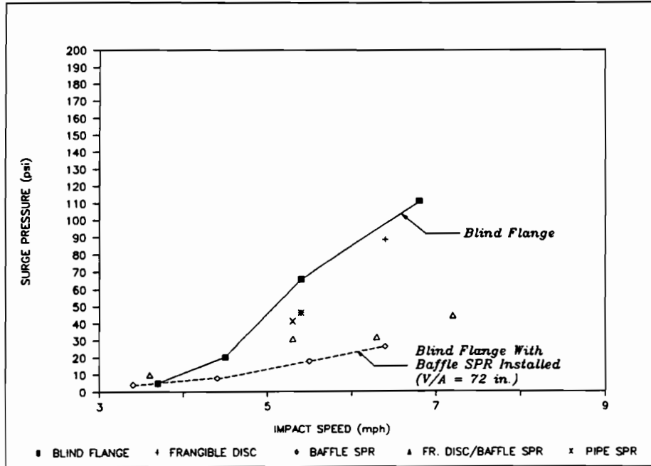
Figure 19. Surge Pressure in 2 1/2" Nozzle 0% Outage, B-end Impacted
