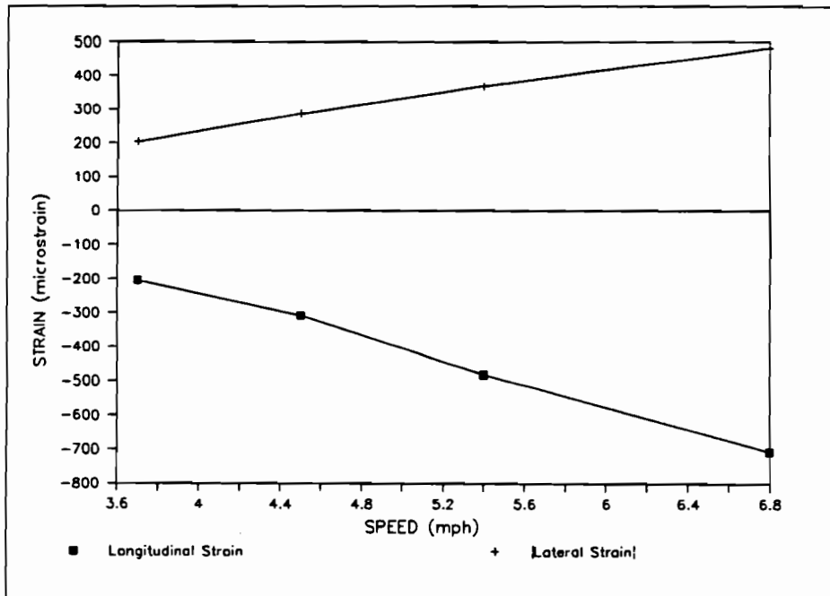
Figure 32. Longitudinal and Lateral Strains vs Impact Speed
