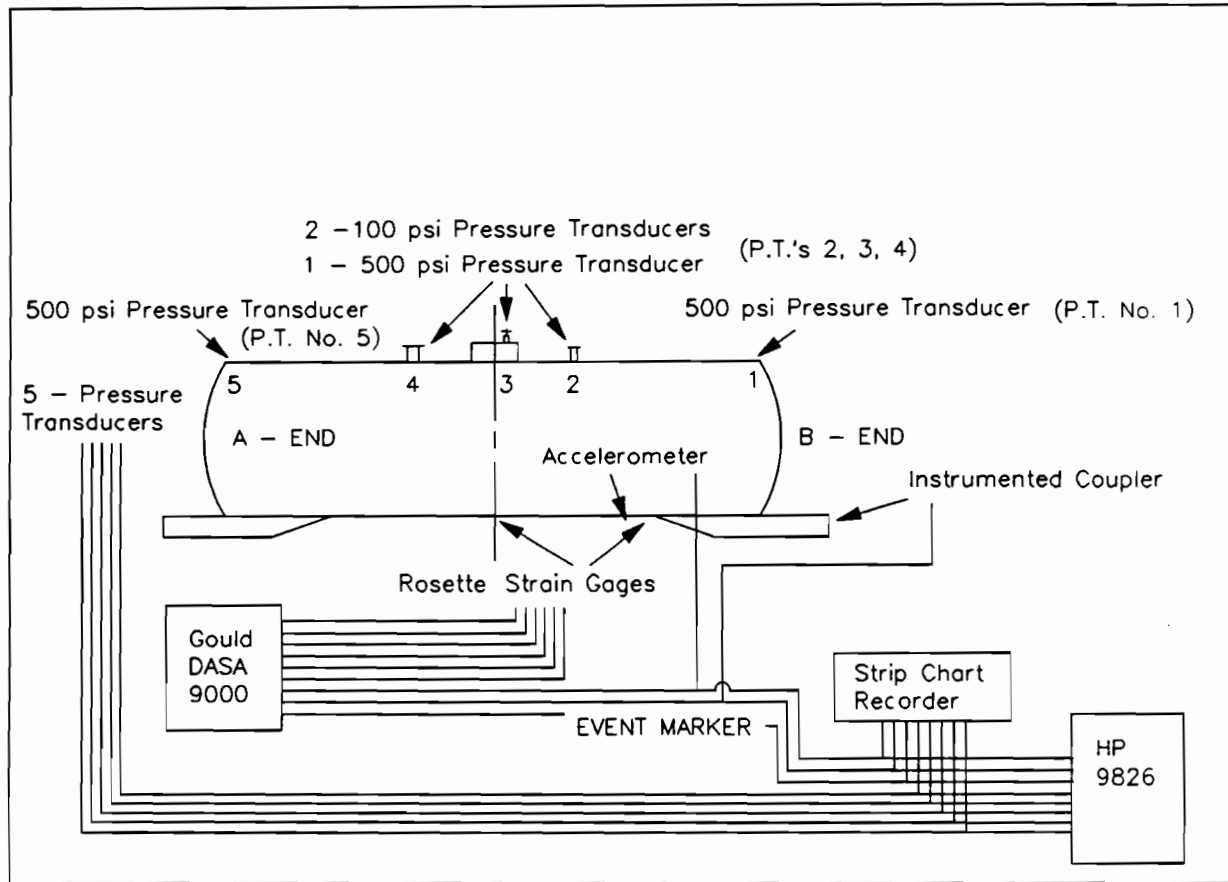
Figure 12. Instrumentation Layout
