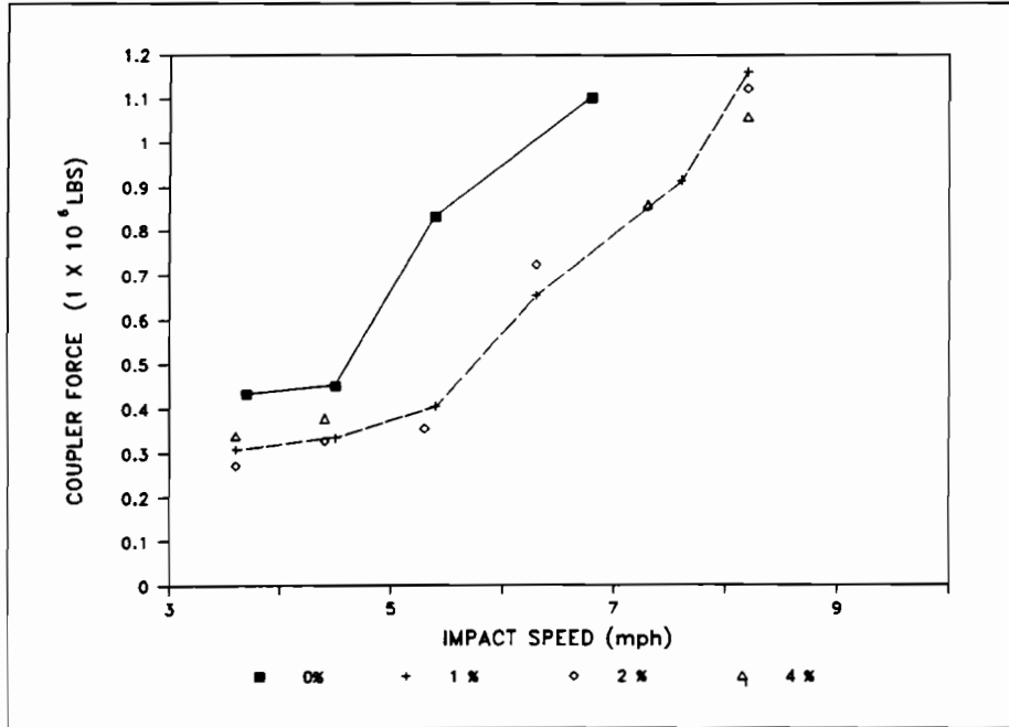
Figure 29. Coupler Force vs Impact Speed, 0% Outage, B-end Impacted
