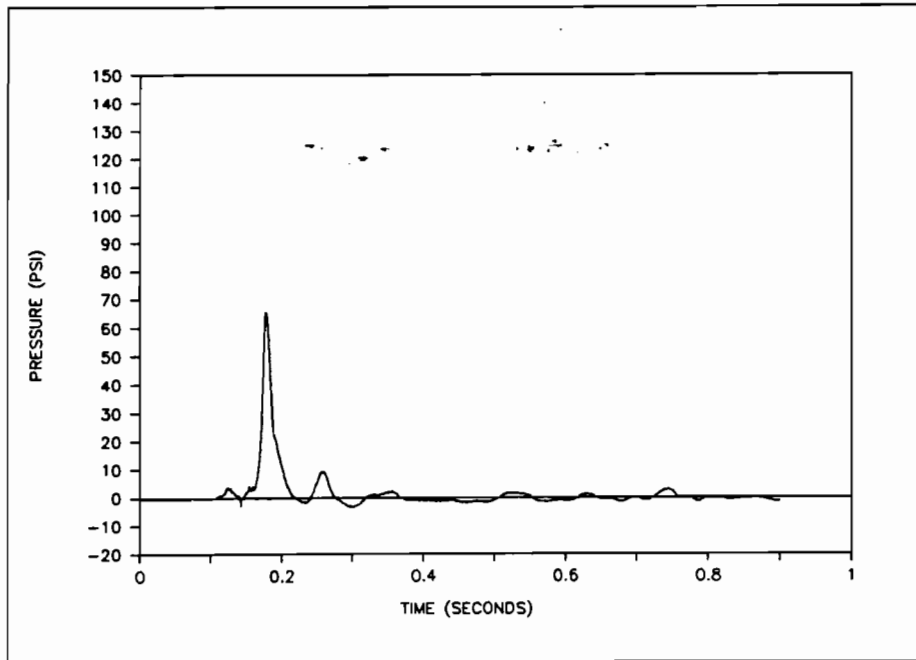
Figure 25. Surge Pressure in 2 1/2" Nozzle without SPR, 0% Outage, B-end Impacted at 5 mph
