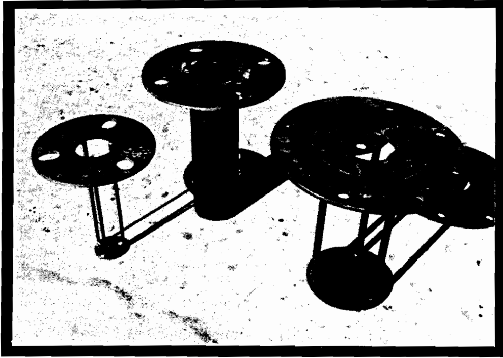
Figure 8. View of Surge Pressure Reducers (left to right): Baffle Type SPR for 2 1/2" Safety Vent, Pipe Type SPR for 4 1/2" Sump Nozzle, Baffle Type SPR for 6 1/2" Safety Vent
