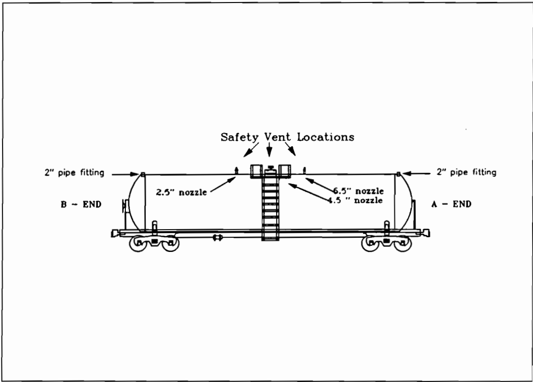
Figure 1. DOT 111A100W2 Tank Car
