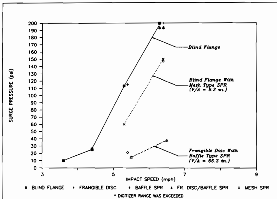
Figure 24. Surge Pressure in 6 1/2" Nozzle 0% Outage, A-end Impacted
