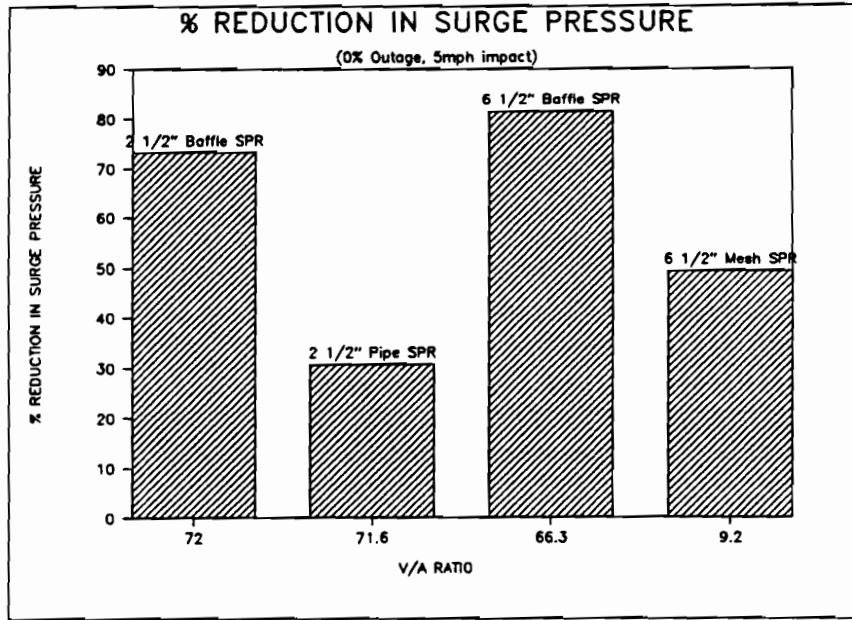
Figure 33. Percent Reduction in Surge Pressure For Four SPR Designs (0% Outage, 5 mph Impact Speed)
