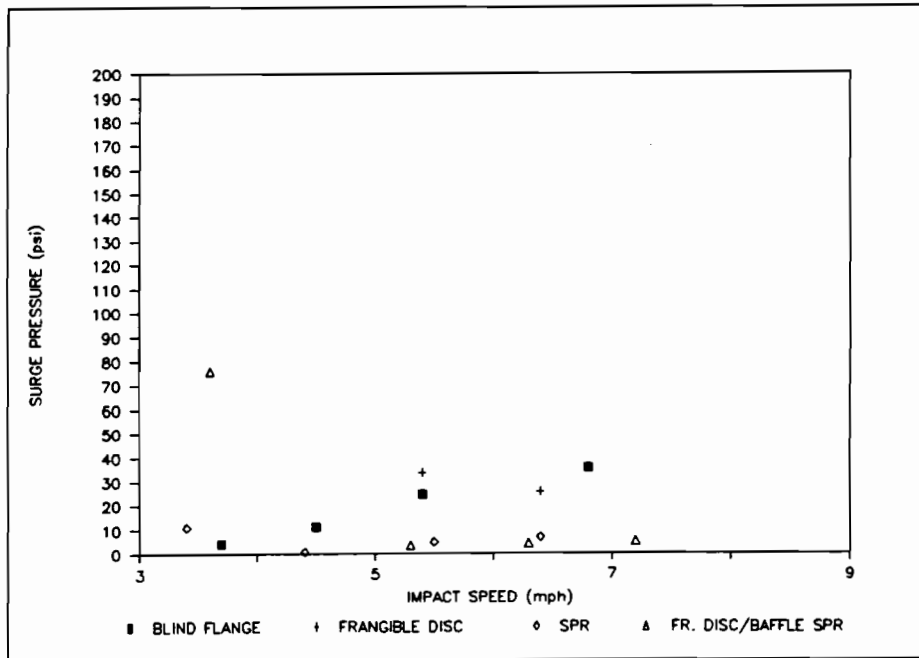
Figure 23. Surge Pressure in 6 1/2" Nozzle 0% Outage, B-end Impacted
