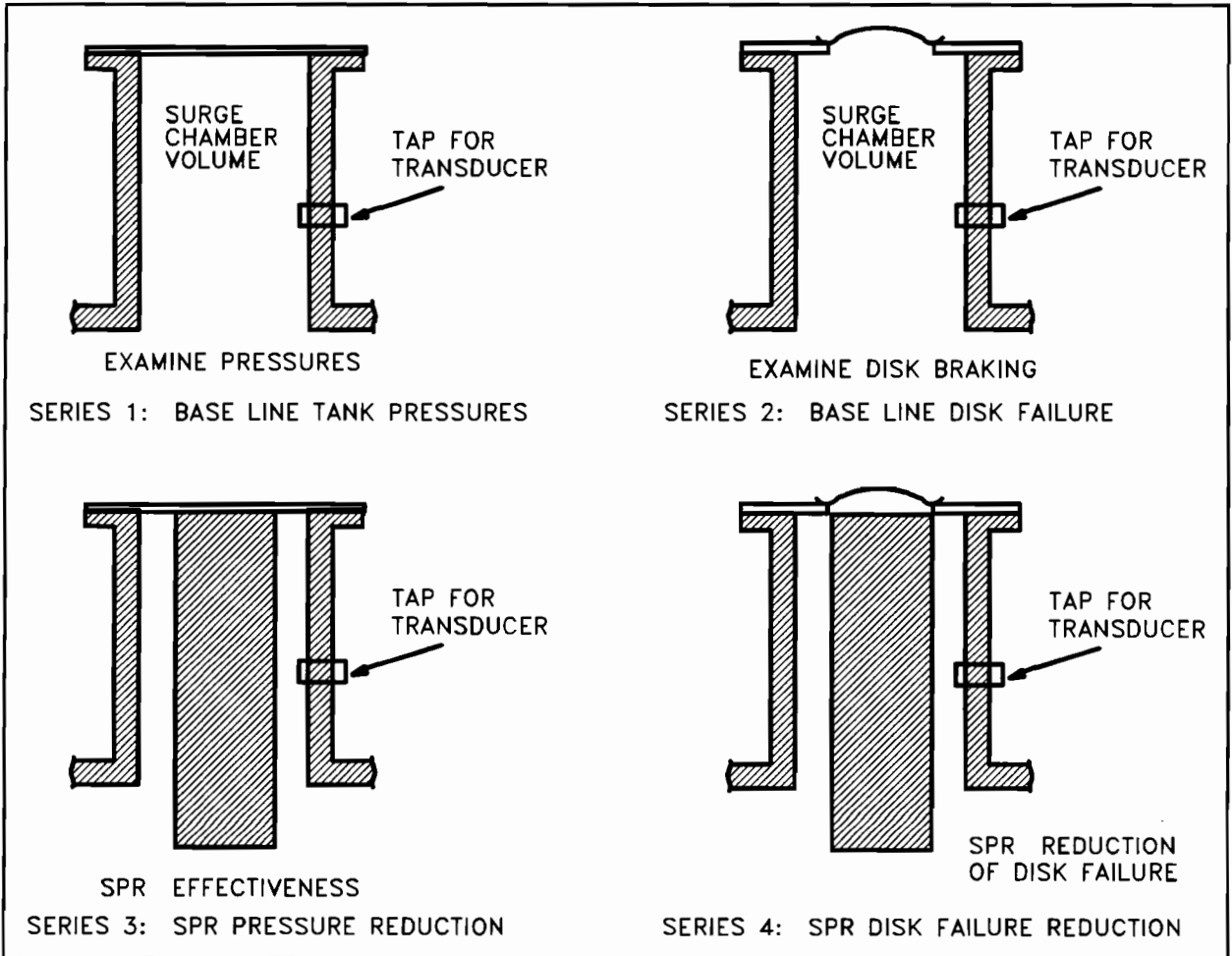
Figure 7. Display of the Four Set-ups Used in this Test
