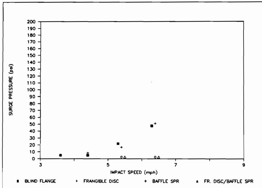
Figure 20. Surge Pressure in 2 1/2" Nozzle 0% Outage, A-end Impacted
