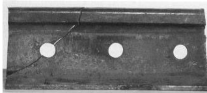
Figure 2-5. Bolt-Hole Crack in Rail
