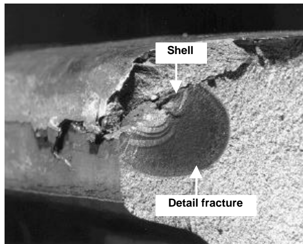
Figure 2-2. Broken Rail Showing Shell Origin of Detail Fracture (Courtesy of Transportation Technology Center, Inc.)
