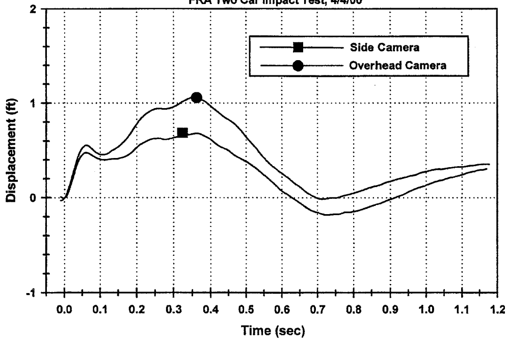
Coupler View Side and Overhead Cameras Longitudinal Displacement Trailing Car Relative to Leading Car FRA Two Car Impact Test, 4/4/00
