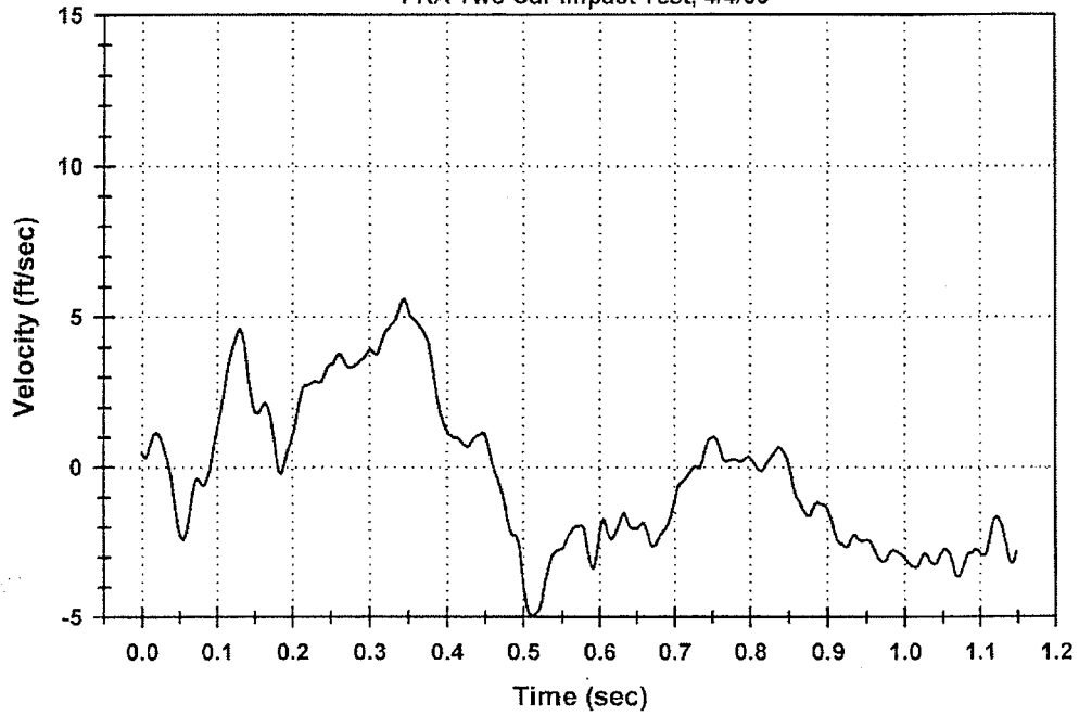
Coupler View Side Camera Vertical Velocity Trailing Car Relative to Leading Car FRA Two Car Impact Test, 4/4/00
