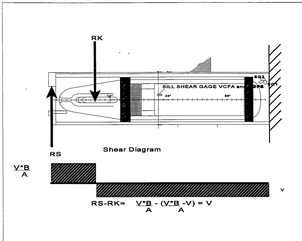
Figure 25. Shear Diagram For Assumed VCF Load Path
