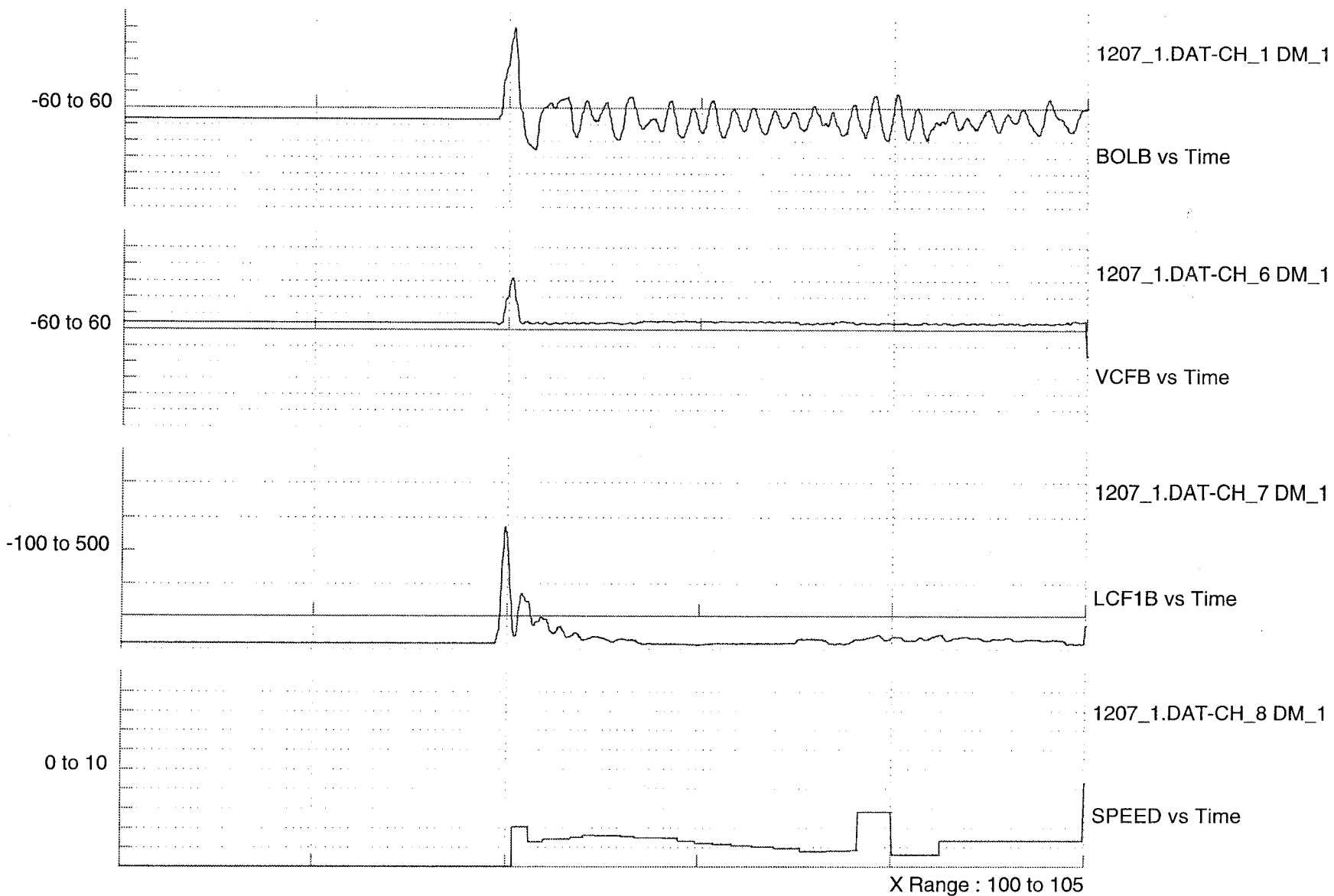
Figure G18. Leg 9 Impact Event
