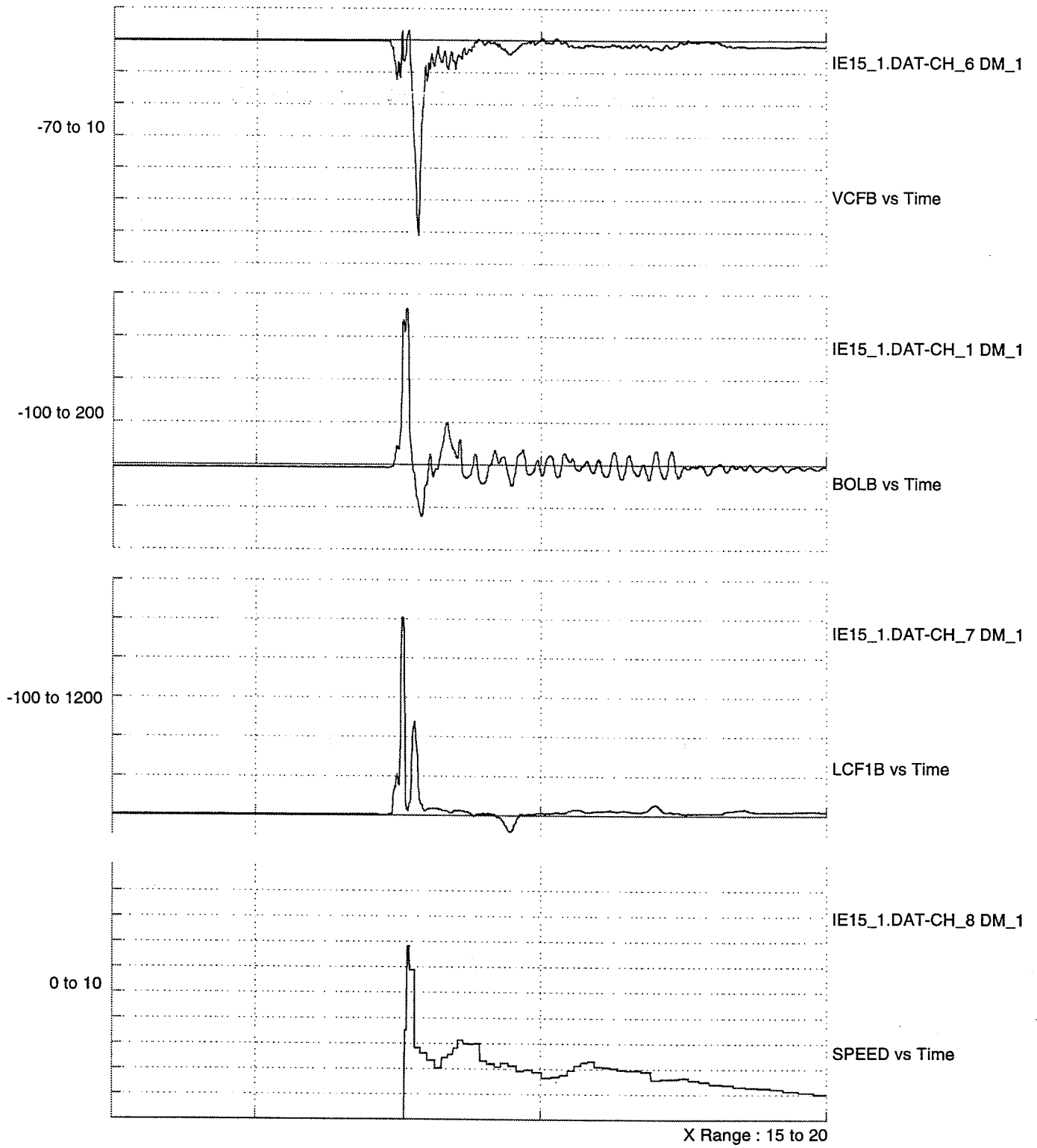
Figure 63. Coupler Force Response To Impact
