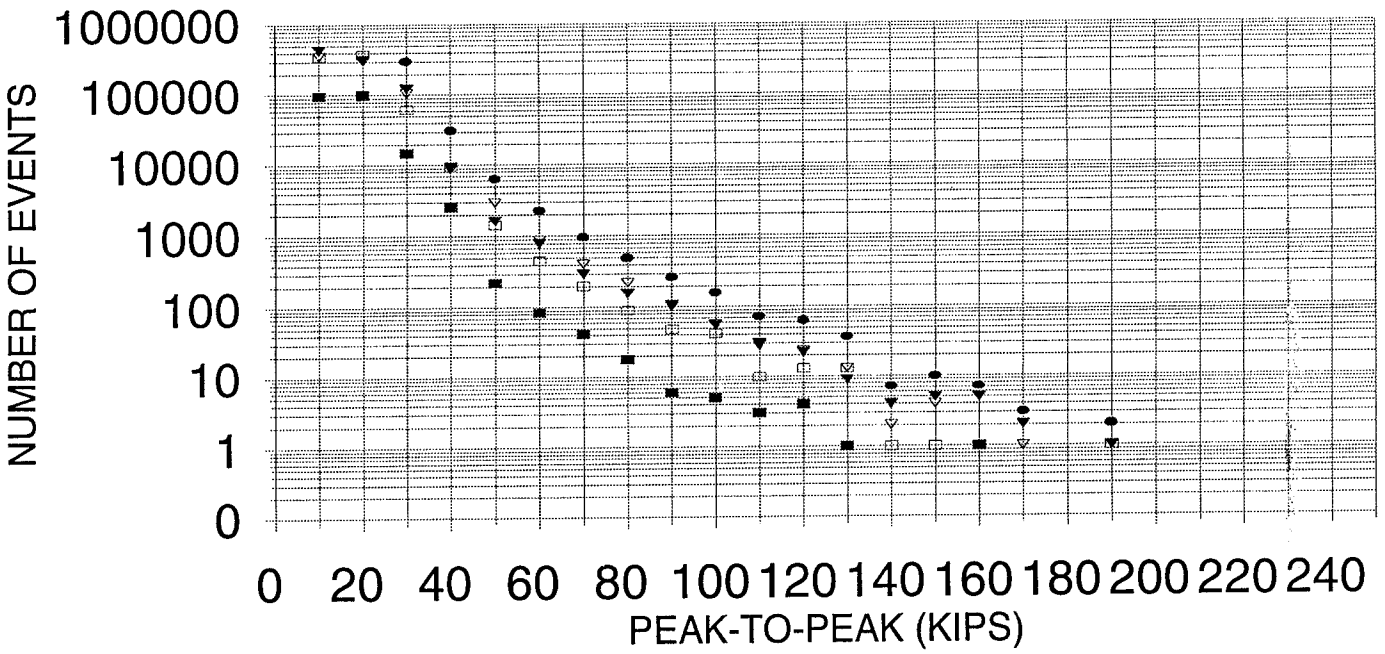
Figure A7. Loaded Portion Histograms for Measurement BOLA Number of Events
