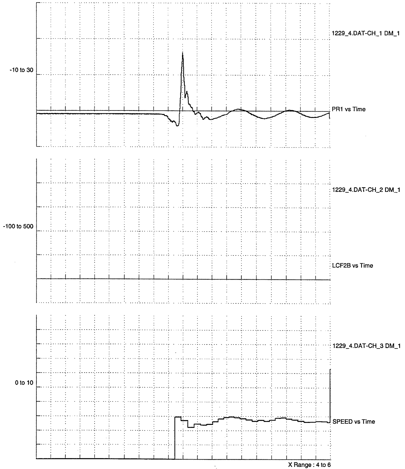
Figure C13. Surge Pressure Event 2 Leg 10
