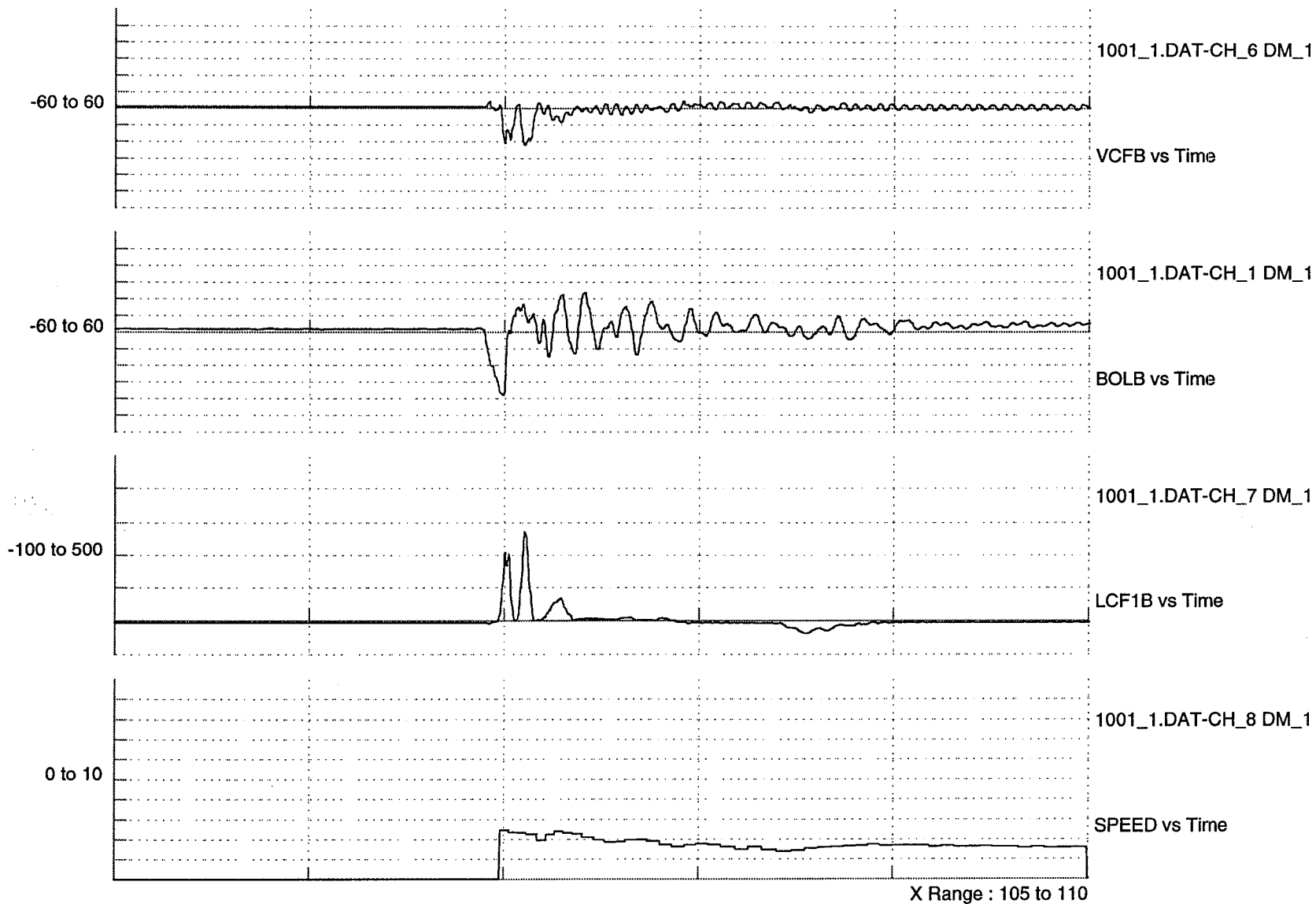
Figure G5. Leg 5 Impact Event
