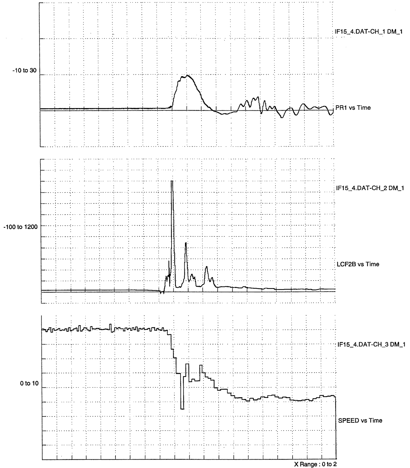
Figure 59. Surge Pressure Repeatability 9 mph
