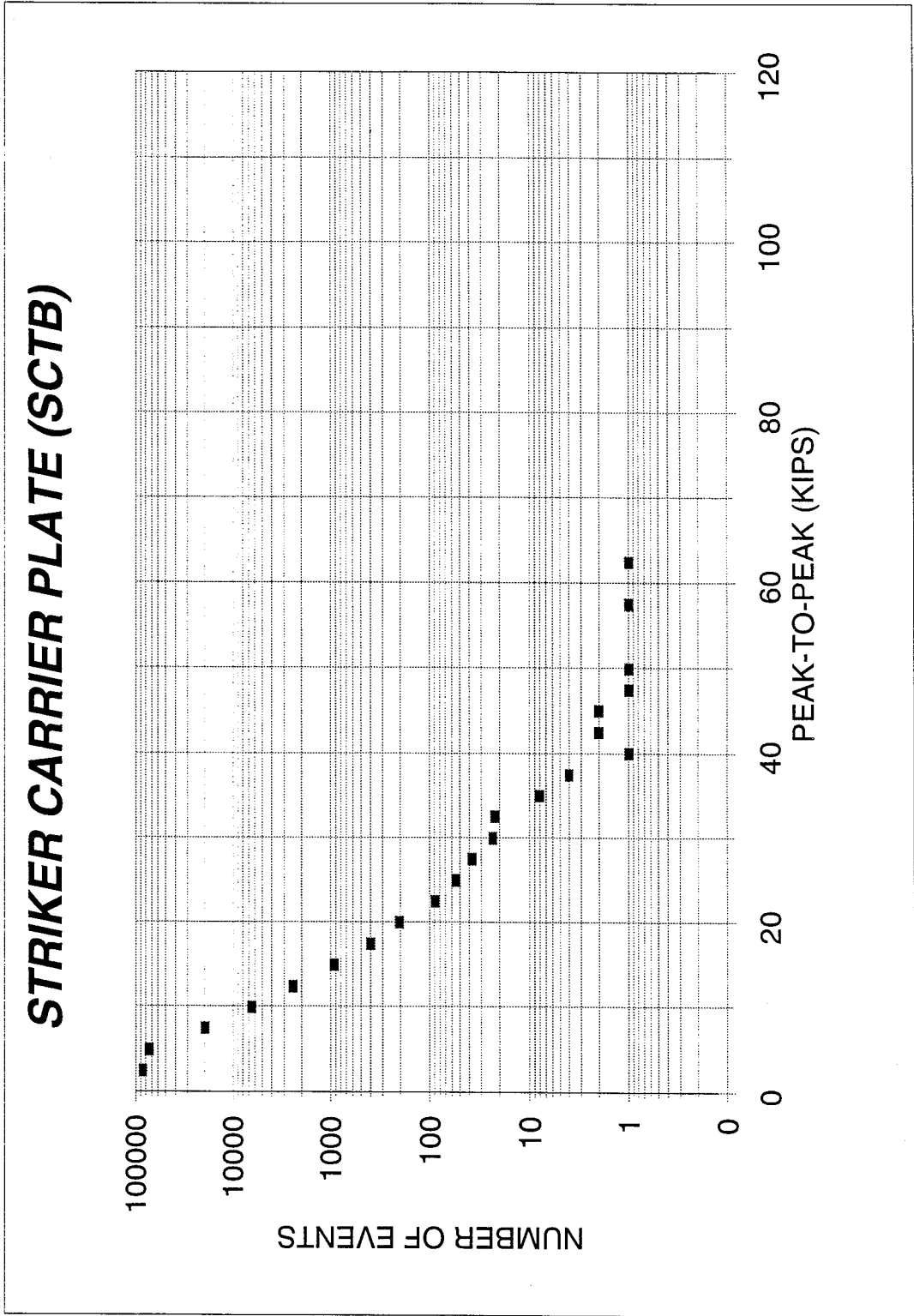
Figure B5. Unloaded Portion Histograms for Measurement SCTB Number of Events
