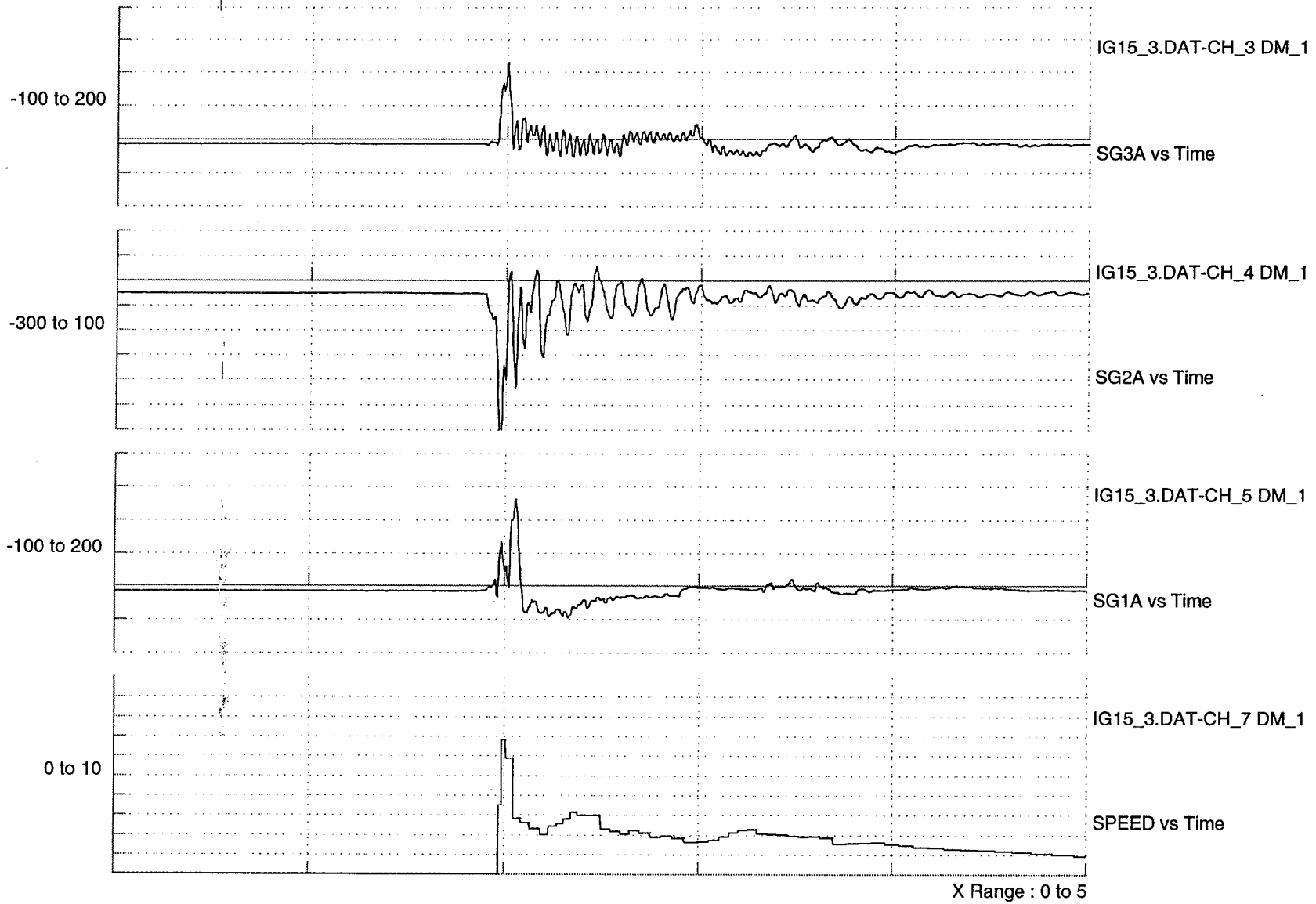
Figure 62. Critical Region Strain Response to Impact
