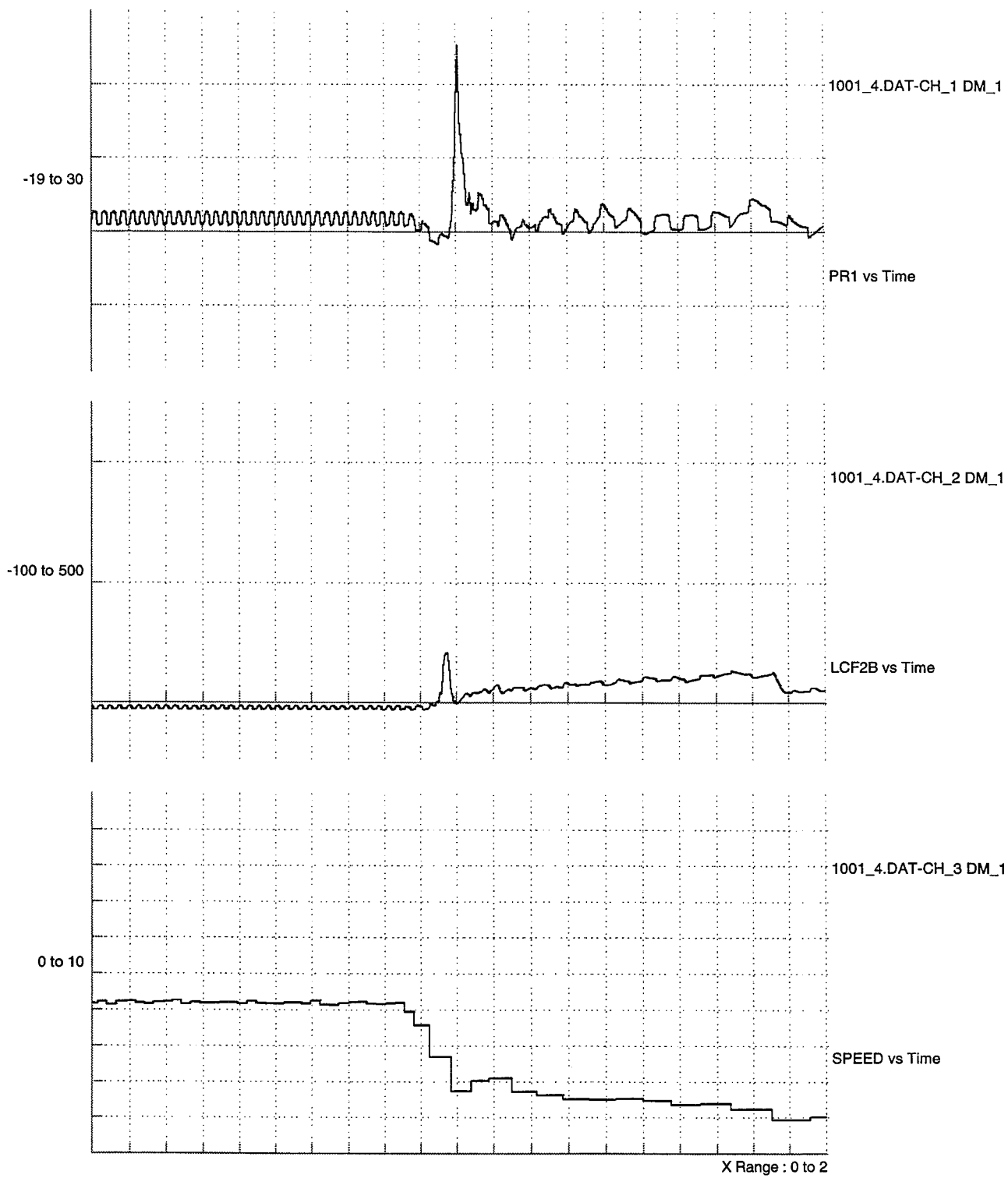
Figure C7. Surge Pressure Event 1 Leg 5
