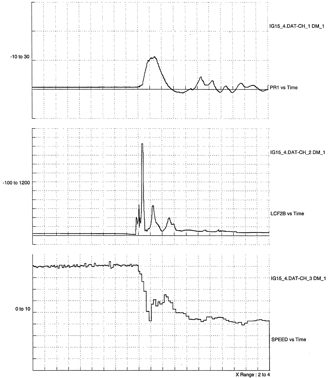
Figure 60. Surge Pressure Repeatability 9 mph
