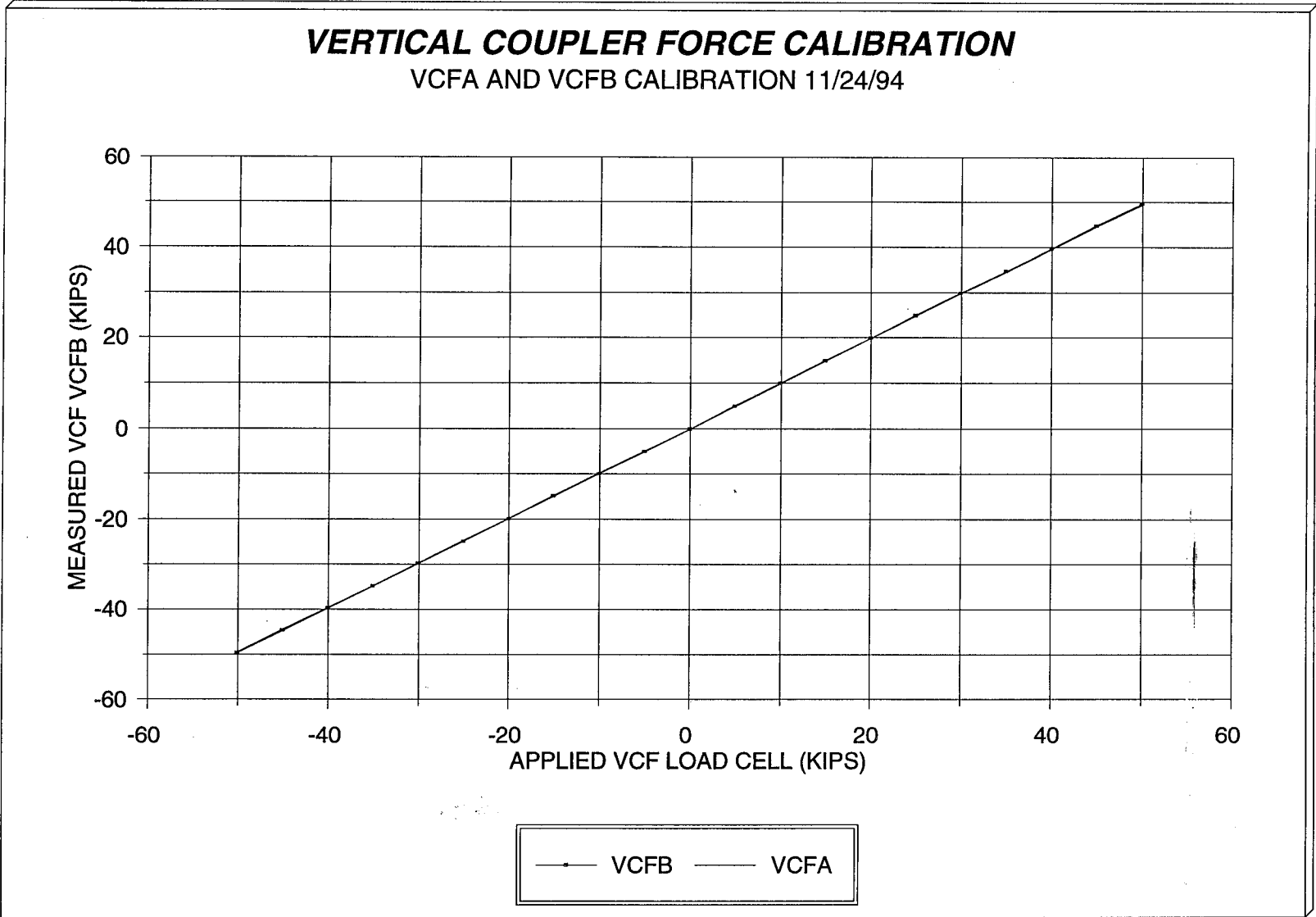
Figure 10. VCFA and VCFB Calibration
