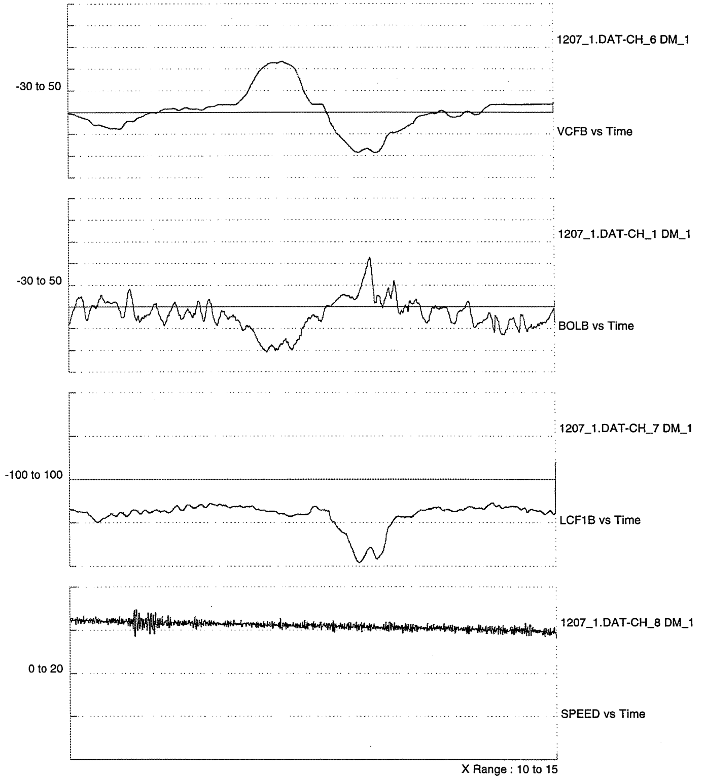
Figure 55. Leg 9 Typical Low Frequency VCF Event
