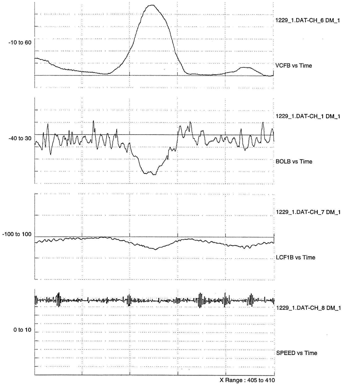
Figure 51. Low Frequency High Magnitude VCF Event
