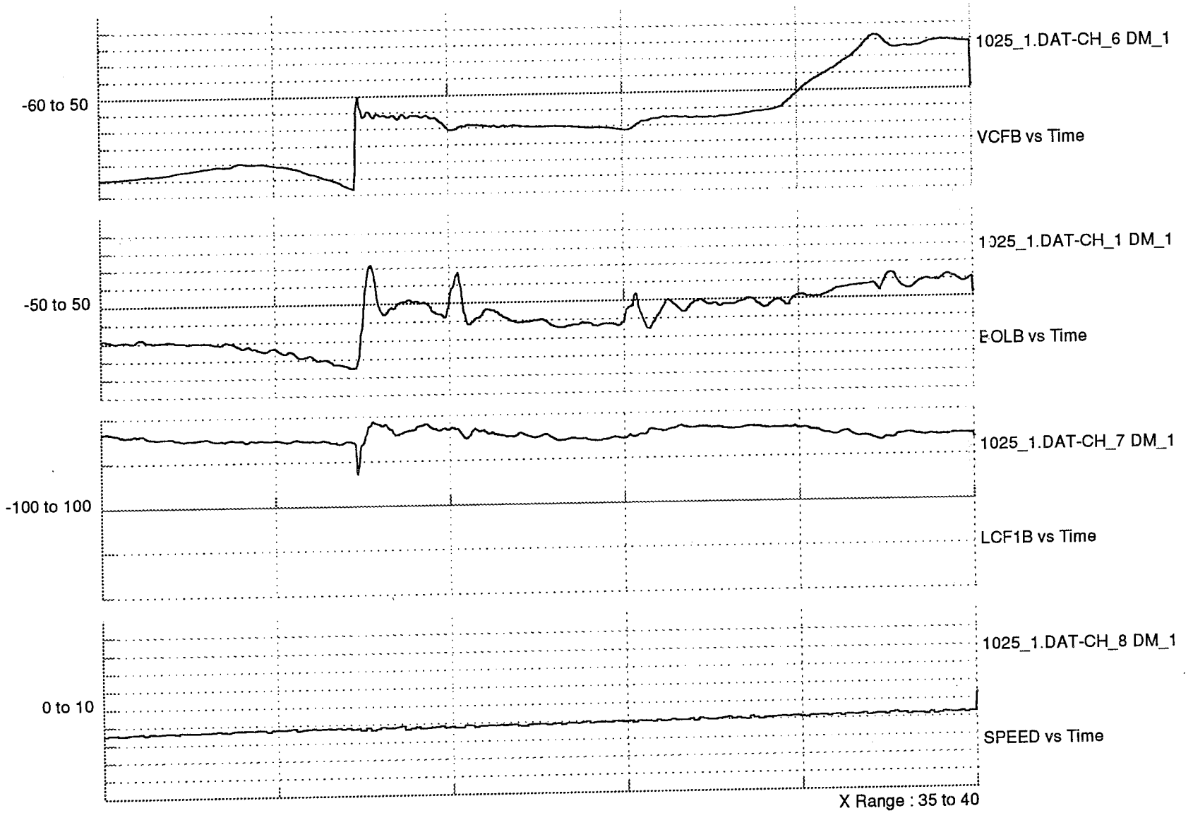
Figure 53. VCF Sticktion Event
