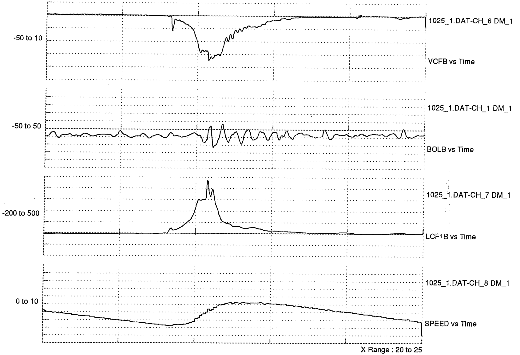
Figure 56. Leg 9 Typical "Smooth" Coupling Event
