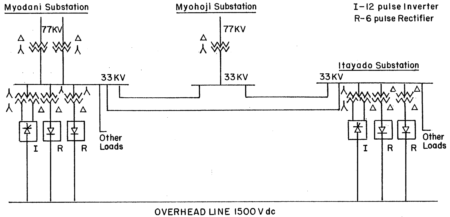
FIGURE A-16. POWER SUPPLY SCHEMATIC AT KOBE SUBWAY
