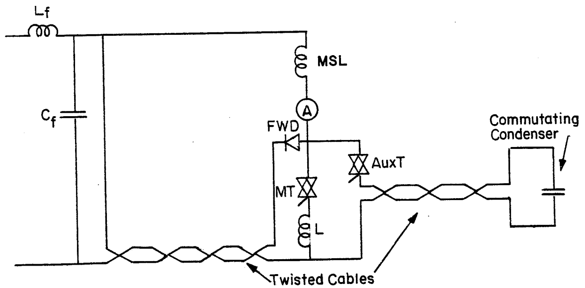
FIGURE 3. USE OF TWISTED CABLES
