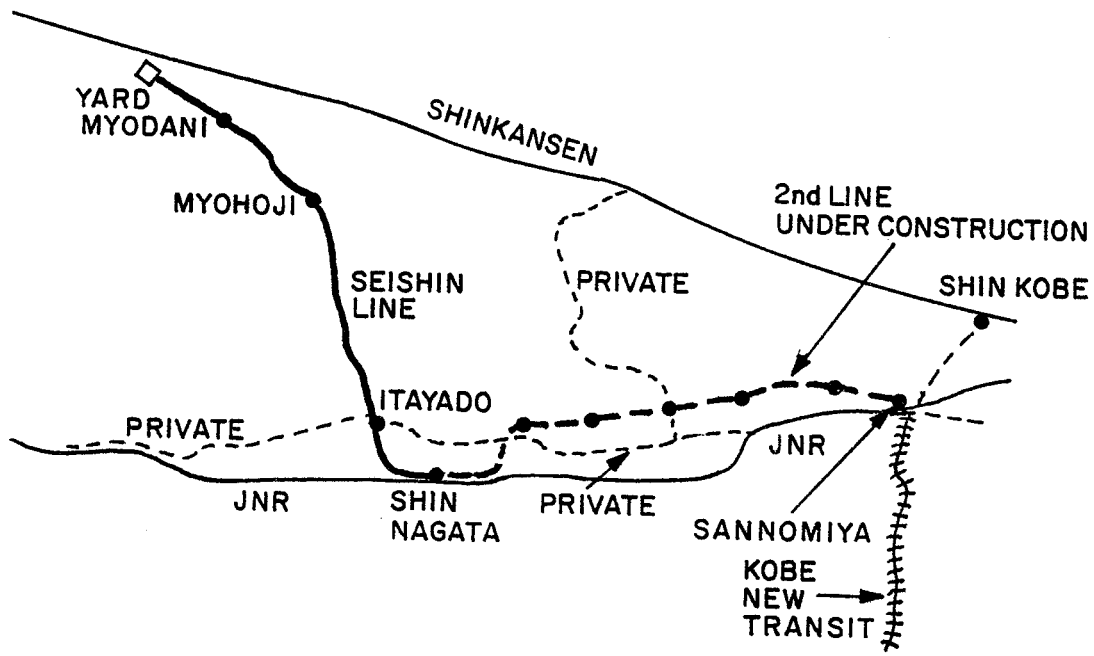
FIGURE A-13. PLANNED NETWORK FOR KOBE SUBWAY
