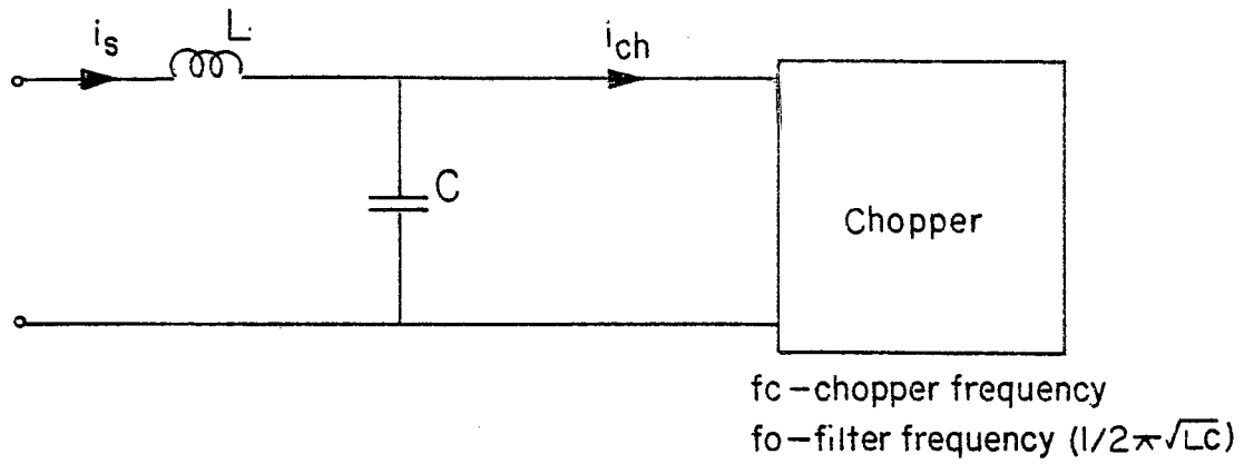
FIGURE 1. ONBOARD FILTERING
