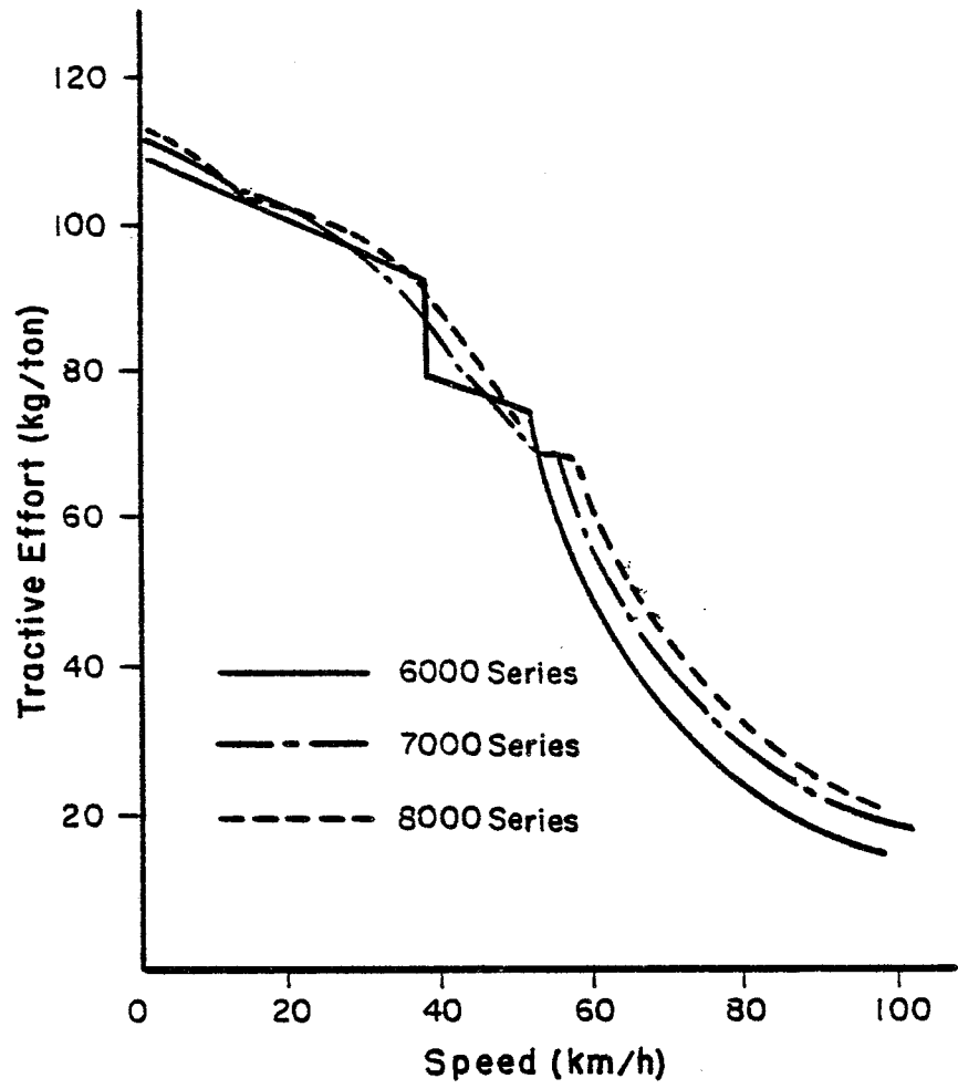
FIGURE 4. CAR PERFORMANCE IN POWERING
