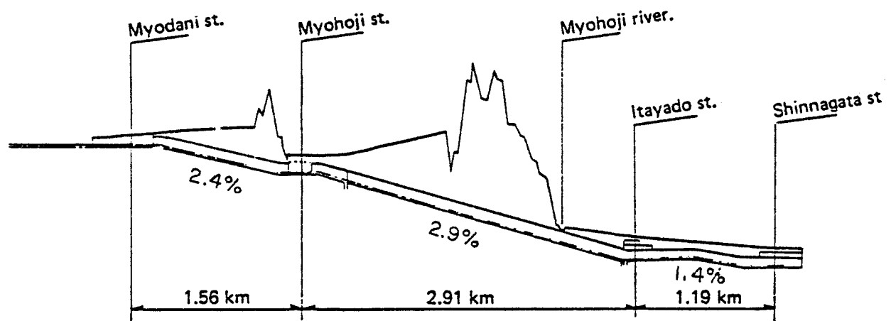
FIGURE A-15. PROFILE OF SEISHIN LINE
