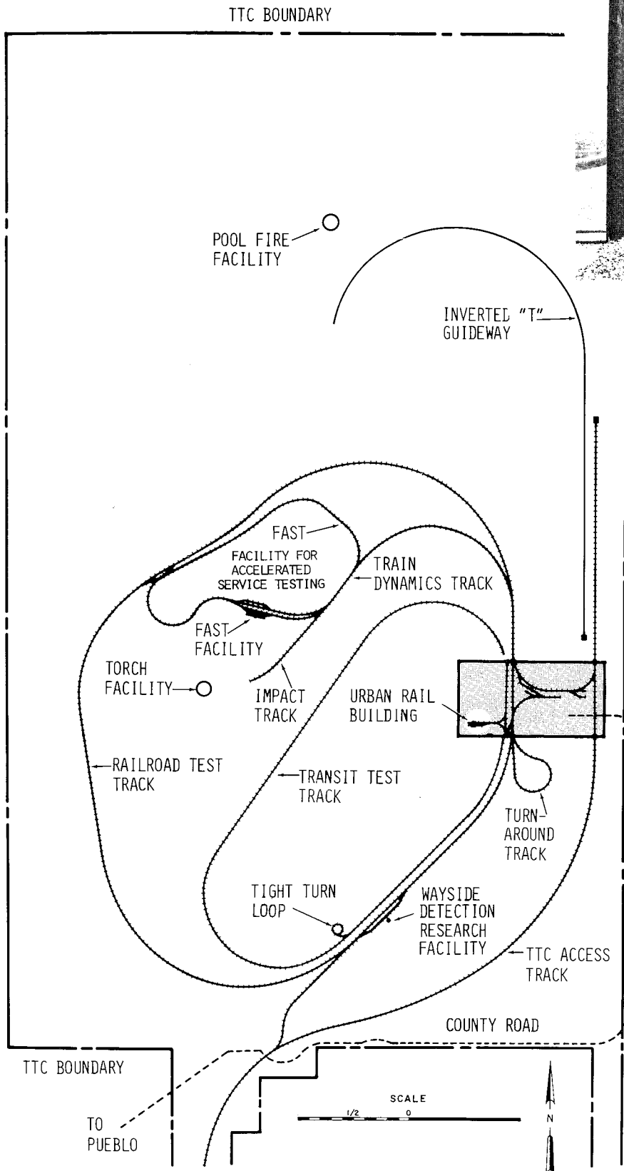
The Transit Test Track is equipped with two miles of simple catenary which can power light rail vehicles.
