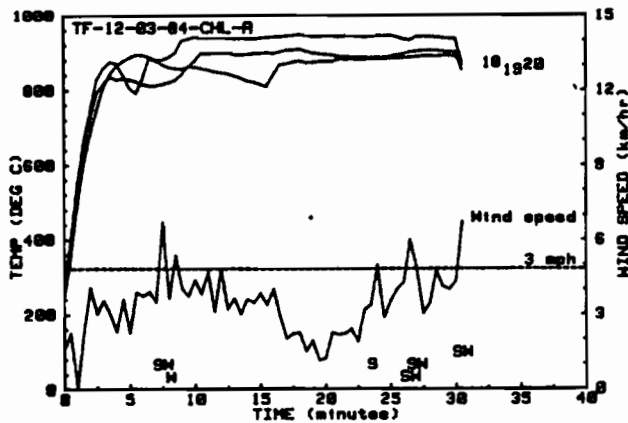
Figure 15: Jacket Temperatures and Wind Speed for the Second Torch Fire Test of Cerawool (C-2)
