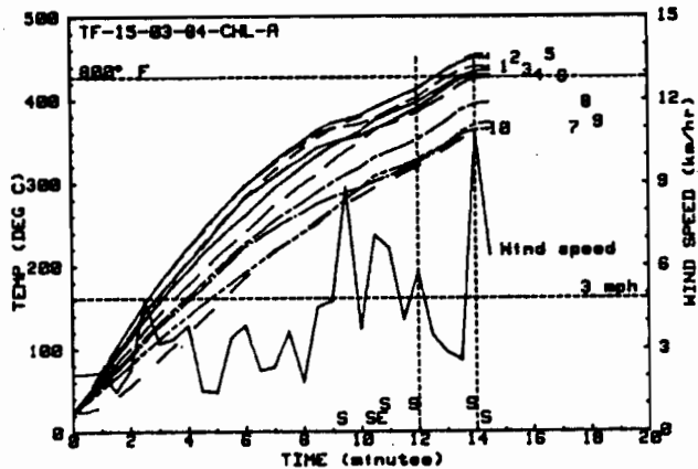
Figure 21: Bare Plate and Rear Enclosure Air Temperatures for the Third Pool Fire Calibration Test
