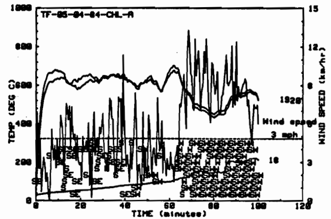
Figure 32: Jacket Temperatures and Wind Speed for the First Pool Fire Test of Kaowool (A-3)
