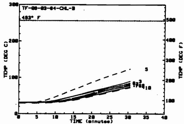
Figure 12: Back Plate and Rear Enclosure Air Temperatures for the Second Torch Fire Test of Fiberfrax (B-2)
