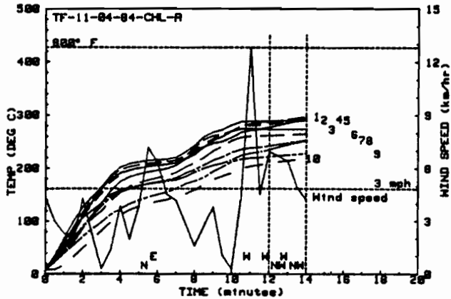
Figure 27: Bare Plate and Rear Enclosure Air Temperatures for the Ninth Pool Fire Calibration Test
