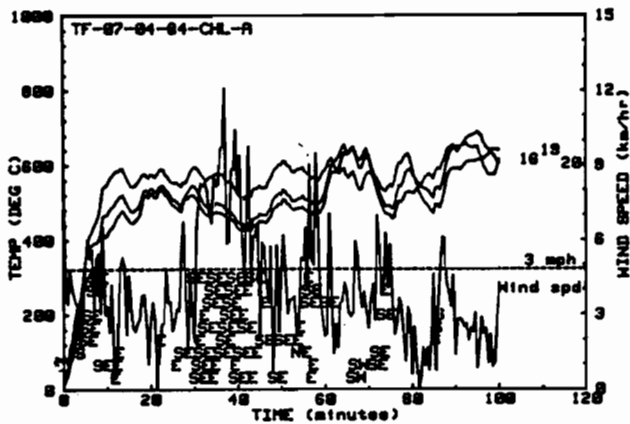
Figure 34: Jacket Temperatures and Wind Speed for the Second Pool Fire Test of Kaowool (A-4)
