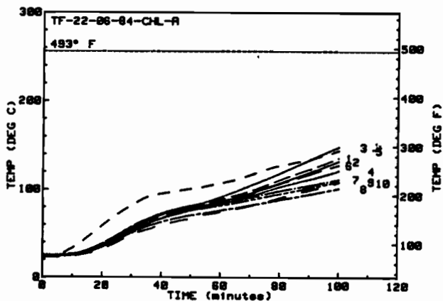
Figure 45: Back Plate and Rear Enclosure Air Temperatures for Third Pool Fire Test of Fiberfrax (B-5)
