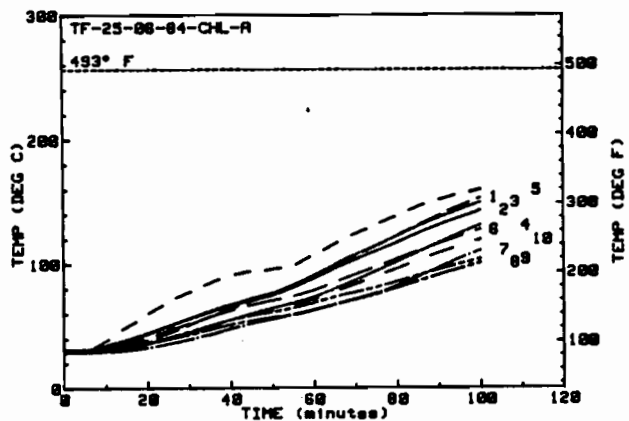
Figure 47: Back Plate and Rear Enclosure Air Temperatures for the First Pool Fire Test of Cerawool (C-4)
