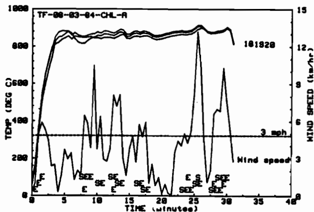
Figure 7: Jacket Temperatures and Wind Speed For the Second Torch Fire Test of Kaowool (A-2)
