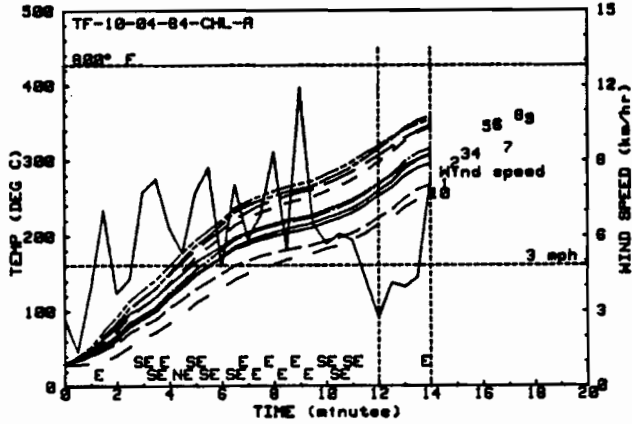
Figure 25: Bare Plate and Rear Enclosure Air Temperatures for the Seventh Pool Fire Calibration Test
