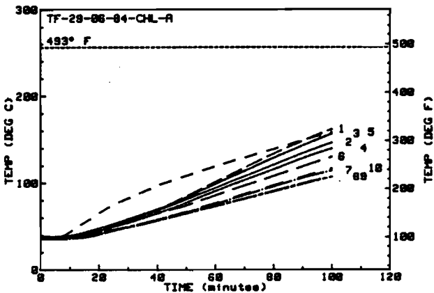
Figure 51: Back Plate and Rear Enclosure Air Temperatures for the Third Pool Fire Test of Cerawool C-6)
