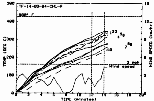
Figure 20: Bare Plate and Rear Enclosure Air Temperatures for the Second Pool Fire Calibration Test
