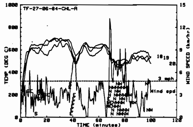
Figure 48: Jacket Temperatures and Wind Speed for the Second Pool Fire Test of Cerawool (C-5)
