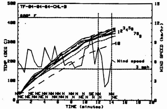
Figure 23: Bare Plate and Rear Enclosure Air Temperatures for the Fifth Pool Fire Calibration Test
