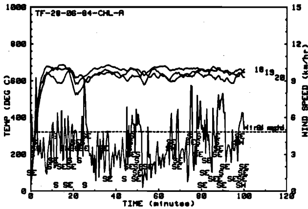
Figure 50: Jacket Temperatures and Wind Speed for the Third Pool Fire Test of Cerawool (C-6)
