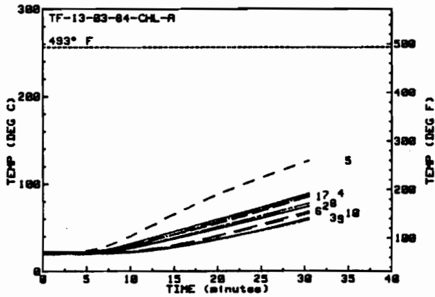
Figure 18: Back Plate and Rear Enclosure Air Temperatures for the Third Torch Fire Test of Cerawool (C-3)
