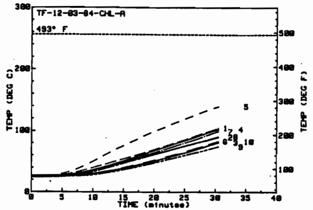
Figure 16: Back Plate and Rear Enclosure Air Temperatures for the Second Torch Fire Test of Cerawool (C-2)
