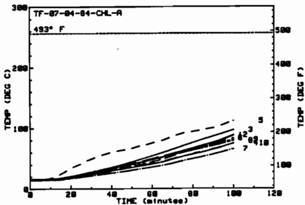
Figure 35: Back Plate and Rear Enclosure Air Temperatures for the Second Pool Fire Test of Kaowool (A-4)
