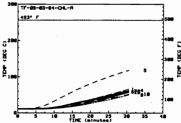
Figure 10: Back Plate and Rear Enclosure Air Temperatures for the First Torch Fire Test of Fiberfrax (B-1)
