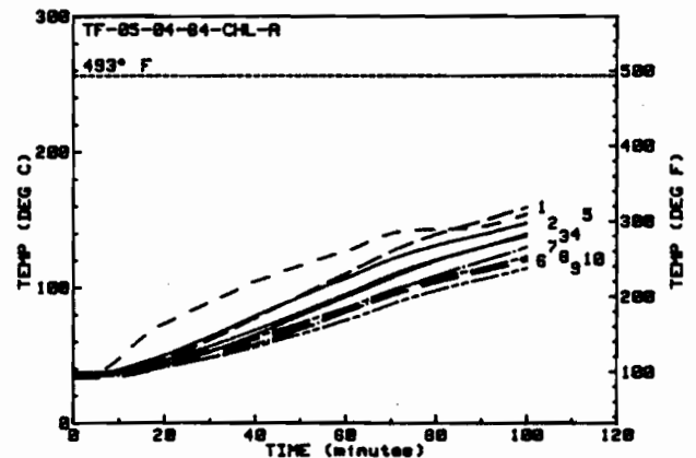
Figure 33: Back Plate and Rear Enclosure Air Temperatures for the First Pool Fire Test of Kaowool (A-3)
