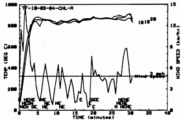
Figure 13: Jacket Temperatures and Wind Speed for the First Torch Fire Test of Cerawool (C-1)
