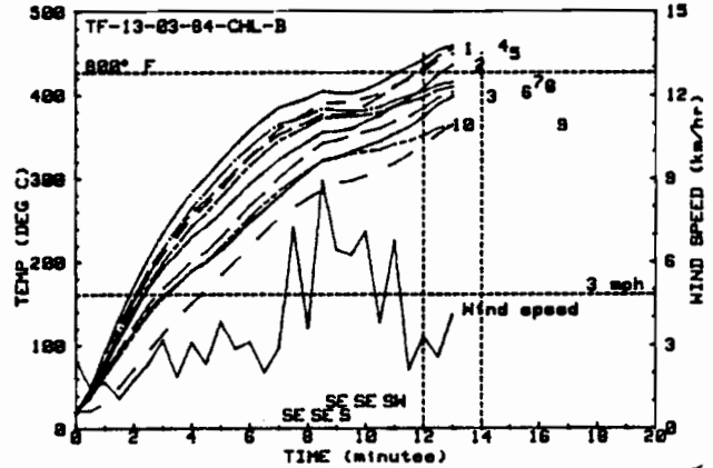
Figure 19: Bare Plate and Rear Enclosure Air Temperatures for the First Pool Fire Calibration Test
