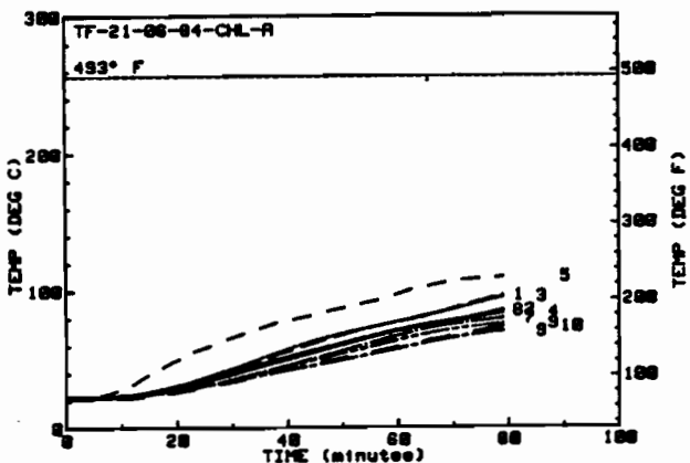
Figure 43: Back Plate and Rear Enclosure Air Temperatures for the Second Pool Fire Test of Fiberfrax (B-4)
