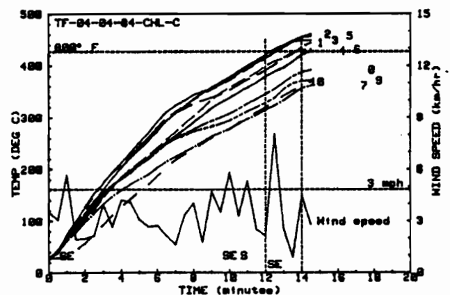
Figure 24: Bare Plate and Rear Enclosure Air Temperatures for the Sixth Pool Fire Calibration Test
