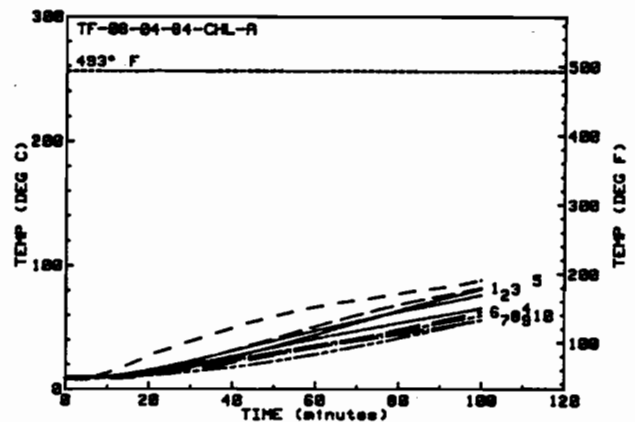
Figure 37: Back Plate and Rear Enclosure Air Temperatures for the Third Pool Fire Test of Kaowool (A-5)
