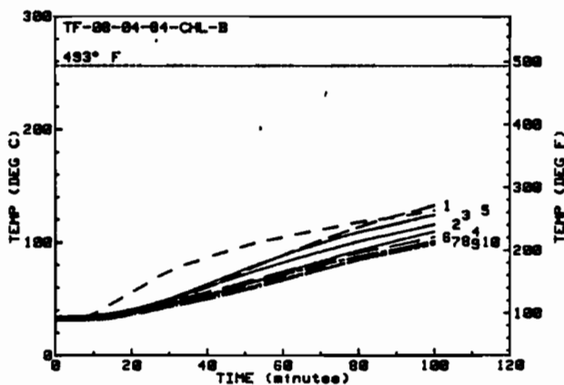
Figure 39: Back Plate and Rear Enclosure Air Temperatures for the Fourth Pool Fire Test of Kaowool (A-6)
