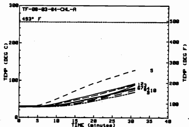
Figure 8: Back Plate and Rear Enclosure Air Temperatures for the Second Torch Fire Test of Kaowool (A-2)
