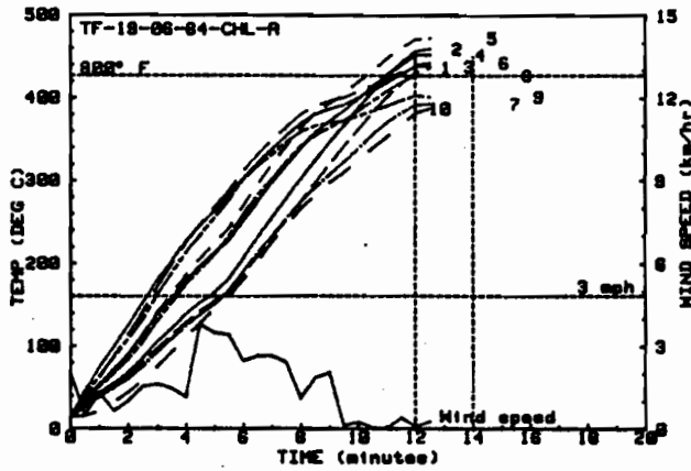
Figure 31: Bare Plate and Rear Enclosure Air Temperatures for the Thirteenth Pool Fire Calibration Test
