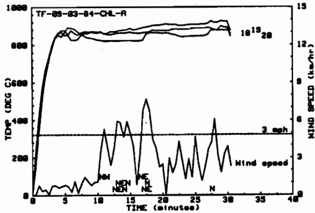
Figure 9: Jacket Temperatures and Wind Speed for the First Torch Fire Test of Fiberfrax (B-1)
