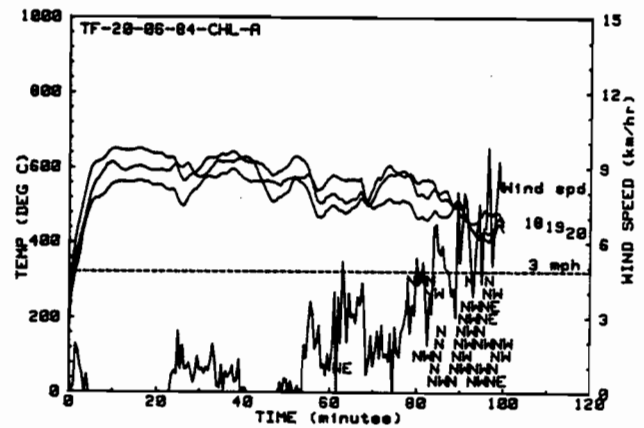
Figure 40: Jacket Temperatures and Wind Speed for the First Pool Fire Test of Fiberfrax (B-3)
