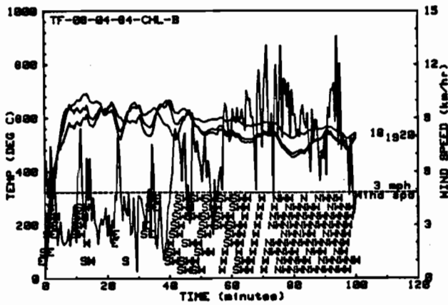
Figure 38: Jacket Temperatures and Wind Speed for the Fourth Test Pool Fire Test of Kaowool (A-6)
