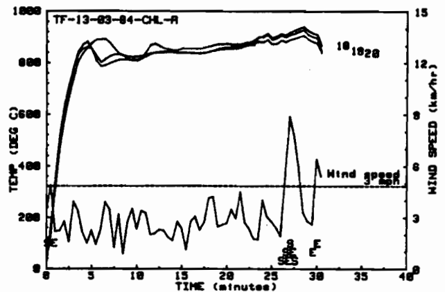
Figure 17: Jacket Temperatures and Wind Speed for the Third Torch Fire Test of Cerawool (C-3)
