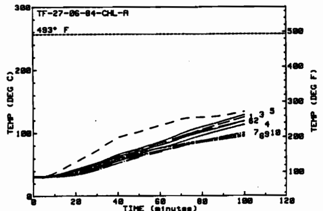
Figure 49: Back Plate and Rear Enclosure Air Temperatures for the Second Pool Test of Cerawool (C-5)
