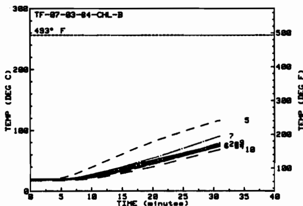
Figure 6: Back Plate and Rear Enclosure Air Temperatures for the First Torch Fire Test of Kaowool (A-1)
