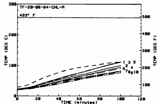
Figure 41: Back Plate and Rear Enclosure Air Temperatures for the First Pool Fire Test of Fiberfrax (B-3)
