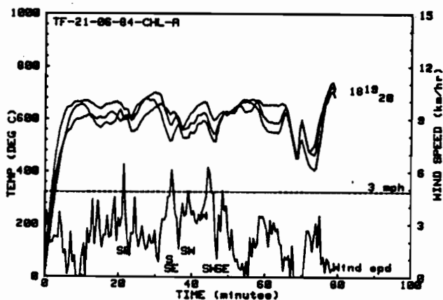
Figure 42: Jacket Temperatures and Wind Speed for the Second Pool Fire Test of Fiberfrax (B-4)
