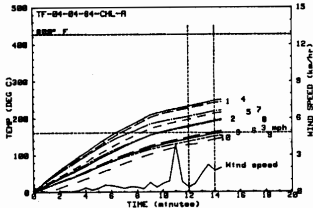
Figure 22: Bare Plate and Rear Enclosure Air Temperatures for the Fourth Pool Fire Calibration Test
