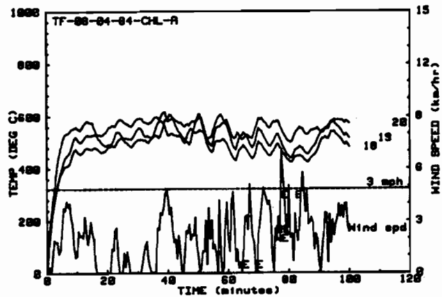
Figure 36: Jacket Temperatures and Wind Speed for the Third Pool Fire Test of Kaowool (A-5)
