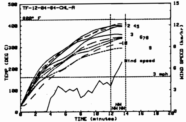
Figure 29: Bare Plate and Rear Enclosure Air Temperatures for the Eleventh Pool Fire Calibration Test
