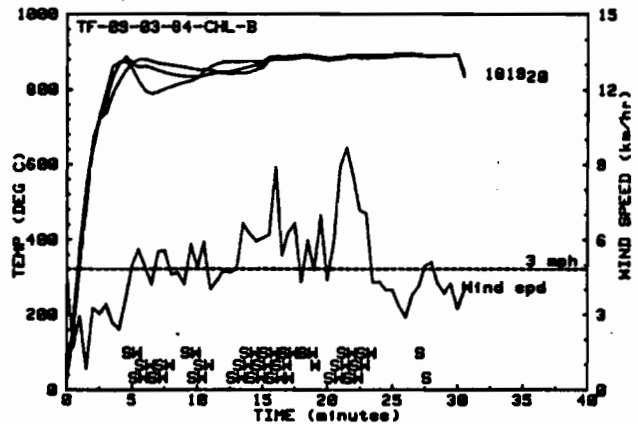
Figure 11: Jacket Temperatures and Wind Speed for the Second Torch Fire Test of Fiberfrax (B-2)
