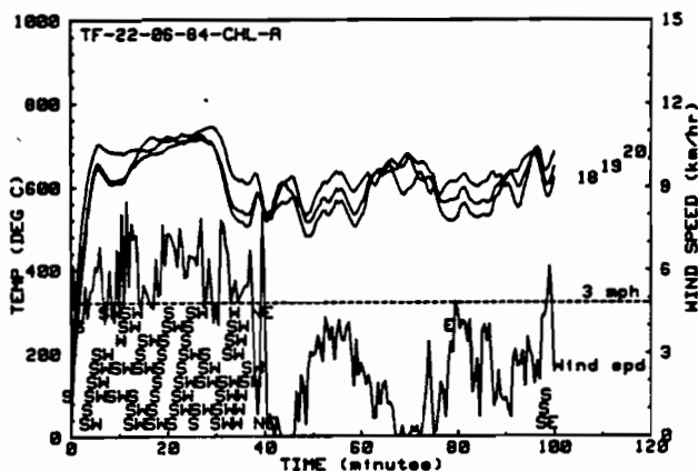
Figure 44: Jacket Temperatures and Wind Speed for the Third Pool Fire Test of Fiberfrax (B-5)
