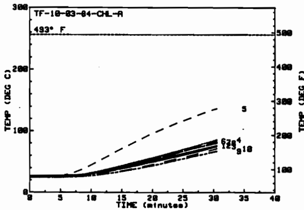
Figure 14: Back Plate and Rear Enclosure Air Temperatures for the First Torch Fire Test of Cerawool (C-1)
