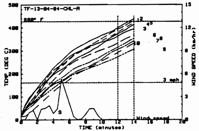
Figure 30: Bare Plate and Rear Enclosure Air Temperatures for the Twelfth Pool Fire Calibration Test
