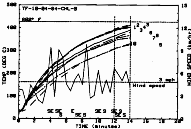
Figure 26: Bare Plate and Rear Enclosure Air Temperatures for the Eighth Pool Fire Calibration Test
