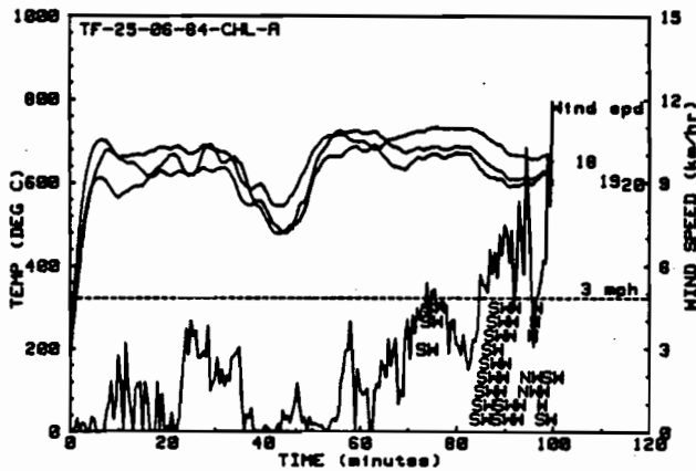
Figure 46: Jacket Temperatures and Wind Speed for the First Pool Fire Test of Cerawool (C-4)
