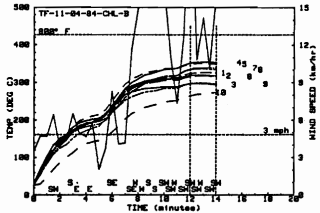
Figure 28: Bare Plate and Rear Enclosure Air Temperatures for the Tenth Pool Fire Calibration Test
