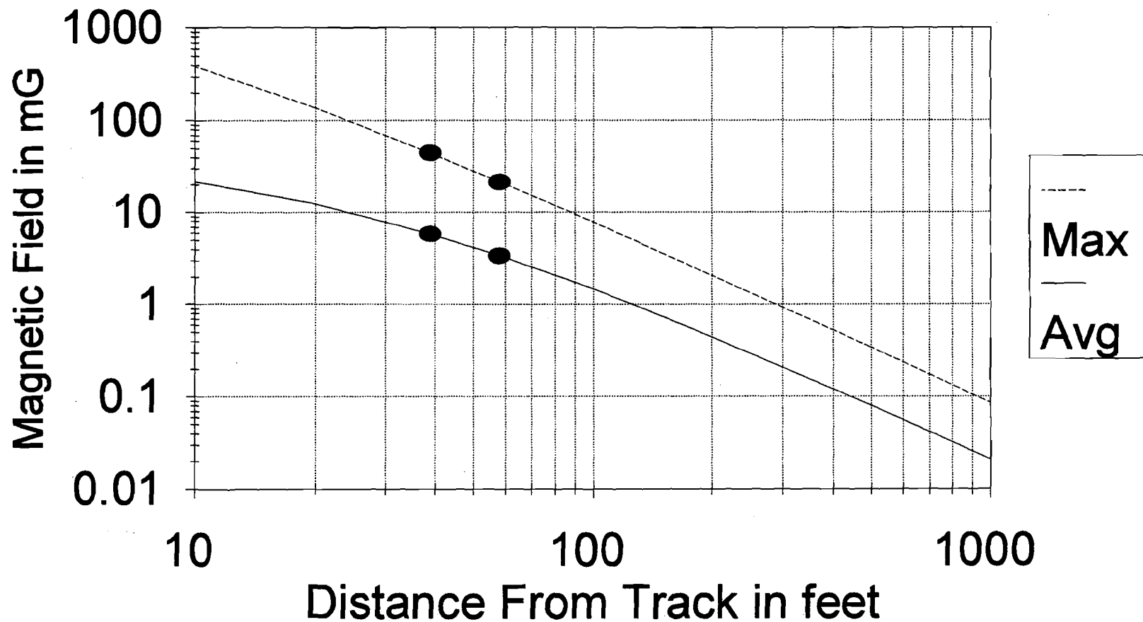
FIGURE 5-10. THEORETICAL ATTENUATION CURVES FITTED THROUGH THE AVERAGE AND MAXIMUM MAGNETIC FIELD VALUES MEASURED AT THE WAYSIDE OF THE 60 HZ SECTION OF THE NEC AT RYE, NY
