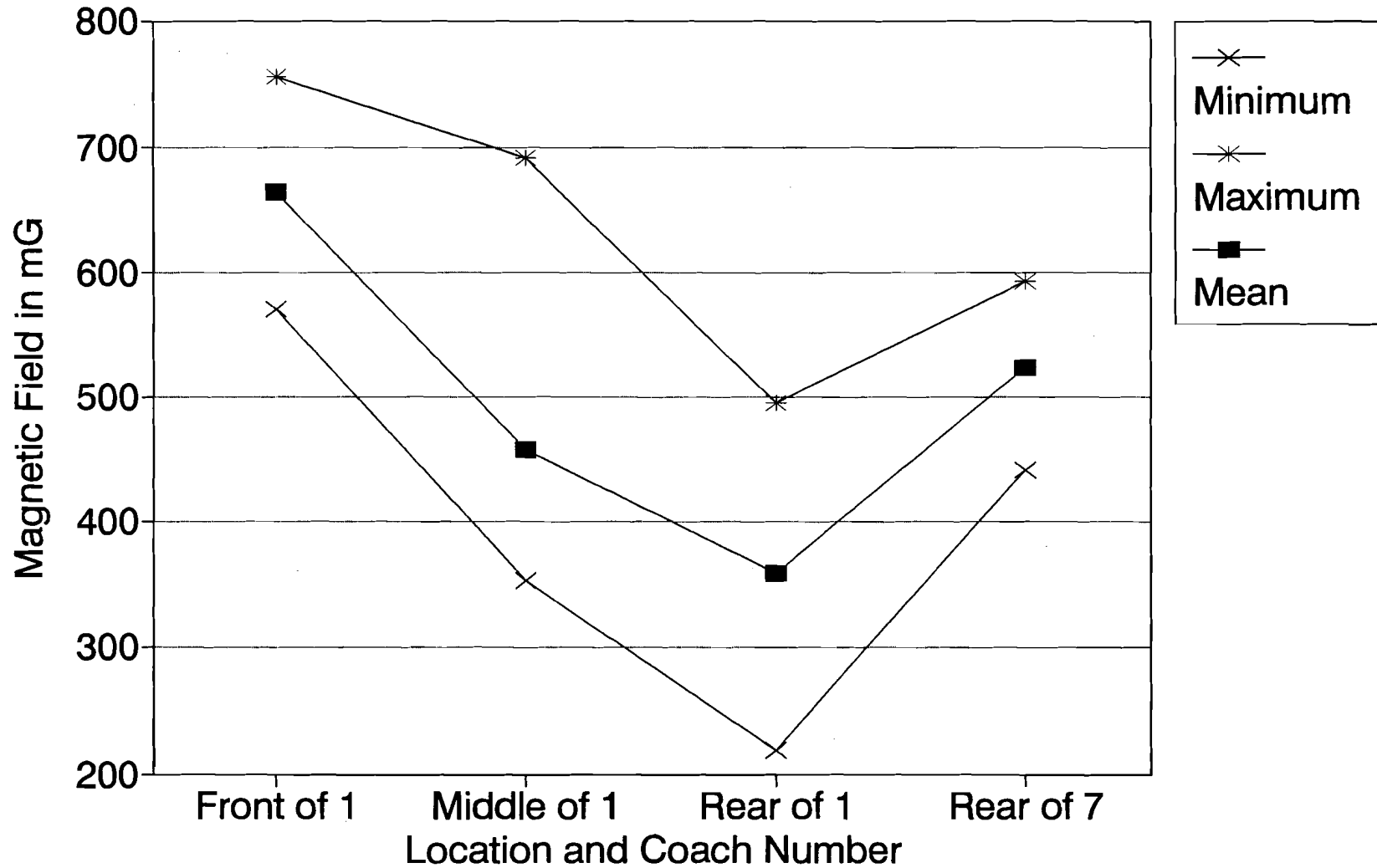
FIGURE 3-12. STATIC MAGNETIC FIELD AT VARIOUS LOCATIONS
