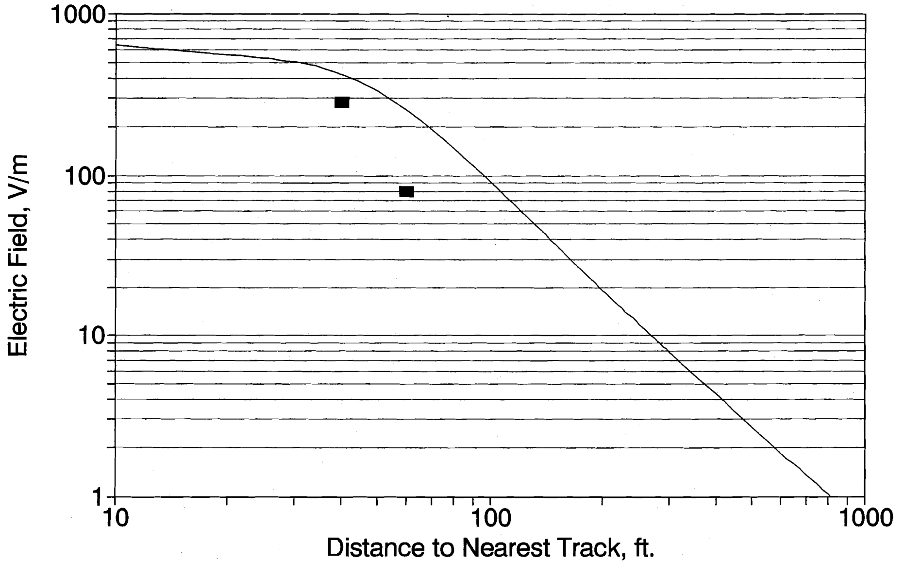
FIGURE 5-13. CALCULATED AND MEASURED 25 HZ ELECTRIC FIELD LEVELS AT THE WAYSIDE OF THE 25 HZ SECTION OF THE NEC AT THE PRINCETON JUNCTION MEASUREMENT SITE
