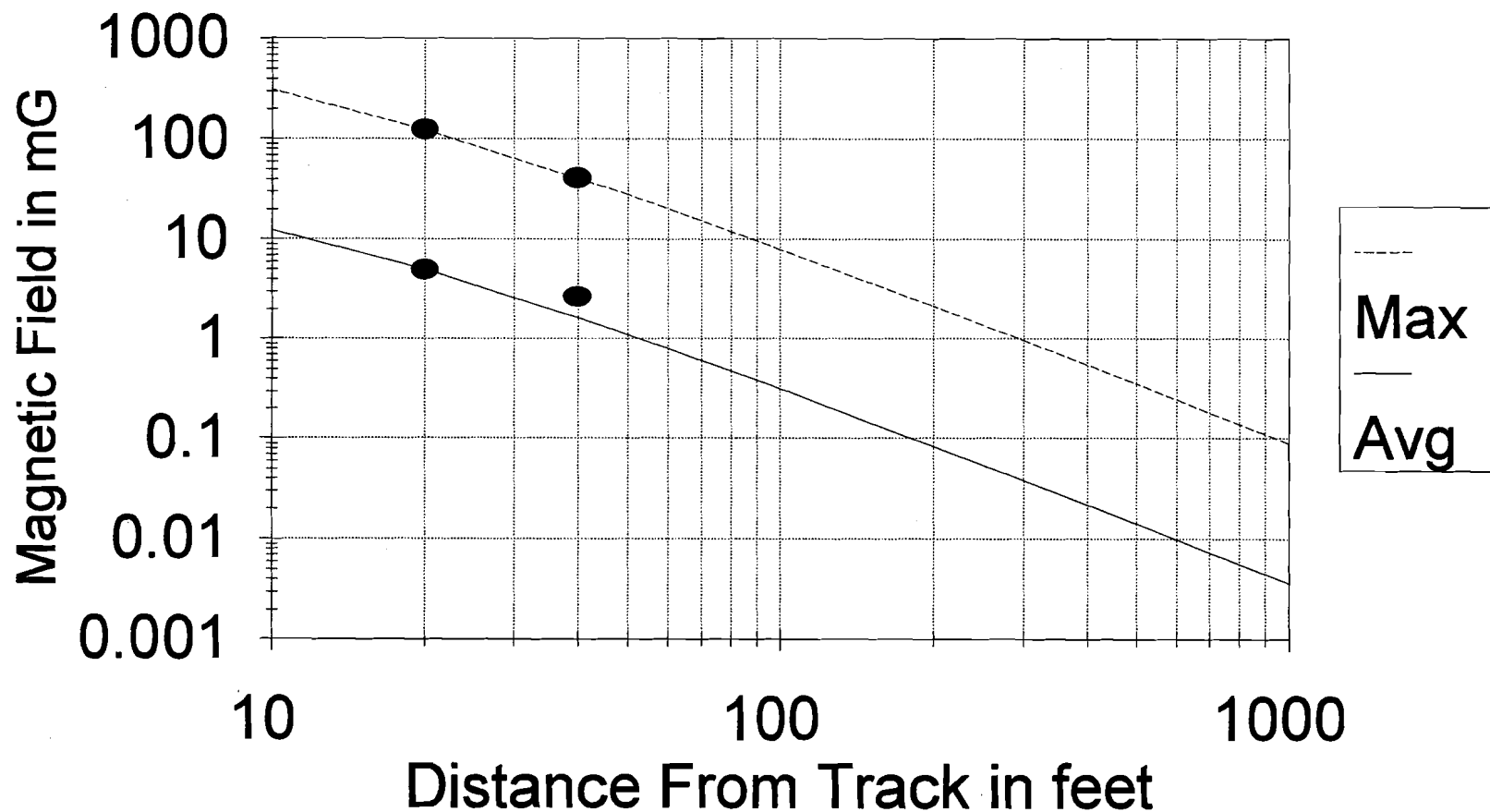
FIGURE 5-11. THEORETICAL ATTENUATION CURVES FITTED THROUGH THE AVERAGE AND MAXIMUM MAGNETIC FIELD VALUES MEASURED AT THE SOUTH SIDE OF THE NORTH JERSEY COAST LINE NEAR RED BANK, NJ
