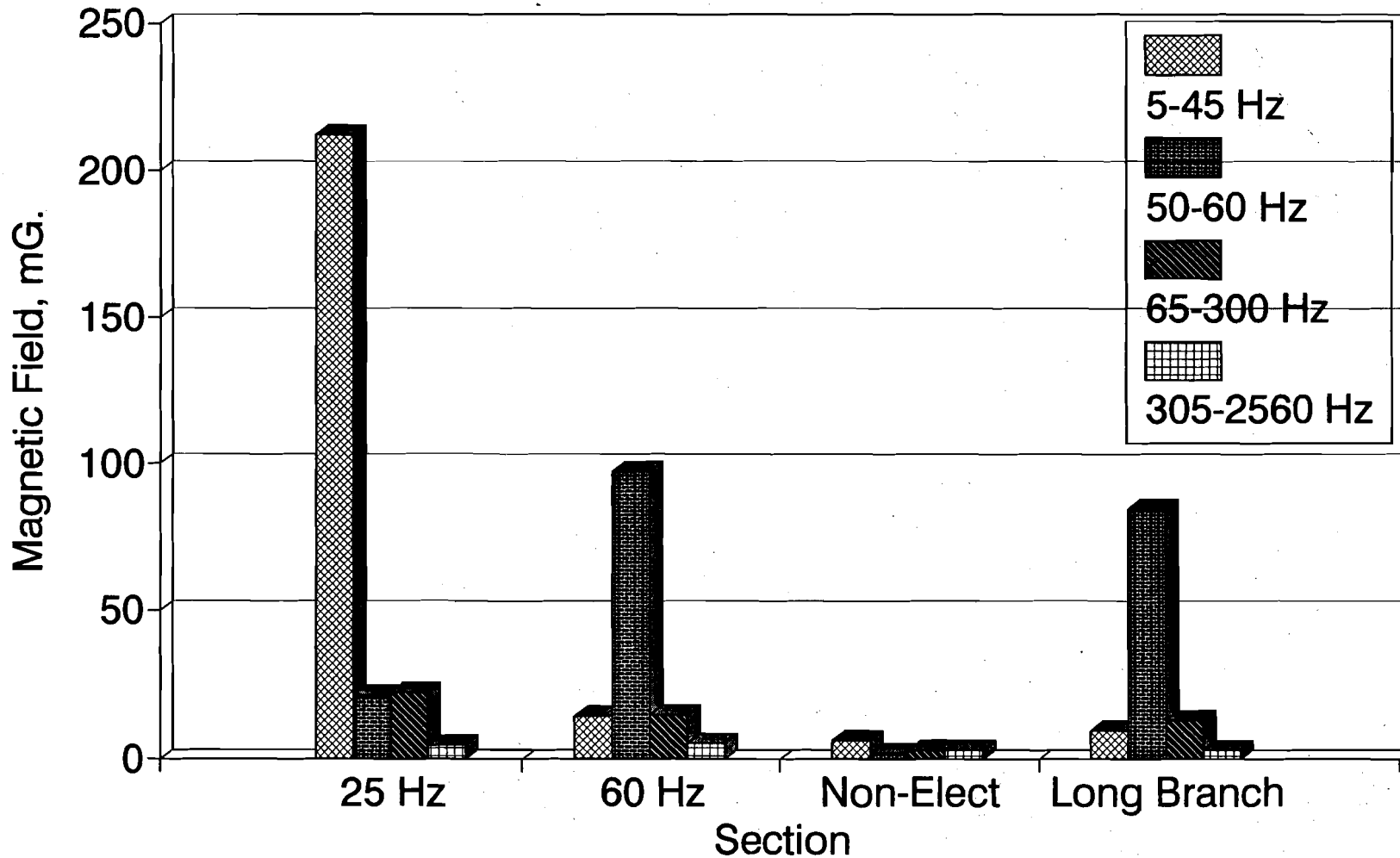
FIGURE 4-24. COMPARISON OF MAXIMUM TIME-VARYING MAGNETIC FIELD LEVELS IN FOUR FREQUENCY BANDS AT TYPICAL LOCATIONS IN CABS OF LOCOMOTIVES OPERATING ON VARIOUS SECTIONS OF THE NEC OR ON THE NORTH JERSEY COAST LINE
