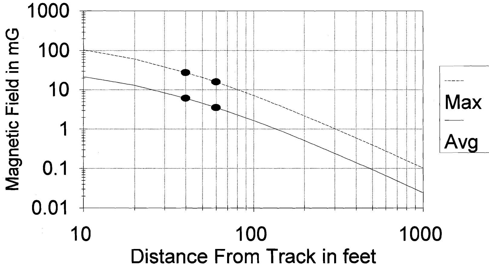
FIGURE 5-9. THEORETICAL ATTENUATION CURVES FITTED THROUGH THE AVERAGE AND MAXIMUM MAGNETIC FIELD VALUES MEASURED AT THE WAYSIDE OF THE 25 HZ SECTION OF THE NEC AT PRINCETON JUNCTION, NJ
