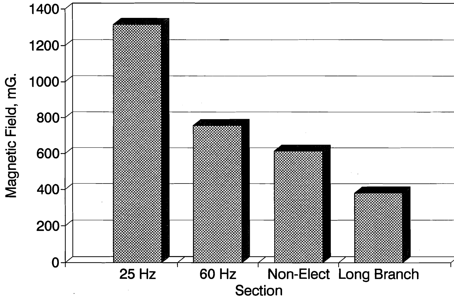
FIGURE 4-18. COMPARISON OF THE MAXIMUM STATIC MAGNETIC FIELD LEVEL TYPICAL FOR A LOCATION IN THE CABS OF LOCOMOTIVES OPERATING ON VARIOUS SECTIONS OF THE NORTHEAST CORRIDOR AND ON THE NORTH JERSEY COAST LINE
