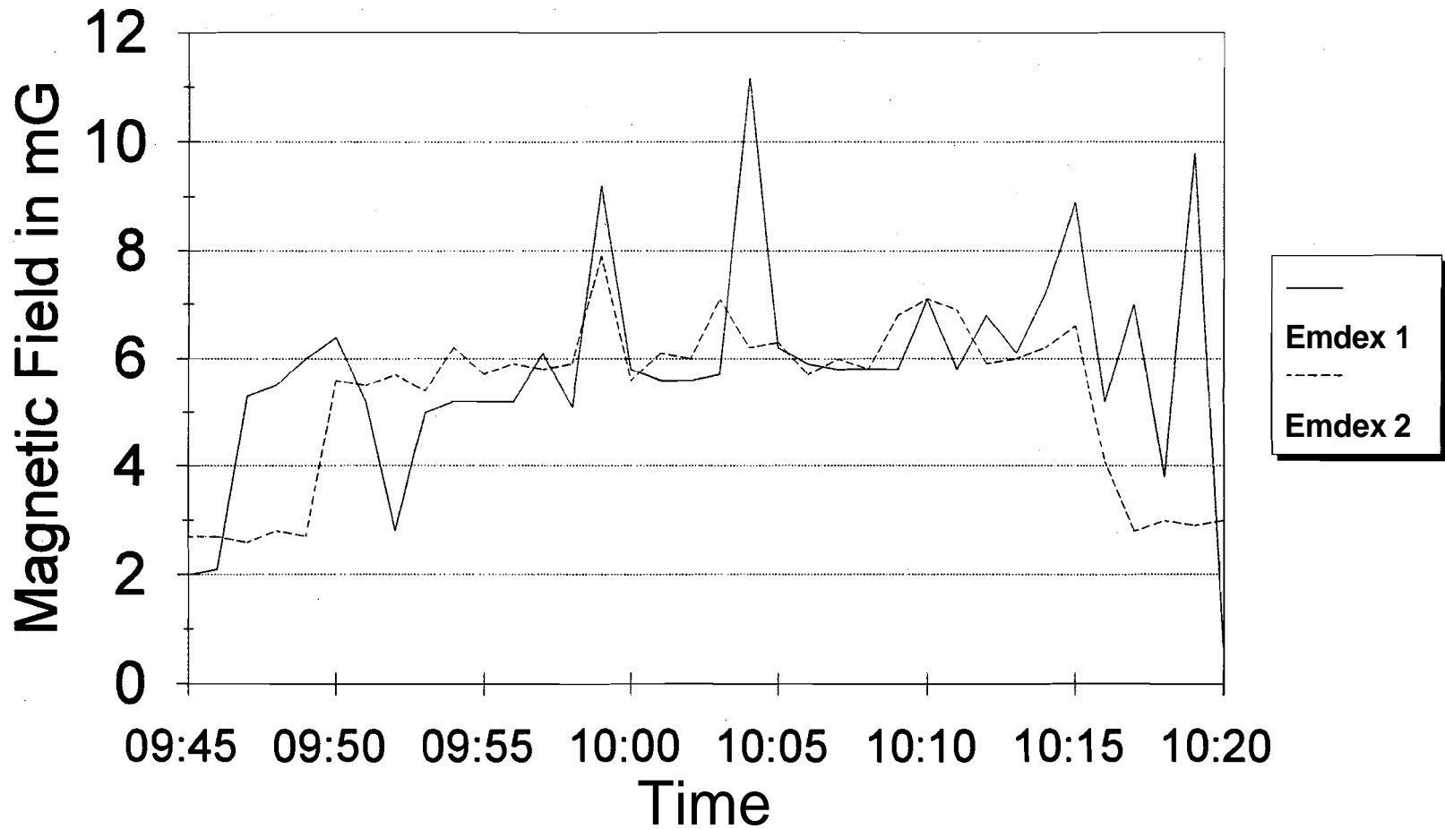
FIGURE 7-11. RMS RECORDINGS OF THE MAGNETIC FIELD LEVELS ENCOUNTERED BY TWO RESEARCHERS WORKING OUTSIDE THE RED BANK SUBSTATION BENEATH THE INCOMING 345 KV TRANSMISSION LINE
