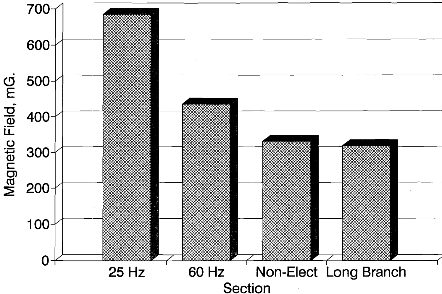
FIGURE 4-17. COMPARISON OF THE AVERAGE STATIC MAGNETIC FIELD LEVELS IN CABS OF LOCOMOTIVES OPERATING ON VARIOUS SECTIONS OF THE NEC AND ON THE NORTH JERSEY COAST LINE
