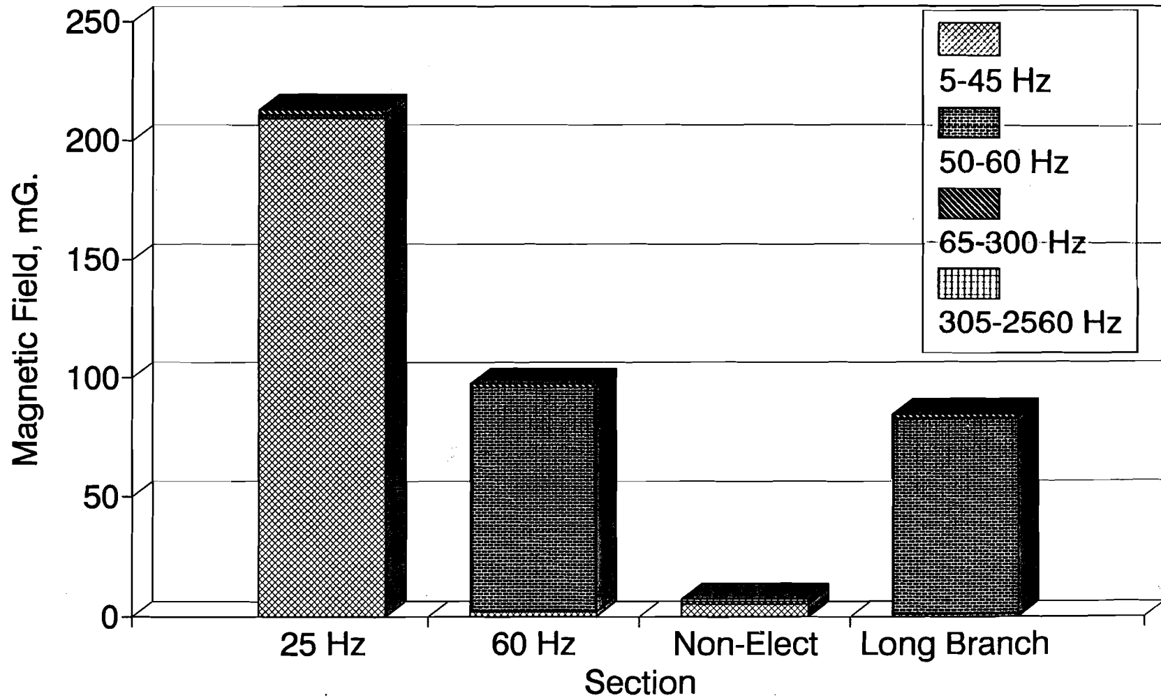
FIGURE 4-22. COMPARISON OF THE MAXIMUM TIME-VARYING MAGNETIC FIELD LEVELS IN TYPICAL LOCATIONS IN CABS OF LOCOMOTIVES OPERATING ON VARIOUS SECTIONS OF THE NEC OR THE NORTH JERSEY COAST LINE AND THE PRINCIPAL COMPONENT FREQUENCY RANGES
