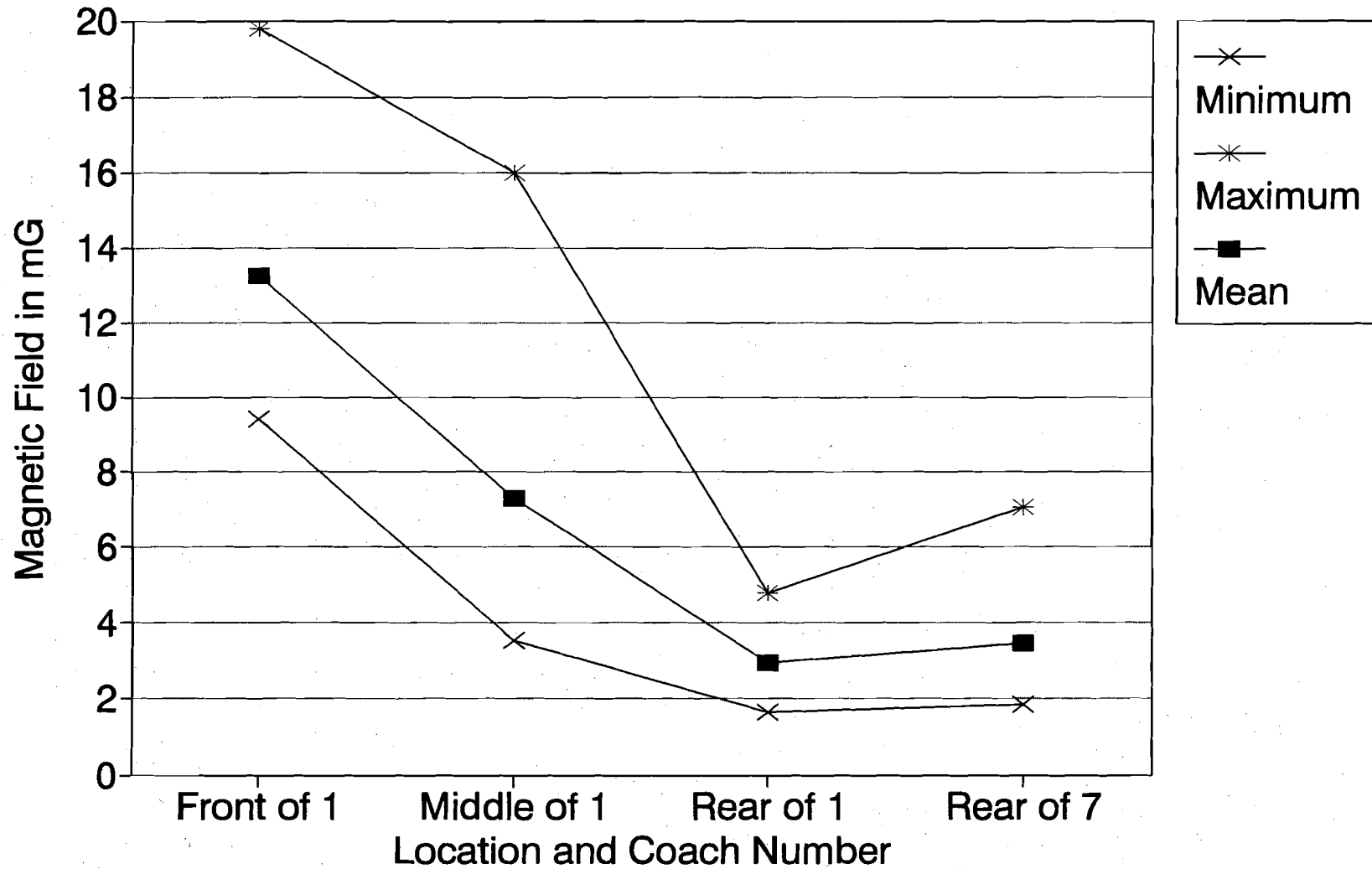
FIGURE 3-6. POWER FREQUENCY MAGNETIC FIELD LEVELS AT VARIOUS LOCATIONS ALONG THE 25 HZ NEC SEGMENT
