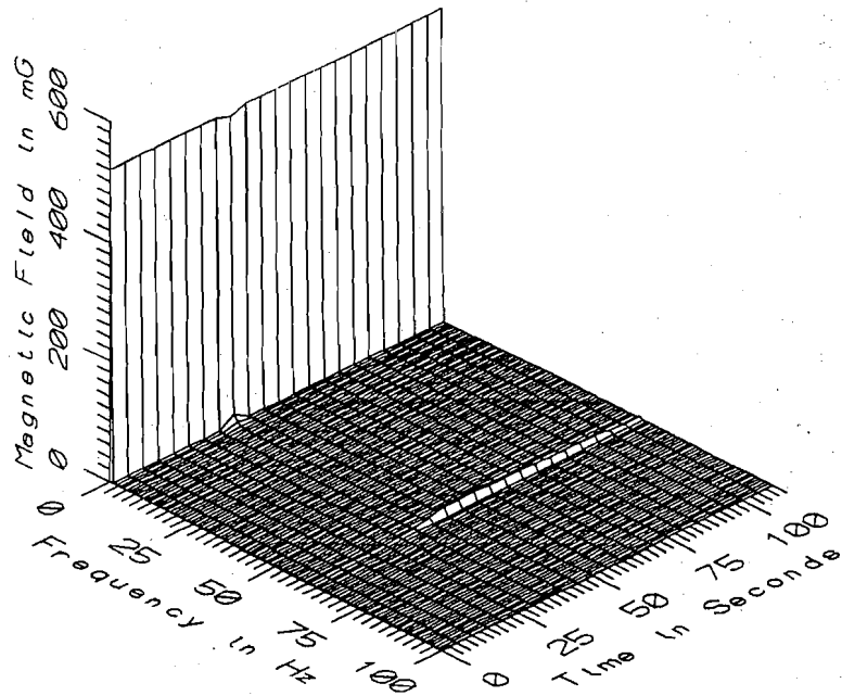
NEC053 - 10 cm ABOVE GROUND, 20FT FROM CENTERLINE OF TRACK
