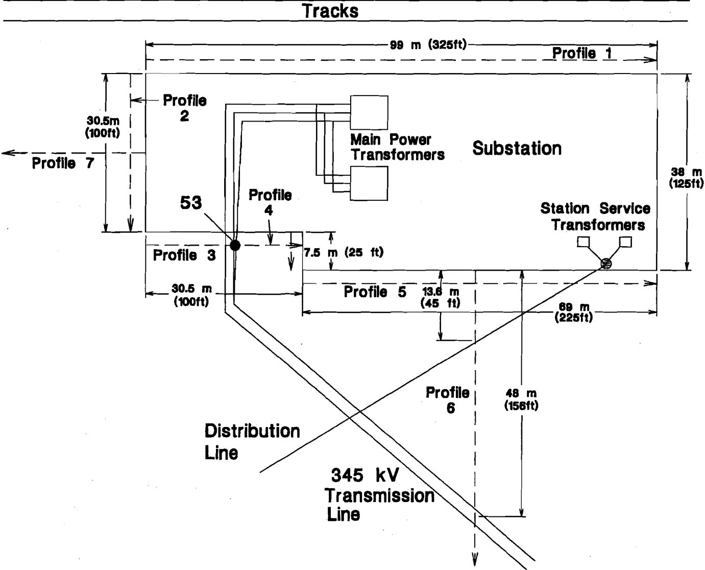
FIGURE 7-3. MAGNETIC FIELD MEASUREMENT LOCATIONS AT THE RED BANK SUBSTATION
