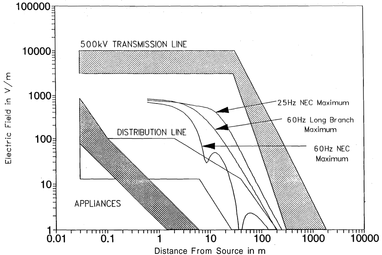
FIGURE 9-8. MAXIMUM TIME-VARYING ELECTRIC FIELD AT THE WAYSIDE OF ELECTRIFIED RAILROADS AS A FUNCTION OF DISTANCE FROM THE NEAREST TRACK COMPARED TO TYPICAL LEVELS OF POWER-FREQUENCY ELECTRIC FIELDS PRODUCED BY COMMON SOURCES
