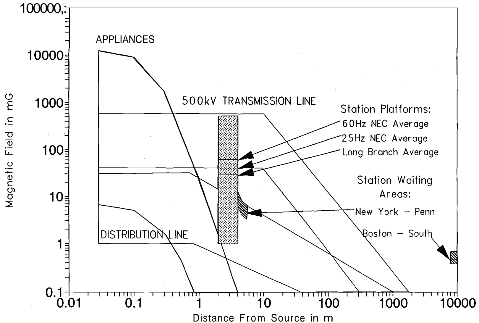
FIGURE 9-9. THE RANGE OF TOTAL TIME-VARYING MAGNETIC FIELD LEVELS ON STATION PLATFORMS OR IN STATION WAITING AREAS COMPARED TO TYPICAL POWER-FREQUENCY MAGNETIC FIELD LEVELS FROM COMMON SOURCES
