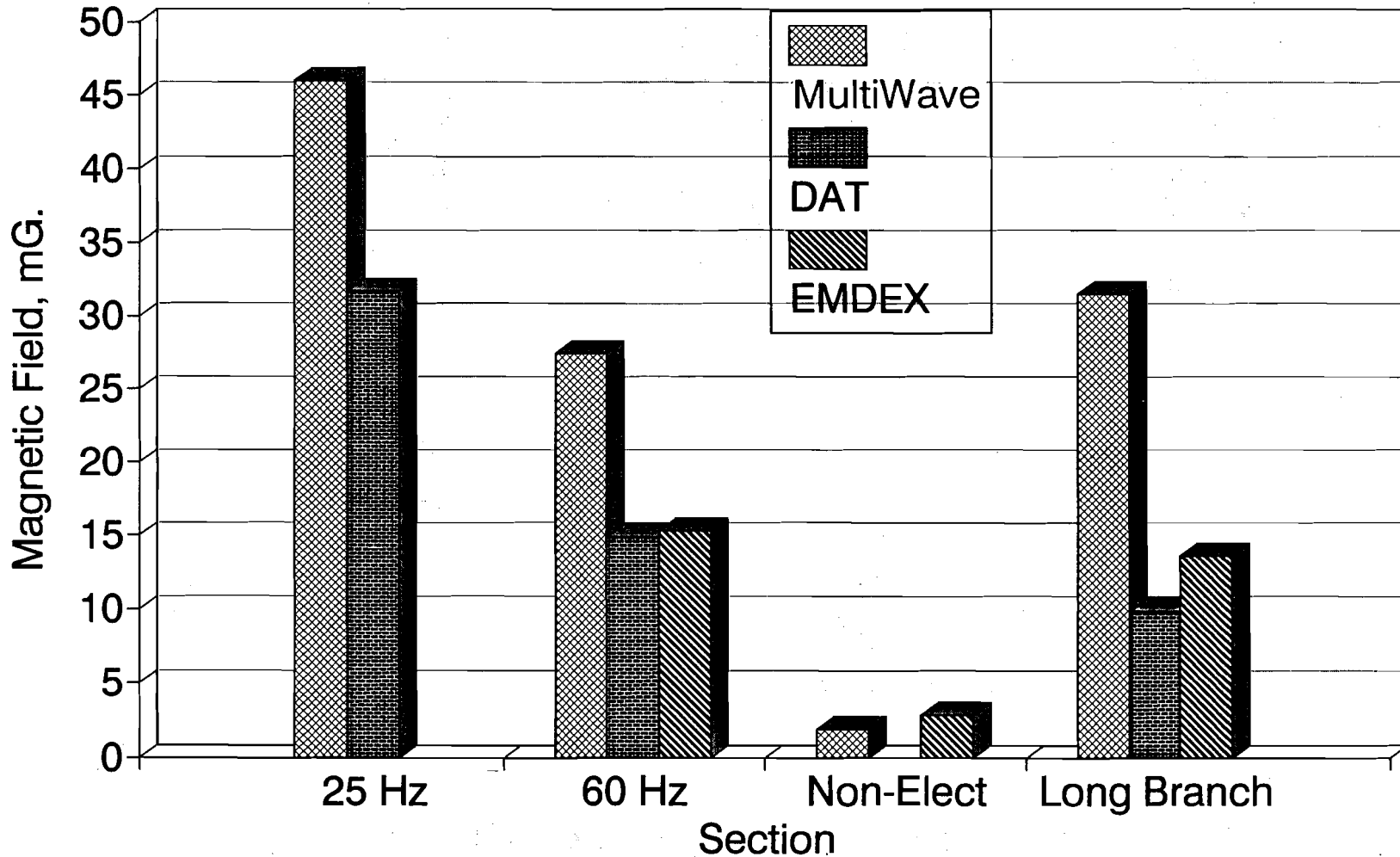
FIGURE 4-19. COMPARISON OF THE AVERAGE TIME-VARYING MAGNETIC FIELD LEVELS IN CABS OF LOCOMOTIVES OPERATING ON VARIOUS SECTIONS OF THE NEC AND ON THE NORTH JERSEY COAST LINE MEASURED IN DIFFERENT WAYS
