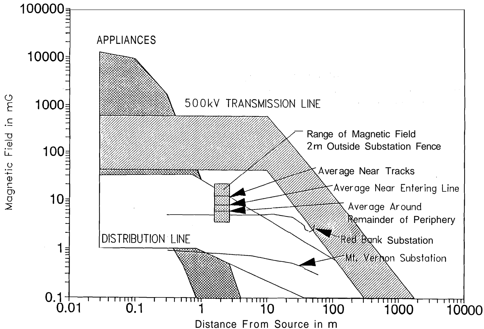
FIGURE 9-11. THE RANGE OF TOTAL TIME-VARYING MAGNETIC FIELD LEVELS 2 M (6.6 FT.) OUTSIDE THE FENCE OF THE RED BANK SUBSTATION AND LATERAL ATTENUATION PROFILES FOR THE RED BANK AND MT. VERNON SUBSTATIONS COMPARED TO TYPICAL POWER-FREQUENCY MAGNETIC FIELD LEVELS FROM COMMON SOURCES
