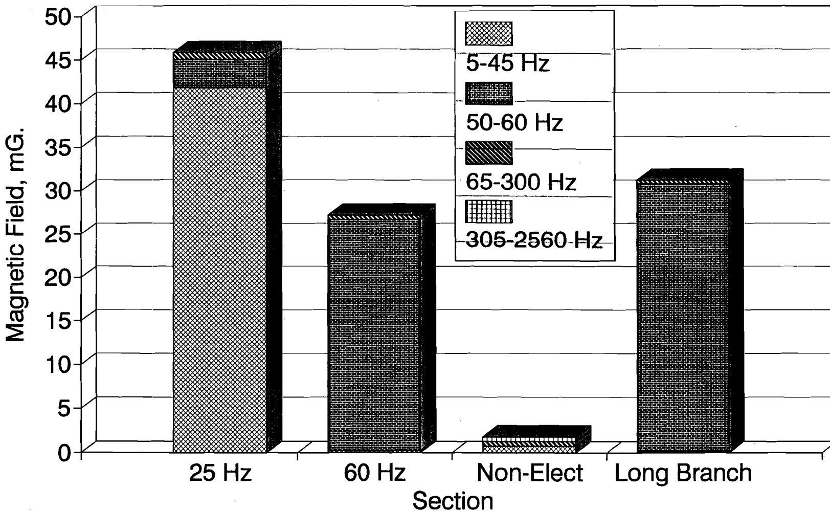
FIGURE 4-21. COMPARISON OF THE AVERAGE TIME-VARYING MAGNETIC FIELD LEVELS IN CABS OF LOCOMOTIVES OPERATING ON VARIOUS SECTIONS OF THE NEC OR THE NORTH JERSEY COAST LINE AND THE PRINCIPAL COMPONENT FREQUENCY RANGES
