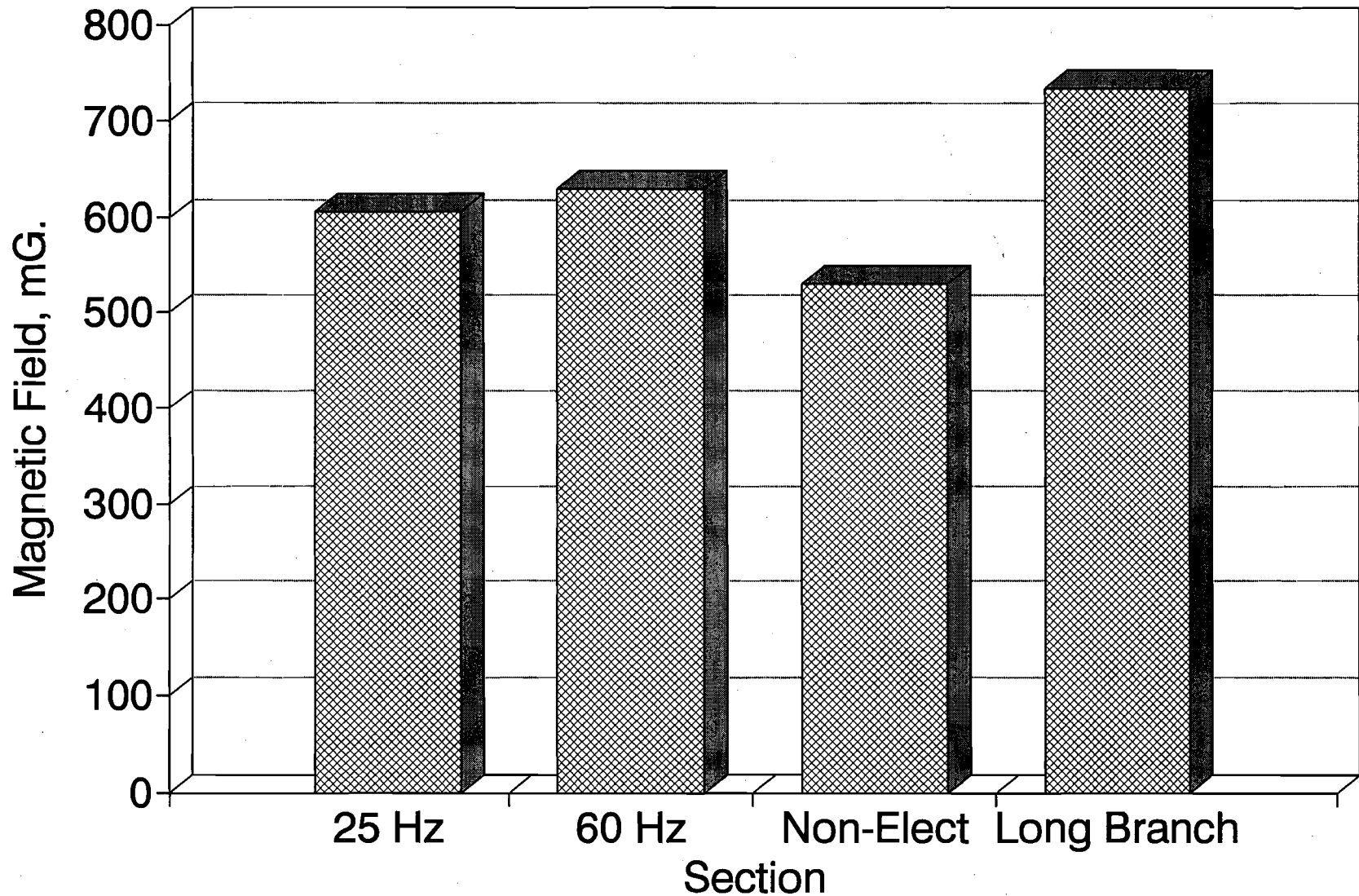
FIGURE 3-22. COMPARISON OF AVERAGE STATIC MAGNETIC FIELD LEVELS IN COACHES ON VARIOUS SECTIONS OF THE NEC AND ON THE NORTH JERSEY COAST LINE
