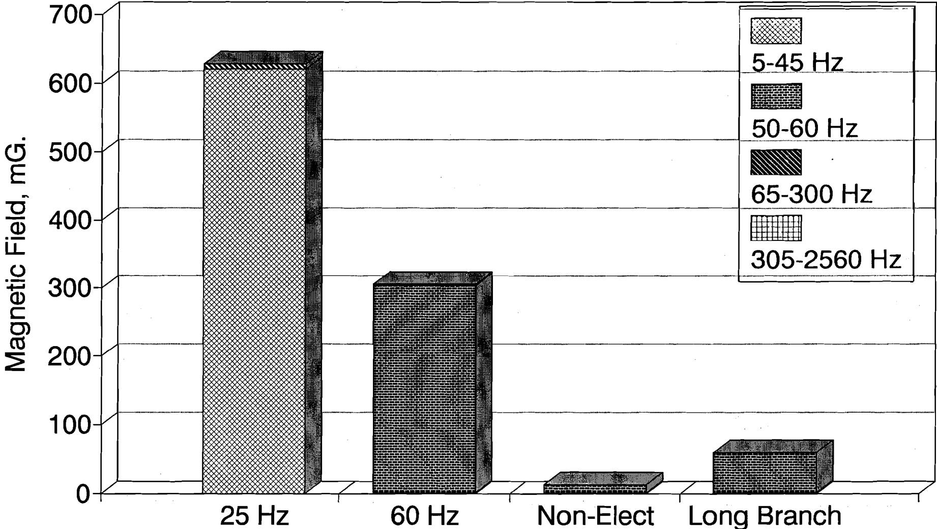
FIGURE 3-27. COMPARISON OF THE MAXIMUM TIME-VARYING MAGNETIC FIELD LEVELS IN COACHES ON VARIOUS SECTIONS OF THE NEC AND ON THE NORTH JERSEY COAST LINE AND THEIR PRINCIPAL COMPONENT FREQUENCY RANGES
