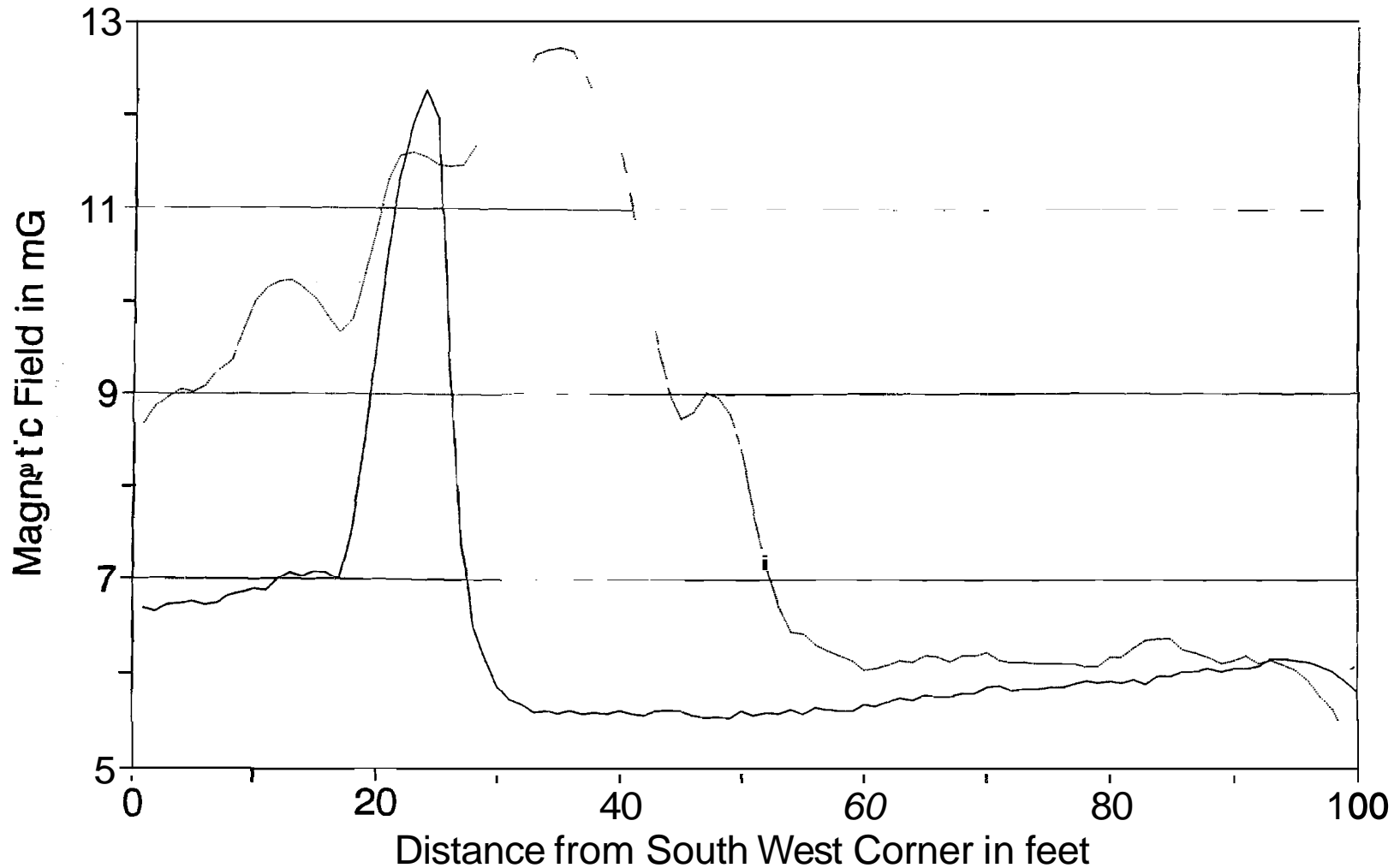
FIGURE 7-8. MAGNETIC FIELD AS A FUNCTION OF DISTANCE ALONG THE SUBSTATION FENCE ALONG PROFILE LINE 3 BENEATH THE ENTERING TRANSMISSION LINE AT THE RED BANK SUBSTATION
