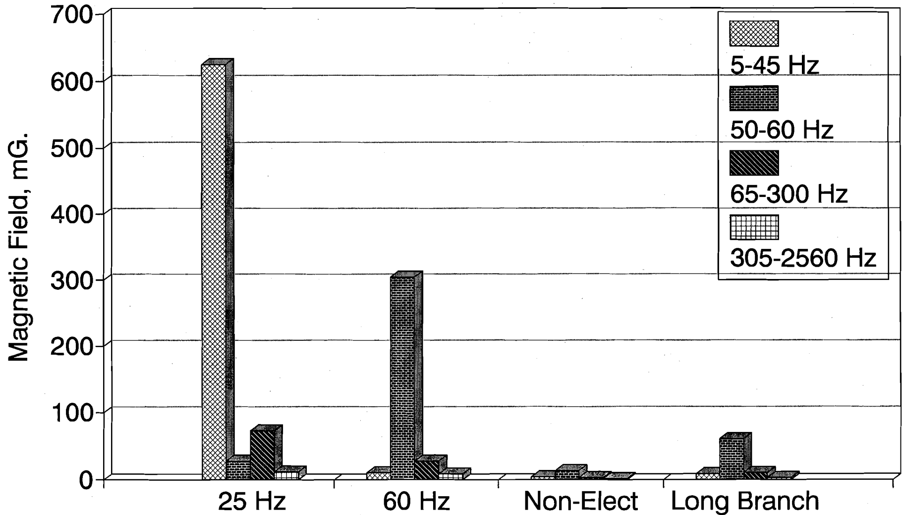
FIGURE 3-28. COMPARISON OF THE TIME-VARYING MAGNETIC FIELD LEVELS IN VARIOUS FREQUENCY BANDS DURING MAXIMUM FIELD CONDITIONS IN COACHES ON VARIOUS SECTIONS OF THE NEC AND ON THE NORTH JERSEY COAST LINE
