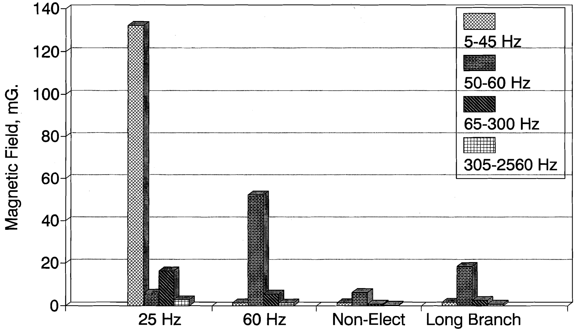
FIGURE 3-25. COMPARISON OF AVERAGE TIME-VARYING MAGNETIC FIELD LEVELS IN FOUR FREQUENCY BANDS IN THE COACHES ON VARIOUS SECTIONS OF THE NEC AND ON THE NORTH JERSEY COAST LINE
