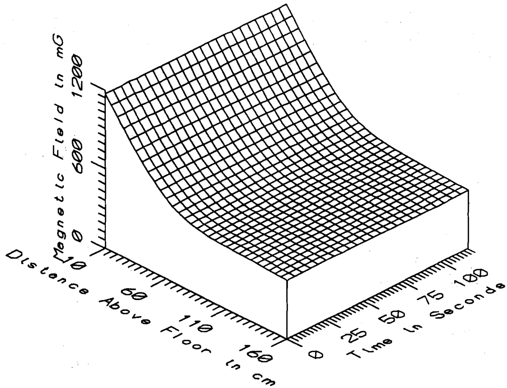
NEC020 - 2' IN FRONT OF UPS UNIT - STATIC
