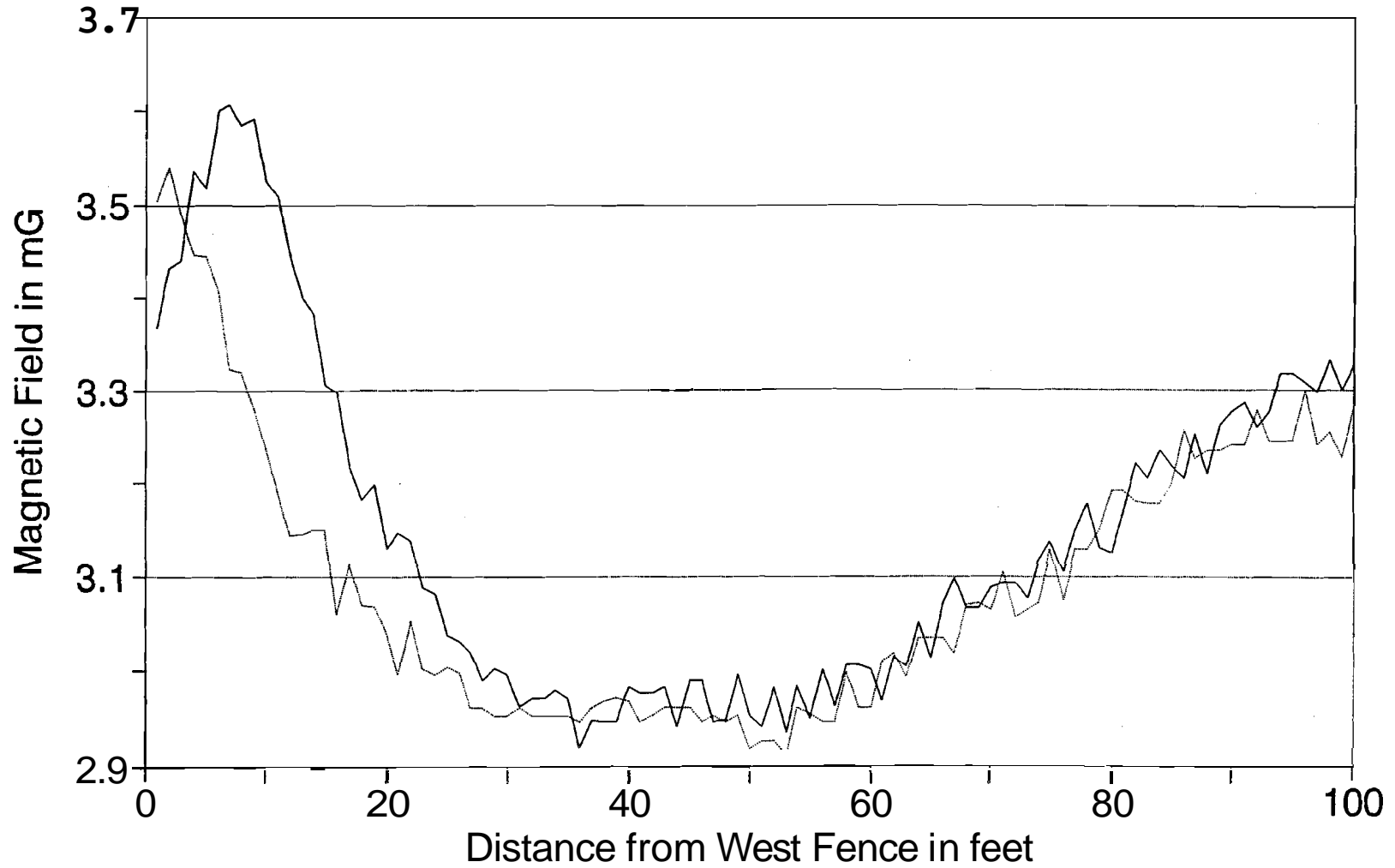
FIGURE 7-10. MAGNETIC FIELD AS A FUNCTION OF DISTANCE FROM THE SUBSTATION FENCE ALONG PROFILE LINE 7 AT THE RED BANK SUBSTATION
