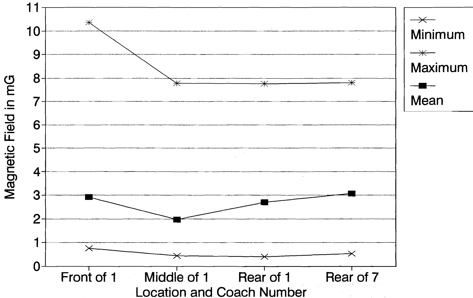
FIGURE 3-10. MAGNETIC FIELD LEVELS IN THE HIGH FREQUENCY BAND (305-2560 HZ)
