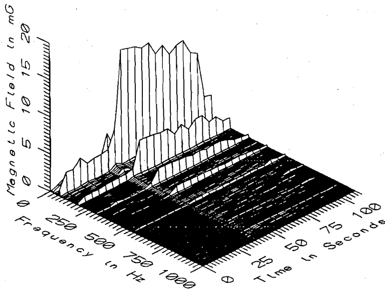
NEC053 - 10 cm ABOVE GROUND, 20FT FROM CENTERLINE OF TRACK
