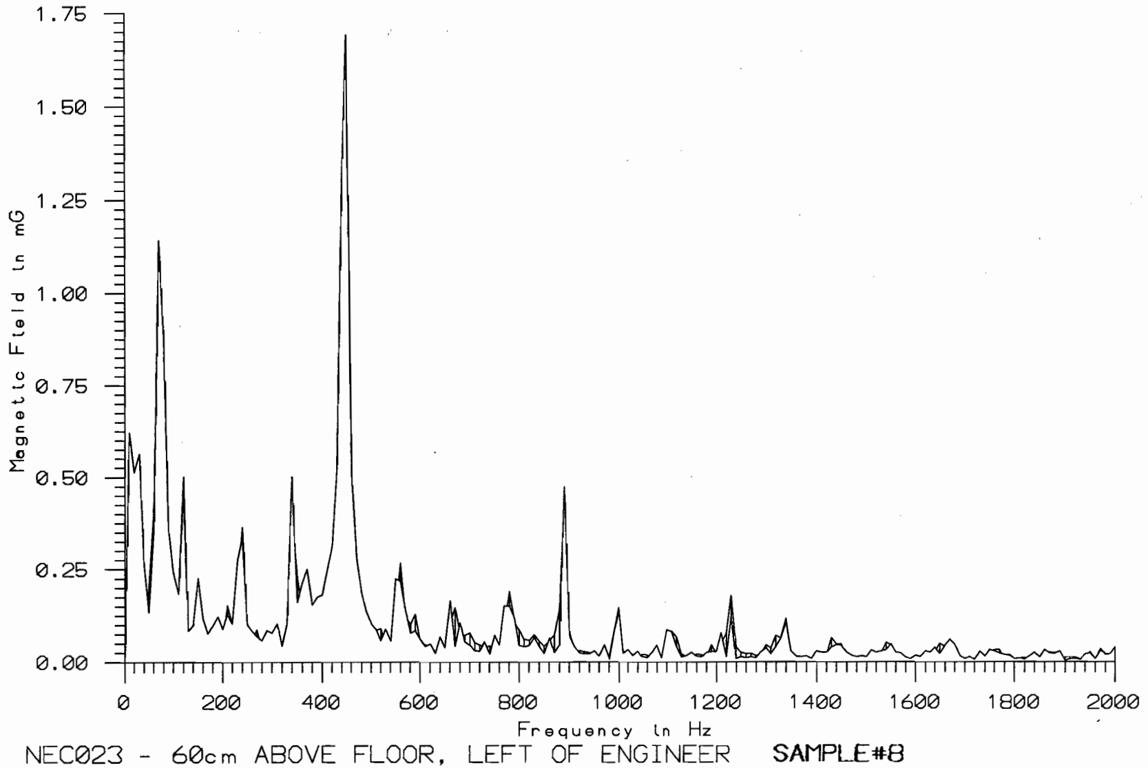
FIGURE 4-11. MAGNETIC FIELD FREQUENCY SPECTRUM NEAR THE ENGINEER'S SEAT IN A DIESEL-ELECTRIC LOCOMOTIVE OPERATING ON THE NON-ELECTRIFIED PORTION OF THE NORTHEAST CORRIDOR
