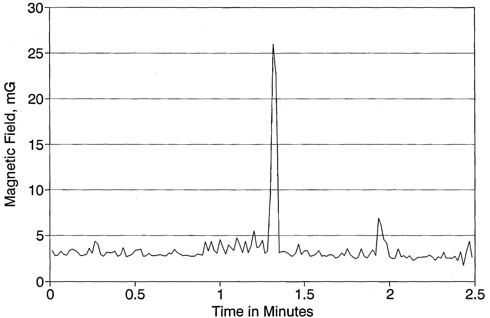
FIGURE 3-21. TOTAL RMS TIME-VARYING ELF MAGNETIC FIELD MEASURED IN A COACH SEAT ON THE NON-ELECTRIFIED PORTION OF THE NEC AS THE TRAIN PASSES AN APPARENT EXTERNAL MAGNETIC FIELD SOURCE BELIEVED TO BE AN ELECTRIC POWER TRANSMISSION LINE CROSSING THE TRACKS
