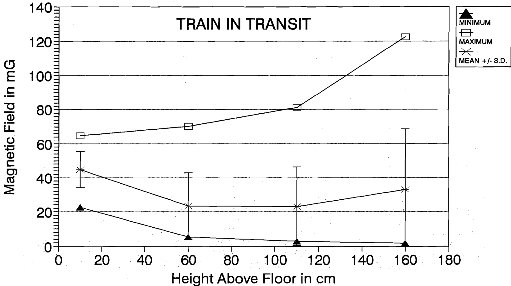
FIGURE 4-15. VERTICAL PROFILE OF THE POWER FREQUENCY MAGNETIC FIELD STRENGTH IN THE REAR CAB OF A LOCOMOTIVE OPERATING ON THE 60 HZ SECTION OF THE NORTH JERSEY COAST LINE
