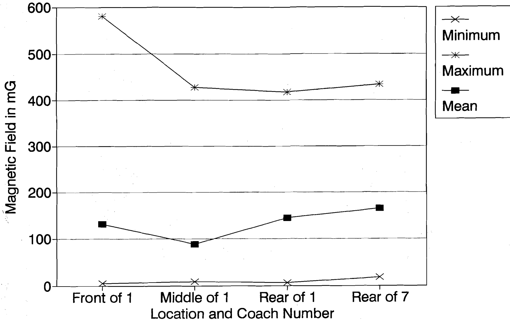
FIGURE 3-5. LOW FREQUENCY MAGNETIC FIELD LEVELS AT VARIOUS LOCATIONS ALONG THE 25 HZ NEC SEGMENT
