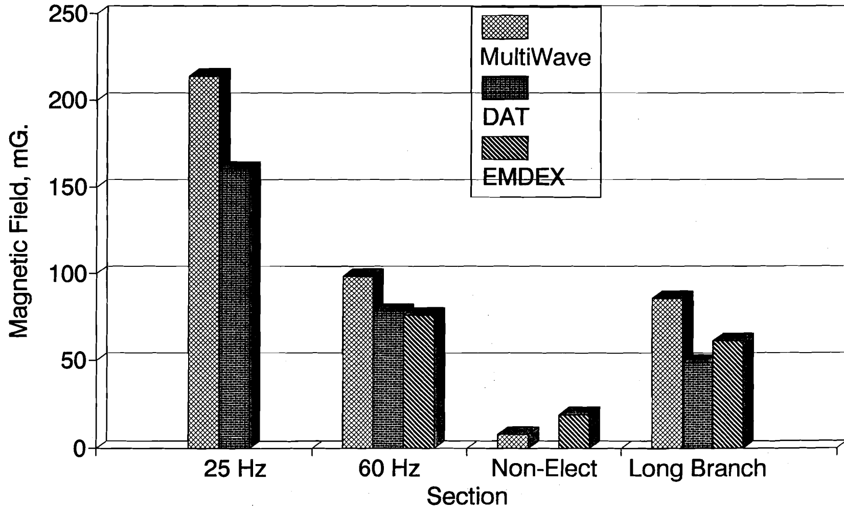
FIGURE 4-20. COMPARISON OF THE MAXIMUM TIME-VARYING MAGNETIC FIELD LEVELS AT TYPICAL LOCATIONS IN CABS OF LOCOMOTIVES OPERATING ON VARIOUS SECTIONS OF THE NEC AND THE NORTH JERSEY COAST LINE MEASURED IN DIFFERENT WAYS
