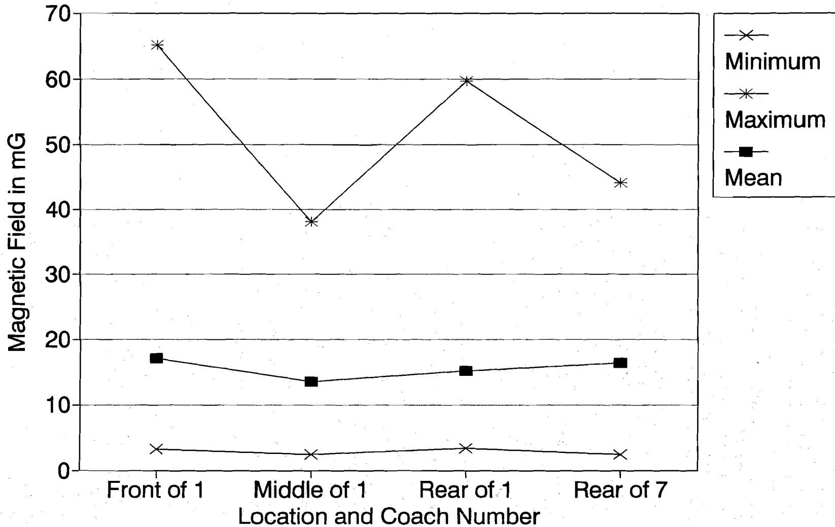
FIGURE 3-9. MAGNETIC FIELD LEVELS IN THE POWER HARMONICS BAND (65-300 HZ)
