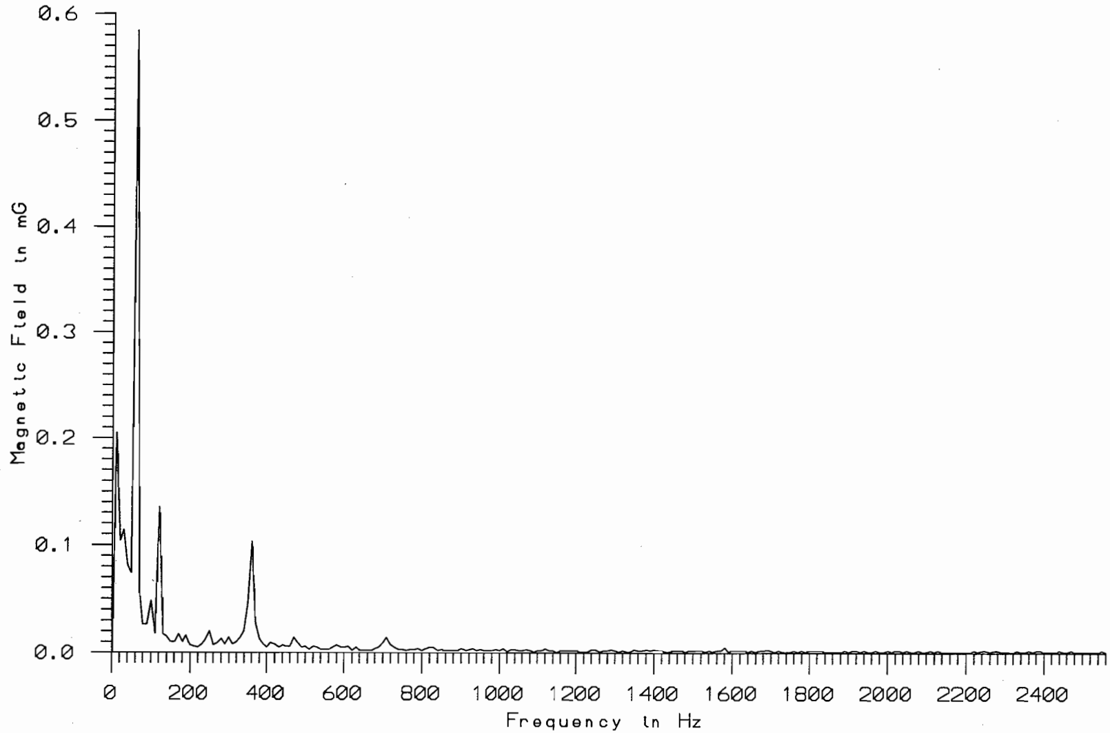
FIGURE 4-12. MAGNETIC FIELD FREQUENCY SPECTRUM NEAR THE ENGINEER'S SEAT IN A DIESEL-ELECTRIC LOCOMOTIVE STOPPED AT A STATION
