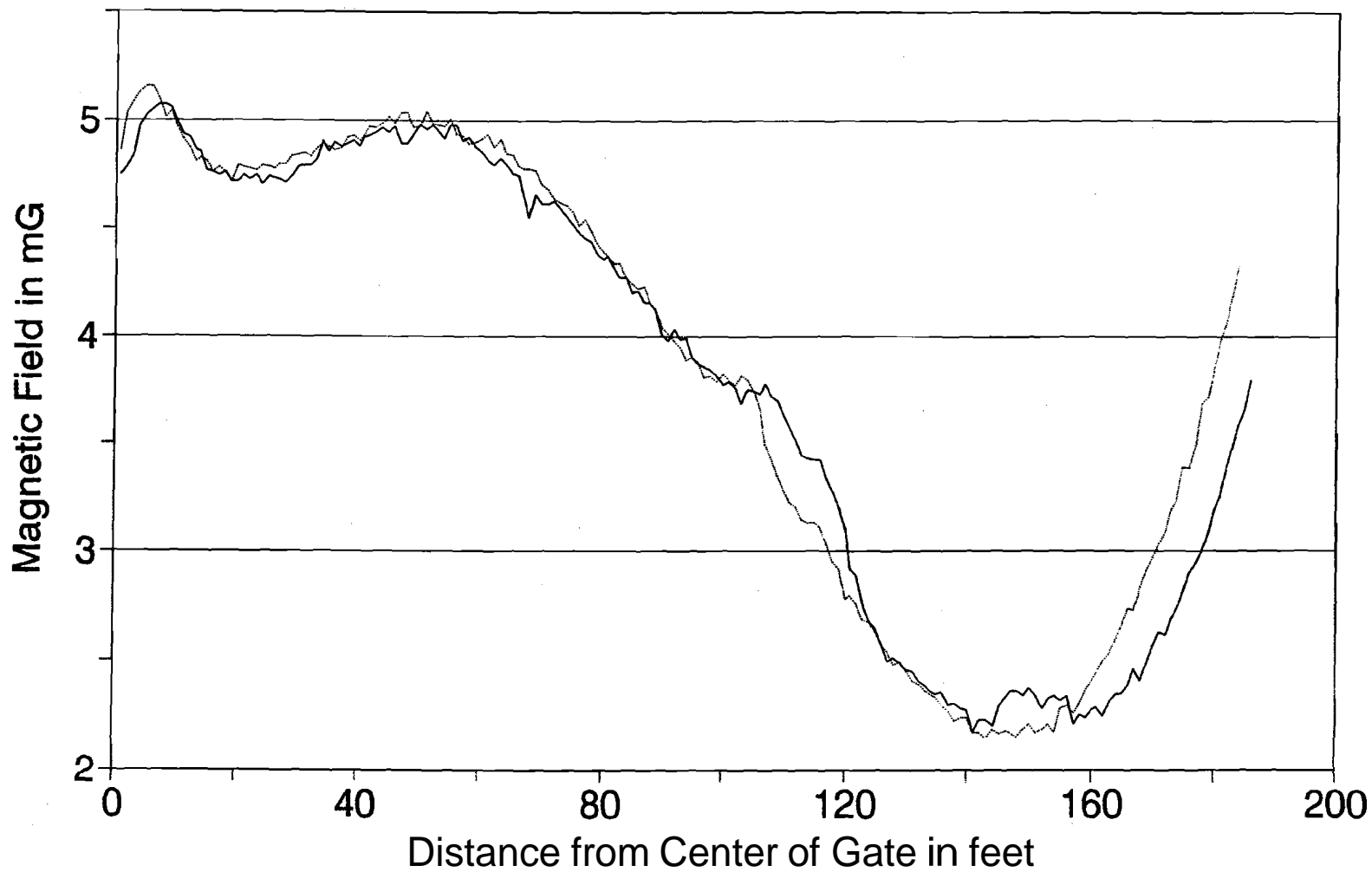
FIGURE 7-9. MAGNETIC FIELD AS A FUNCTION OF DISTANCE AWAY FROM THE SUBSTATION FENCE ALONG PROFILE LINE 6 AT THE RED BANK SUBSTATION
