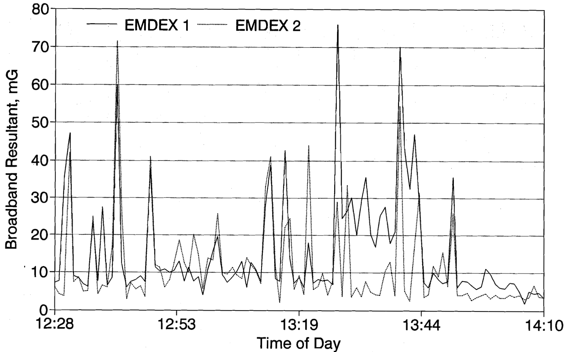
FIGURE 4-13. RMS RECORDINGS OF MAGNETIC FIELD LEVELS ENCOUNTERED BY A PERSON STANDING (RMS RECORDER 1) OR SEATED IN THE ENGINEER'S SEAT (RMS RECORDER 2) OF THE REAR CAB OF A LOCOMOTIVE ON THE 60 HZ SECTION OF THE NEC
