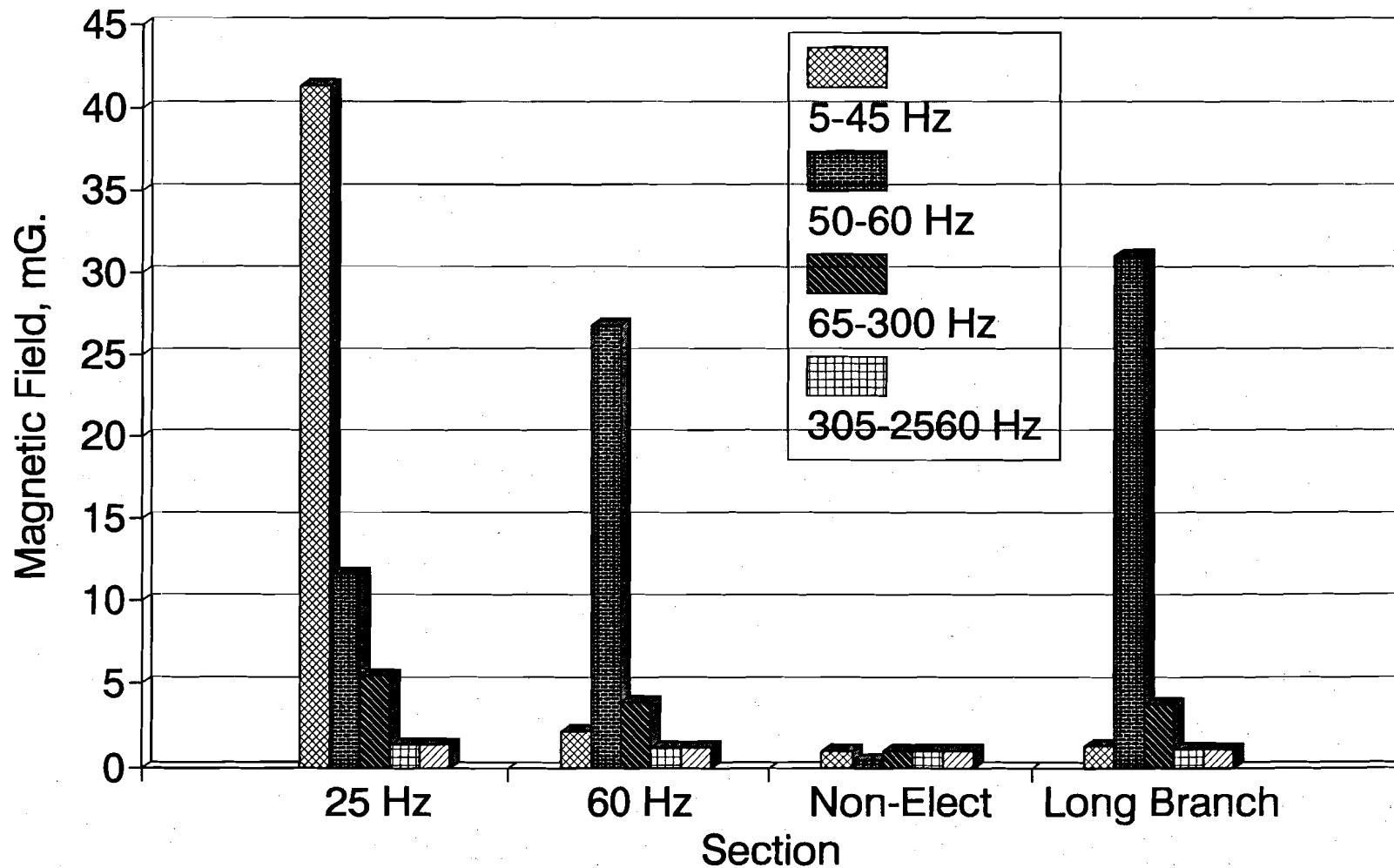
FIGURE 4-23. COMPARISON OF AVERAGE TIME-VARYING MAGNETIC FIELD LEVELS IN THE FOUR FREQUENCY BANDS IN THE CABS OF LOCOMOTIVES OPERATING ON VARIOUS SECTIONS OF THE NEC OR THE NORTH JERSEY COAST LINE
