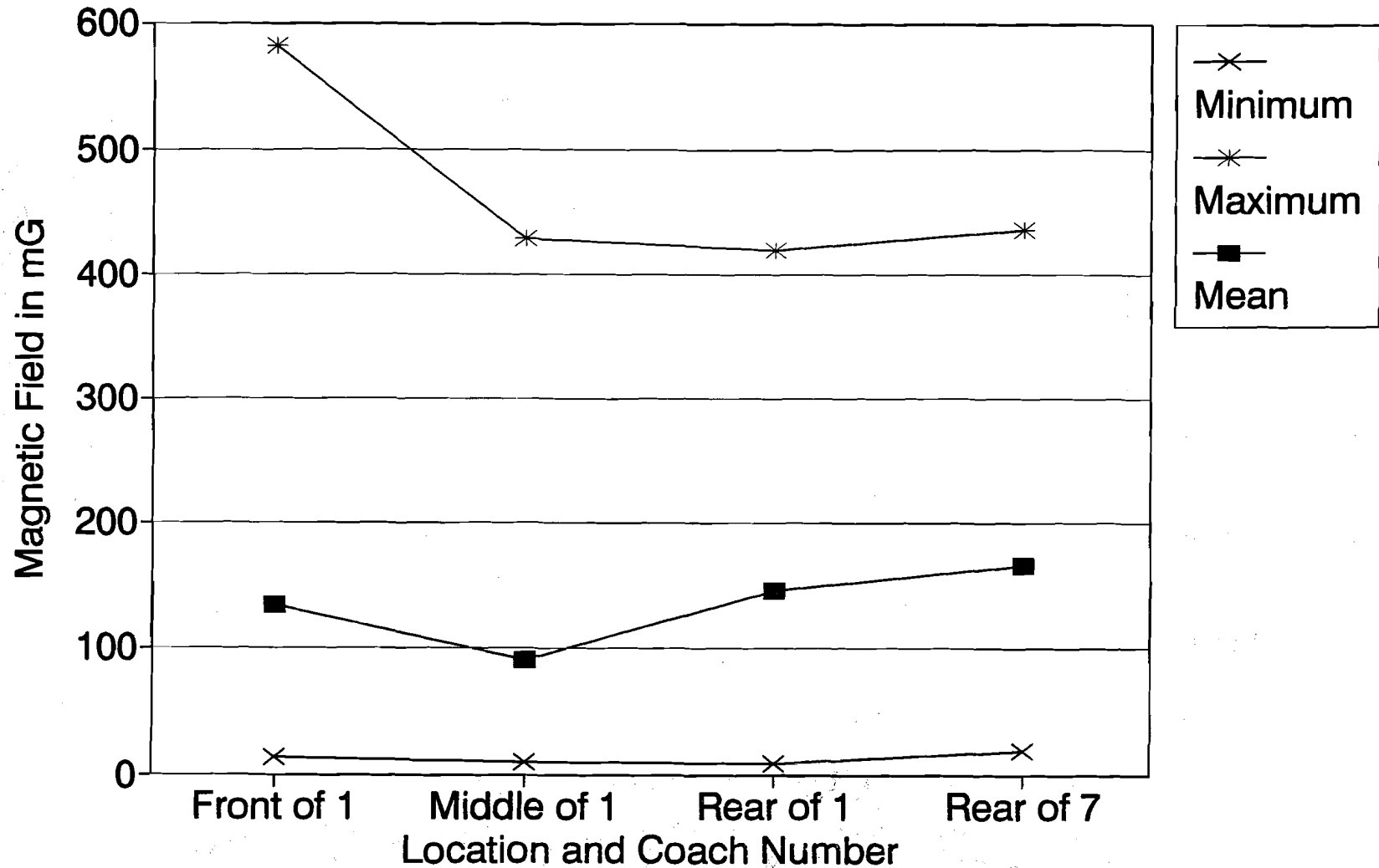
FIGURE 3-11. TOTAL TIME-VARYING MAGNETIC FIELD (5-2560 HZ) AT VARIOUS LOCATIONS
