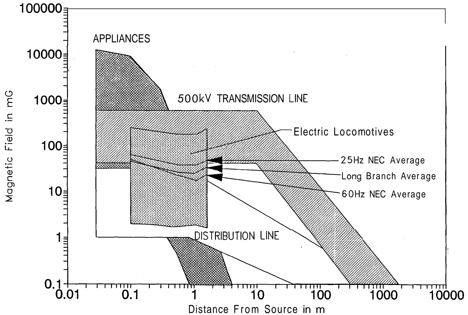
FIGURE 9-5. THE RANGE OF TOTAL TIME-VARYING MAGNETIC FIELD LEVELS IN THE CABS OF ELECTRIC LOCOMOTIVES COMPARED TO TYPICAL LEVELS OF POWER-FREQUENCY MAGNETIC FIELDS PRODUCED BY COMMON SOURCES
