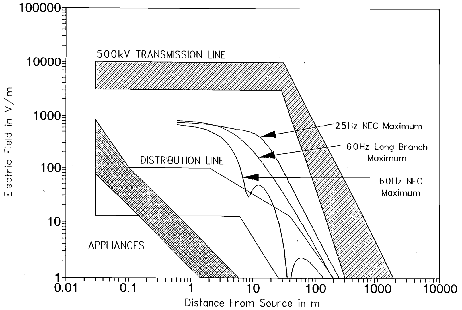
FIGURE 1-6. MAXIMUM TIME-VARYING ELECTRIC FIELD AT THE WAYSIDE OF ELECTRIFIED RAILROADS AS A FUNCTION OF DISTANCE FROM THE NEAREST TRACK COMPARED TO TYPICAL LEVELS OF POWER-FREQUENCY ELECTRIC FIELDS PRODUCED BY COMMON SOURCES
