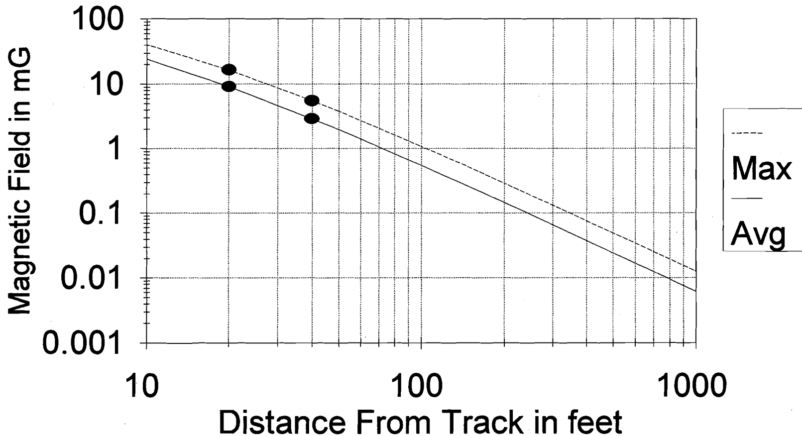
FIGURE 5-12. THEORETICAL ATTENUATION CURVES FITTED THROUGH THE AVERAGE AND MAXIMUM MAGNETIC FIELD VALUES MEASURED AT THE NORTH SIDE OF THE NORTH JERSEY COAST LINE NEAR RED BANK, NJ
