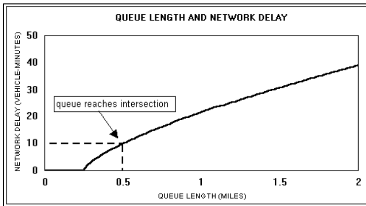
Figure 7 Network Delay as a Function of Queue Length (when intersection is 0.5 miles from crossing)
