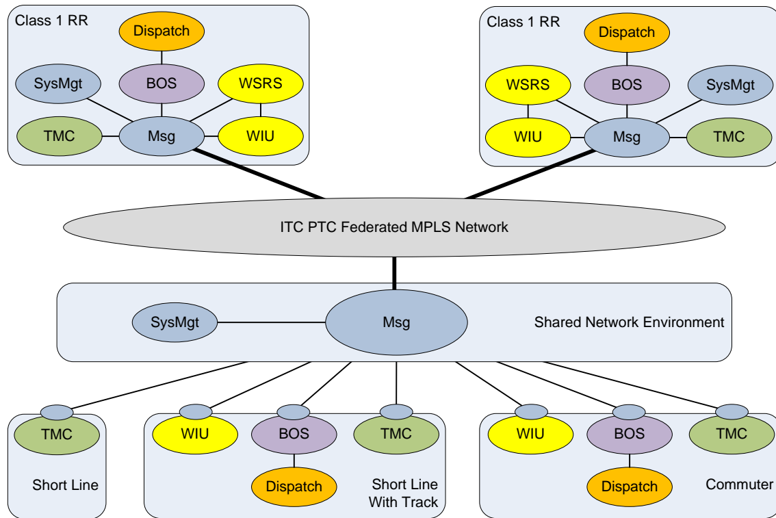
Figure 1 ITC PTC Shared Network Concept
