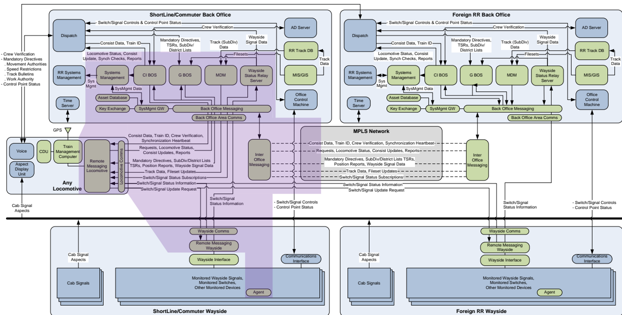
Figure 6 IPSN Major Components and External Interfaces for Host/Tenant Railroad
