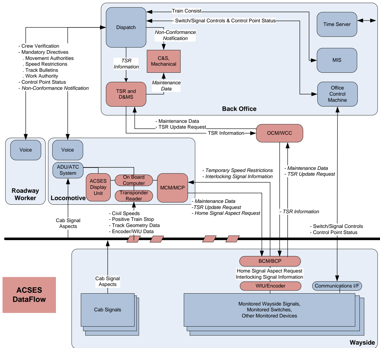
Figure 3 ACSES PTC Message Flows
