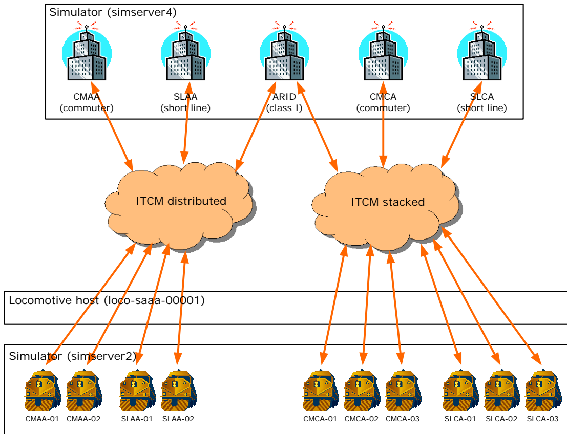
Figure 10 Core Test Configuration
