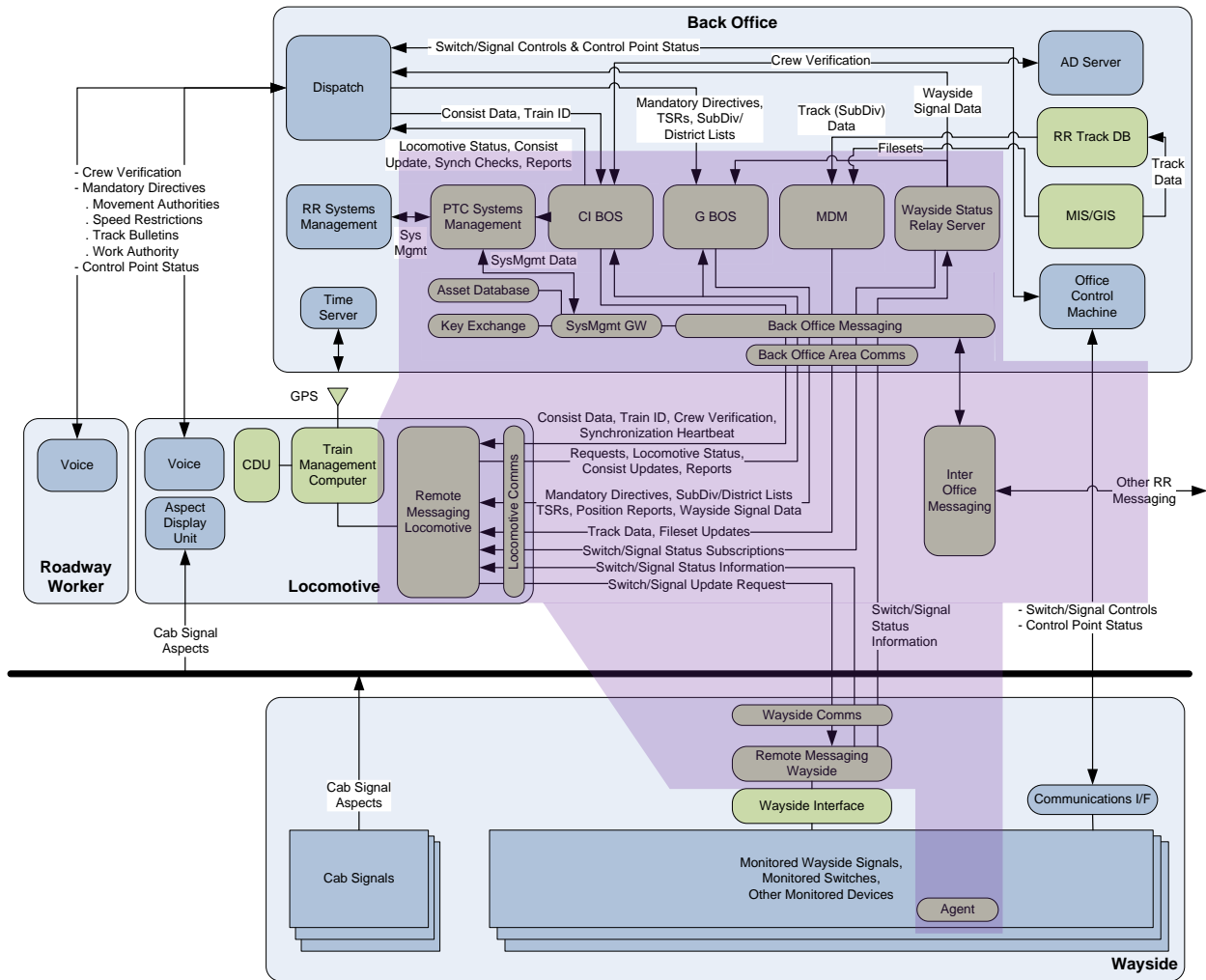
Figure 4 System Boundary of ITC PTC Shared Network Implementations
