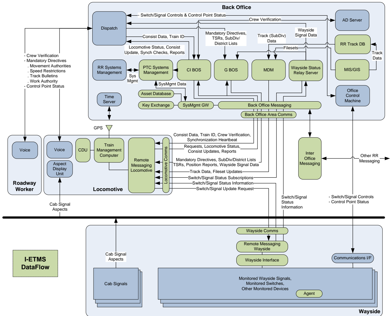
Figure 2 I-ETMS PTC Message Flows
