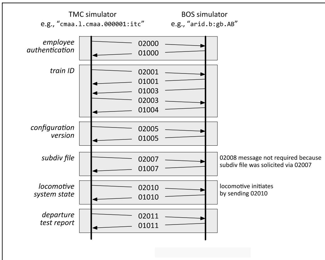
Figure 8 Illustration of Core Test Initialization Scenario
