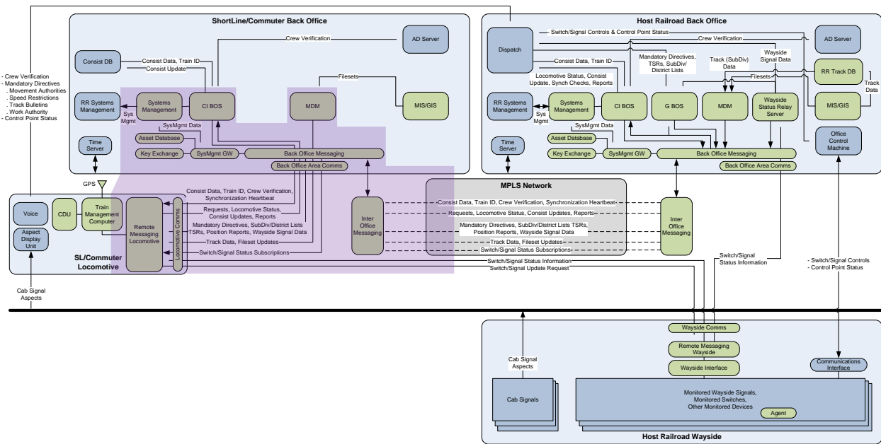
Figure 5 IPSN Major Components and External Interfaces for Tenant only Railroad
