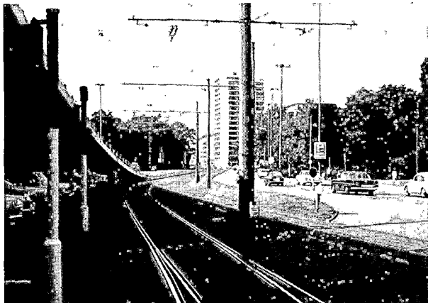
P-37. Special switch with long points to allow switching prior to street crossing (Düsseldorf)
