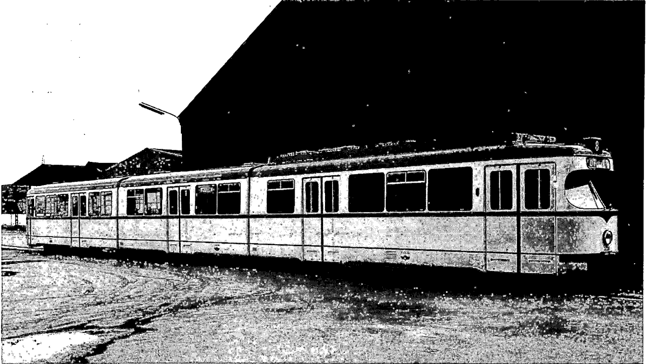
P-7. Eight-axle double-articulated 2.5 m. (8'2") wide car
