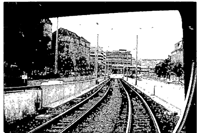
P-29. Median ROW protected by concrete barriers (Stuttgart)
