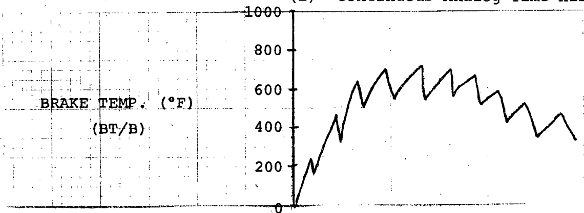
(2) Sequential recording on "Series" type recorder (many channels) page BT/B-2
