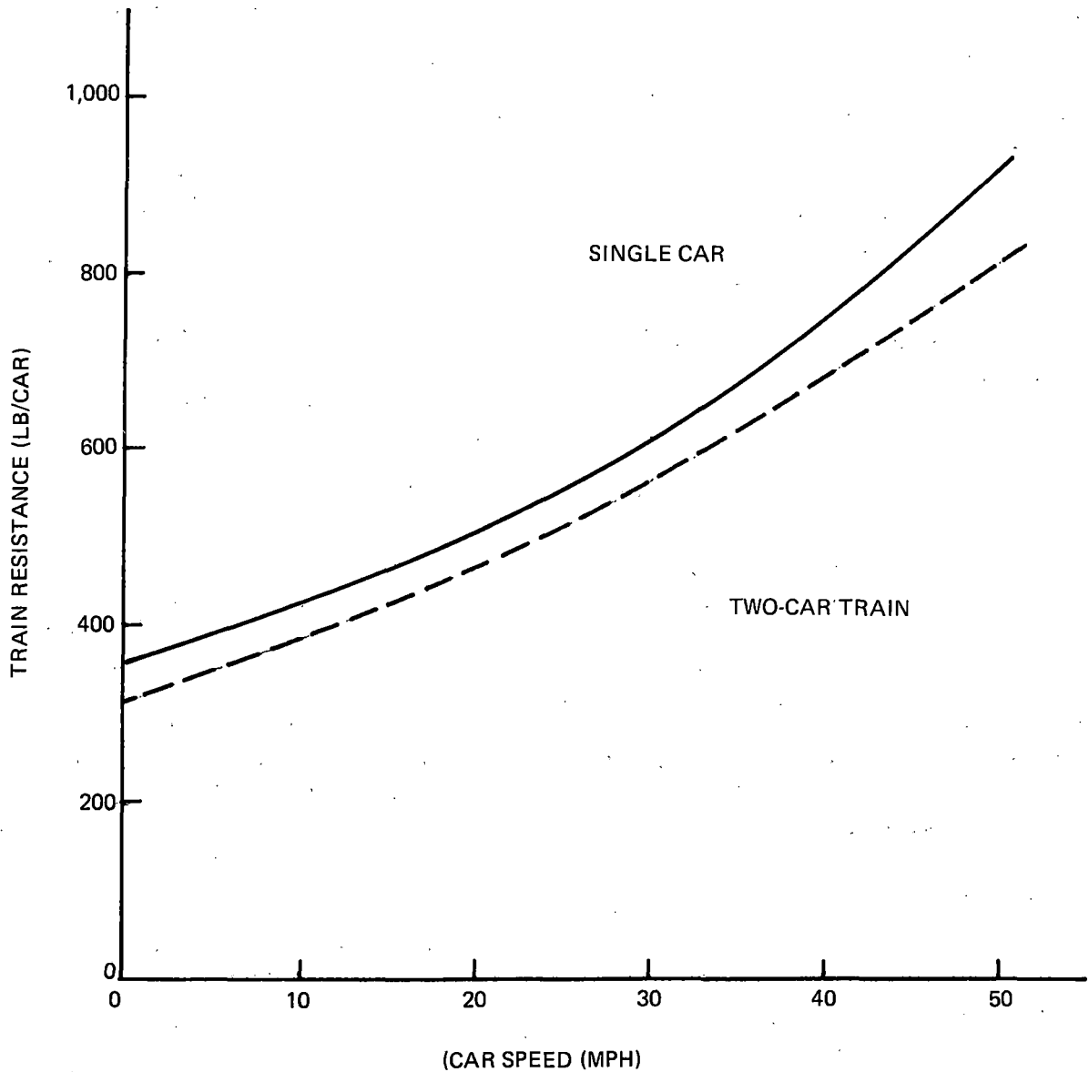
Figure 3-5. Traction Resistance
