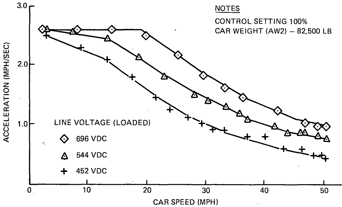
Figure 3-1. Effect of Line Voltage on Acceleration
