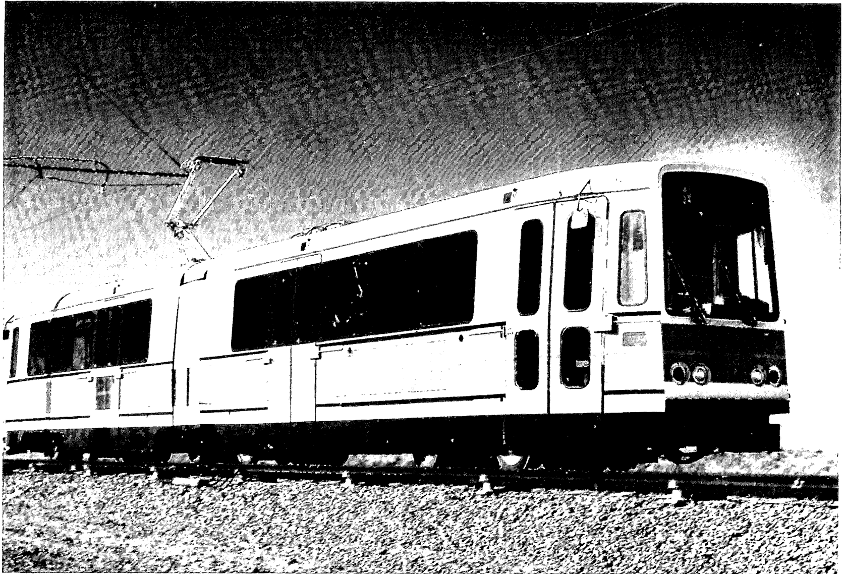
Figure 1-10. SLRV on Test Track Showing Catenary, Support, and Jumper Wiring
