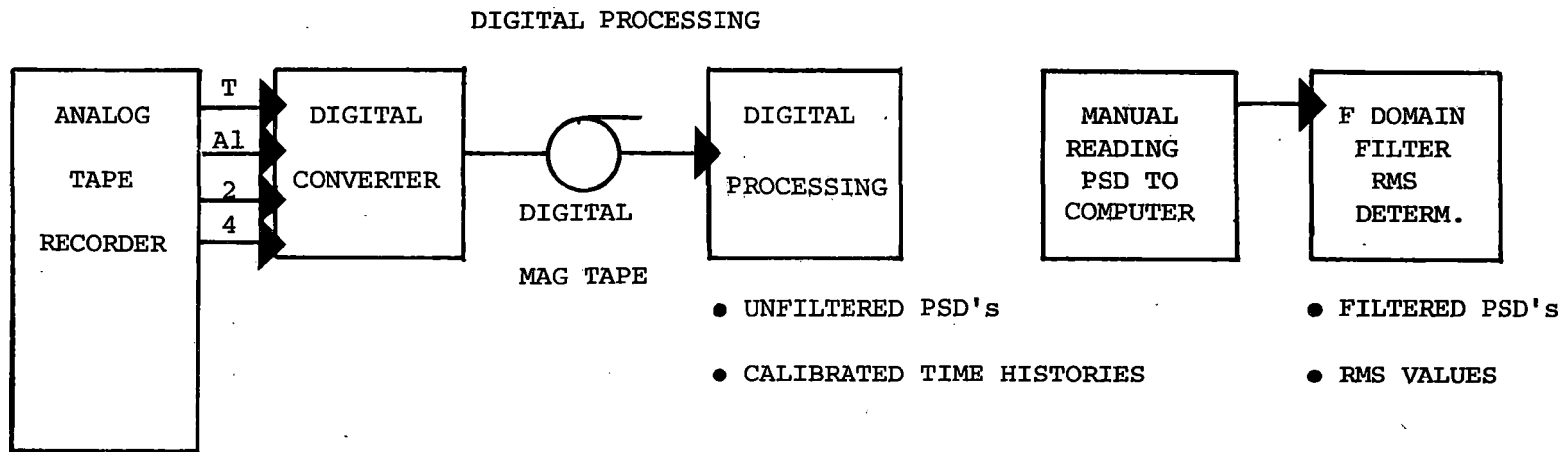
FIGURE 2-27. RIDE QUALITY DATA PROCESSING SCHEMATIC.
