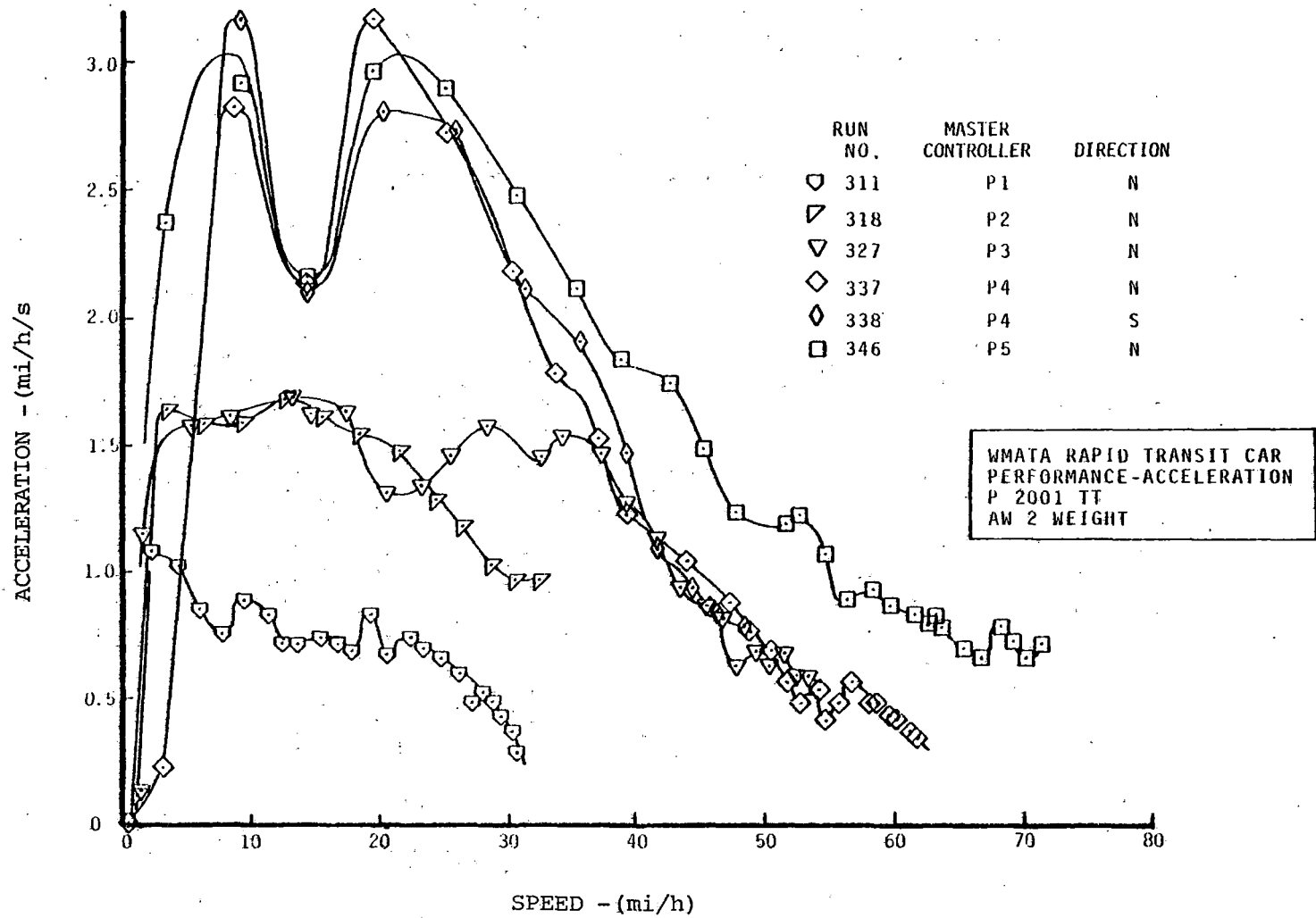
FIGURE 2-2. PERFORMANCE ACCELERATION - SPEED vs. ACCELERATION, EFFECT OF MASTER CONTROLLER POSITION.
