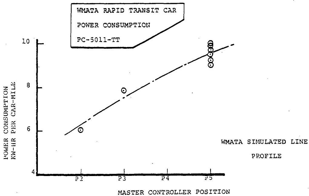
FIGURE 2-22. POWER CONSUMPTION - TREND WITH MASTER CONTROLLER DEMAND.
