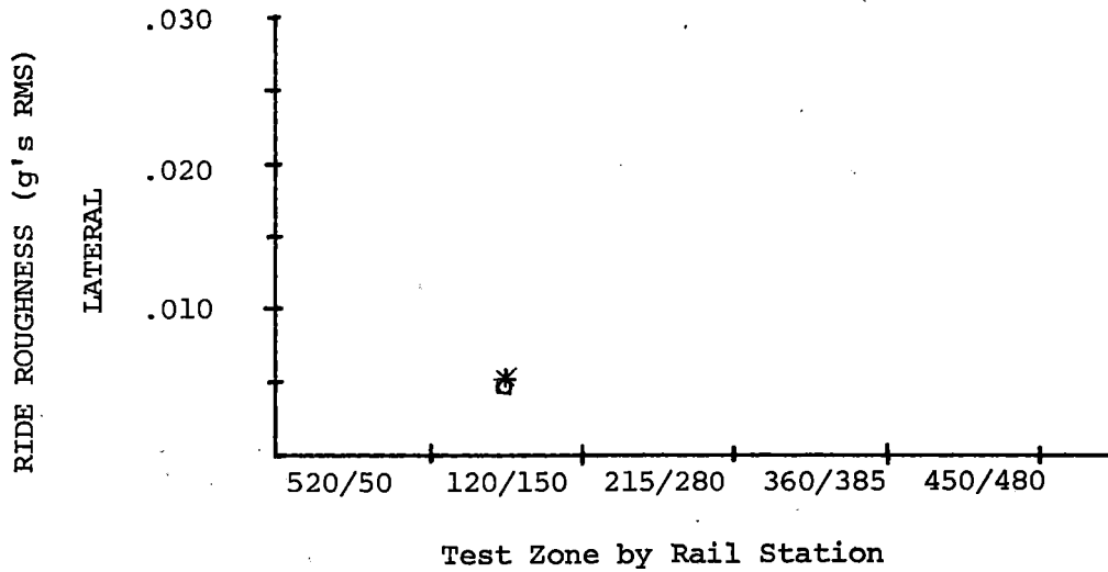
FIGURE 2-31. RIDE ROUGHNESS vs. TEST ZONES, B.
