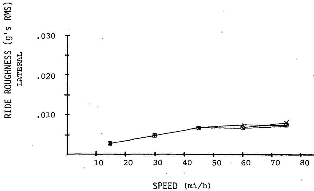
FIGURE 2-34. RIDE ROUGHNESS vs. SPEED, C.
