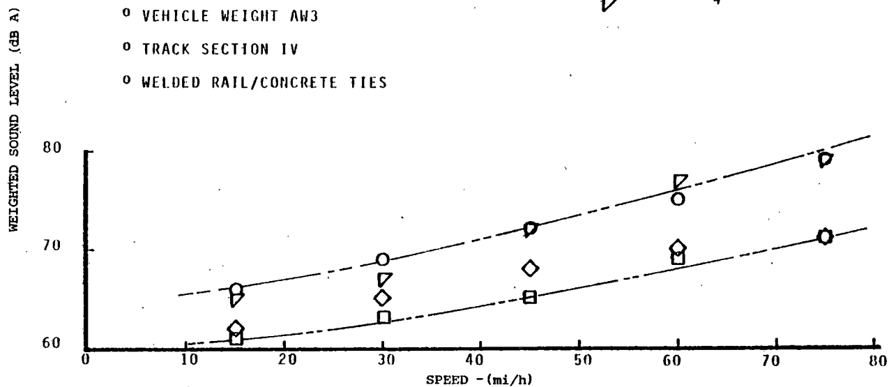
FIGURE 2-26. INTERIOR NOISE LEVELS - EFFECT OF SPEED, AW3 WEIGHT.
