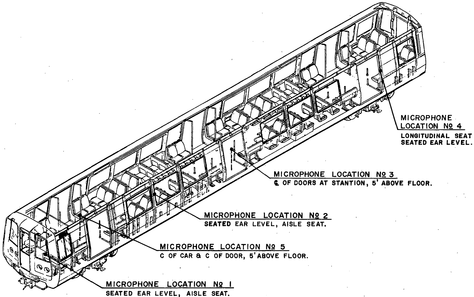
FIGURE 2-24. MICROPHONE LOCATIONS CAR NO. 1104.
