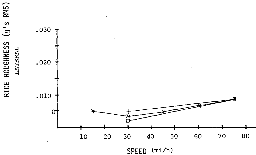
FIGURE 2-35. RIDE ROUGHNESS vs. SPEED, D.
