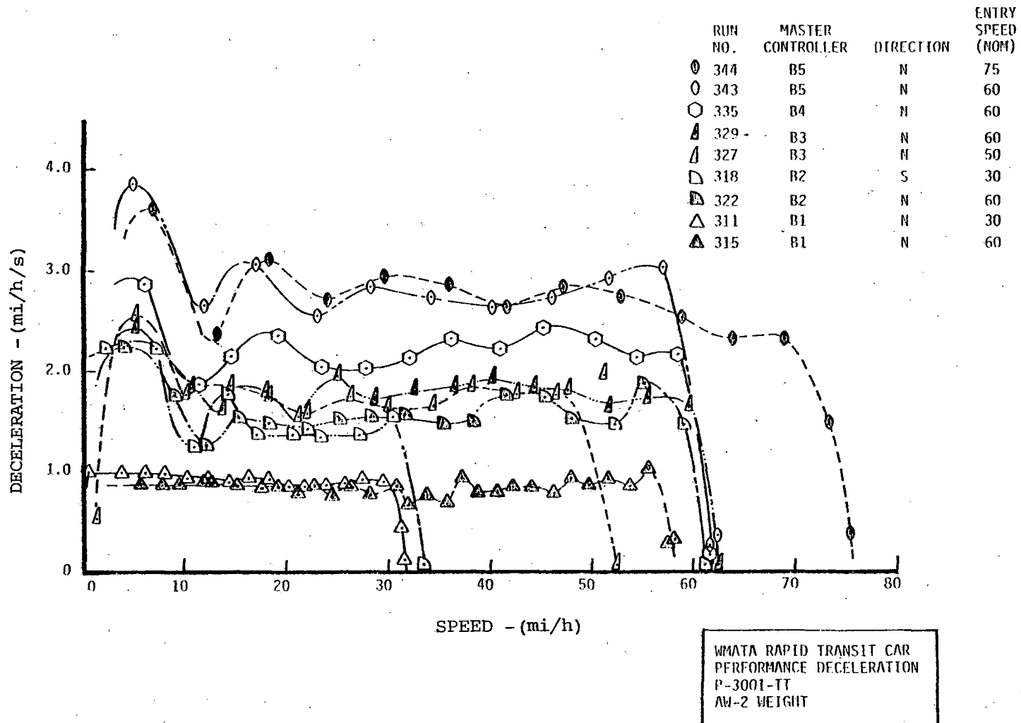
FIGURE 2-8. PERFORMANCE DECELERATION - BLENDED BRAKING, DECELERATION vs. SPEED.
