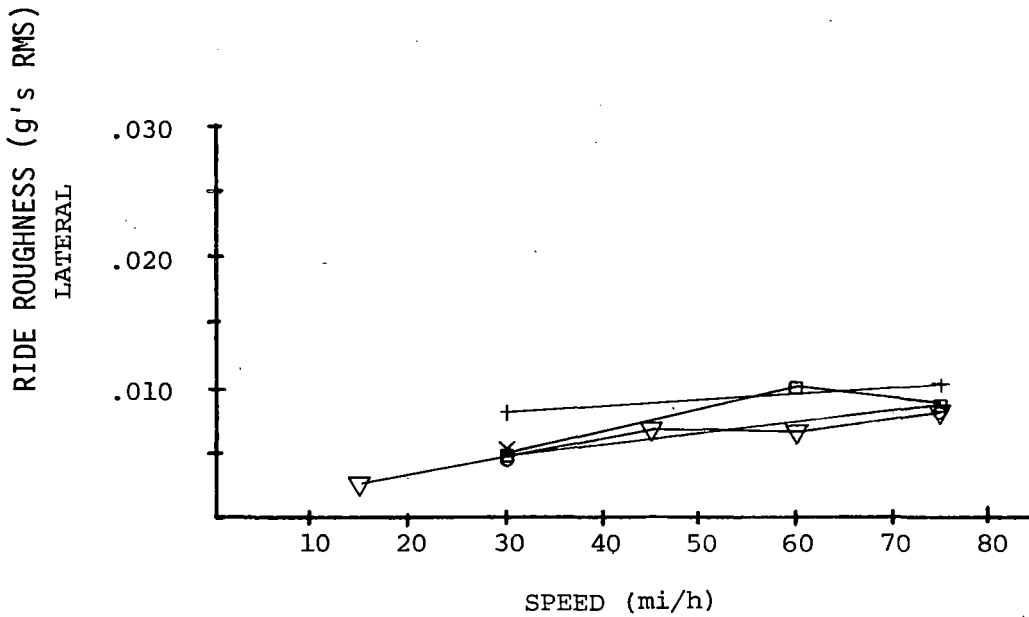
FIGURE 2-32. RIDE ROUGHNESS vs. SPEED, A.
