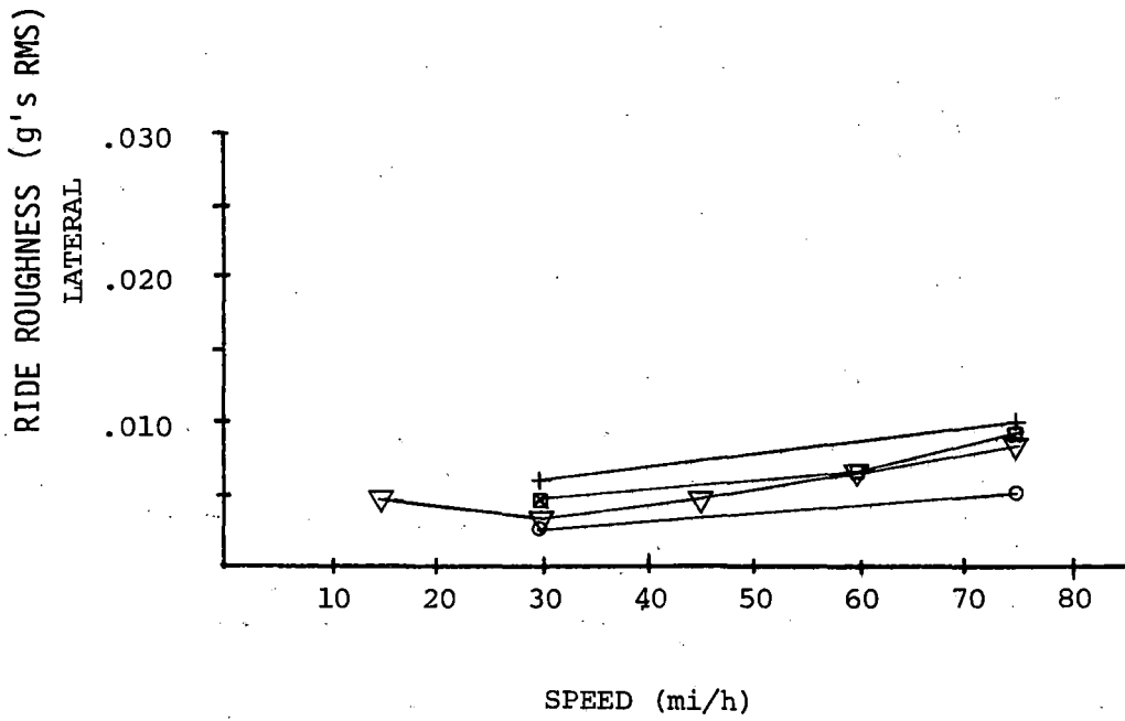
FIGURE 2-33 RIDE ROUGHNESS vs. SPEED, B.
