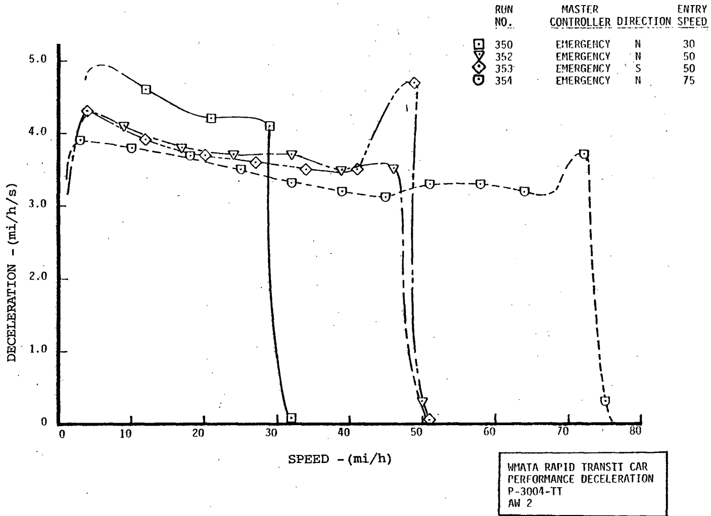
FIGURE 2-9. PERFORMANCE DECELERATION - EMERGENCY BRAKING, DECELERATION vs. SPEED.
