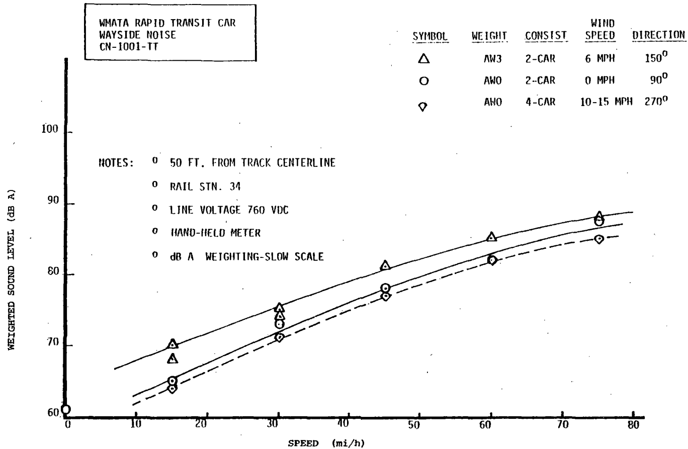
FIGURE 2-23. WAYSIDE NOISE LEVELS.
