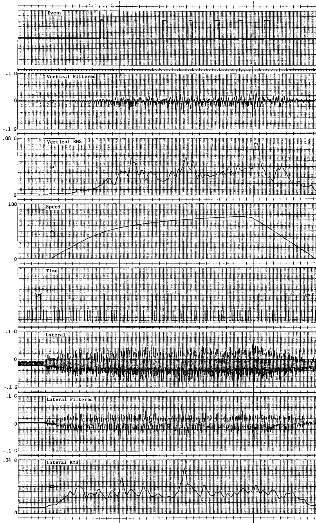
FIGURE 2-42. ACCELERATION/DECELERATION RMS HISTORY, RUN 440.
