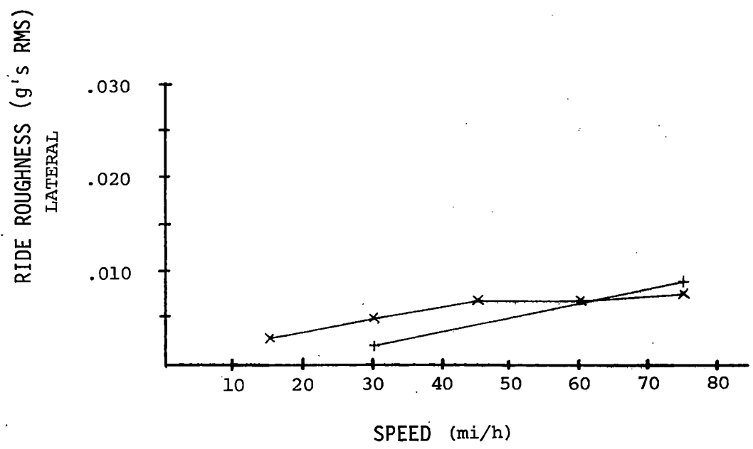
FIGURE 2-38. RIDE ROUGHNESS vs. SPEED, G.
