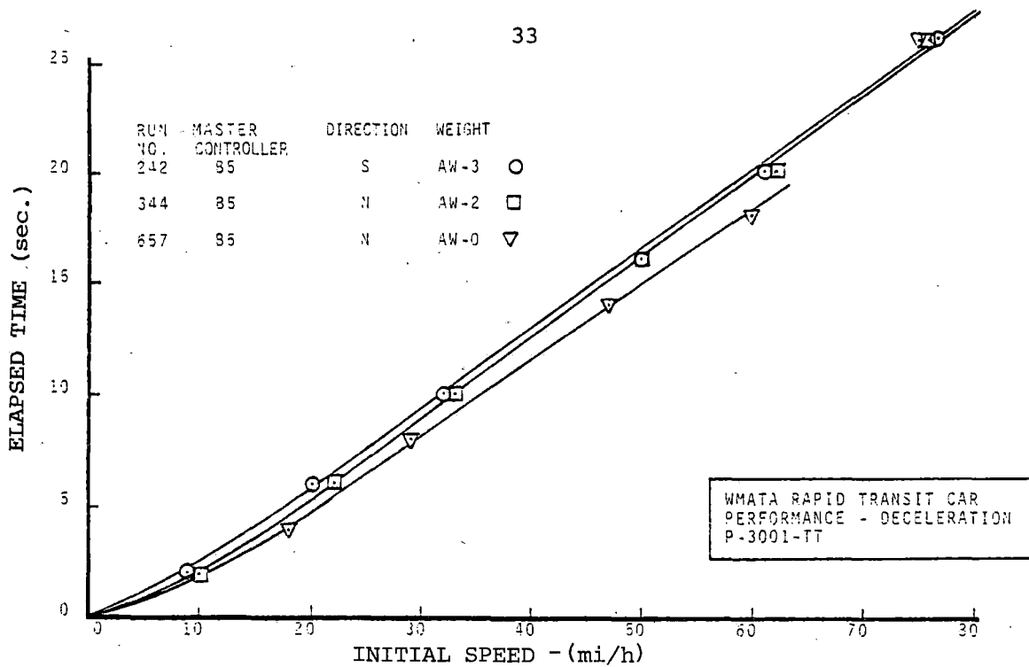
FIGURE 2-16. PERFORMANCE DECELERATION -LOAD-WEIGH COMPARISON, SPEED vs. TIME.
