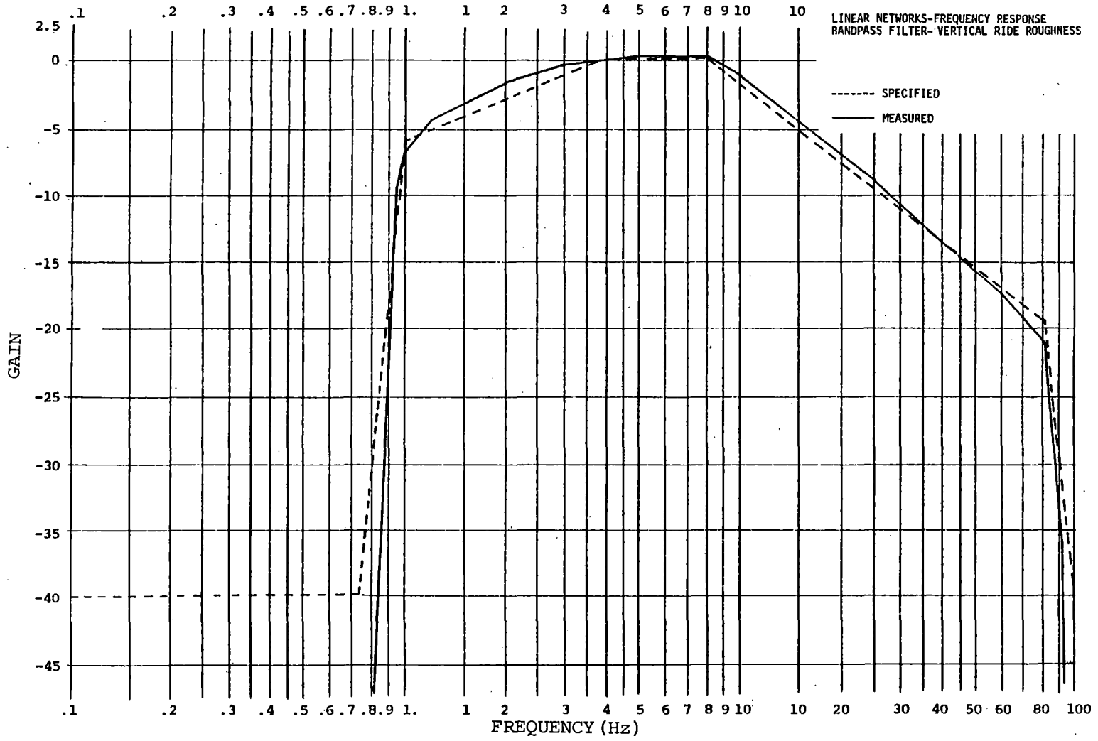
FIGURE 5-1. VERTICAL RIDE ROUGHNESS.
