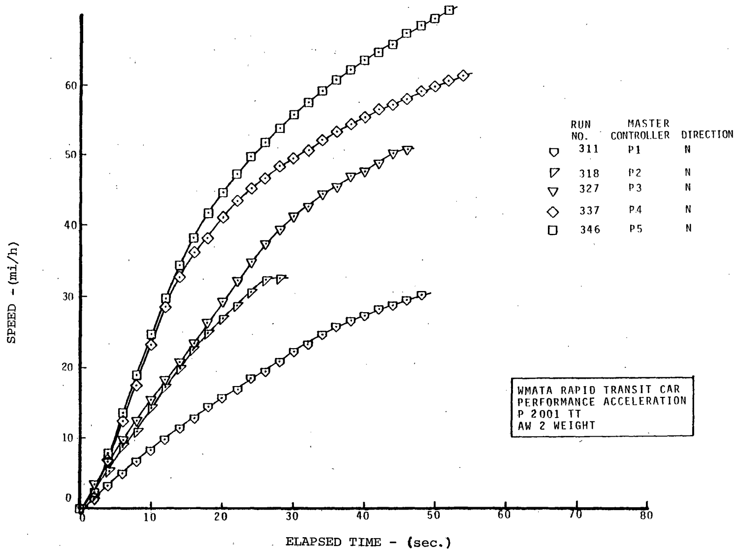
FIGURE 2-3. PERFORMANCE ACCELERATION - SPEED vs. ELAPSED TIME, EFFECT OF MASTER CONTROLLER POSITION.
