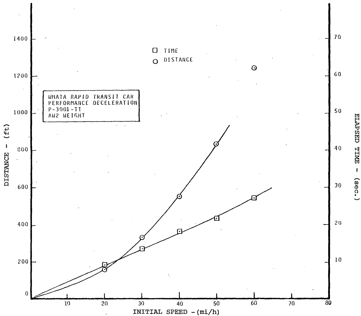
FIGURE 2-13. PERFORMANCE DECELERATION - BRAKE 4 RATE, DISTANCE vs. INITIAL SPEED.
