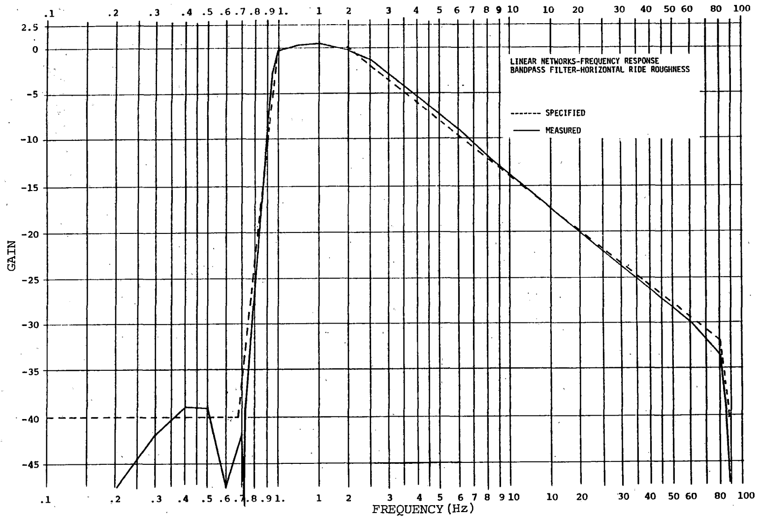
FIGURE 5-2. HORIZONTAL RIDE ROUGHNESS.
