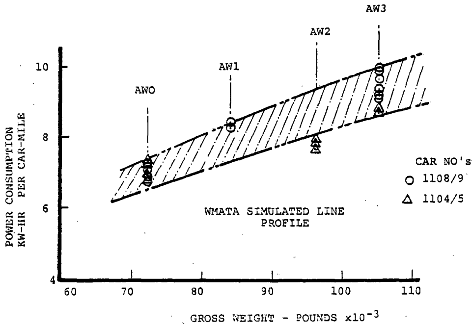
FIGURE 2-21. POWER CONSUMPTION - TREND WITH CAR WEIGHT.
