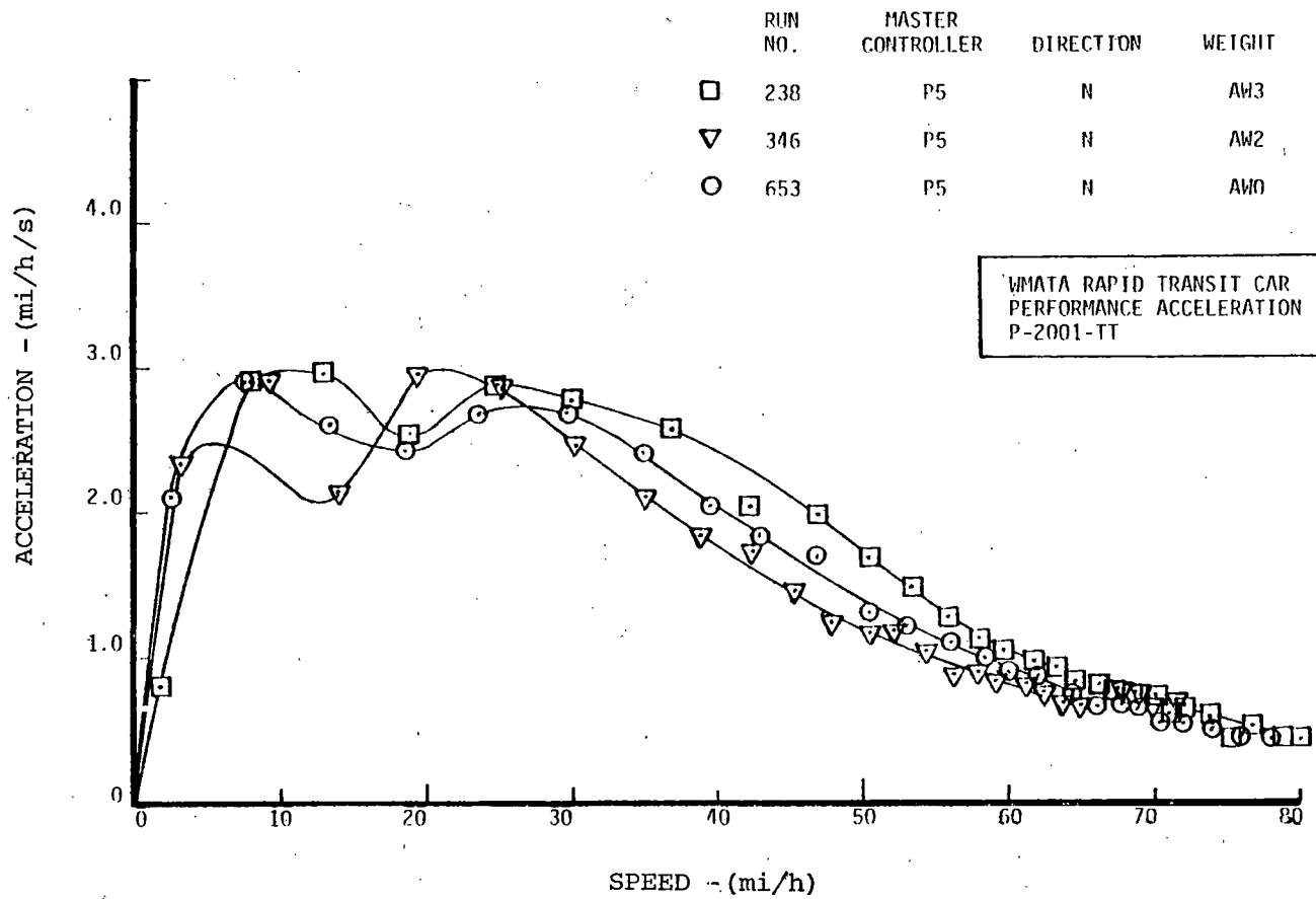
FIGURE 2-5. PERFORMANCE ACCELERATION - LOAD-WEIGH COMPARISON, SPEED vs. ACCELERATION.
