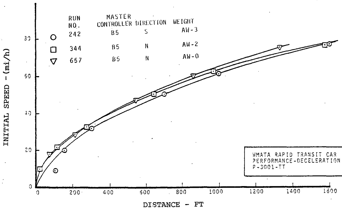
FIGURE 2-17. PERFORMANCE DECELERATION -LOAD-WEIGH COMPARISON, DISTANCE vs. SPEED.
