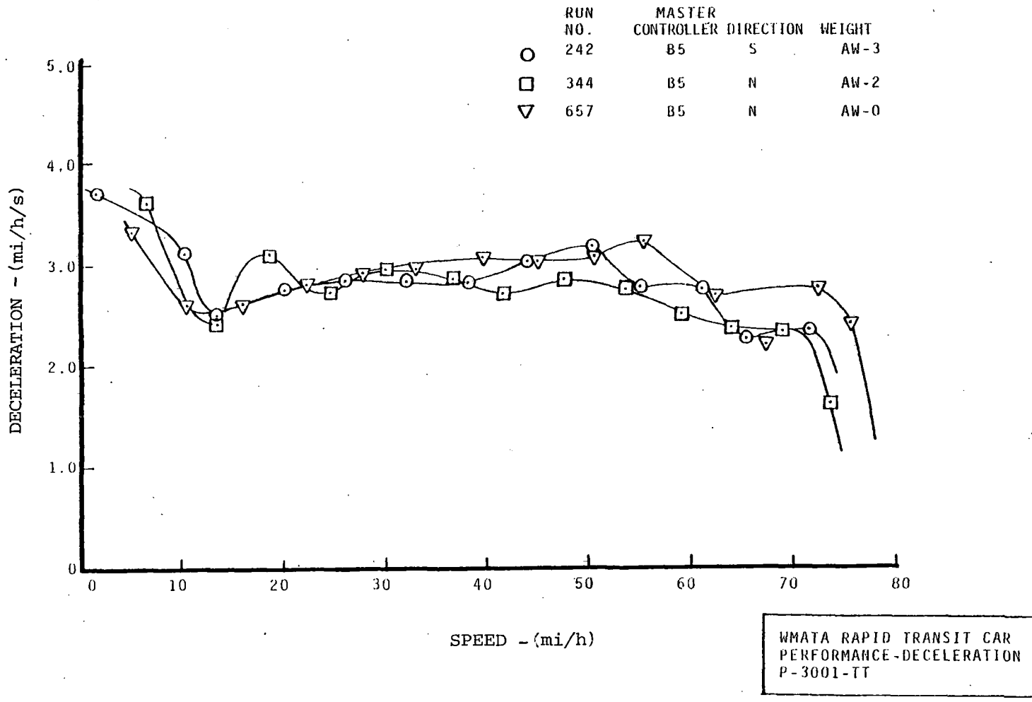
FIGURE 2-15. PERFORMANCE DECELERATION - LOAD-WEIGH COMPARISON, DECELERATION vs. SPEED.
