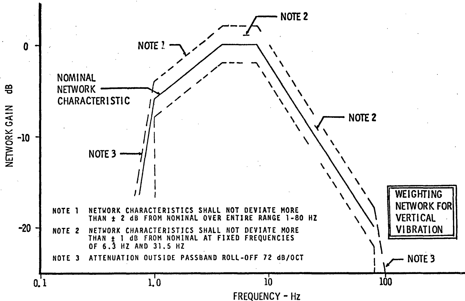
FIGURE 2-29. GVTP VERTICAL RIDE QUALITY FILTER.
