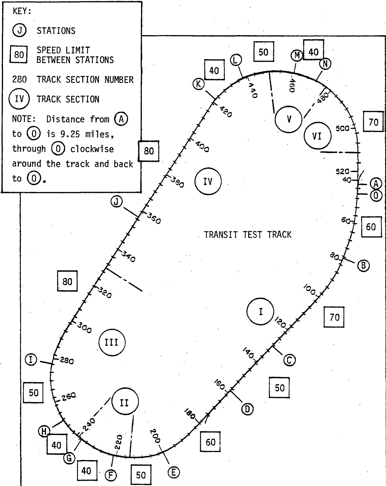
FIGURE 2-20. ACT-1 SYNTHETIC TRANSIT ROUTE.
