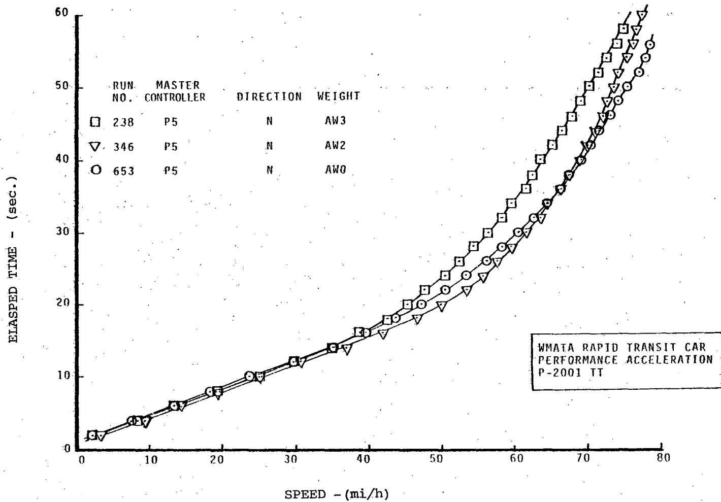
FIGURE 2-6. PERFORMANCE ACCELERATION - LOAD-WEIGH COMPARISON, SPEED vs. ELAPSED TIME.
