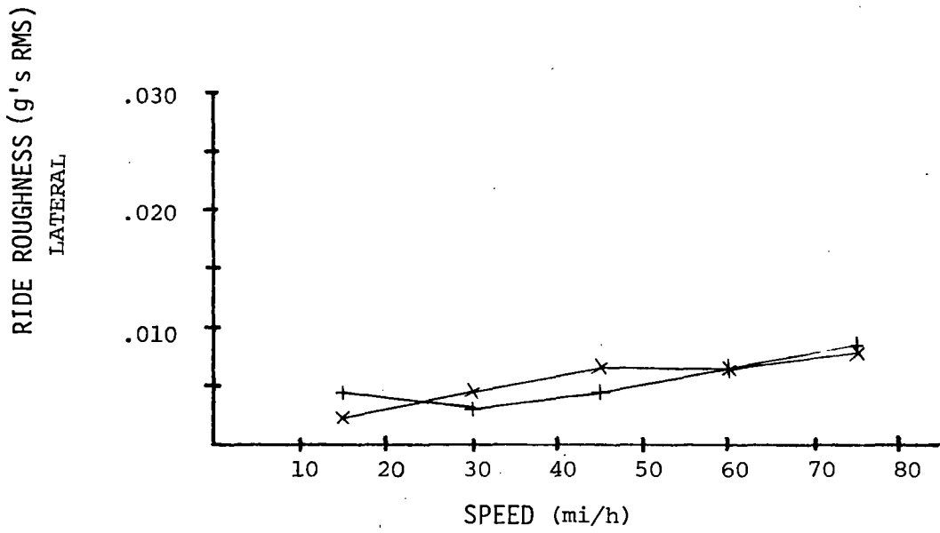
FIGURE 2-36. RIDE ROUGHNESS vs. SPEED, E.
