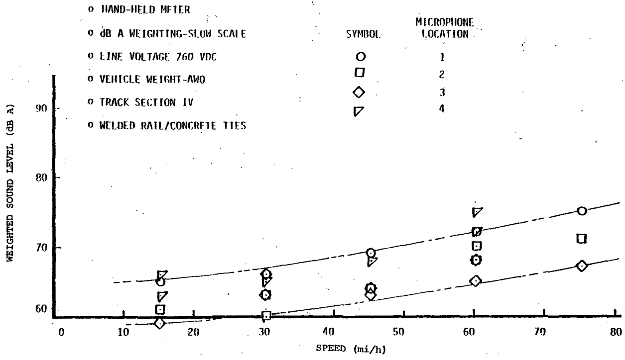
FIGURE 2-25. INTERIOR NOISE LEVELS - EFFECT OF SPEED, AWO WEIGHT.
