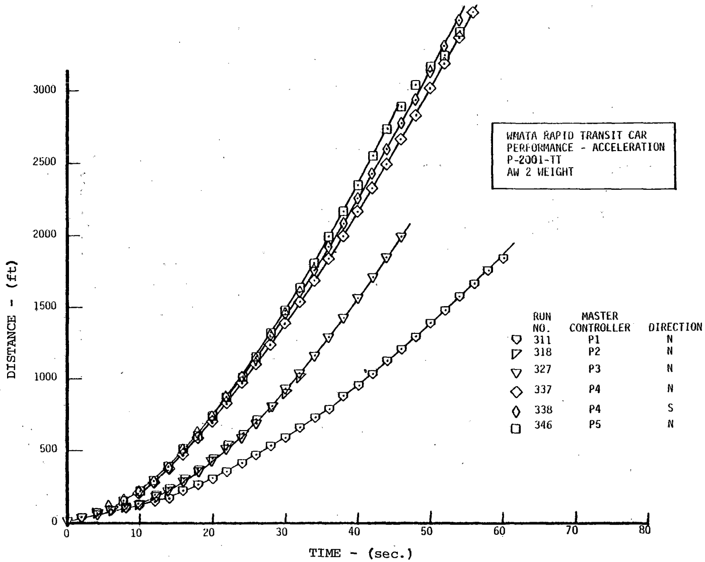
FIGURE 2-4. PERFORMANCE ACCELERATION - TIME vs. DISTANCE, EFFECT OF MASTER CONTROLLER POSITION.
