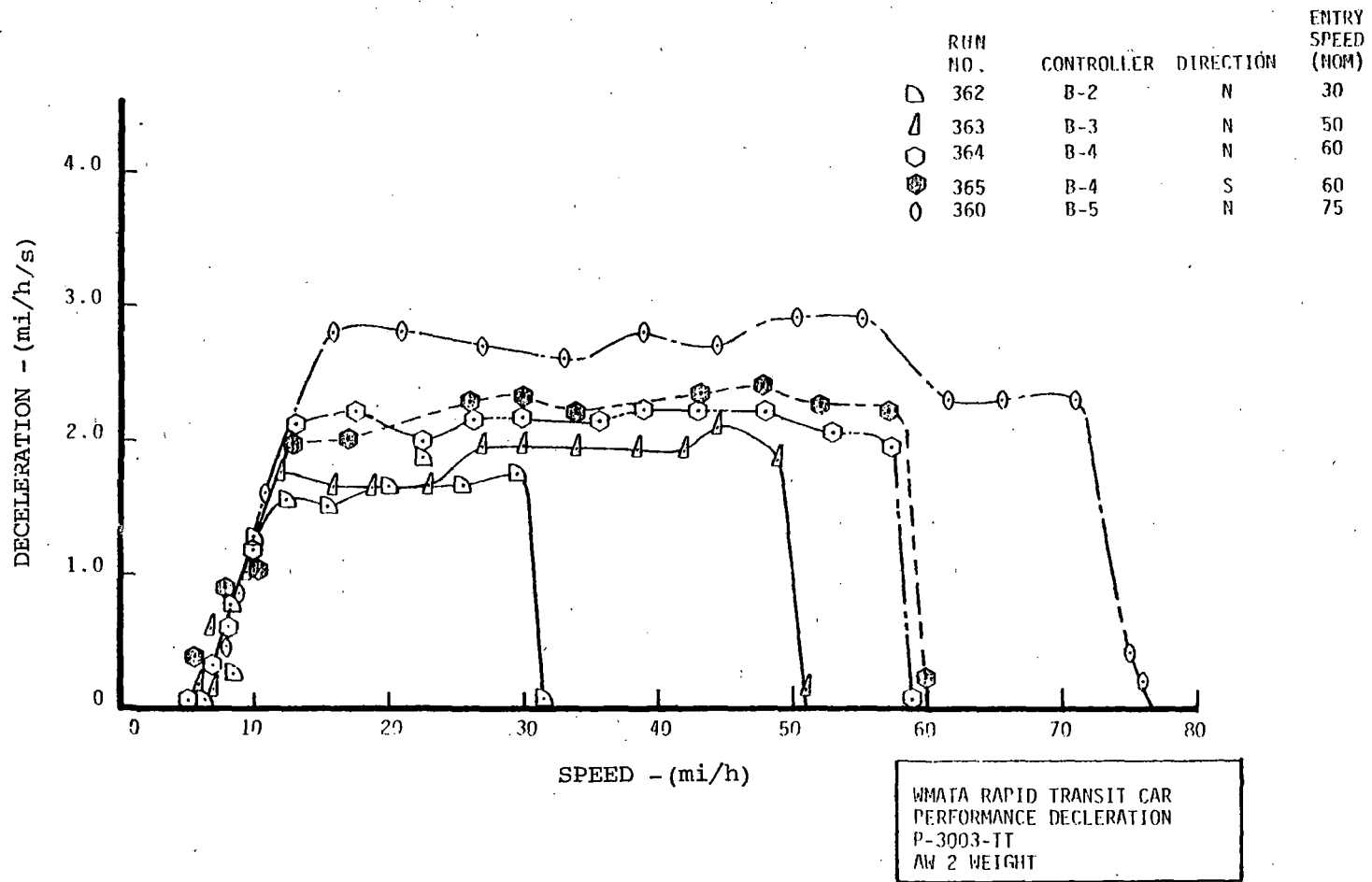
FIGURE 2-11. PERFORMANCE DECELERATION - DYNAMIC-ONLY BRAKING, DECELERATION vs. SPEED.
