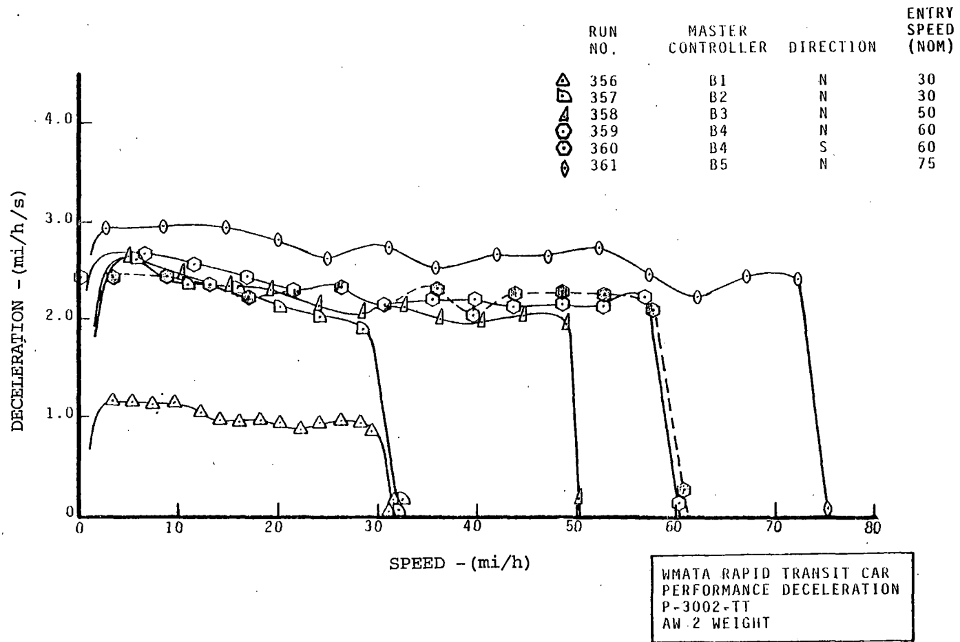
FIGURE 2-10. PERFORMANCE DECELERATION - FRICTION-ONLY BRAKING, DECELERATION vs. SPEED.
