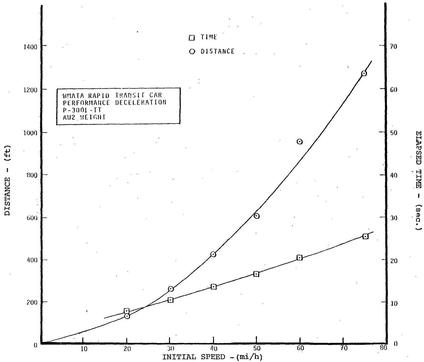
FIGURE 2-12. PERFORMANCE DECELERATION - BRAKE 5 RATE, DISTANCE vs. INITIAL SPEED.
