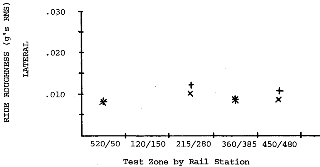
FIGURE 2-30. RIDE ROUGHNESS vs. TEST ZONES, A.
