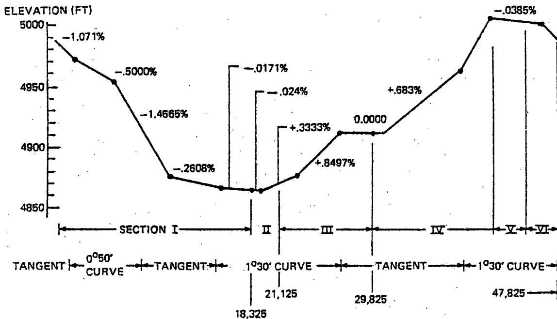
FIGURE 1-3. TRANSIT TEST TRACK PROFILE SHOWING GRADES.
