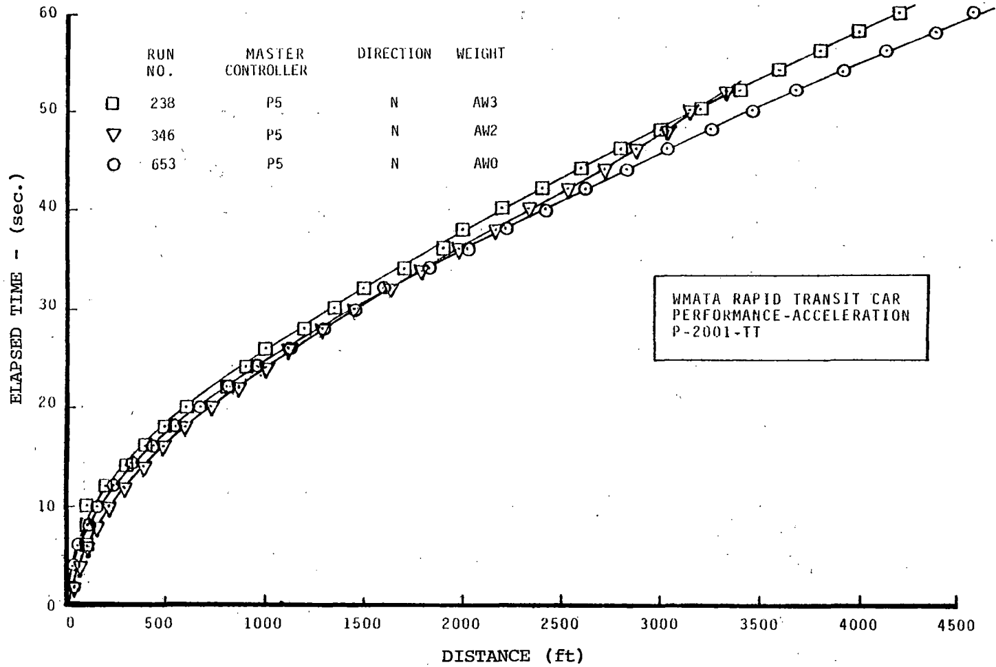
FIGURE 2-7. PERFORMANCE ACCELERATION - LOAD-WEIGH COMPARISON, TIME vs. DISTANCE.
