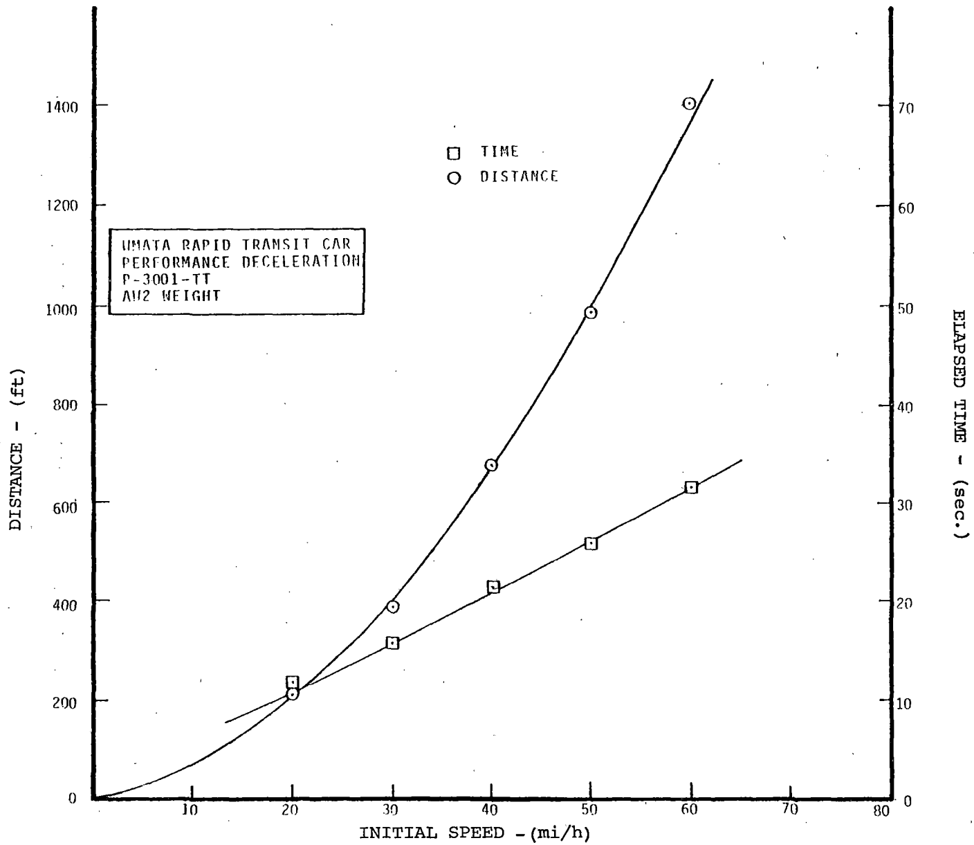
FIGURE 2-14. PERFORMANCE DECELERATION - BRAKE 3 RATE, DISTANCE vs. INITIAL SPEED.
