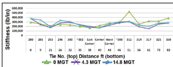
Figure 3. Vertical Track Stiffness
