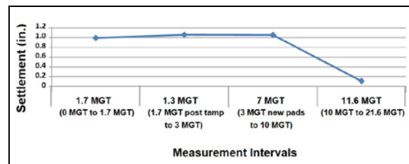
Figure 5. Settlement rate at the center of the diamond during three measurement cycles
