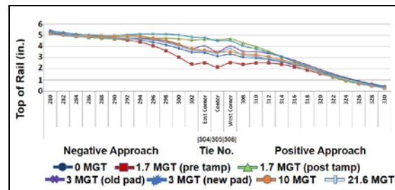
Figure 4. Top of Rail Elevation
