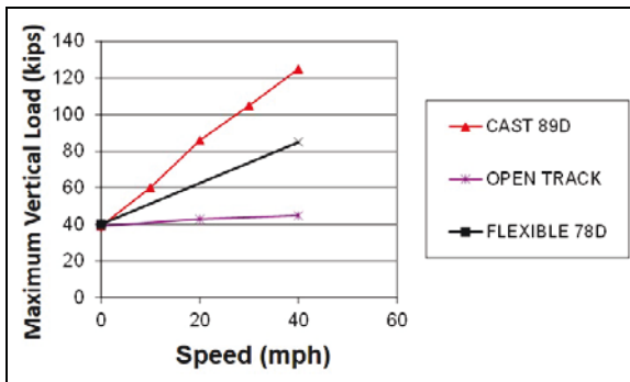
Figure 8. Measured Maximum Vertical Loads
