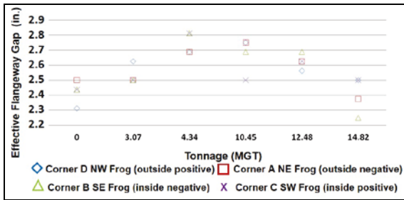
Figure 7. Flangeway gaps measured on the prototype diamond
