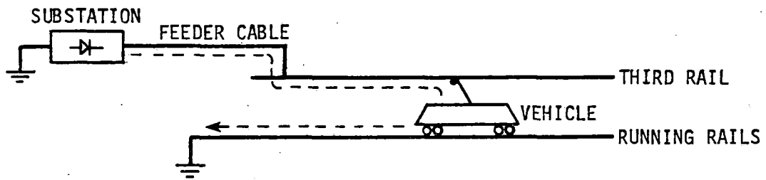
(a) CIRCUIT COMPONENTS
