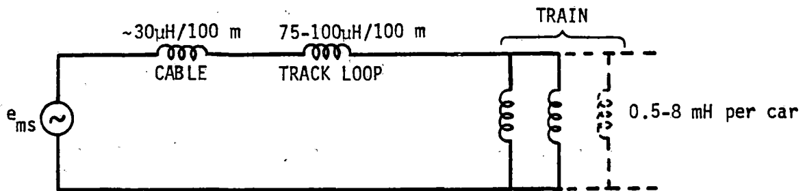
(c) CIRCUIT CONSTANTS
