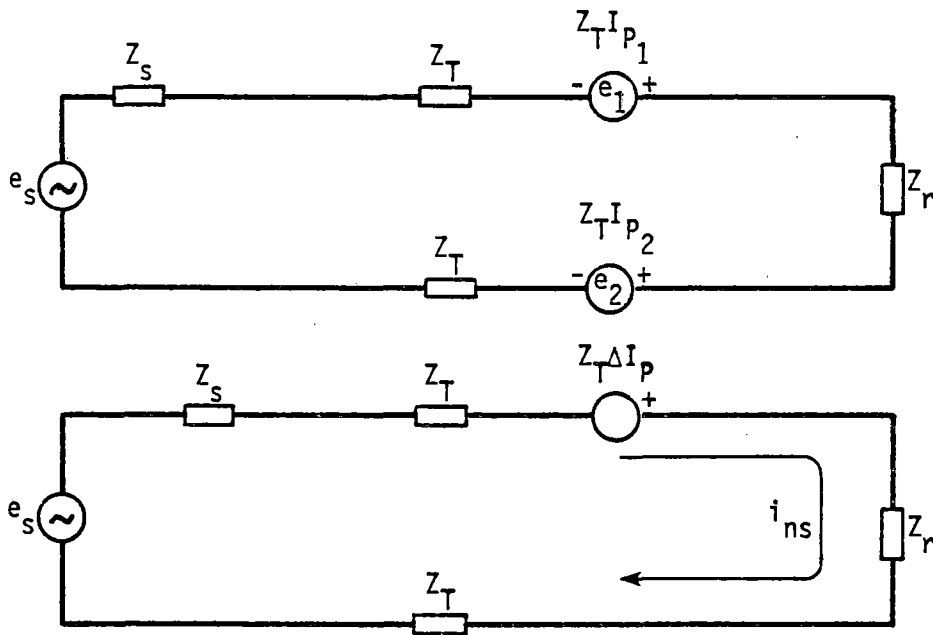
B. EQUIVALENT CIRCUITS
