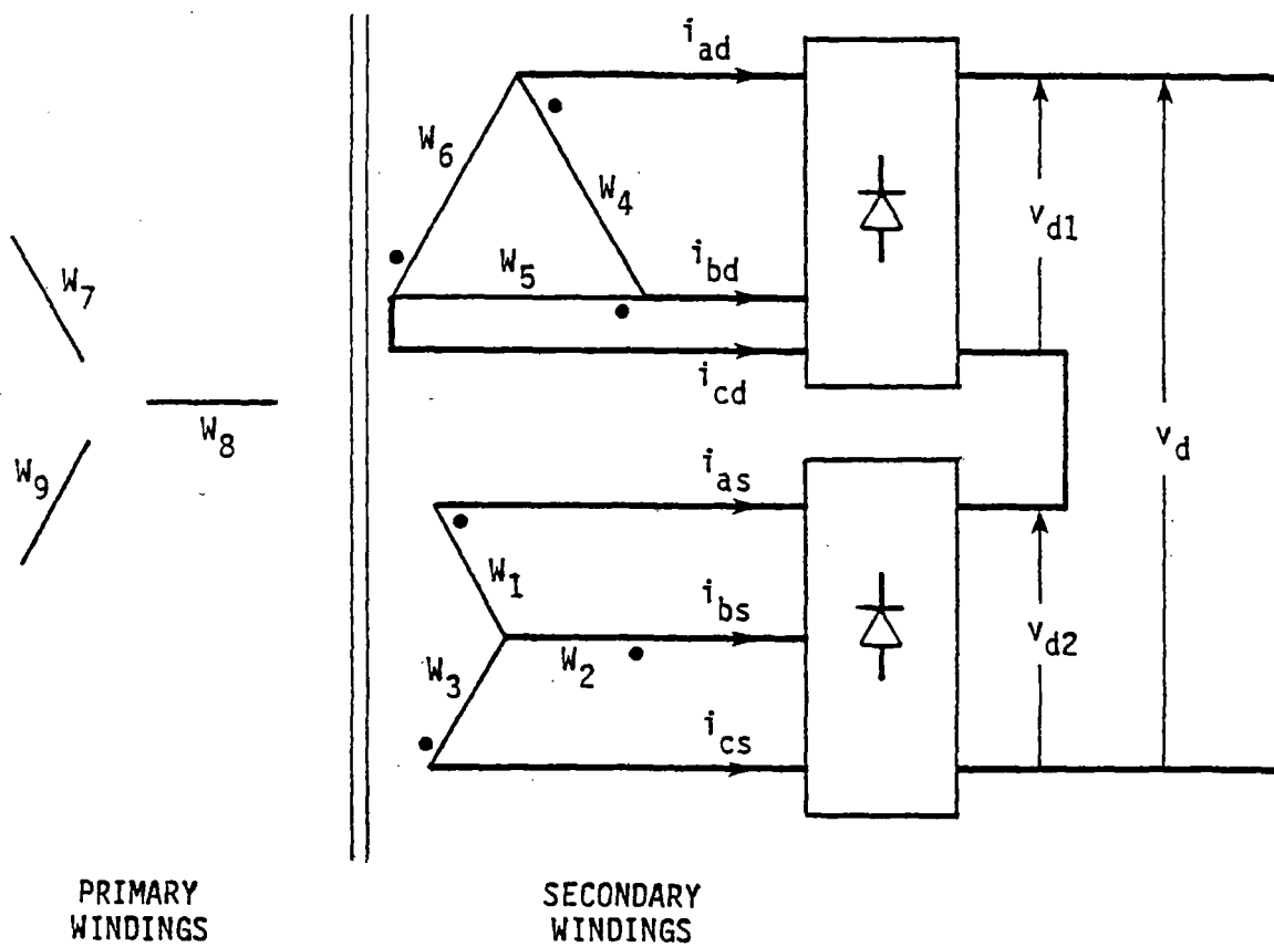
FIGURE 2-11. A 12-Pulse Rectifier (Series Connection)
