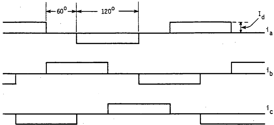
FIGURE 2-3. Line Current Waveforms
