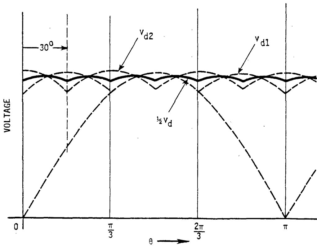
FIGURE 2-12. Output Voltage of 12-Pulse Circuit
