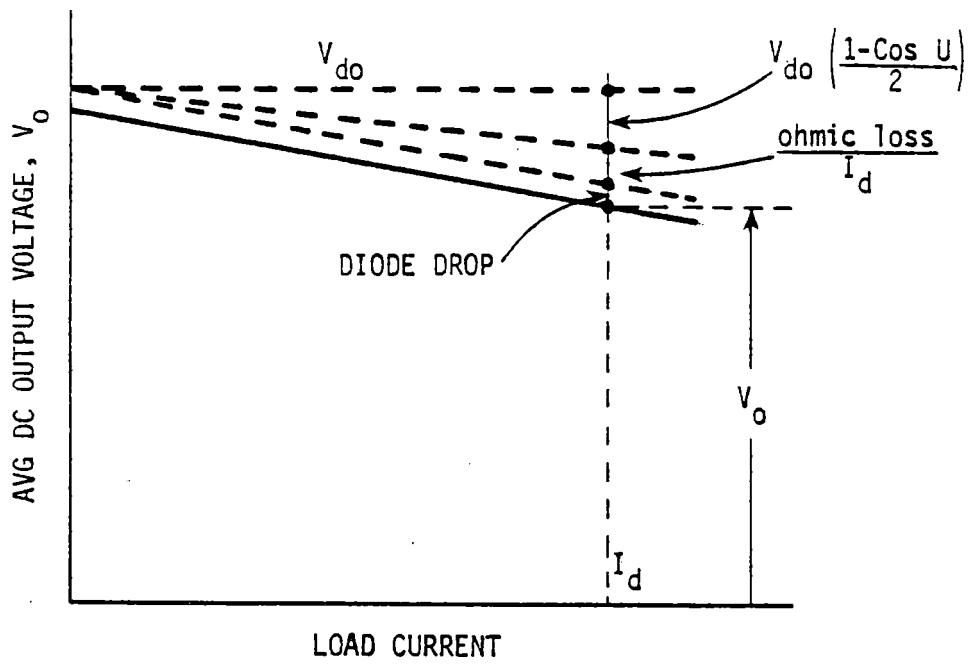
FIGURE 2-7. Voltage Regulation
