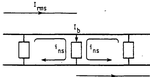
b) THIRD RAIL ON BOTH SIDES
