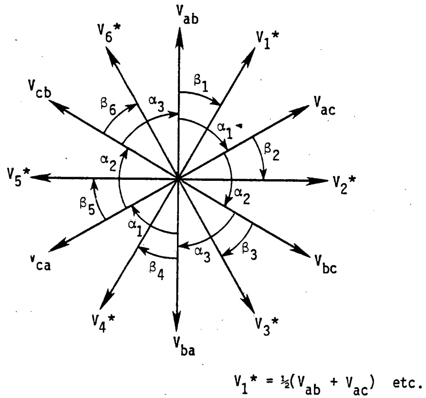
FIGURE A-1. Phasor Diagram
