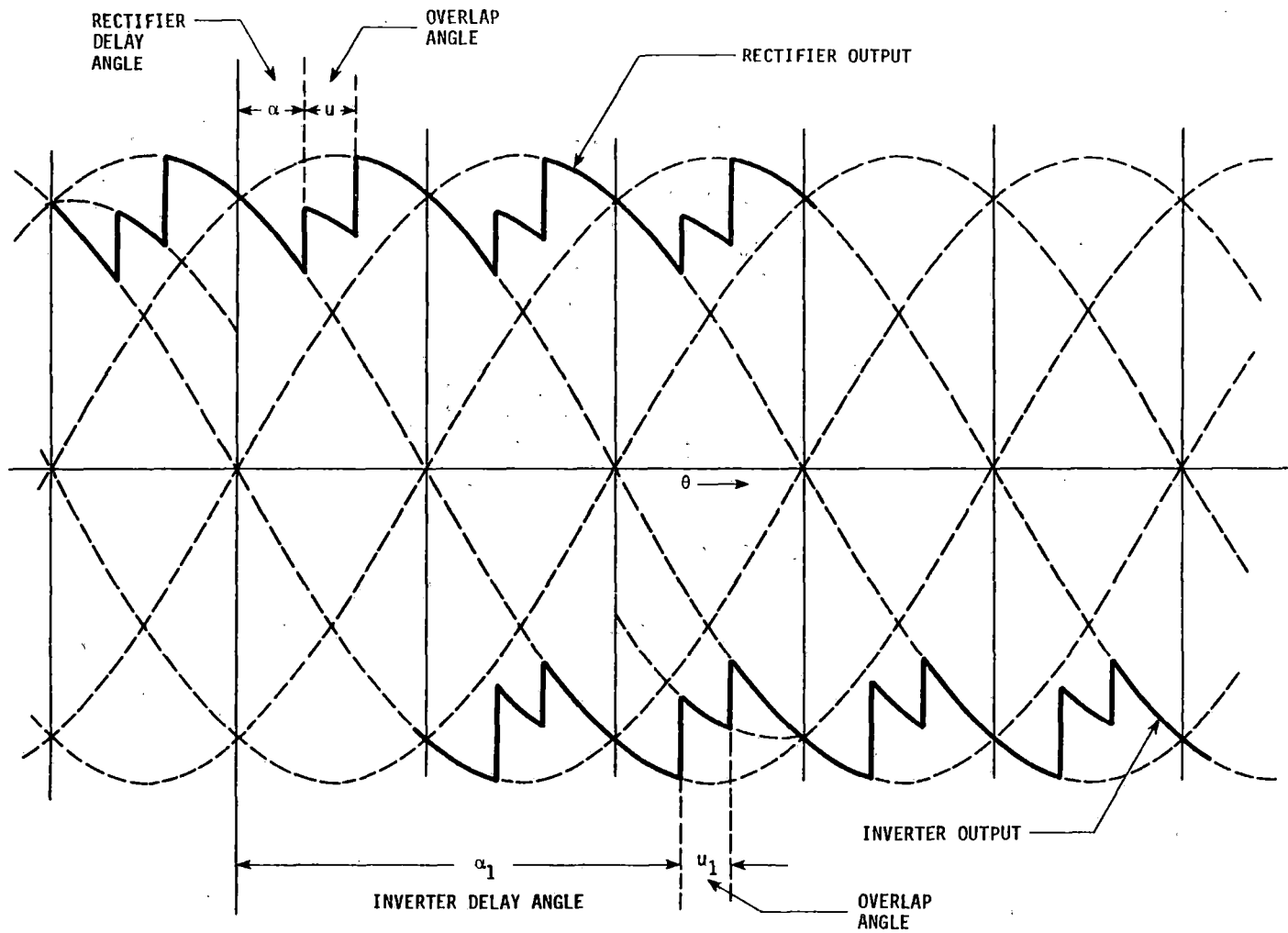
FIGURE 2-15. Operating Modes of a Controlled Rectifier
