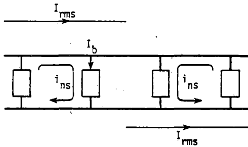
c) THIRD RAIL ON BOTH SIDES
