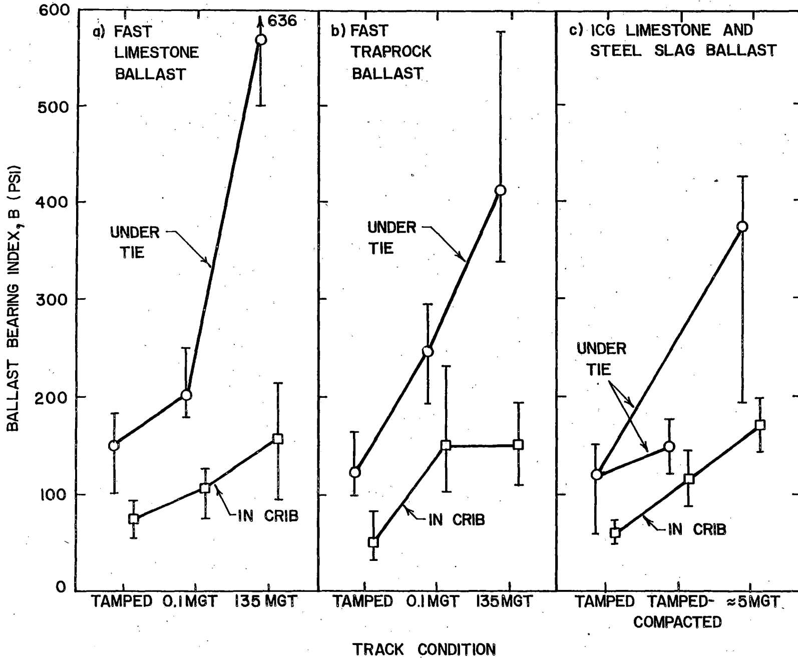
Figure 4.7. Summary of ICG and FAST PLT at 0.2 in. (5.1 mm) Displacement Under the Rail
