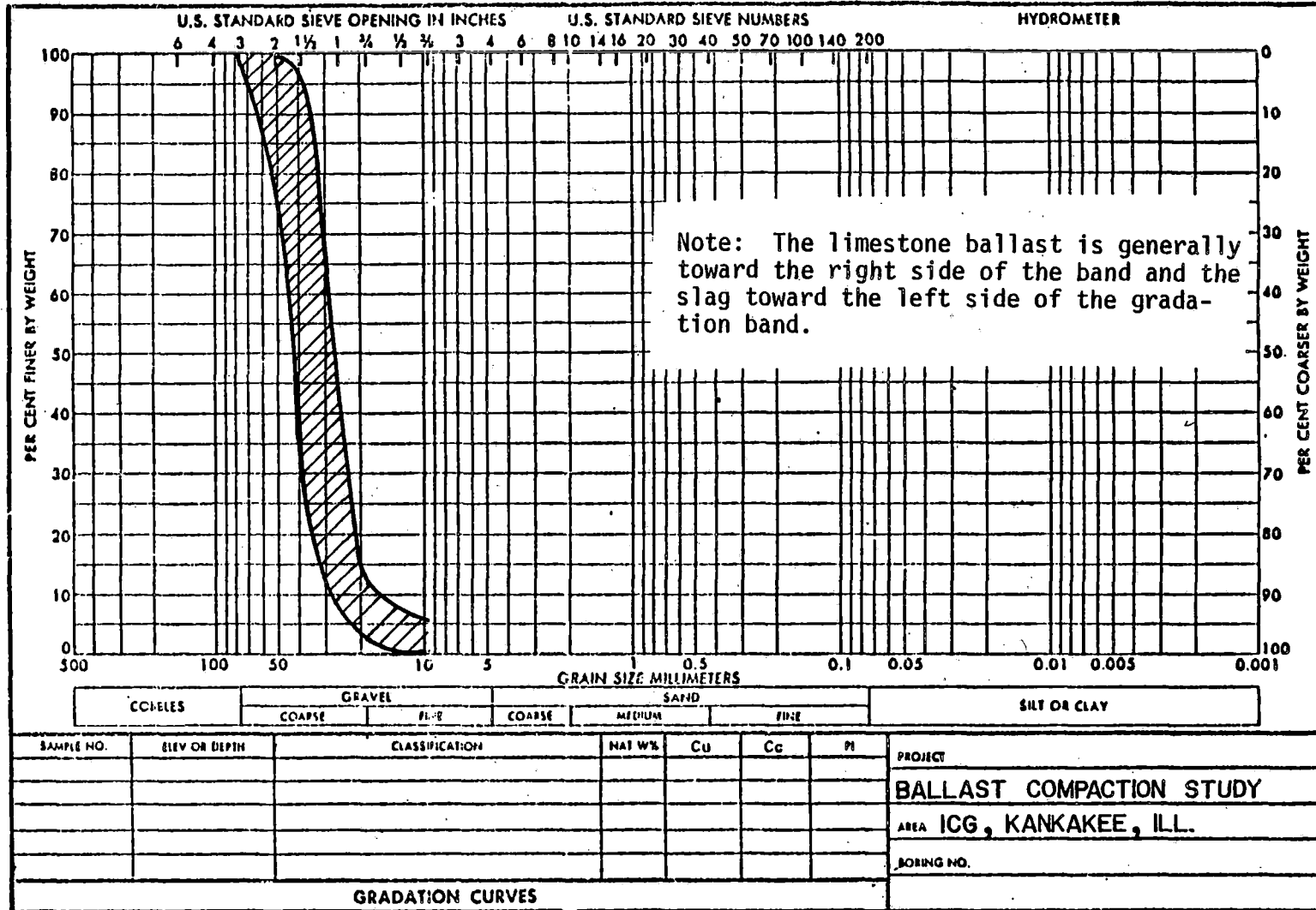
Figure 2.3. Gradation Distribution of Ballast at the ICG Site
