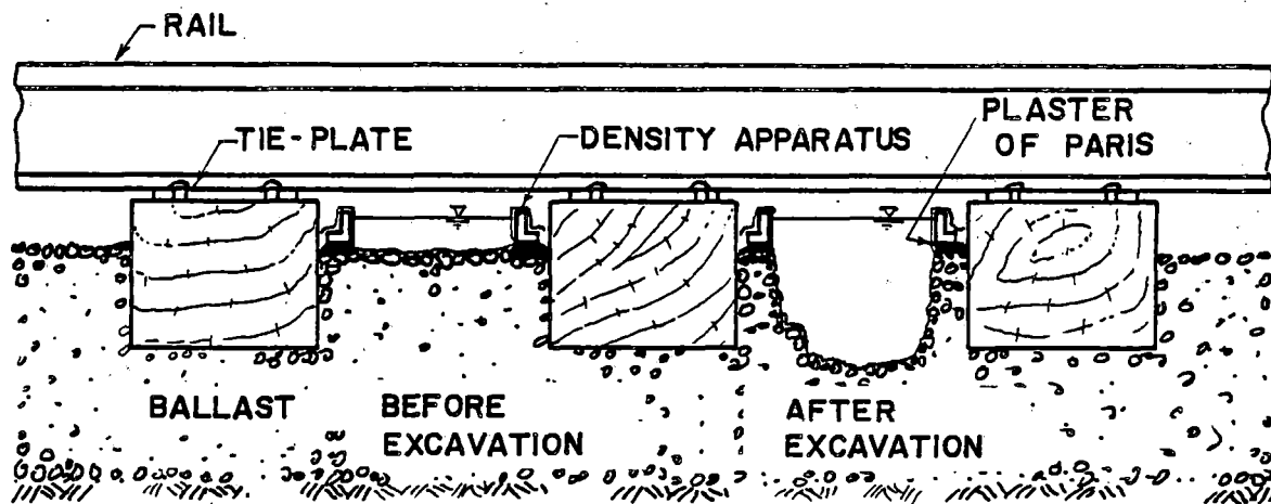
Figure 3.2. Schematic Illustration of In-situ Ballast Density Measurement Using the Preliminary Apparatus
