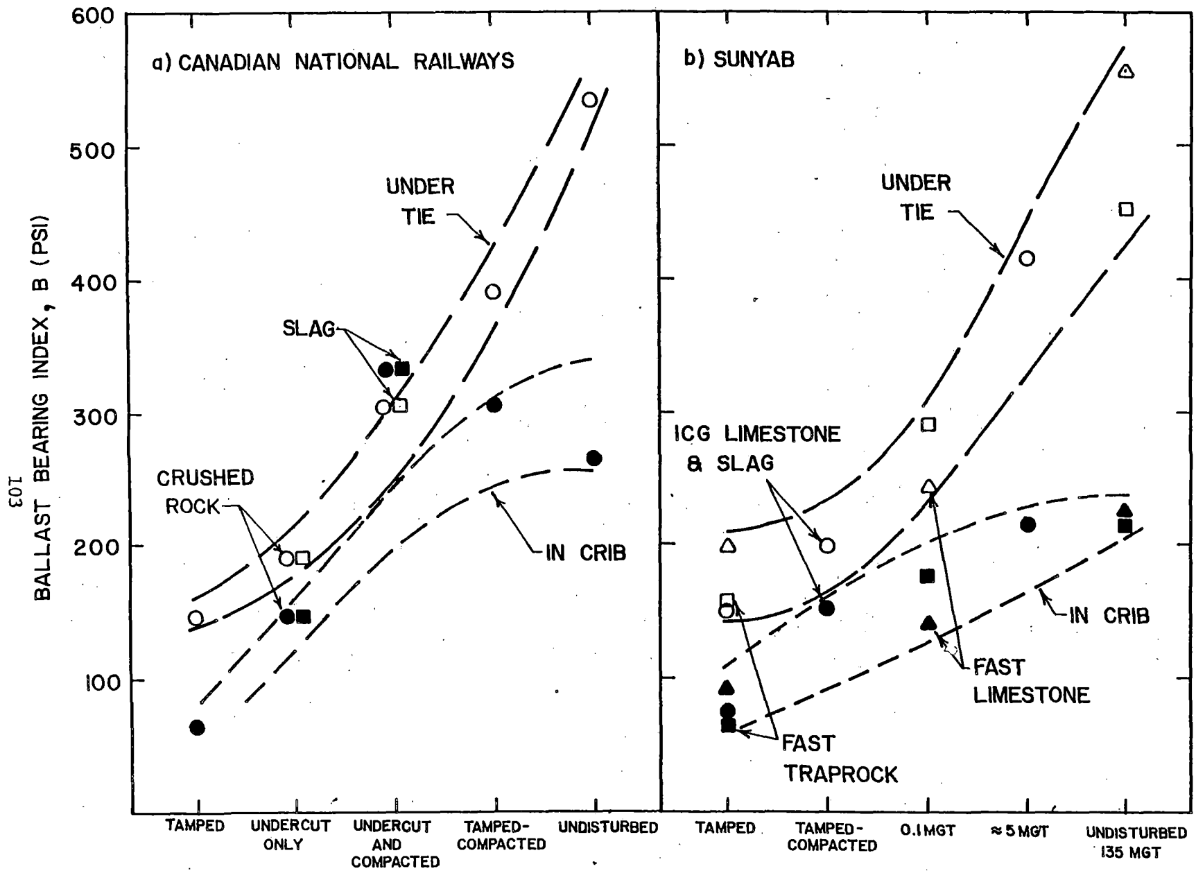
Figure 4.8. Ballast Bearing Index at 0.3 in. (7.6 mm) Plate Displacement under the Rail for Various Track Conditions
