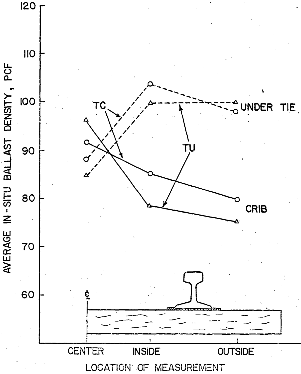
Figure 3.8. Average In-situ Ballast Density Measured During Initial Tests at the ICG Site
