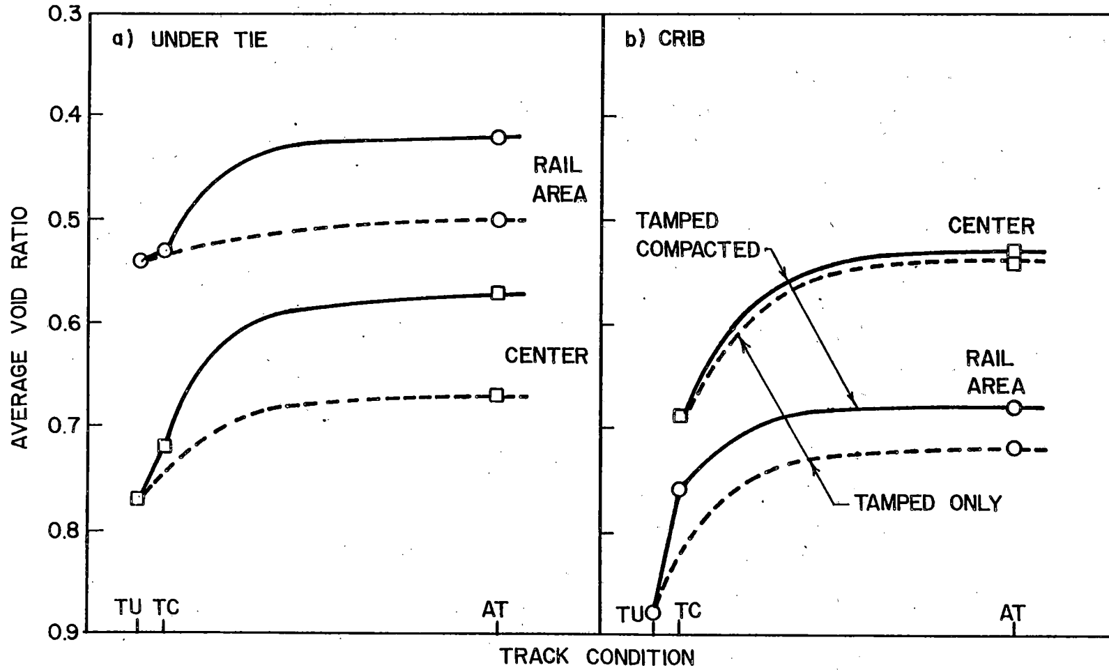
Figure 3.29. Effect of Crib and Shoulder Compaction on the Ballast Density, ICG
