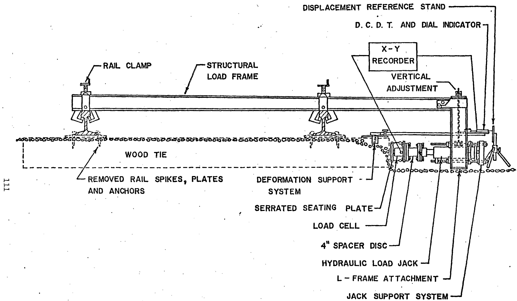
Figure 5.1. Assembled Lateral Tie Push Test Apparatus (Ref. 1)
