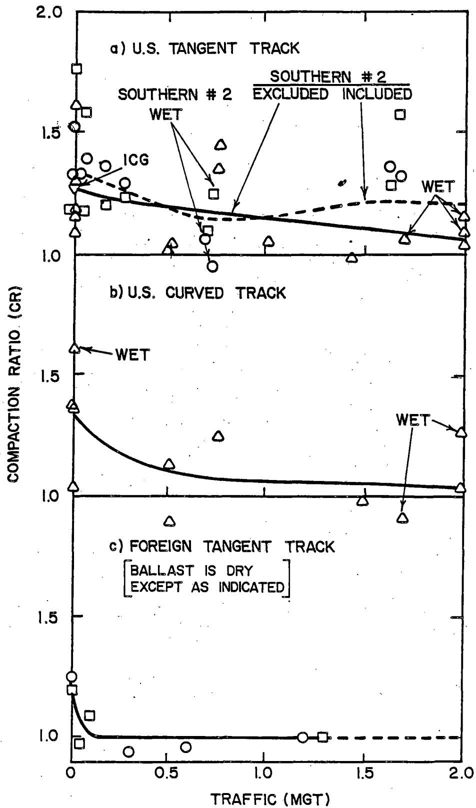
Figure 5.18. Summary of LTPT Compaction Ratio at 0.157 in. (4 mm) Displacement for all Data
