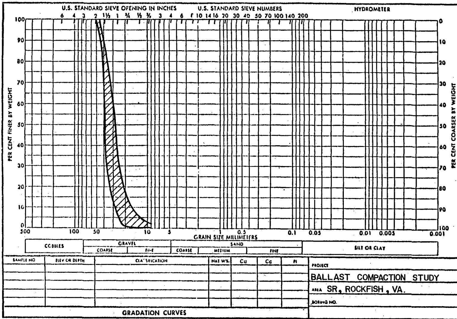
Figure 2.2. Gradation Distribution of Granite Ballast at the SR Site
