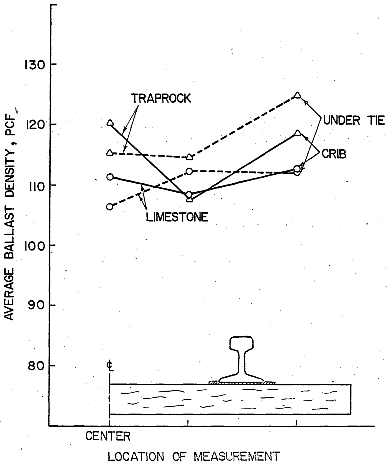
Figure 3.19. Distribution of Ballast Density Along the Tie for Different Ballast Types, After Additional 0.1 MGT, FAST
