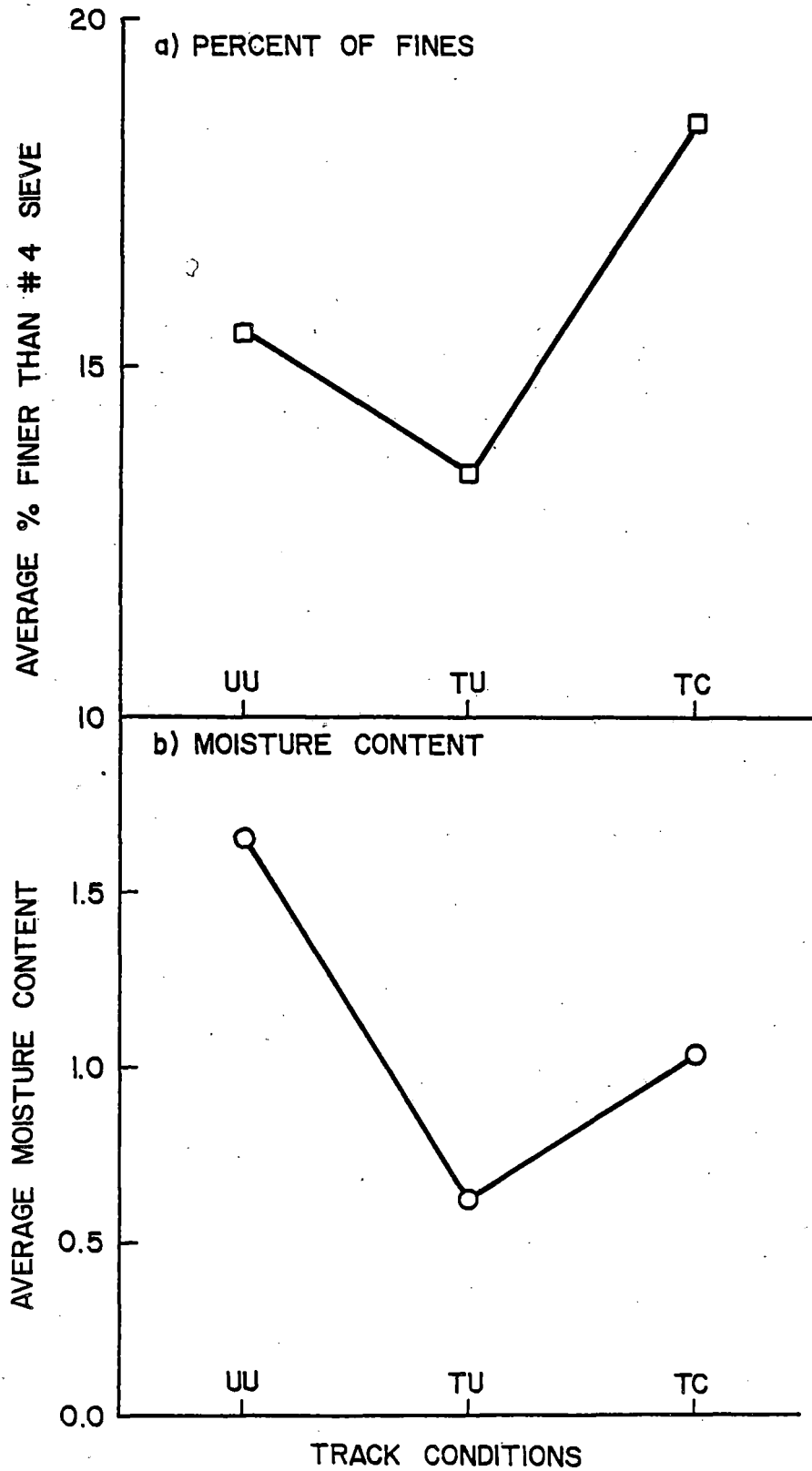
Figure 3.31. Changes in Percent Fines and Moisture Content in the Ballast Layer with Track Conditions, CNR
