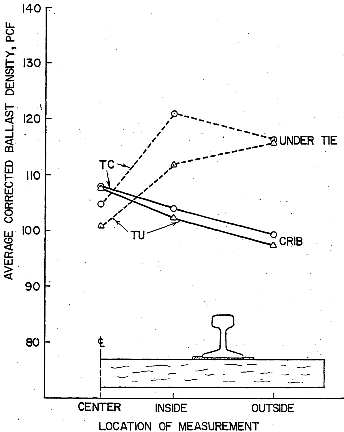
Figure 3.12. Average Corrected Ballast Density Measured during Follow-up Tests for Different Initial Conditions at the ICG Site
