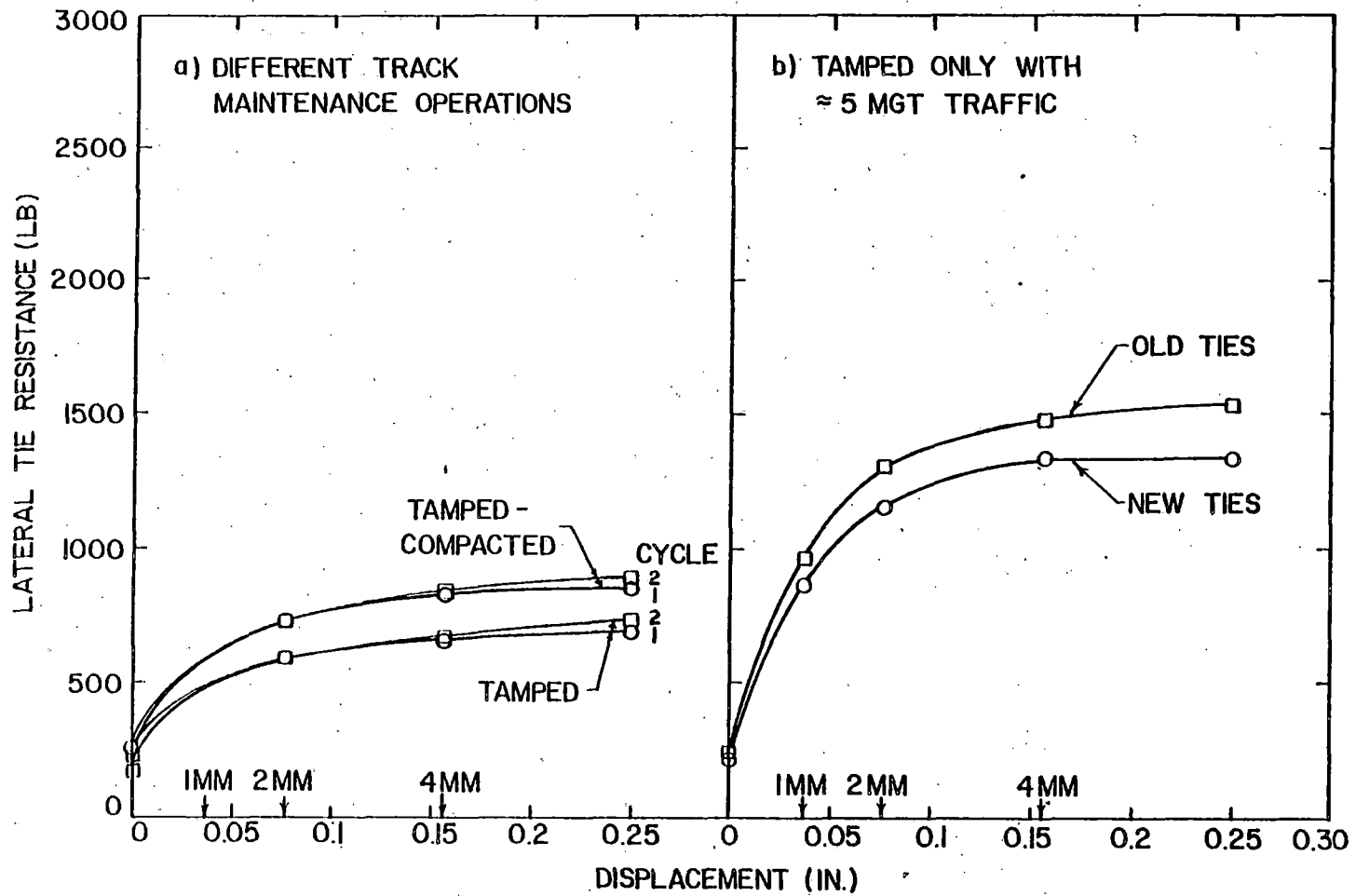
Figure 5.2. LTPT Load-Displacement Curves for ICG Limestone and Steel Slag Ballast
