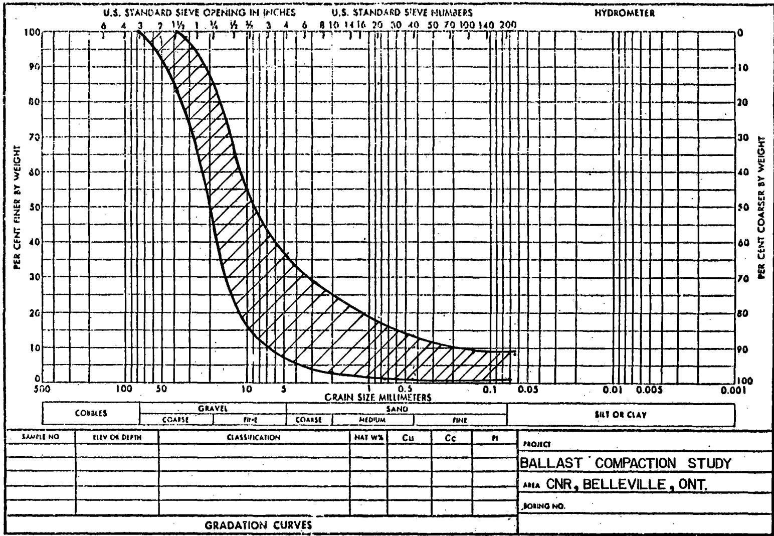
Figure 2.1. Gradation Distribution of Nickel Slag at the CNR Site
