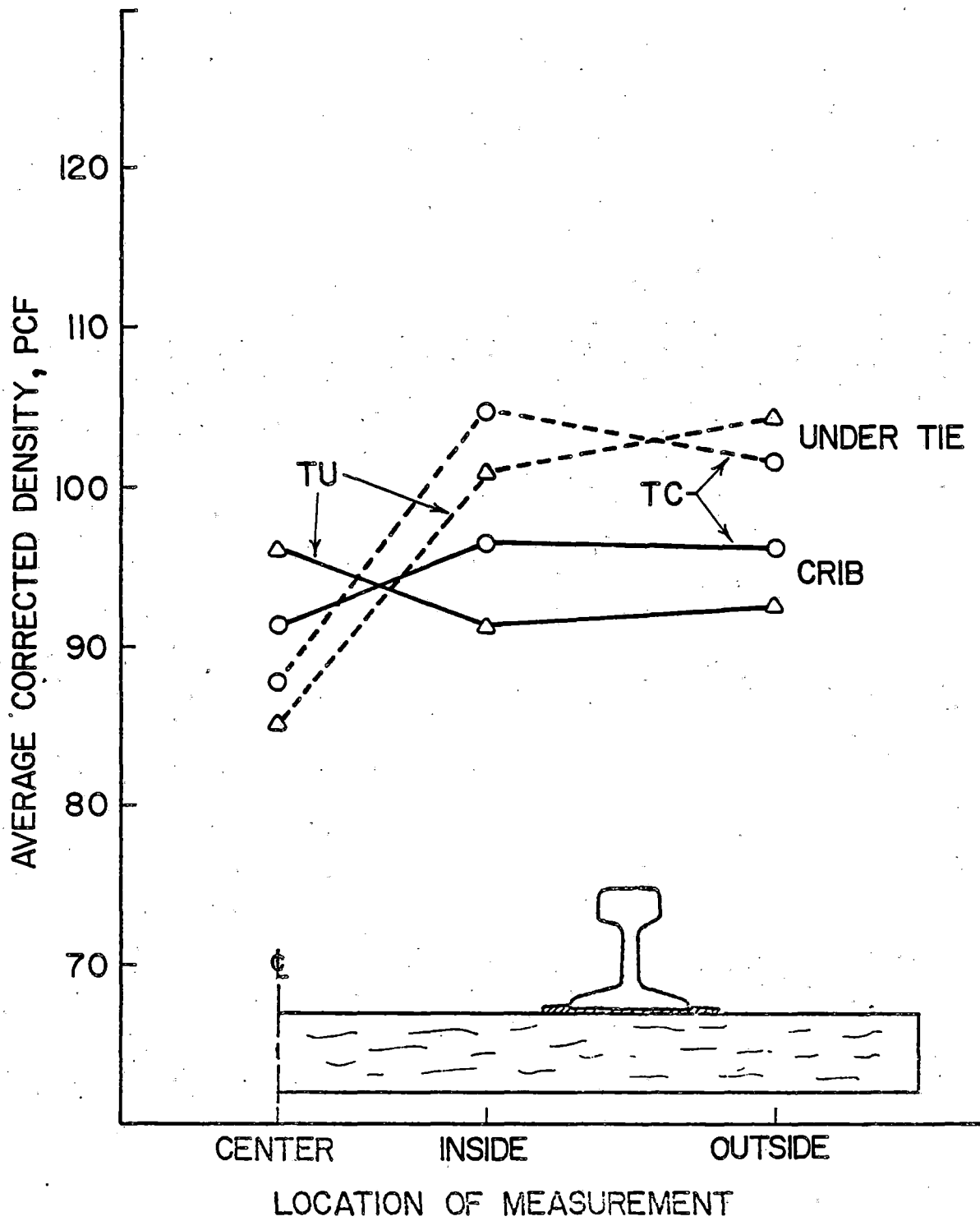
Figure 3.9. Average In-situ Ballast Density after Correction
