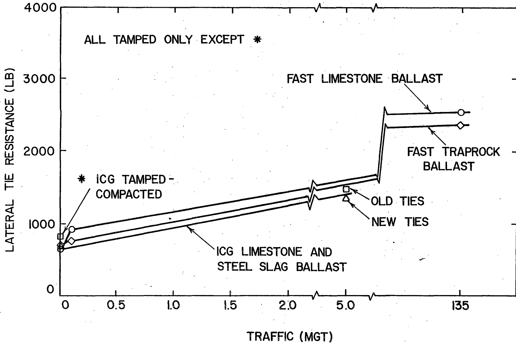
Figure 5.13. SUNYAB LTPT Results on Tangent Track at 0.157 in. (4 mm) Displacement for Various Track Conditions
