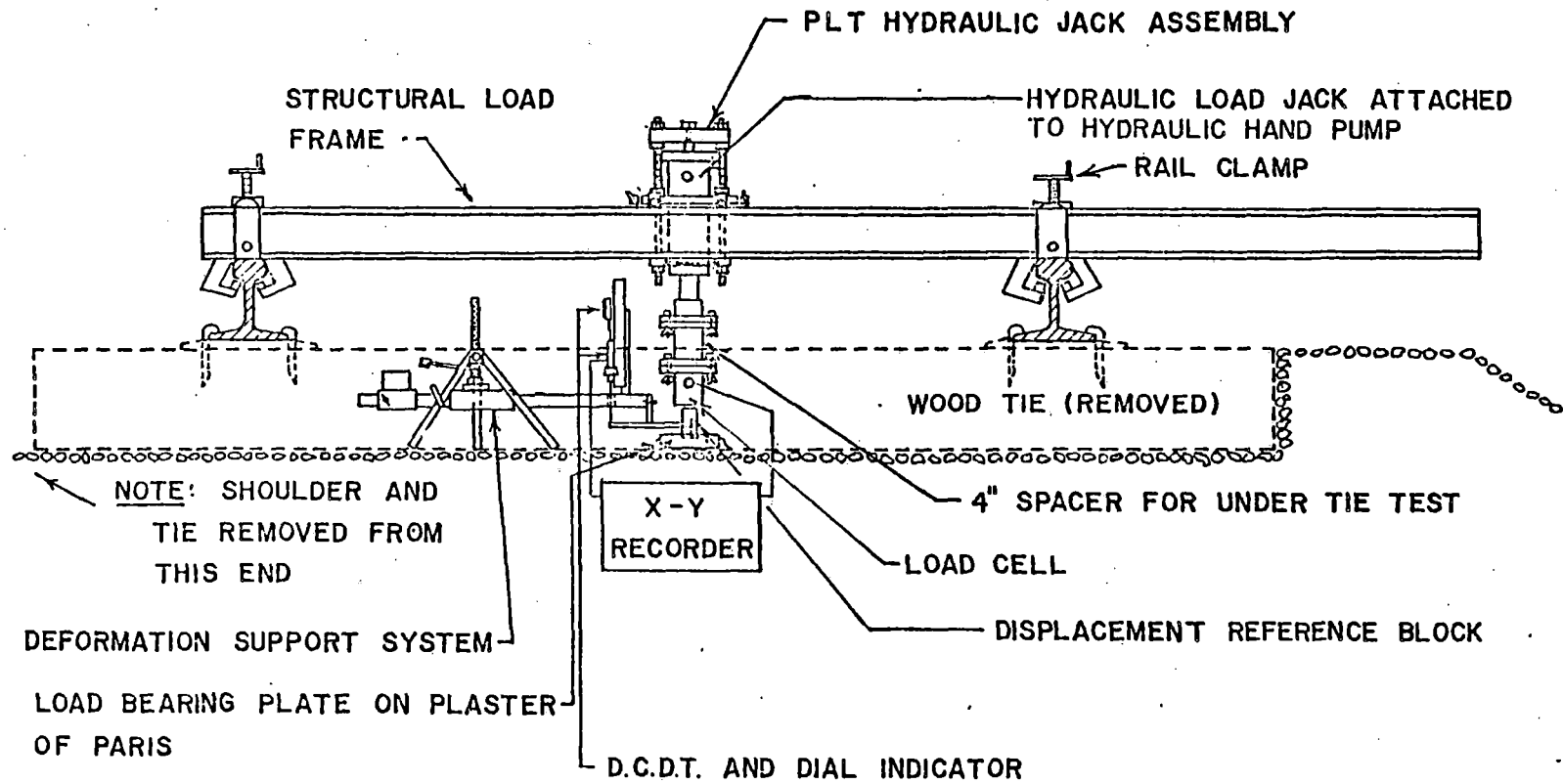
Figure 4.1. Assembled Plate Load Test Apparatus
