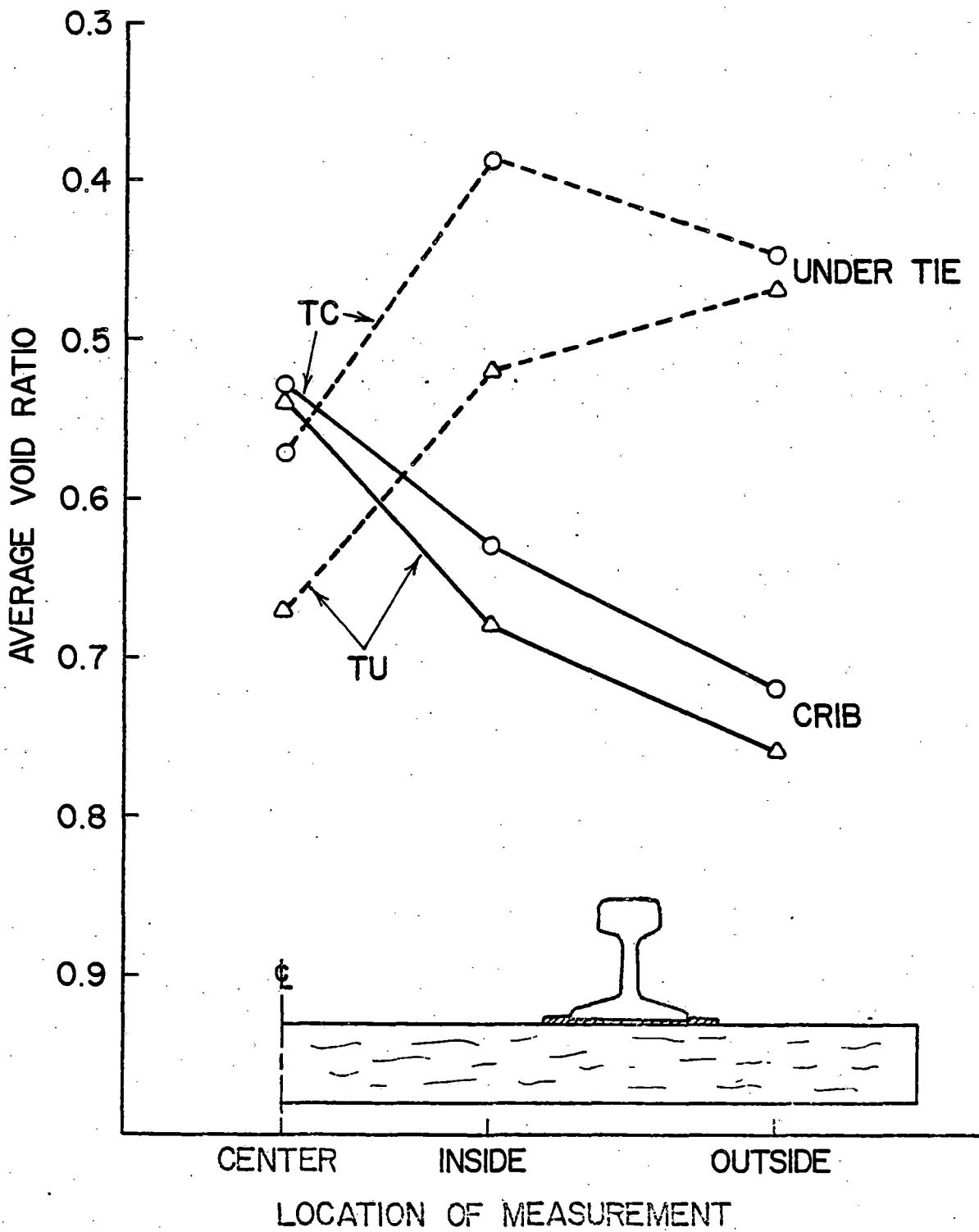
Figure 3.13. Average Void Ratio Obtained during Follow-up Tests for Different Initial Conditions at the ICG Site
