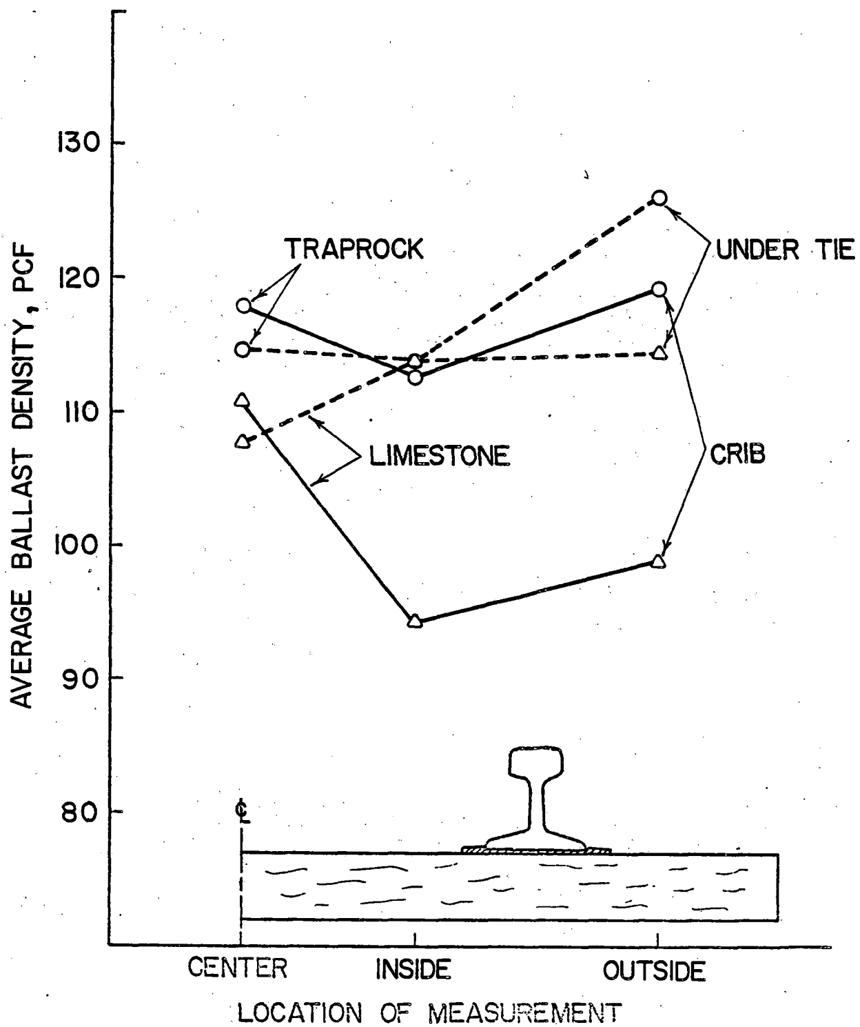
Figure 3.18. Distribution of Ballast Density Along the Tie for Different Ballast Types, After Maintenance Tamping, FAST
