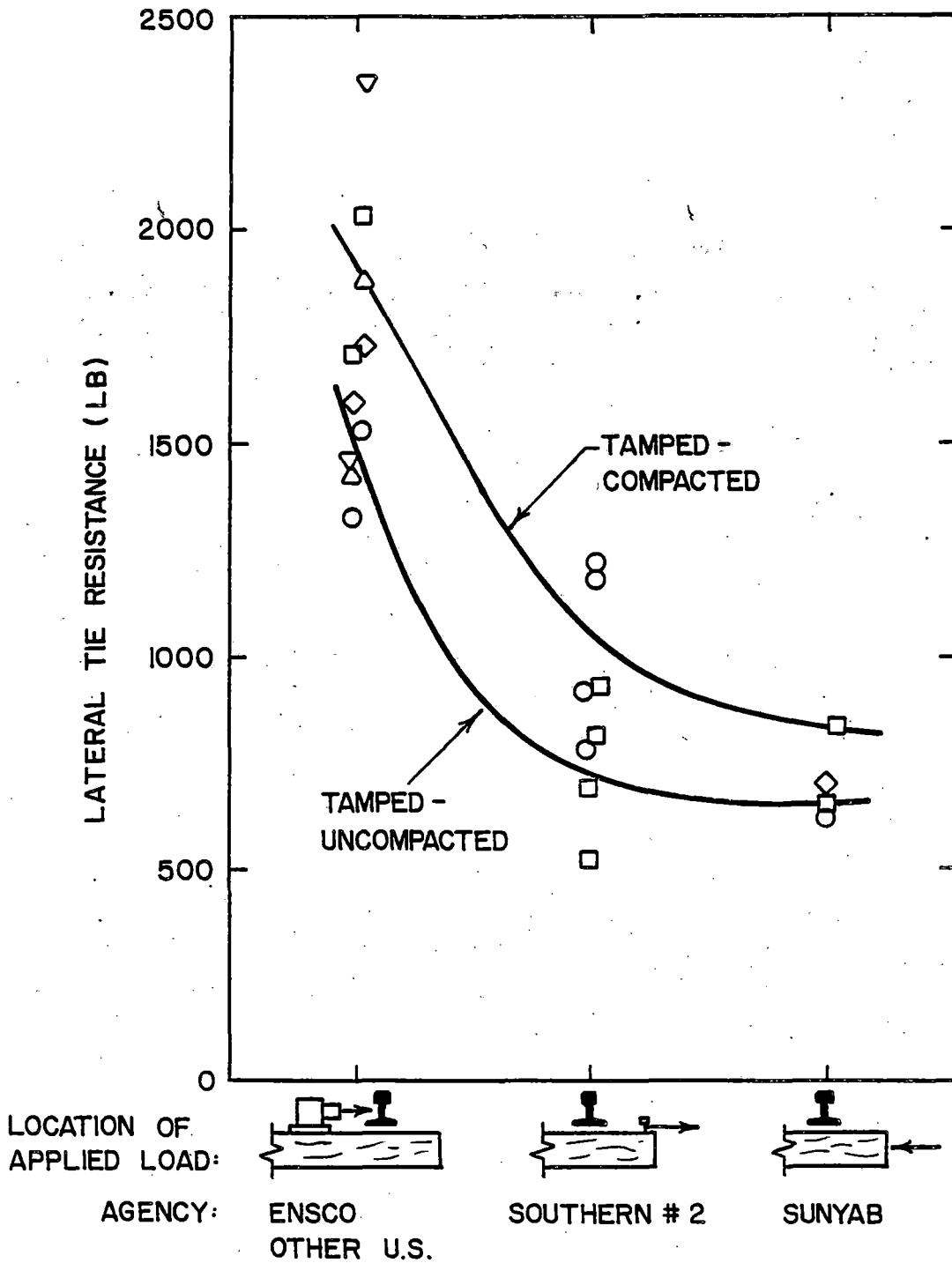
Figure 5.15. Comparison of LIPT Results at 0.157 in. (4 mm) Displacement with Location of Load Applying System on U.S. Tangent Track at Zero MGT Traffic
