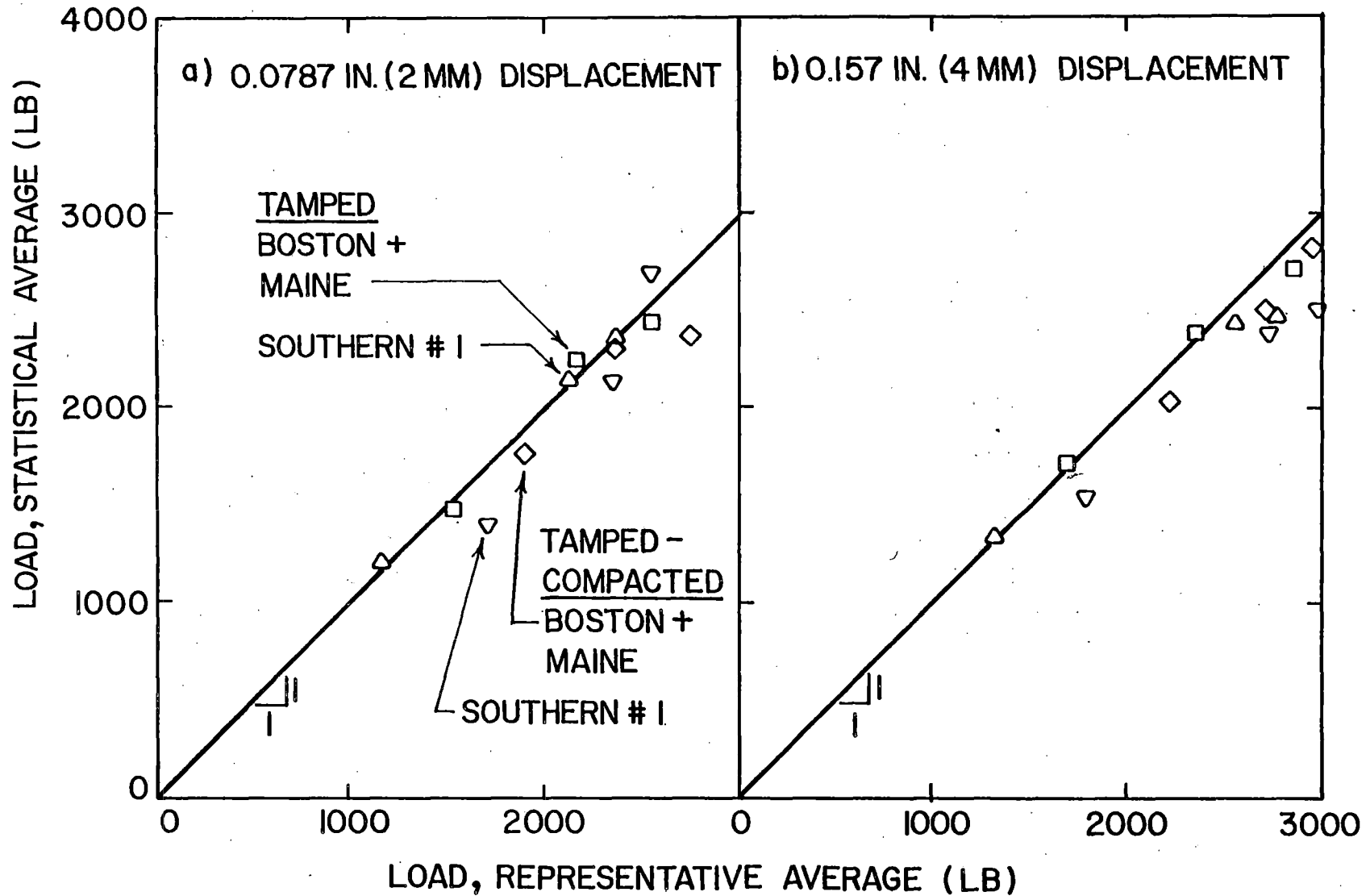
Figure 5.7. Comparison of Statistical and Representative Average LTPT Results on U.S. Tangent Track for Different Track Conditions
