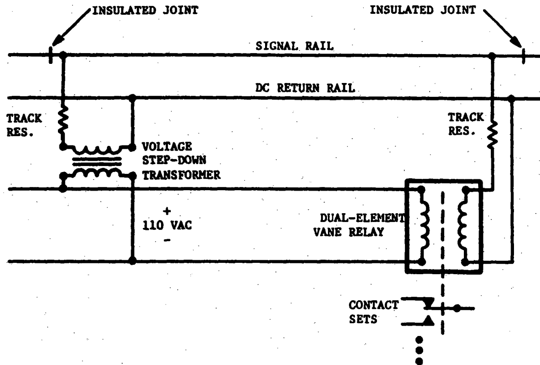
FIGURE 1-3. A SINGLE-RAIL POWER-FREQUENCY TRACK CIRCUIT
