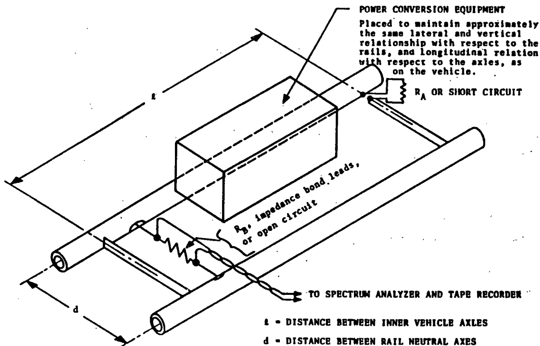
FIGURE RT/IE04A-1. TEST SETUP
