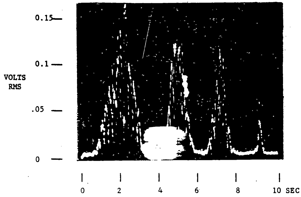
b. STRENGTH OF 9TH HARMONIC (3600 HZ) OF RAIL-TO-RAIL VOLTAGE AS TRAIN PASSES
