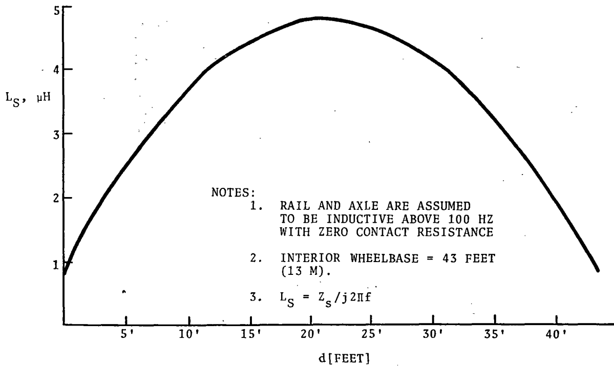
FIGURE 1-9. PLOT OF SOURCE INDUCTANCE VERSUS d
