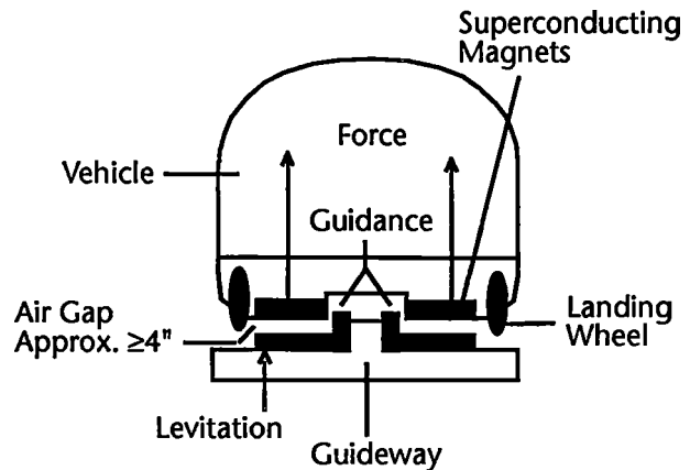
Figure 3. Electrodynamic Maglev
