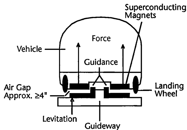
Figure ES-3. Electrodynamic Maglev
