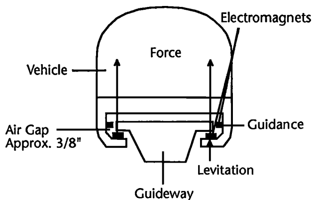
Figure 2. Electromagnetic Maglev
