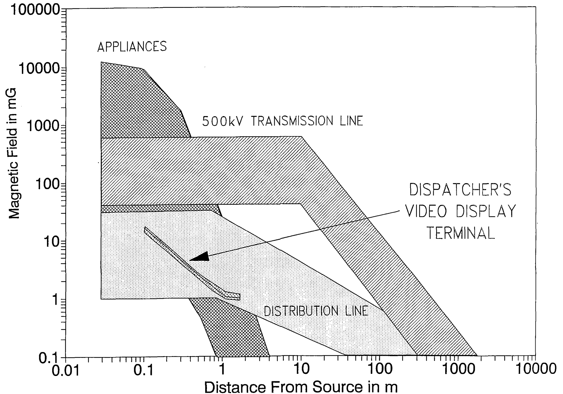
Figure 9-10 The range of total time varying magnetic field levels in front of a dispatcher's video display terminal compared to typical levels of power frequency magnetic fields produced by common sources.
