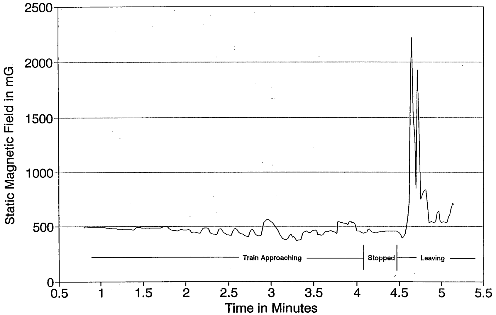
Figure 6-6 Continuous magnetic field recording at the edge of the Grosvenor station platform at the departing end as a train enters, stops, and departs.
