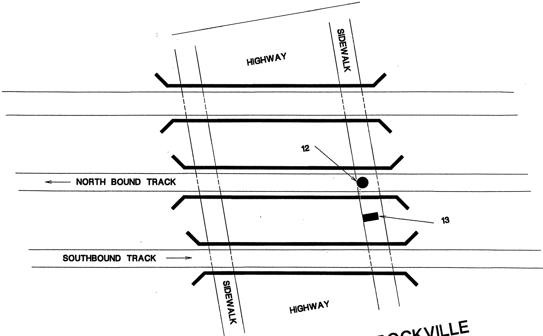
Figure 5-1 Repetitive waveform measurement location at highway underpass at Rockville.
