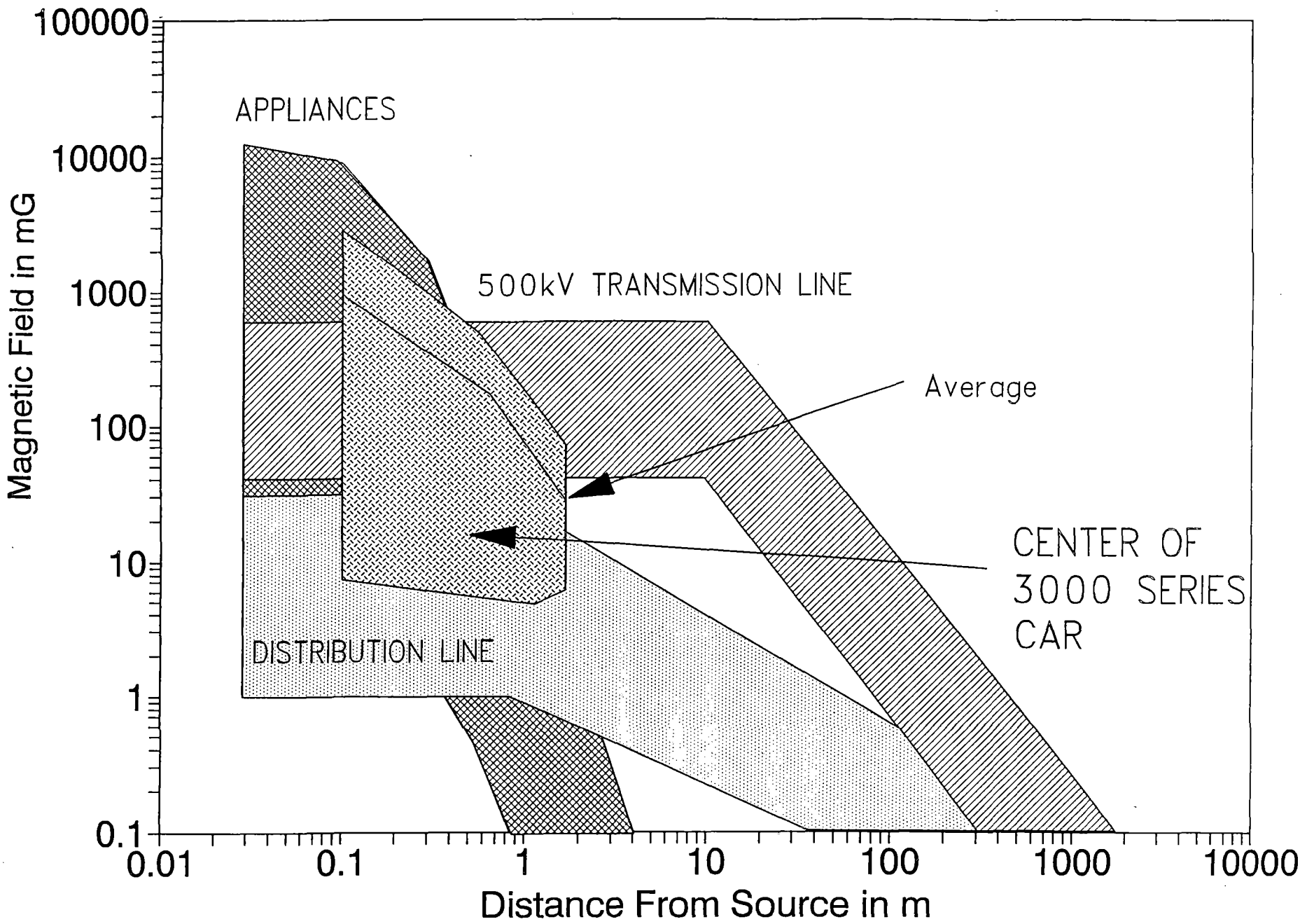
Figure 9-5 The range of total time varying magnetic field levels in the center of the 3000 series Metrorail cars compared to typical levels of power frequency magnetic fields produced by common sources.
