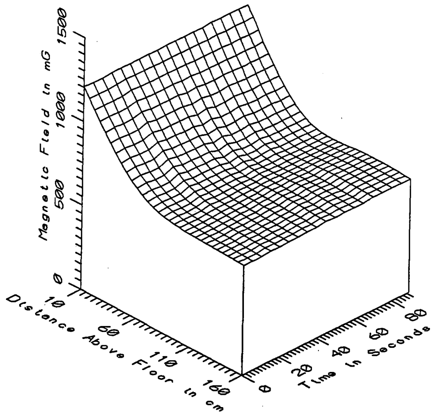
MET046 - SHADY GROVE DISPATCHER'S SEAT - STATIC
