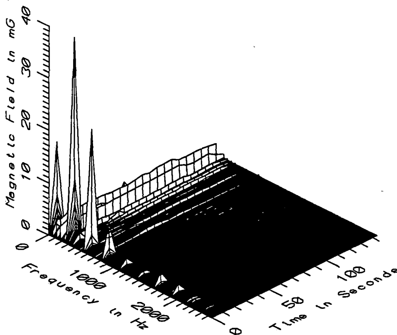
MET017 - 10cm ABOVE PLATFORM AT SAFETY LINE, ARRIVING END
