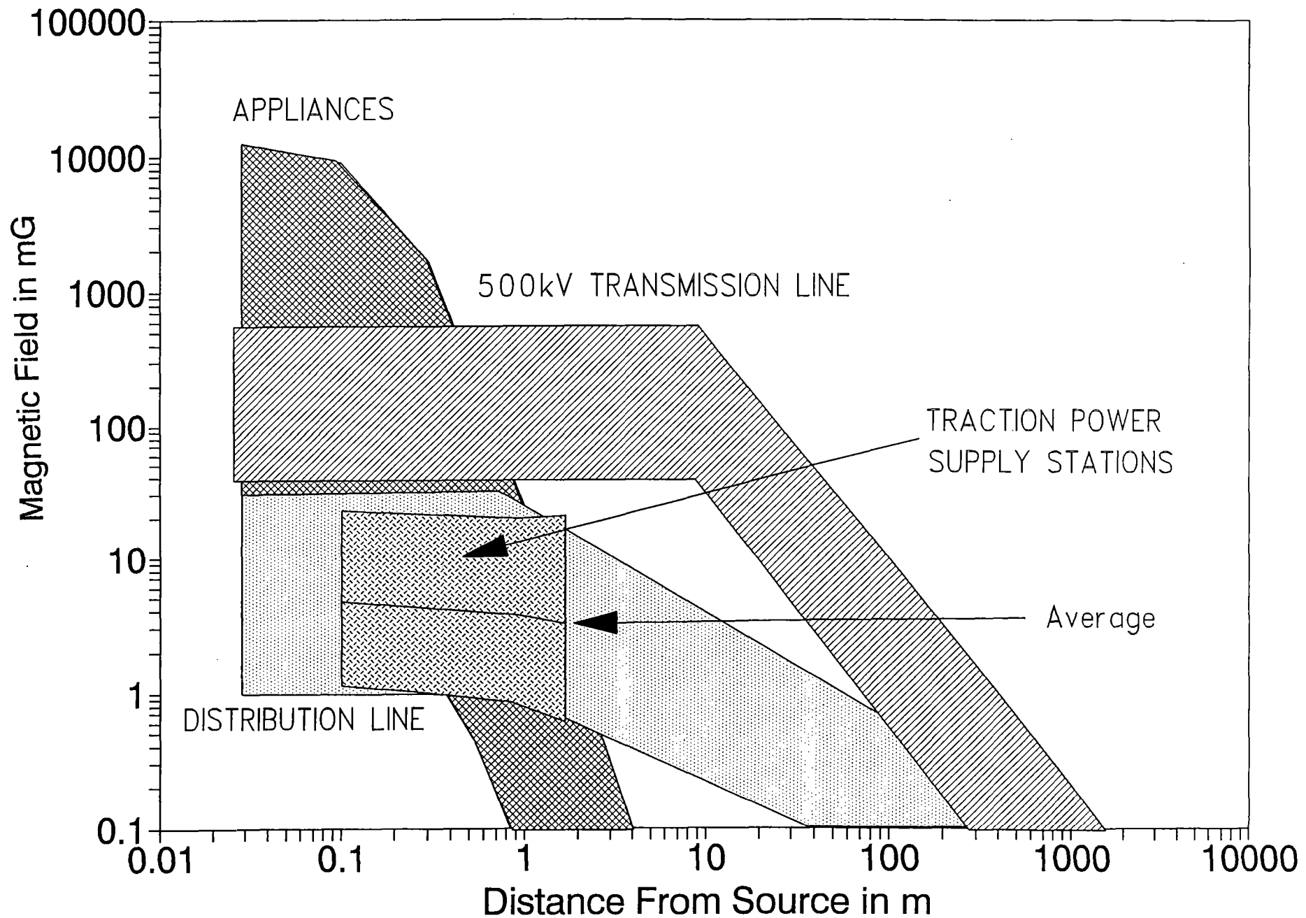
Figure 9-9 The range of total time varying magnetic field levels outside traction power supply stations, at various distances from the fence or wall, compared to typical levels of power frequency magnetic fields produced by common sources.
