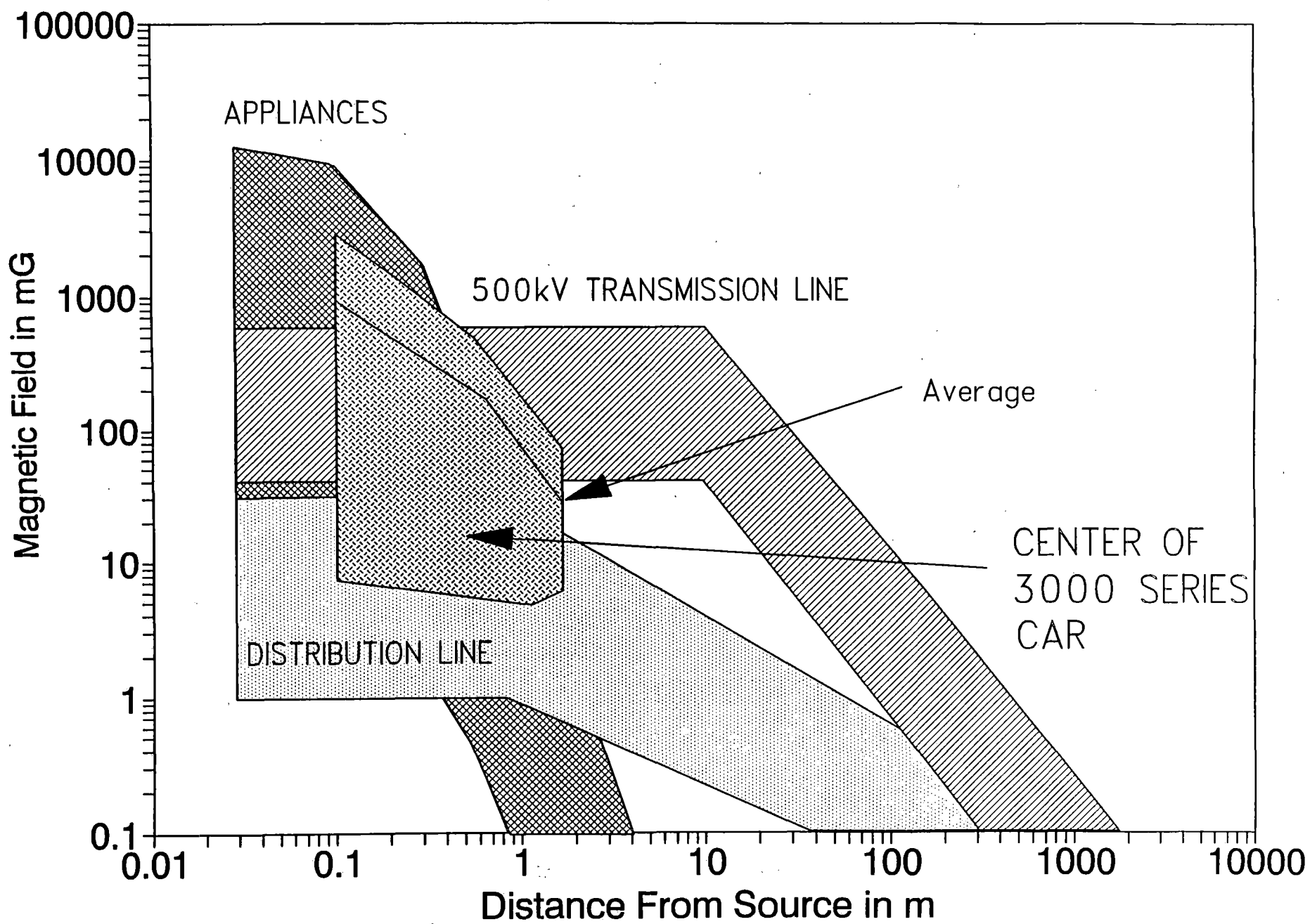
Figure 1-3 The range of total time varying magnetic field levels in the center of the 3000 series Metrorail cars compared to typical levels of power frequency magnetic fields produced by common sources.
