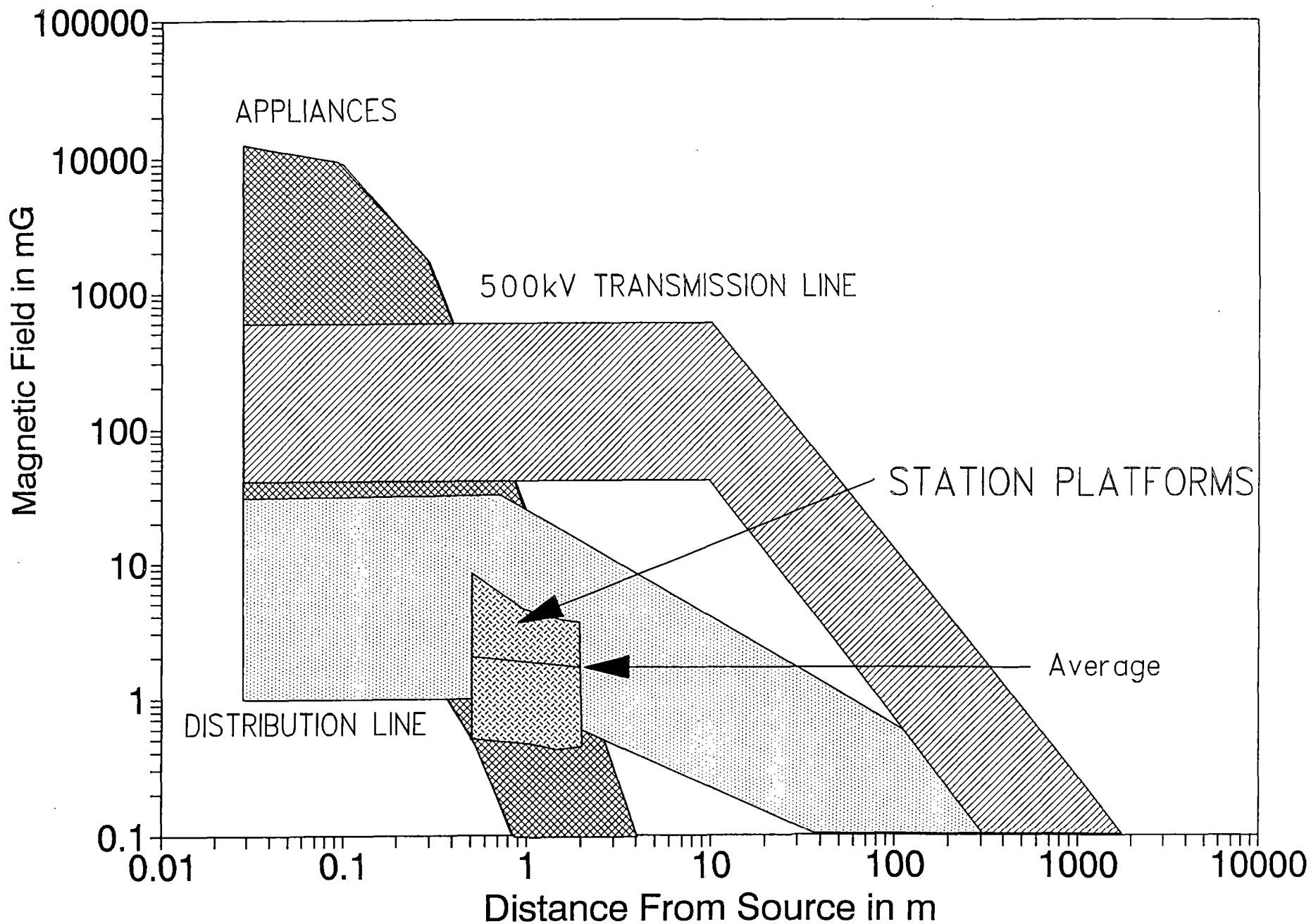
Figure 9-8 The range of total time varying magnetic field levels on the platforms, at various distances from the track, compared to typical levels of power frequency magnetic fields produced by common sources.
