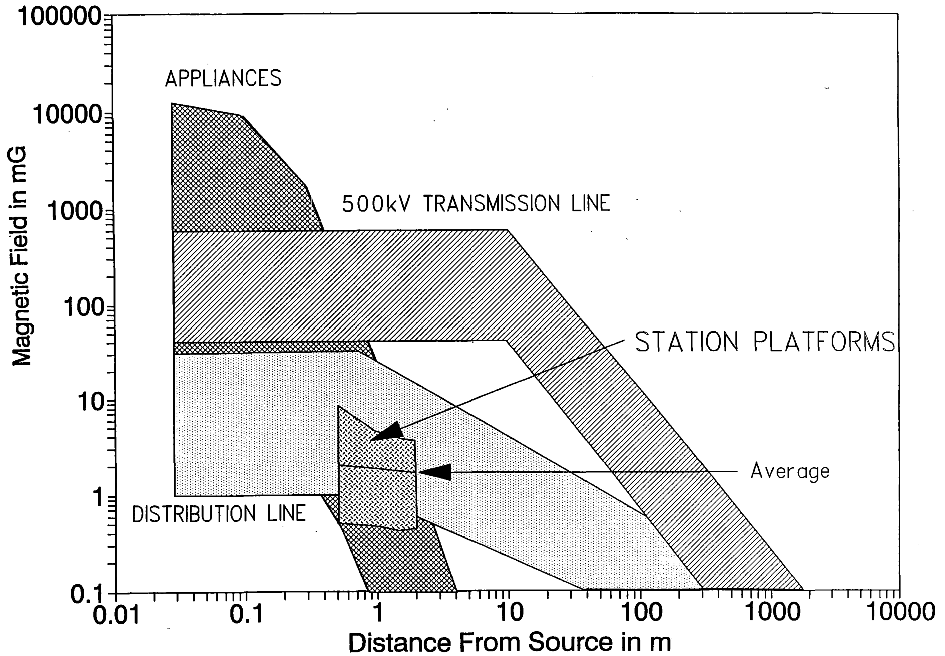
Figure 1-6 The range of total time varying magnetic field levels on the platforms, at various distances from the track, compared to typical levels of power frequency magnetic fields produced by common sources.
