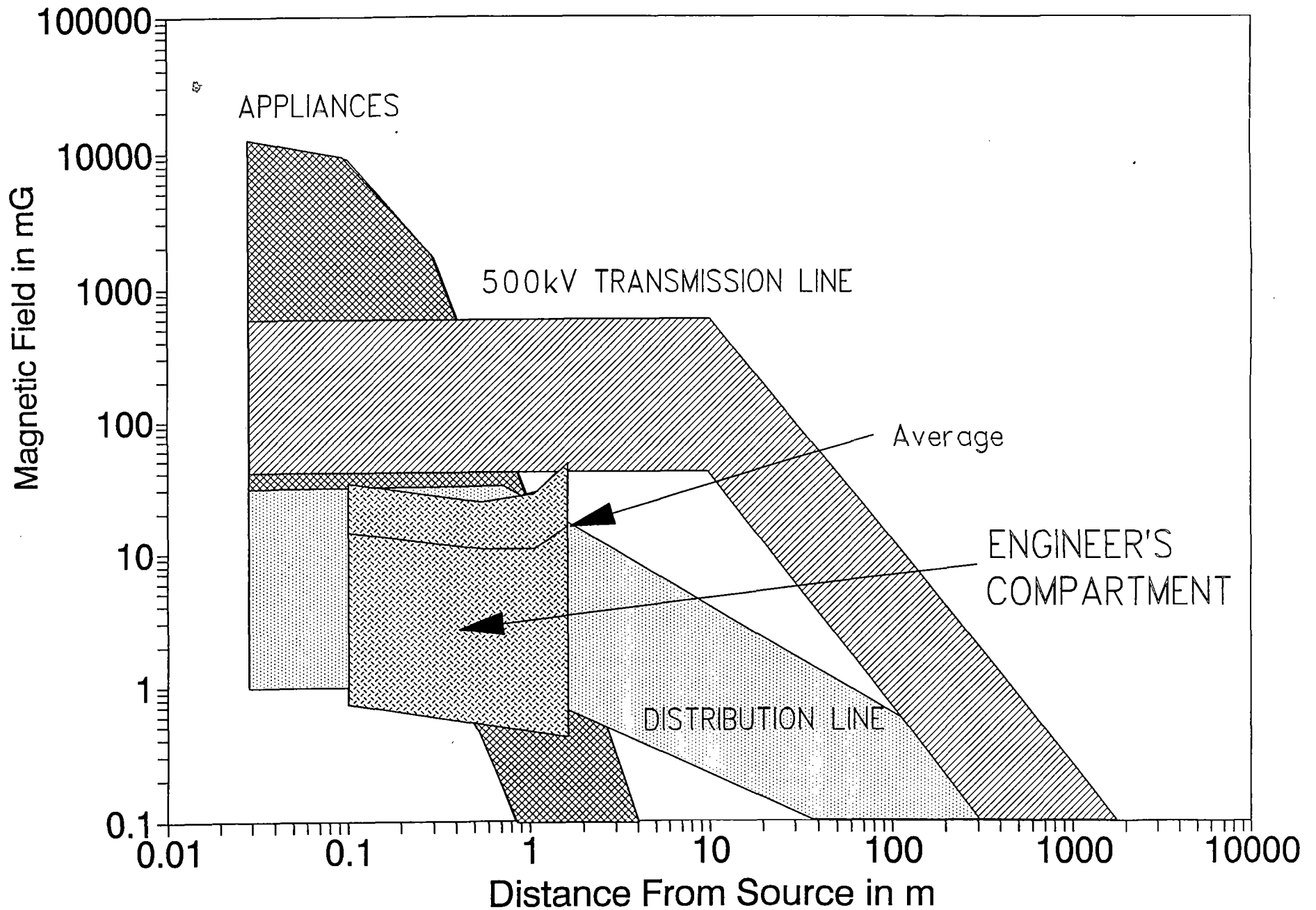
Figure 9-6 The range of total time varying magnetic field levels in the engineer's compartment of the Metrorail cars compared to typical levels of power frequency magnetic fields produced by common sources.
