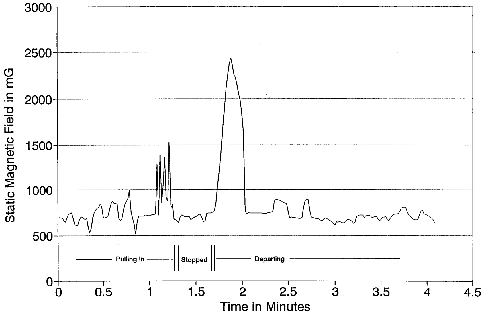
Figure 6-5 Continuous magnetic field recording at the edge of the Grosvenor station platform at the arriving end as a train enters, stops, and departs.
