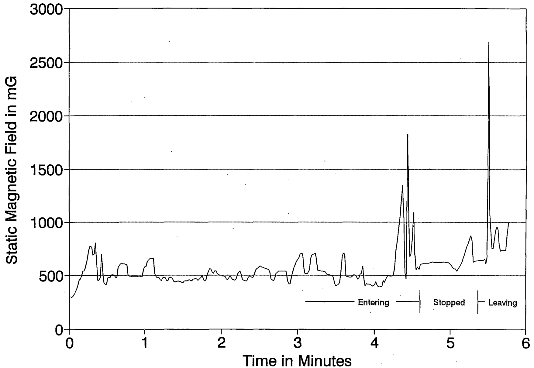
Figure 6-7 Continuous magnetic field recording at the edge of the Grosvenor station platform midway along the platform as a train enters, stops, and departs.
