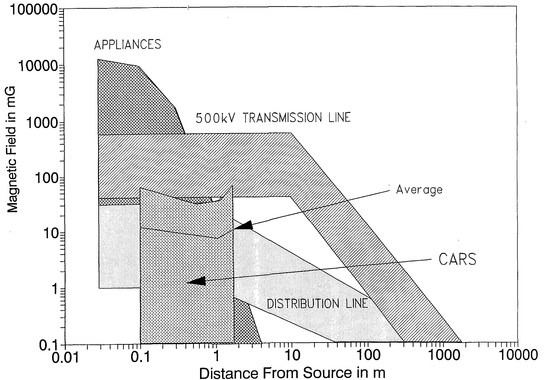
Figure 9-4 The range of total time varying magnetic field levels in the Metrorail cars compared to typical levels of power frequency magnetic fields produced by common sources.
