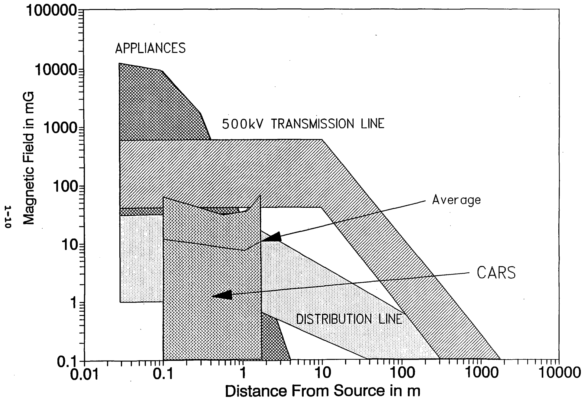
Figure 1-2 The range of total time varying magnetic field levels in the Metrorail cars compared to typical levels of power frequency magnetic fields produced by common sources.
