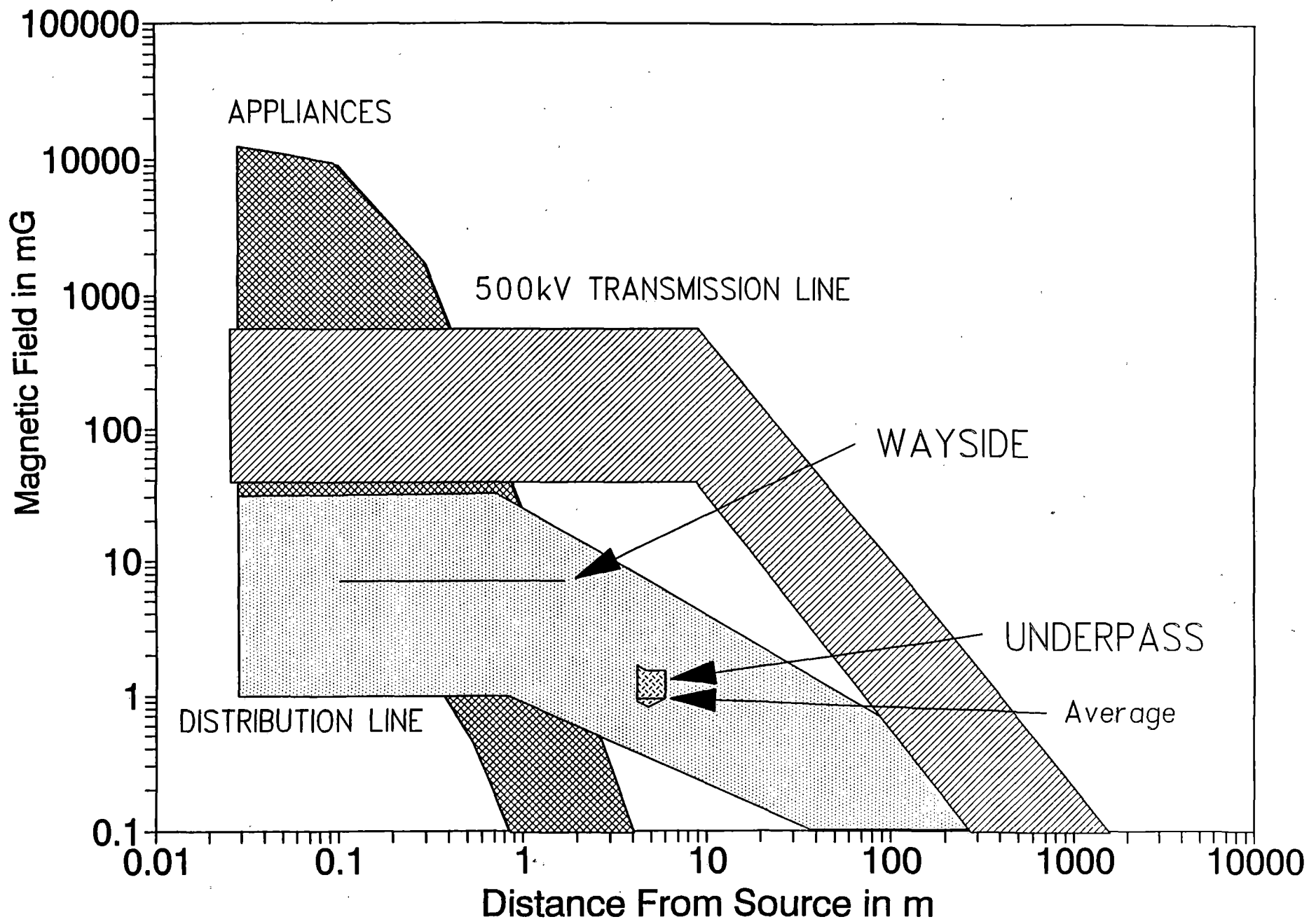
Figure 1-5 The range of total time varying magnetic field levels at a wayside and a highway underpass, at various distances from the nearest fence or track, compared to typical levels of power frequency magnetic fields produced by common sources.
