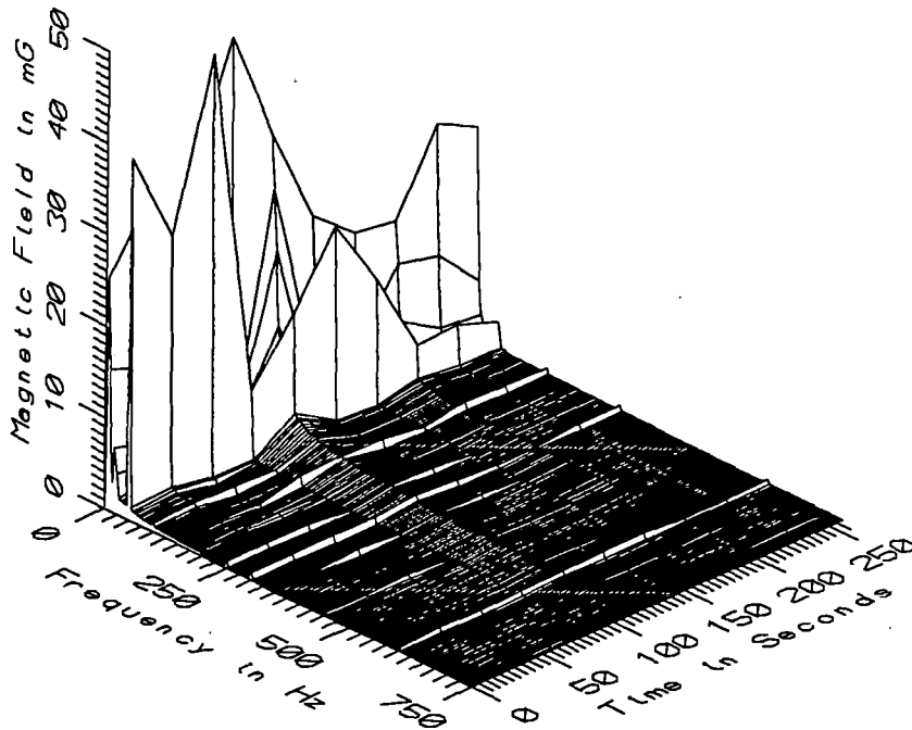
TGV014 - 110cm FROM CENTER LINE BETWEEN SEATS 41 & 42 IN COACH R2B
