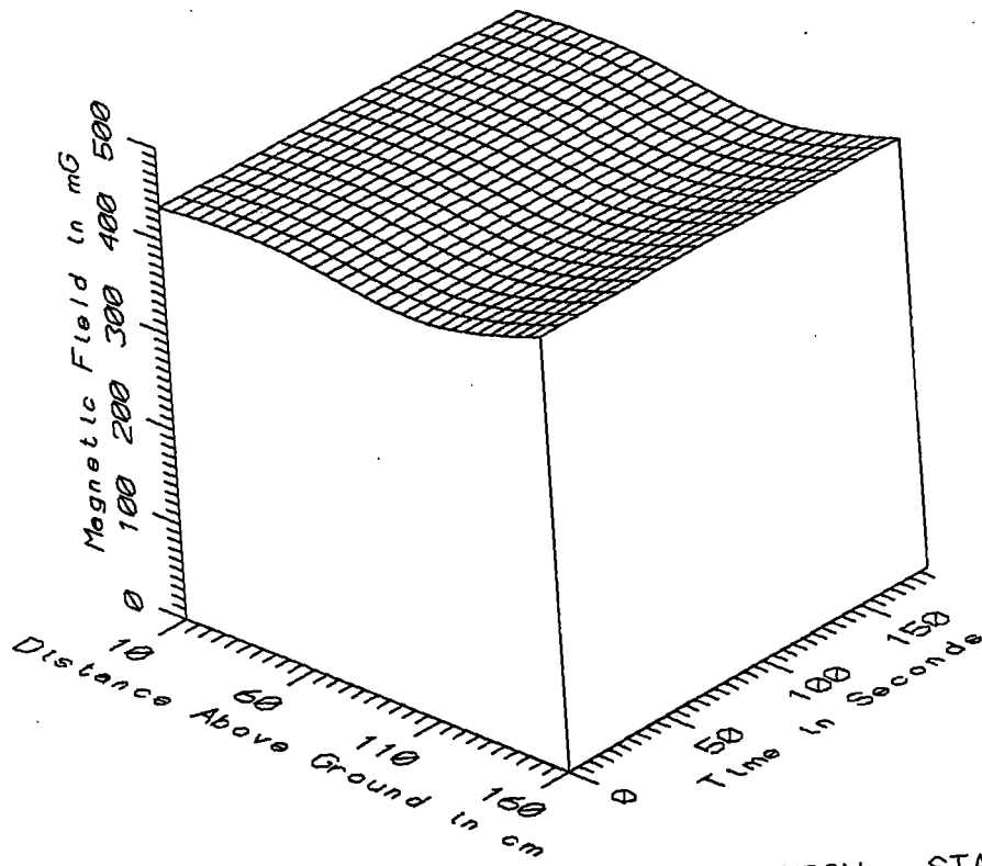
TGV033 - NEAR FENCE OF GAULT ST. DENIS SUBSTATION - STATIC
