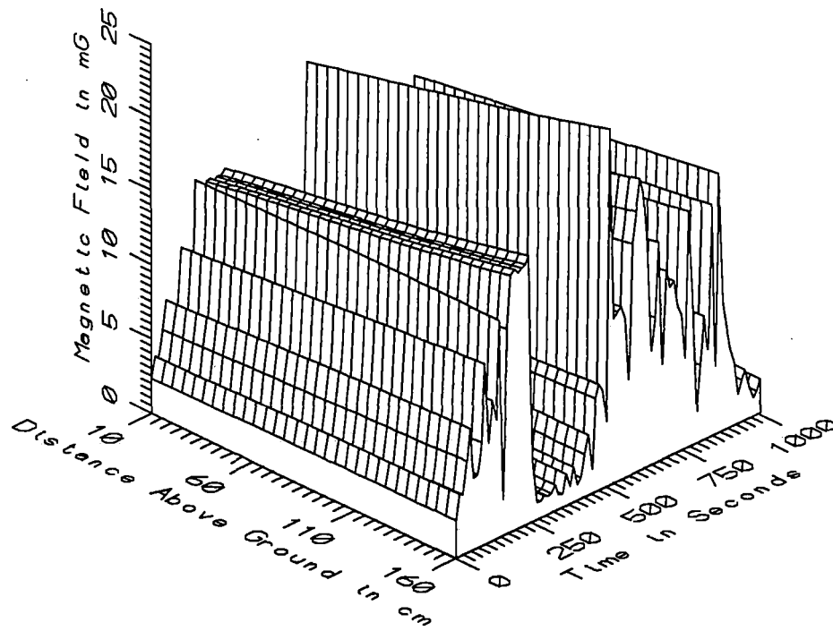
TGV031 - 7.5m FROM PARIS BOUND LINE AT WAYSIDE - POWER FREQ, 50-60Hz
