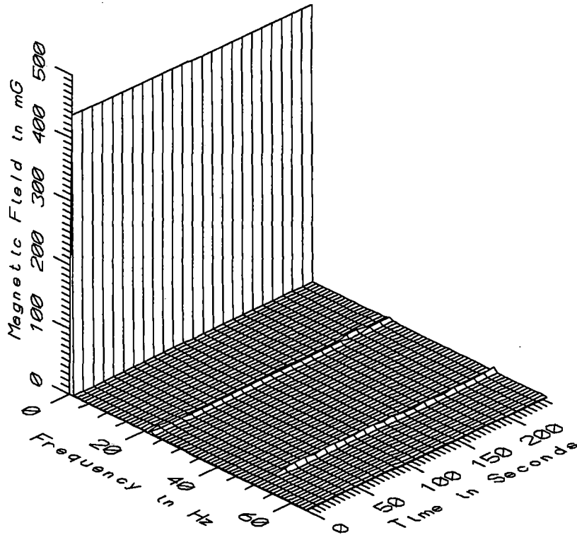
TGV032 - 60cm ABOVE GROUND NEAR FENCE OF GAULT ST. DENIS SUBSTATION
