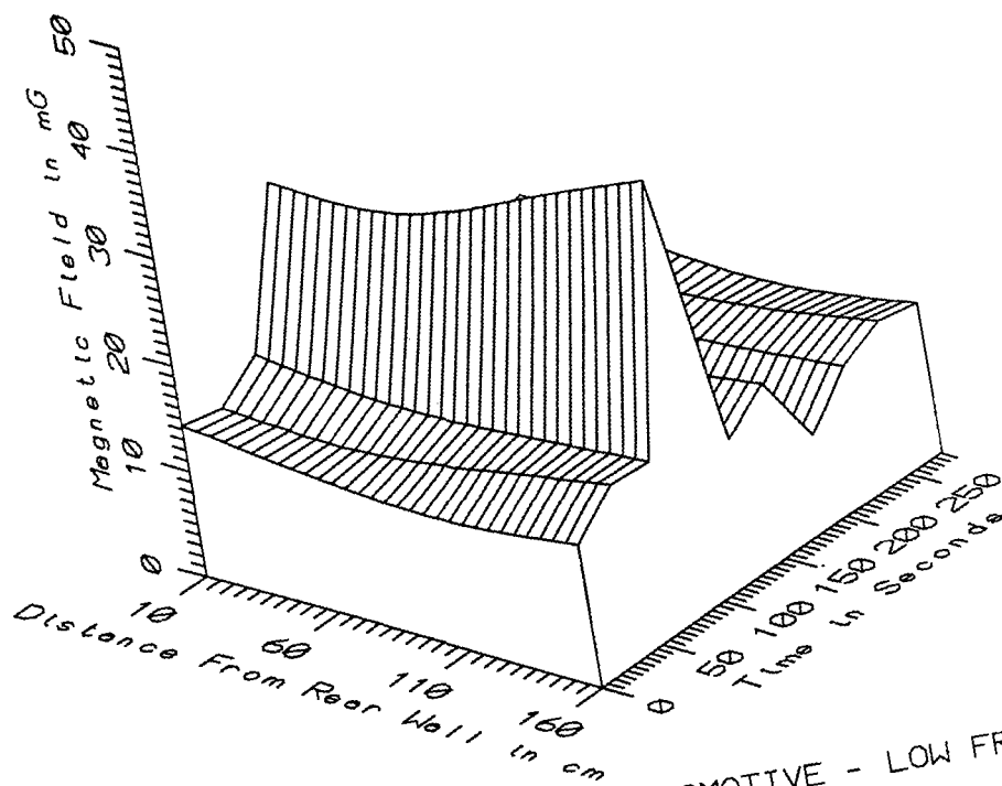
TGV008 - AXIAL PROFILE IN PULL LOCOMOTIVE - STATIC
