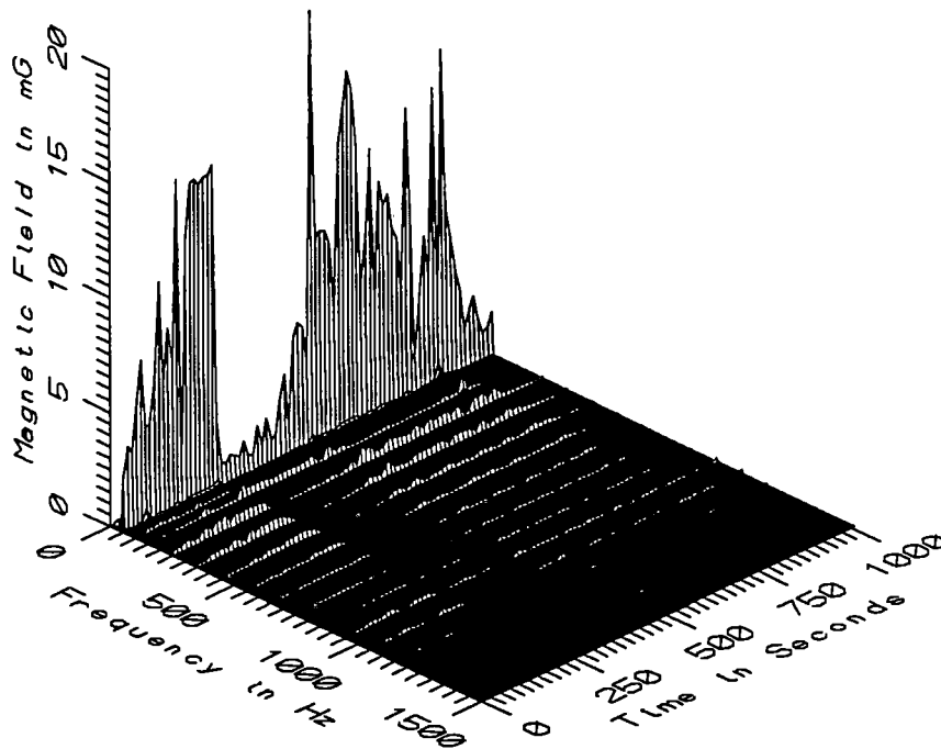
TGV031 - 10cm ABOVE GROUND 7.5m FROM PARIS BOUND LINE AT WAYSIDE
