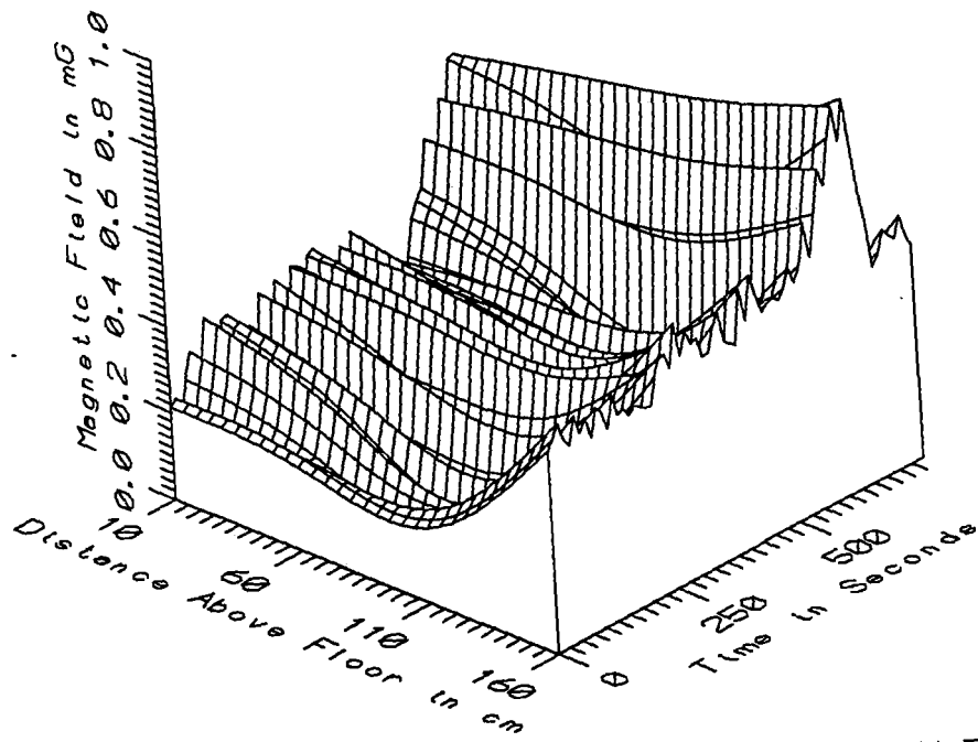
TGV034 - IN CONTROL HOUSE, GAULT ST. DENIS SUB. - LOW FREQ, 5-45Hz
