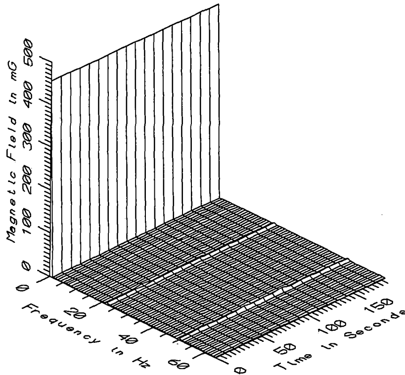
TGV033 - 160cm ABOVE GROUND NEAR FENCE OF GAULT ST. DENIS SUBSTATION
