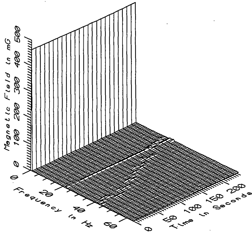
TGV032 - REFERENCE PROBE - 15m BEHIND STAFF, GAULT ST. DENIS SUBSTATION
