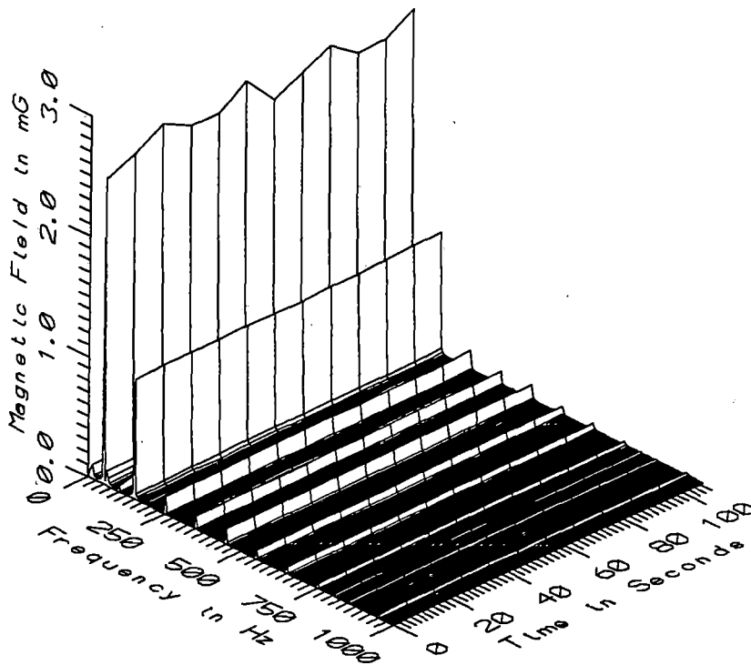
TGV015 - 60cm ABOVE FLOOR NEAR AC SUPPLY CABINET IN VENDOME RELAY ROOM
