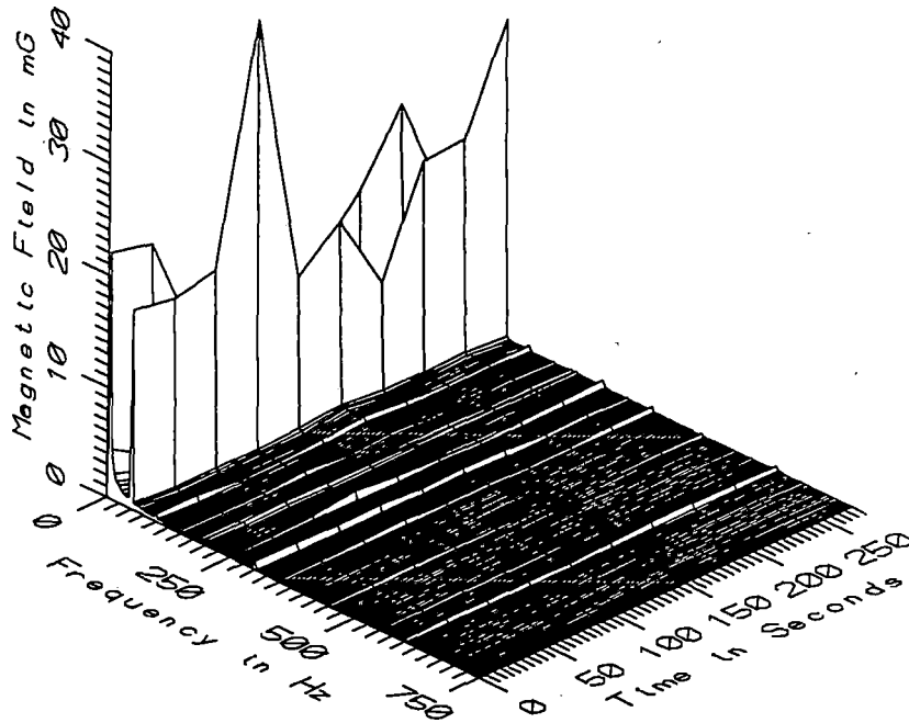
TGV003 - 110cm FROM CENTER OF DOOR AT FRONT OF COACH R1B
