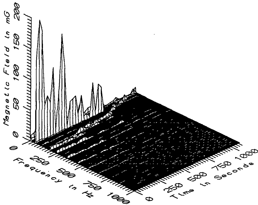
TGV009 - 160cm ABOVE FLOOR AGAINST ENGINEER'S CHAIR, PULL LOCOMOTIVE
