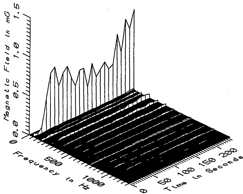
TGV032 - REFERENCE PROBE - 15m BEHIND STAFF, GAULT ST. DENIS SUBSTATION
