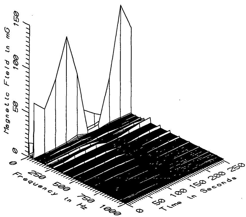
TGV007 - REF. PROBE - ASSISTANT ENGINEER'S CONSOLE, PULL LOCOMOTIVE
