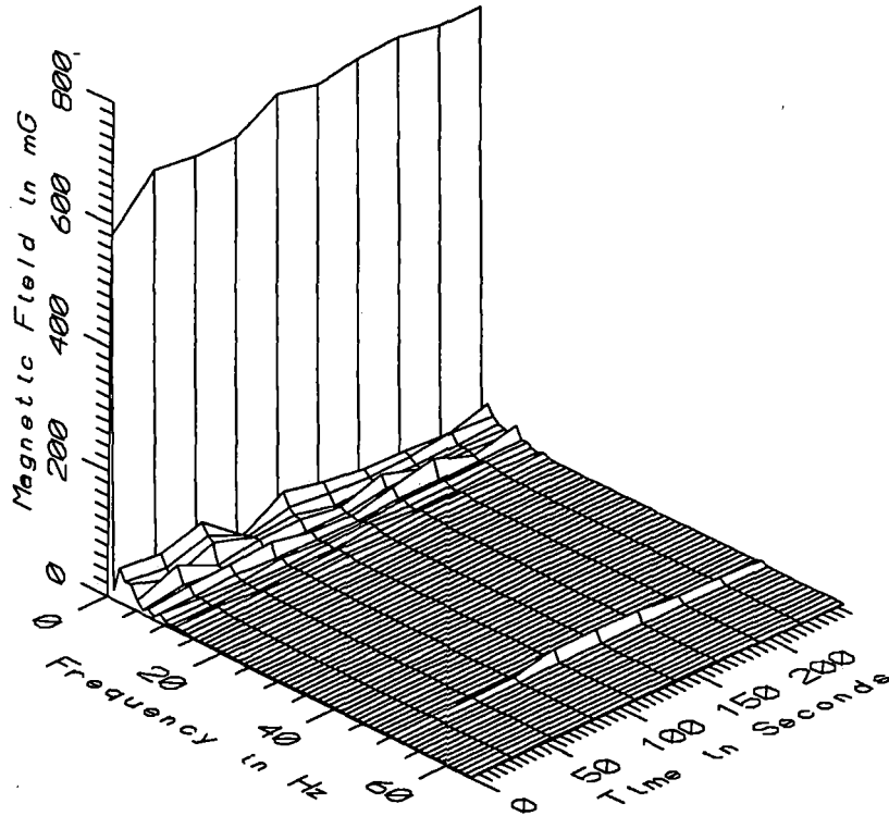
TGV022 - 160cm FROM SIDE WALL ACROSS SEATS 41 & 42 IN COACH R5B
