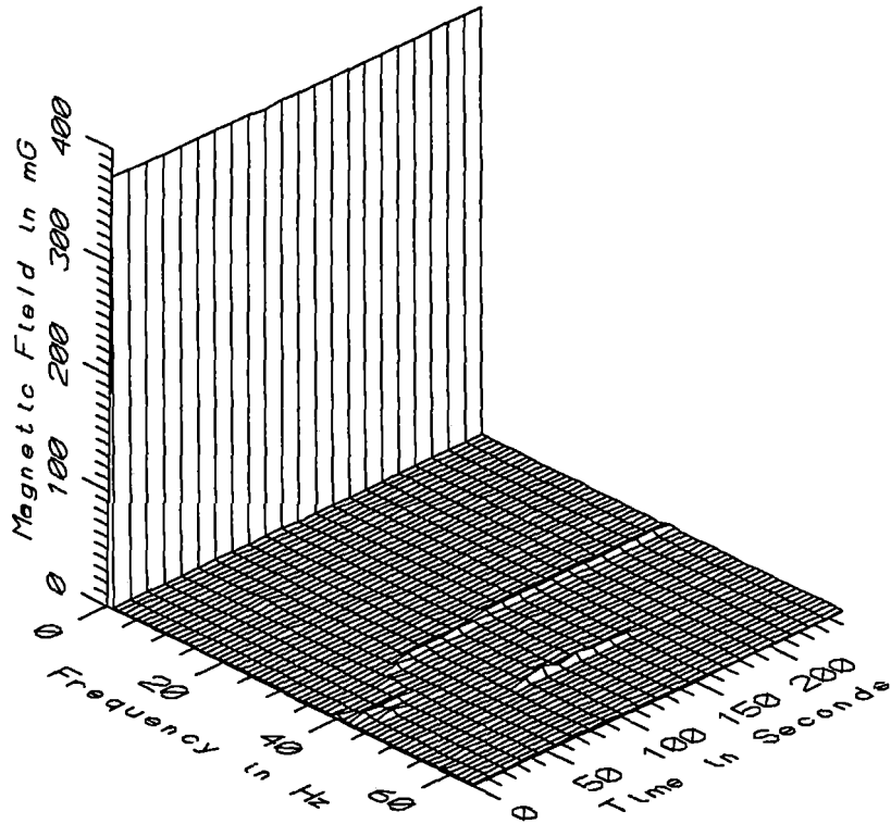
TGV030 - 160cm ABOVE GROUND UNDER TOURS BOUND LINE AT UNDERPASS
