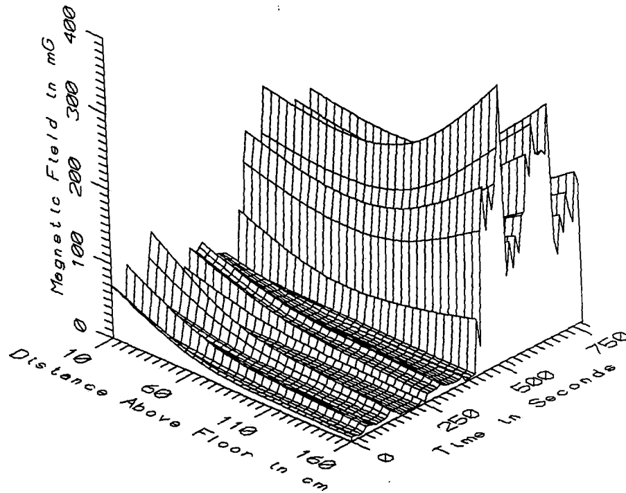
TGV005 - AGAINST ENGINEER'S CHAIR, PULL LOCOMOTIVE - ALL FREQ, 5-2560Hz
