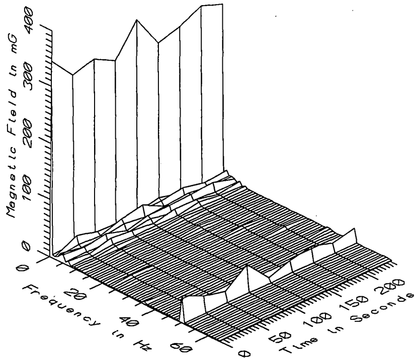
TGV002 - 110cm ABOVE FLOOR IN CENTER OF AISLE AT FRONT OF COACH R1B
