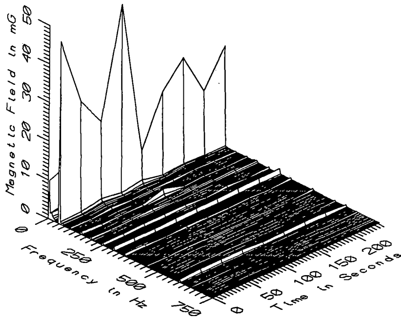
TGV002 - 110cm ABOVE FLOOR IN CENTER OF AISLE AT FRONT OF COACH R1B
