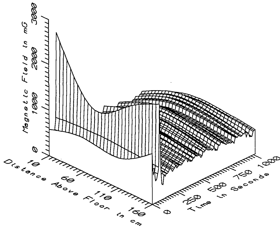
TGVO12 - CENTER OF COACH R2B - STATIC
