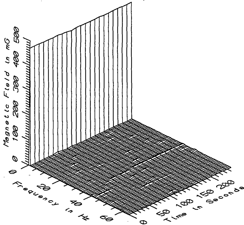
TGV030 - REFERENCE PROBE - ON GROUND 14.5ft FROM STAFF AT UNDERPASS
