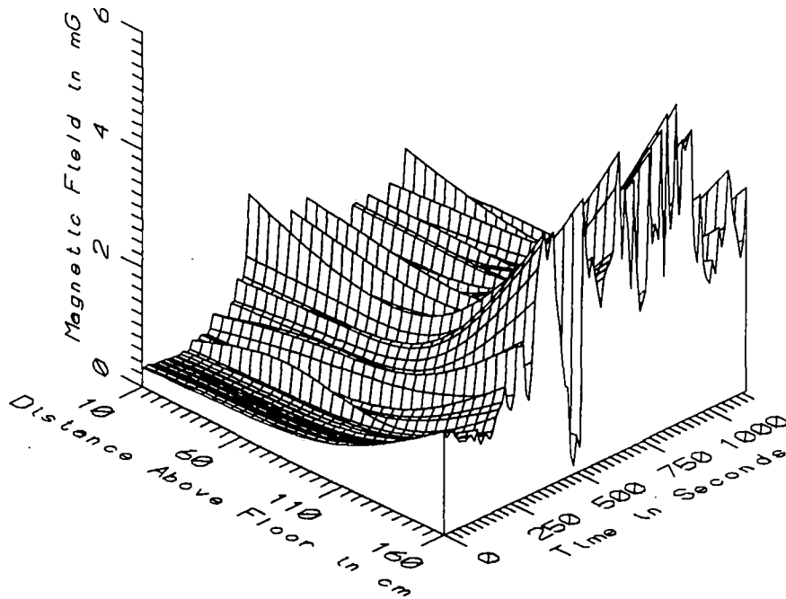
TGV001 - CENTER OF AISLE AT FRONT OF COACH R1B - HIGH FREQ, 305-2560Hz
