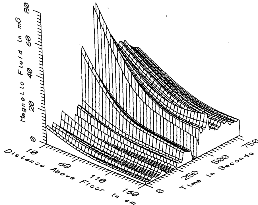
TGV005 - AGAINST ENGINEER'S CHAIR, PULL LOCOMOTIVE - POWER HARM, 65-300Hz
