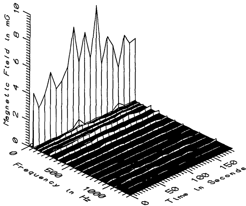
TGV033 - 10cm ABOVE GROUND NEAR FENCE OF GAULT ST. DENIS SUBSTATION
