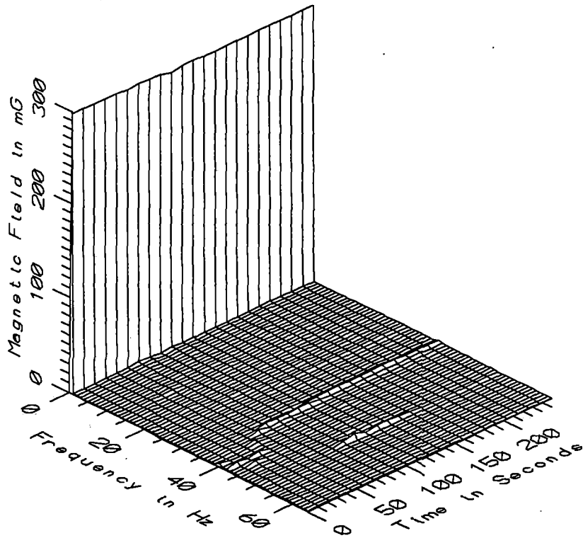
TGV030 - 10cm ABOVE GROUND UNDER TOURS BOUND LINE AT UNDERPASS
