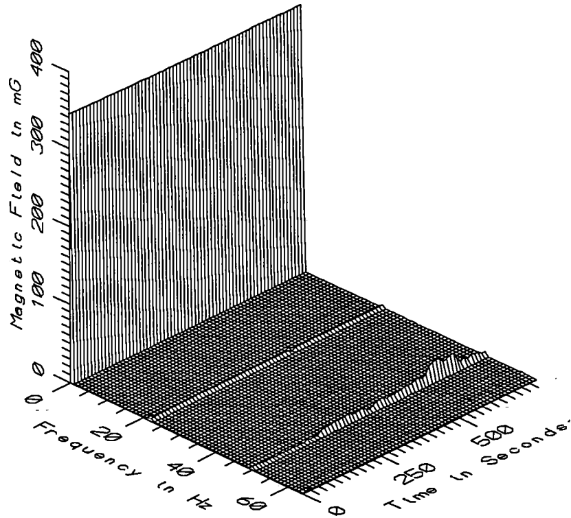
TGV034 - 10cm ABOVE FLOOR IN CONTROL HOUSE, GAULT ST. DENIS SUBSTATION
