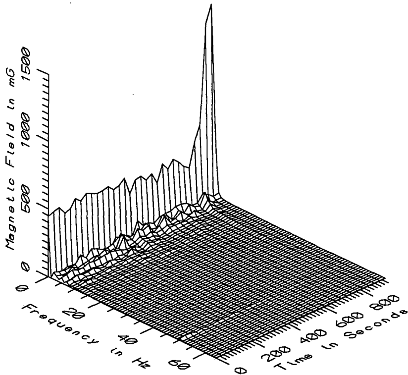
TGV024 - 10cm ABOVE FLOOR NEAR CORNER OF SEAT 47 IN COACH R5B
