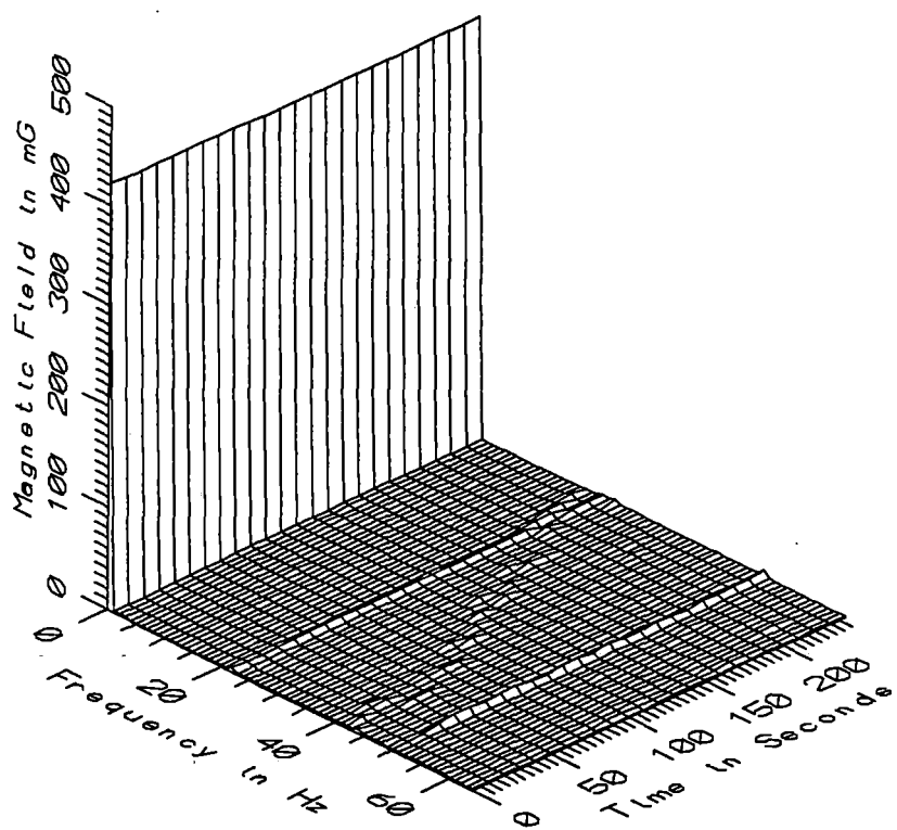
TGV032 - 110cm ABOVE GROUND NEAR FENCE OF GAULT ST. DENIS SUBSTATION
