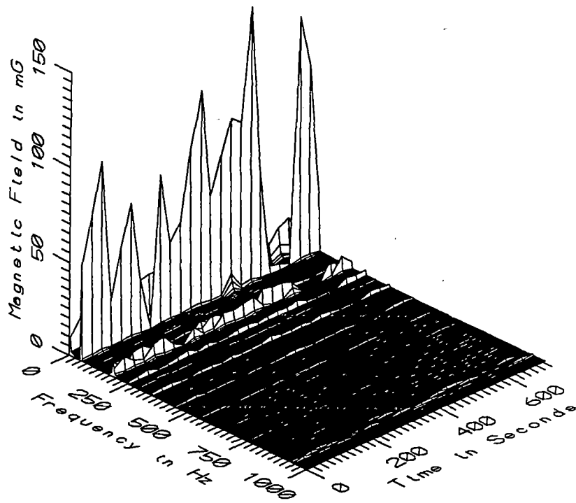
TGV006 - 110cm ABOVE FLOOR AGAINST ENGINEER'S CHAIR, PULL LOCOMOTIVE
