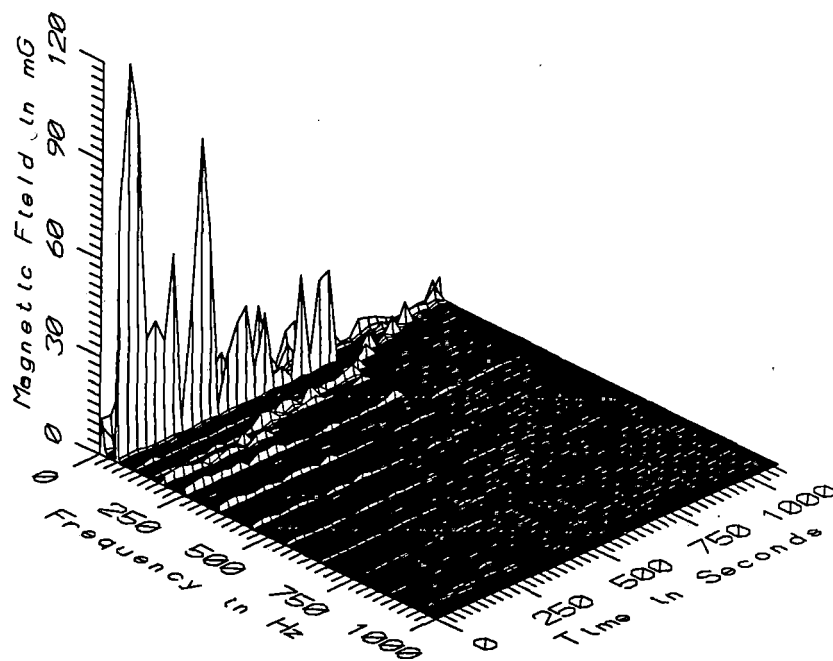
TGV009 - REF. PROBE - ASSISTANT ENGINEER'S CONSOLE, PULL LOCOMOTIVE
