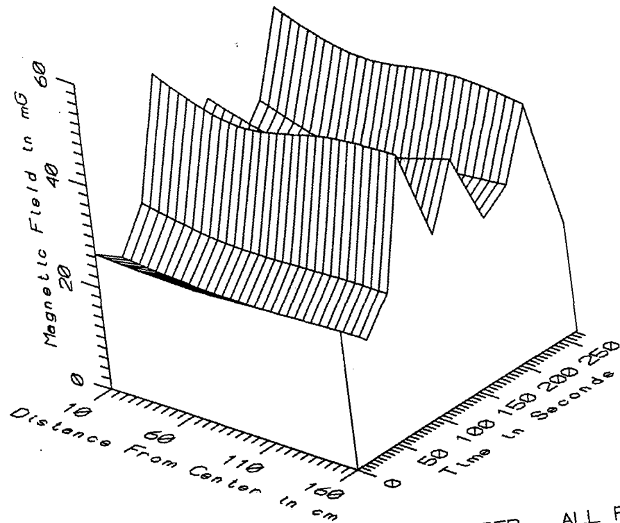
TGV023 - AXIAL PROFILE FROM CENTER OF COACH R5B - HIGH FREQ, 305-2560Hz
