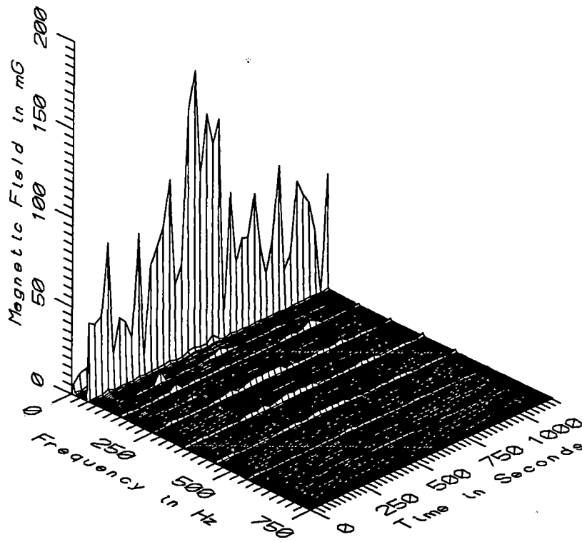
TGV026 - 160cm ABOVE FLOOR AGAINST ENGINEER'S CHAIR, REVENUE TRAIN
