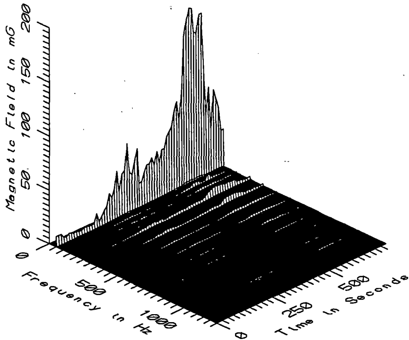
TGV034 - REF. PROBE - OUTSIDE CONTROL HOUSE, GAULT ST. DENIS SUBSTATION
