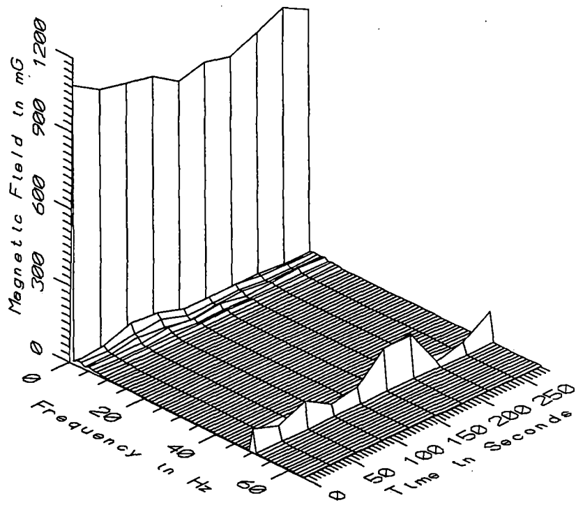
TGV008 - 160cm FROM REAR WALL BETWEEN ENGINEERS' CHAIRS, PULL LOCOMOTIVE
