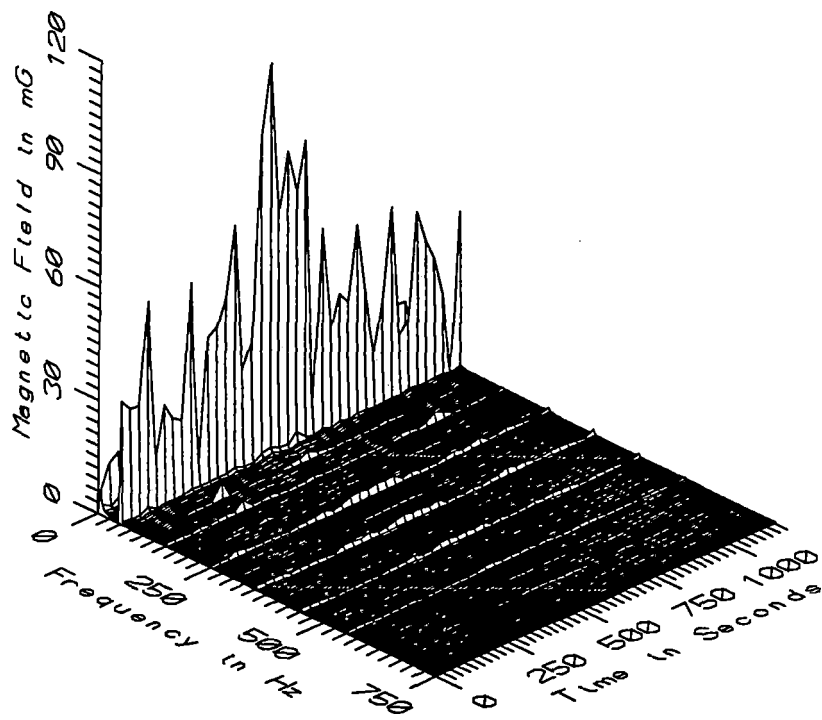
TGV026 - 110cm ABOVE FLOOR AGAINST ENGINEER'S CHAIR, REVENUE TRAIN
