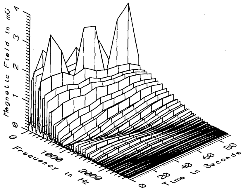
TGV011 - 10cm FROM CENTER OF MONITOR IN TGV CONTROL CENTER
