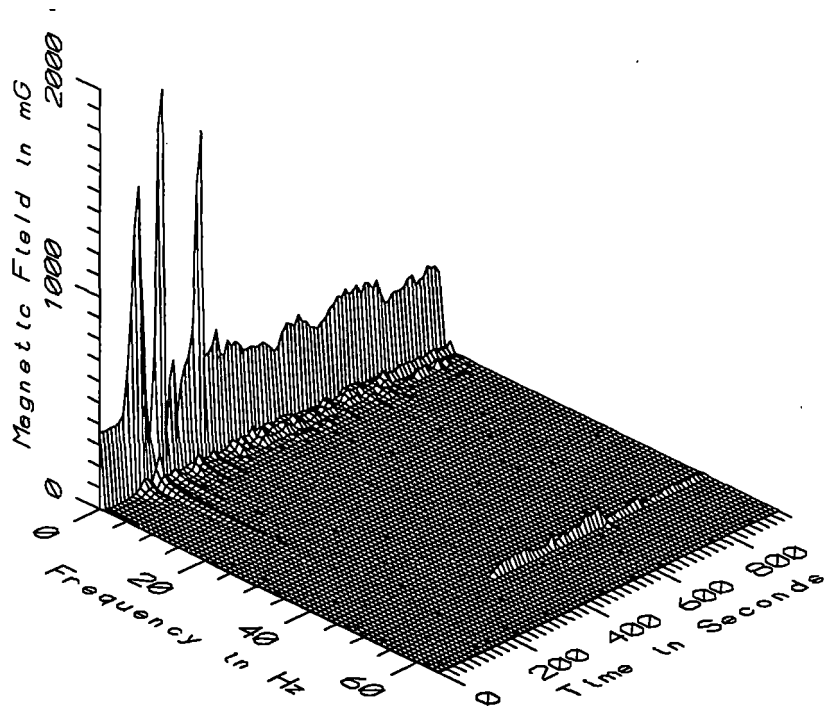
TGV025 - 110cm ABOVE FLOOR AGAINST ENGINEER'S CHAIR, REVENUE TRAIN
