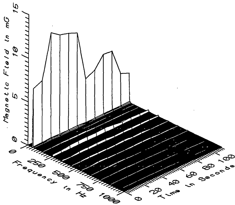
TGV027 - 110cm ABOVE GROUND AT CHAILLOT AUTO-TRANSFORMER, 121km MARKER
