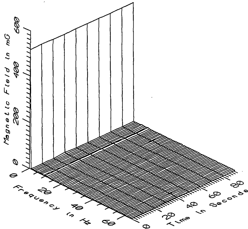
TGV011 - 110cm FROM CENTER OF MONITOR IN TGV CONTROL CENTER
