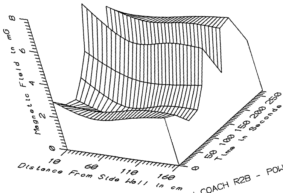
TGV013 - ABOVE SEATS 42 & 43 IN COACH R2B - POWER FREQ. 50-60Hz
