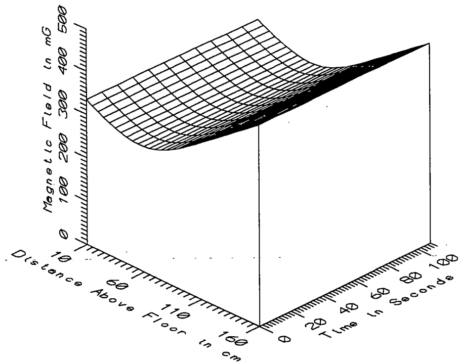
TGV016 - BETWEEN RELAY SHELVES, VENDOME RELAY ROOM - STATIC
