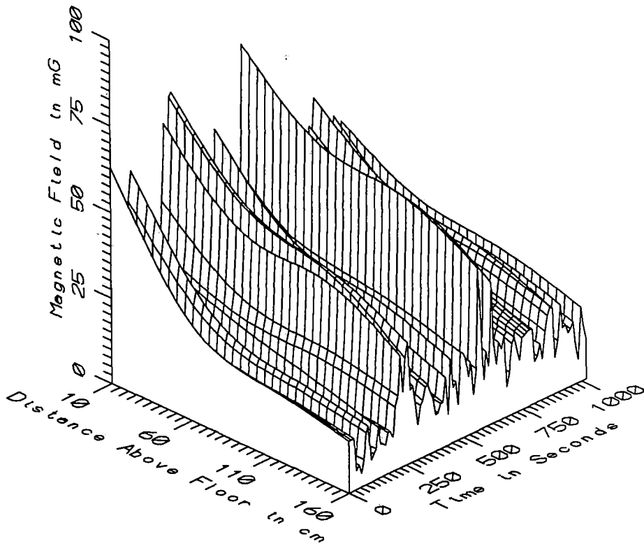
TGVO12 - CENTER OF COACH R2B - LOW FREQ, 5-45Hz
