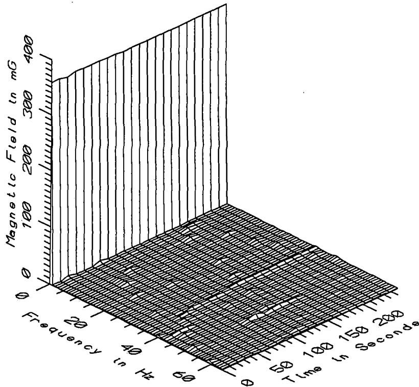
TGV030 - 110cm ABOVE GROUND UNDER TOURS BOUND LINE AT UNDERPASS
