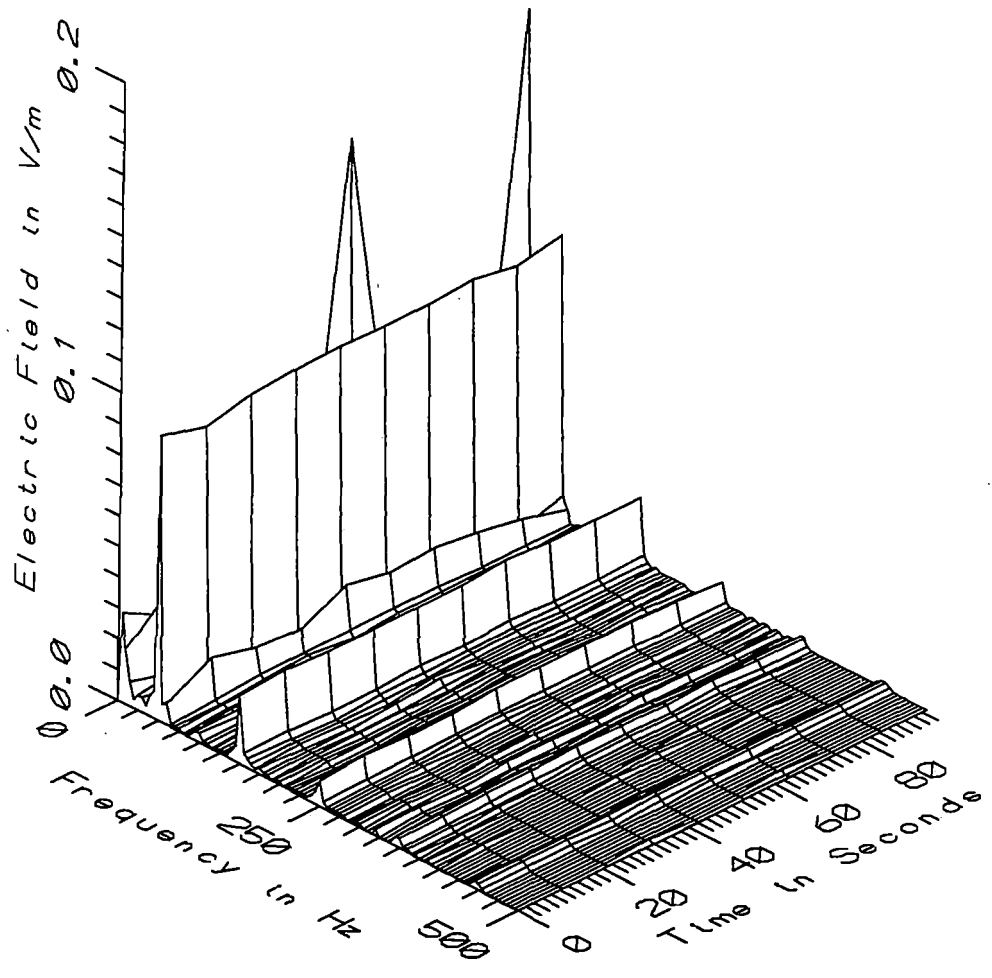
TGV010 - ELECTRIC FIELD IN TGV CONTROL CENTER
