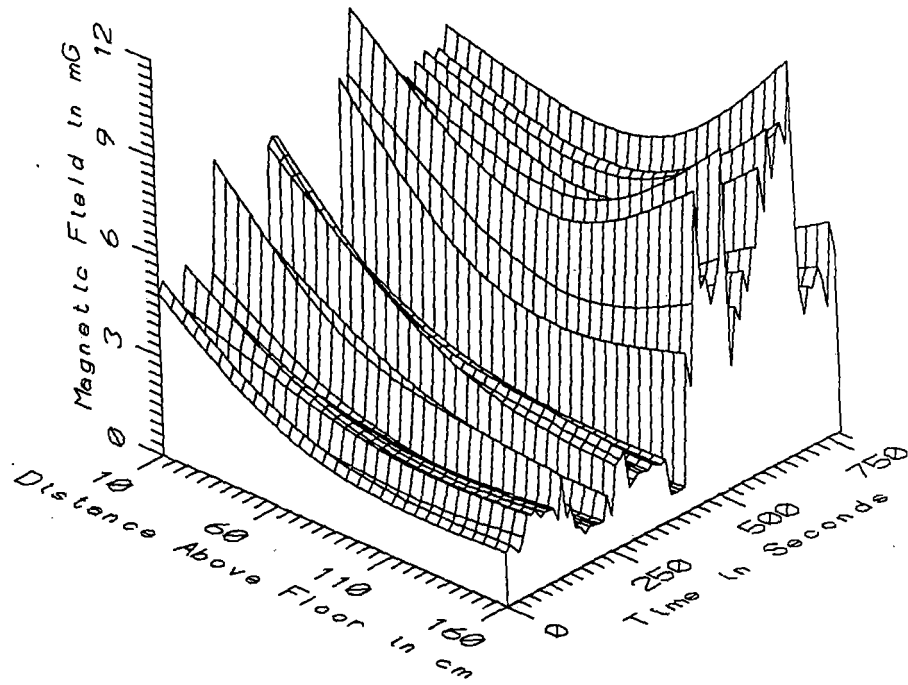
TGV005 - AGAINST ENGINEER'S CHAIR, PULL LOCOMOTIVE - HIGH FREQ, 305-2560Hz
