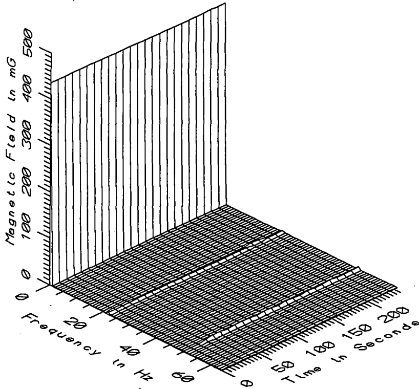
TGV032 - 10cm ABOVE GROUND NEAR FENCE OF GAULT ST. DENIS SUBSTATION
