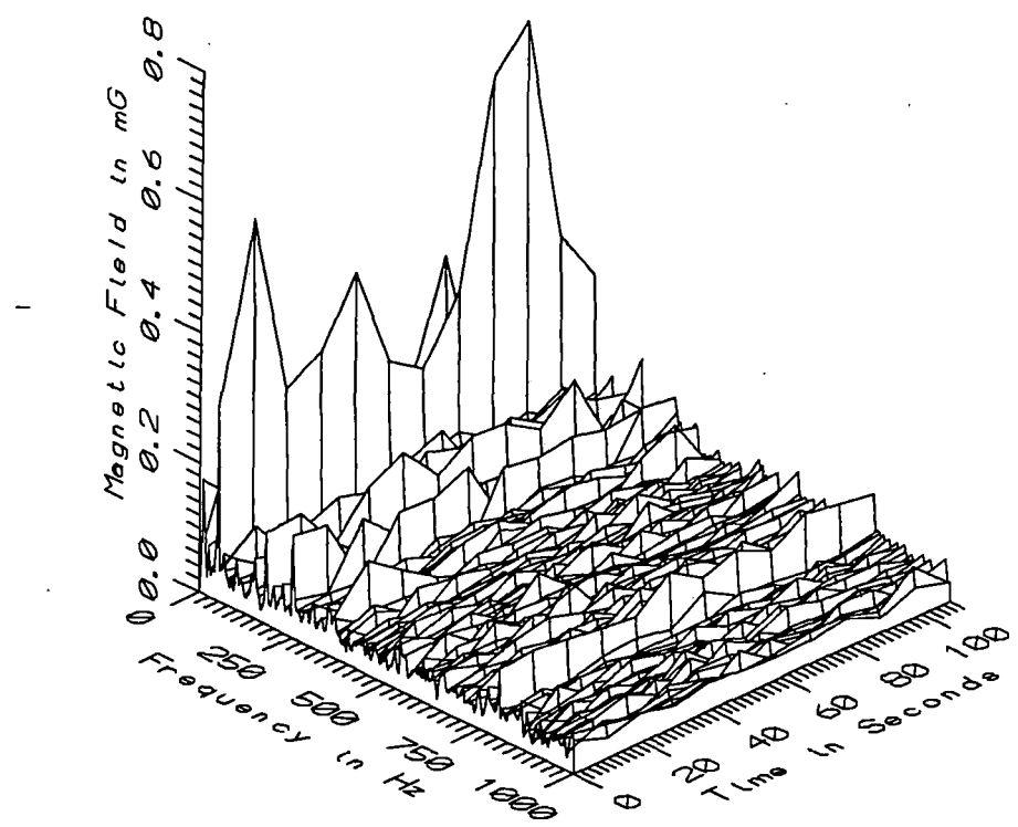
TGV016 - 10cm ABOVE FLOOR BETWEEN RELAY SHELVES, VENDOME RELAY ROOM
