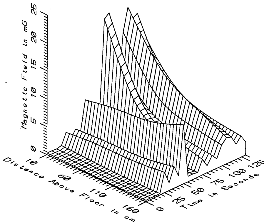
TGV020 - NEAR CORNER OF SEAT 47 IN COACH R5B - LOW FREQ, 5-45Hz
