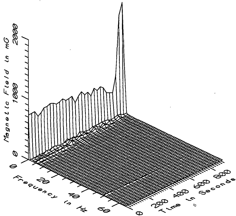
TGV024 - 110cm ABOVE FLOOR NEAR CORNER OF SEAT 47 IN COACH R5B
