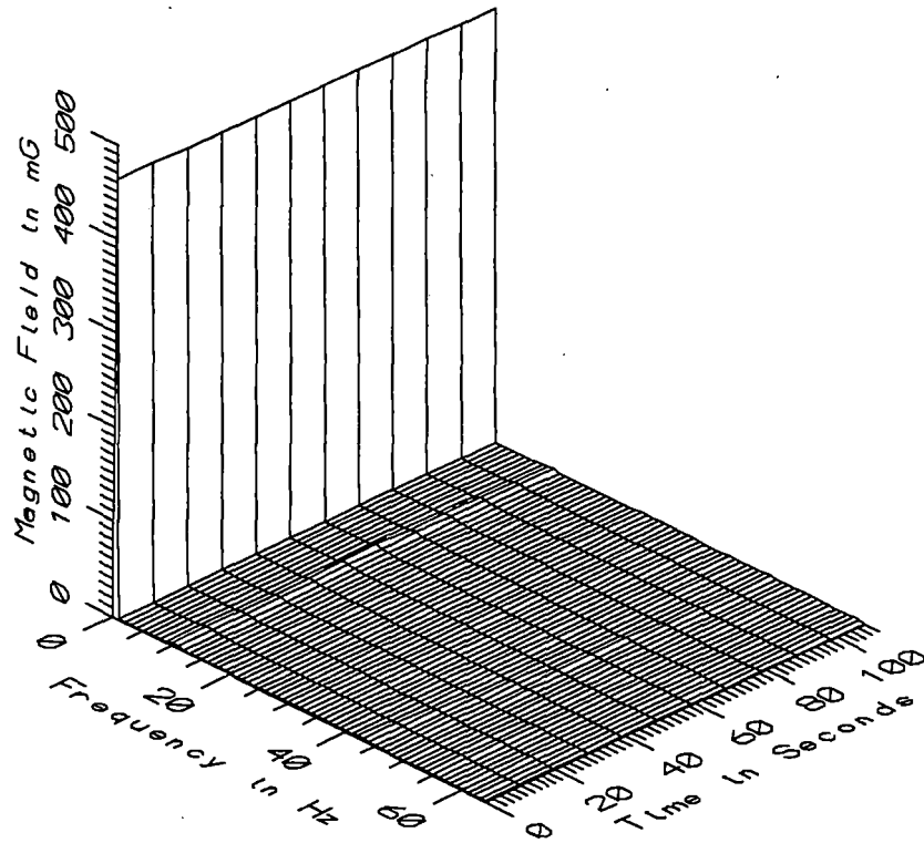
TGV016 - 160cm ABOVE FLOOR BETWEEN RELAY SHELVES, VENDOME RELAY ROOM
