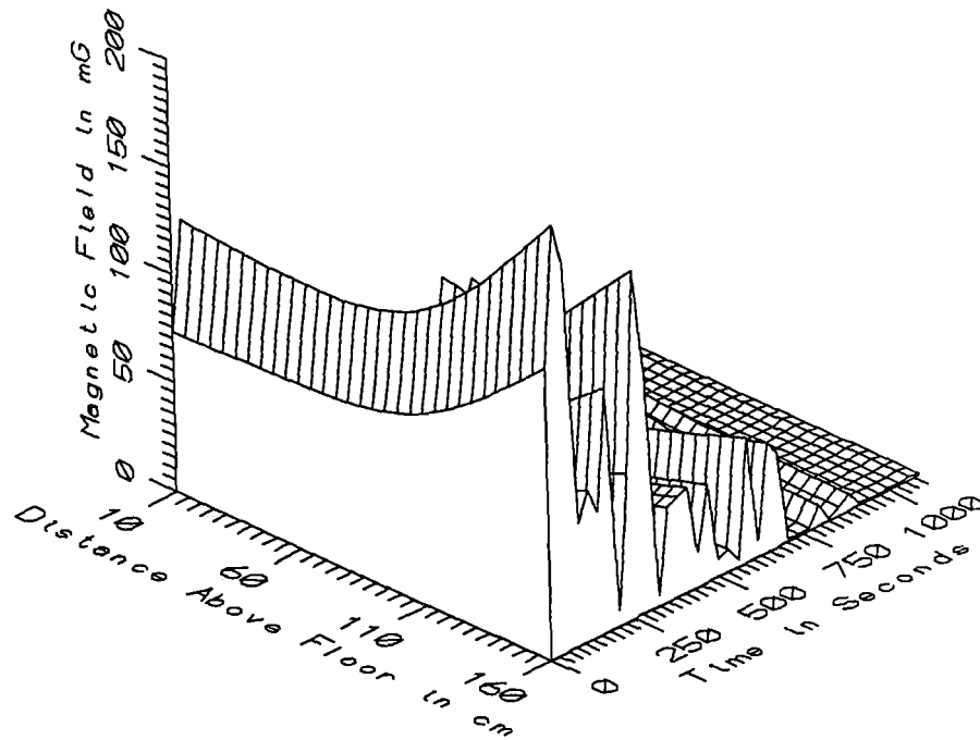
TGV009 - AGAINST ENGINEER'S CHAIR, PULL LOCOMOTIVE - POWER FREQ, 50-60Hz
