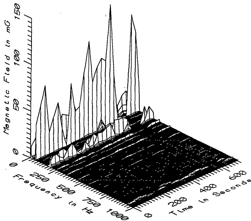
TGV006 - 60cm ABOVE FLOOR AGAINST ENGINEER'S CHAIR, PULL LOCOMOTIVE
