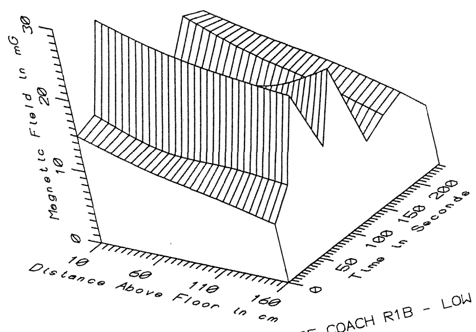
TGV002 - CENTER OF AISLE AT FRONT OF COACH R1B - STATIC
