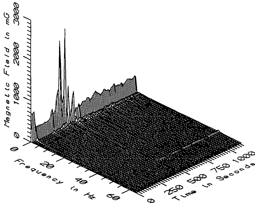
TGV001 - 60cm ABOVE FLOOR IN CENTER OF AISLE AT FRONT OF COACH R1B
