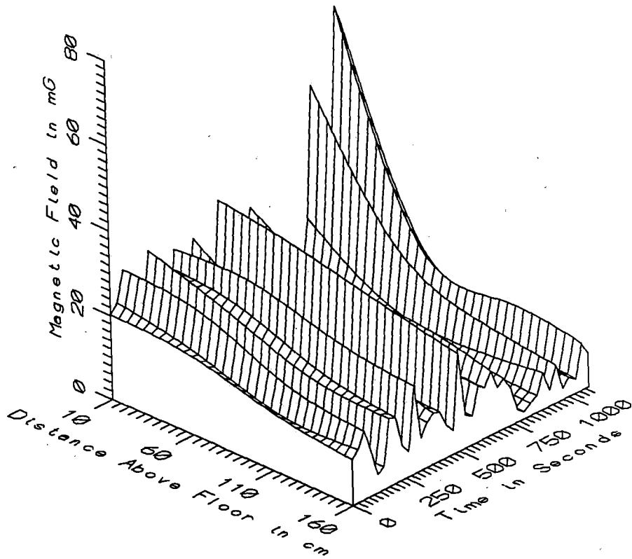
TGV009 - AGAINST ENGINEER'S CHAIR, PULL LOCOMOTIVE - LOW FREQ, 5-45Hz
