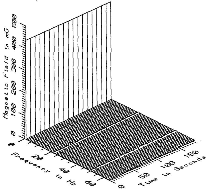
TGV033 - 10cm ABOVE GROUND NEAR FENCE OF GAULT ST. DENIS SUBSTATION
