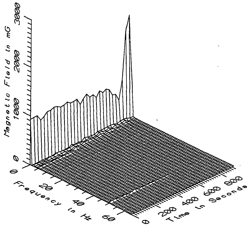
TGV024 - 160cm ABOVE FLOOR NEAR CORNER OF SEAT 47 IN COACH R5B
