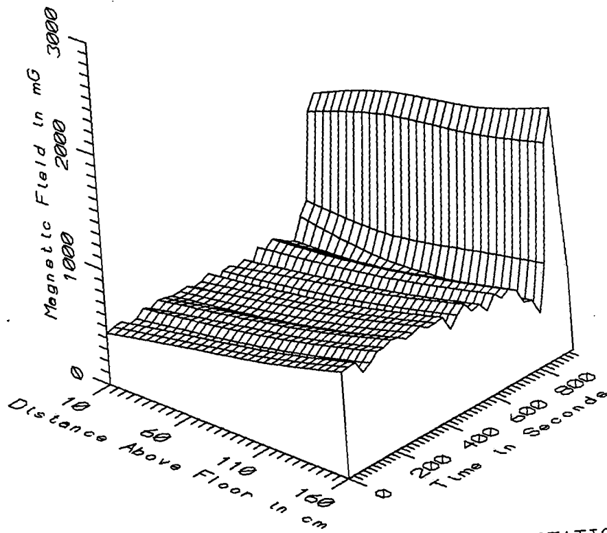
TGV024 - NEAR CORNER OF SEAT 47 IN COACH R5B - STATIC
