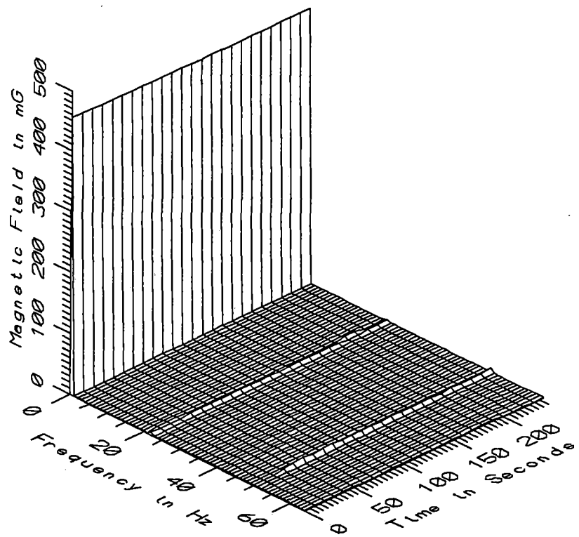
TGV032 - 160cm ABOVE GROUND NEAR FENCE OF GAULT ST. DENIS SUBSTATION
