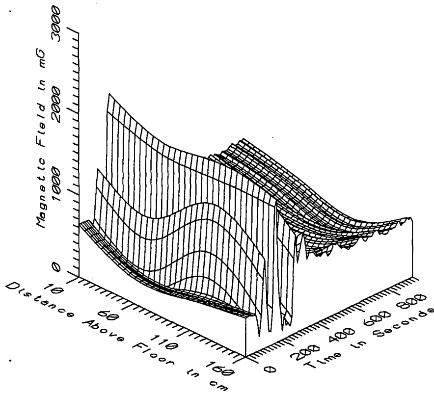
TGV025 - AGAINST ENGINEER'S CHAIR, REVENUE TRAIN - STATIC
