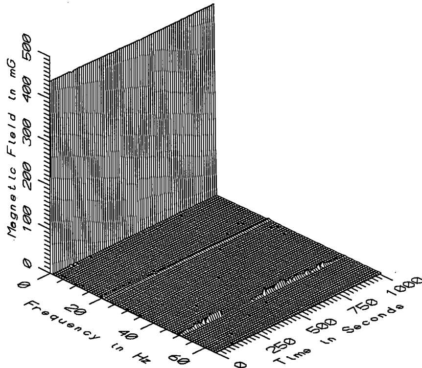
TGV031 - 10cm ABOVE GROUND 7.5m FROM PARIS BOUND LINE AT WAYSIDE
