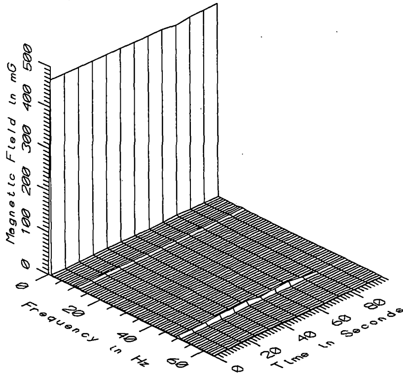
TGV017 - 60cm ABOVE FLOOR AT EDGE OF PLATFORM, VENDOME STATION
