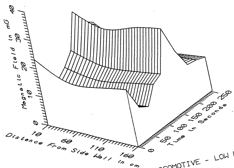
TGV007 - TRANSVERSE PROFILE IN PULL LOCOMOTIVE - STATIC
