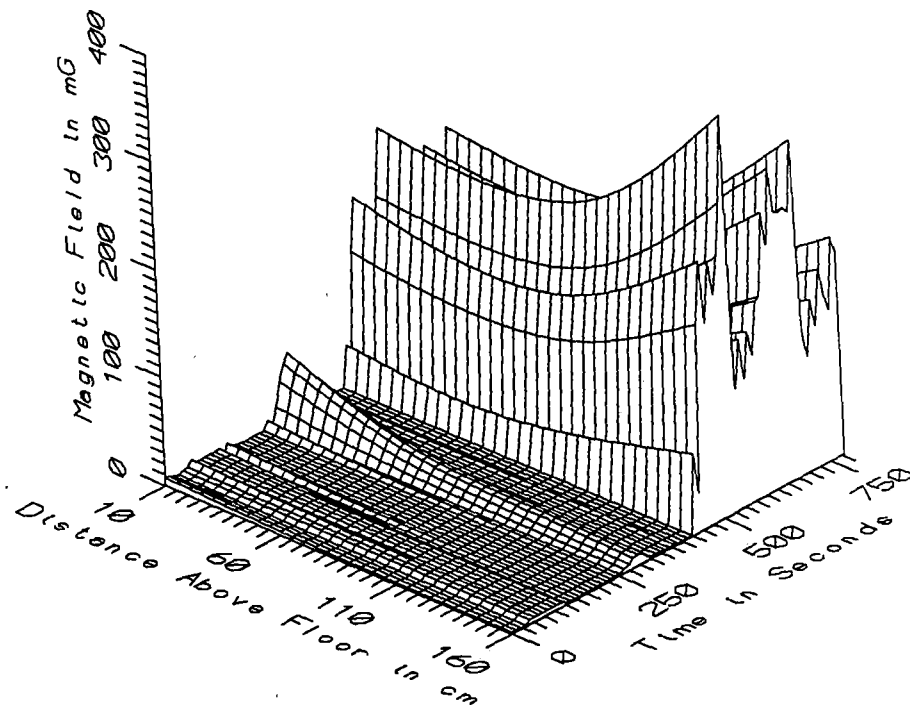
TGV005 - AGAINST ENGINEER'S CHAIR, PULL LOCOMOTIVE - POWER FREQ, 50-60Hz
