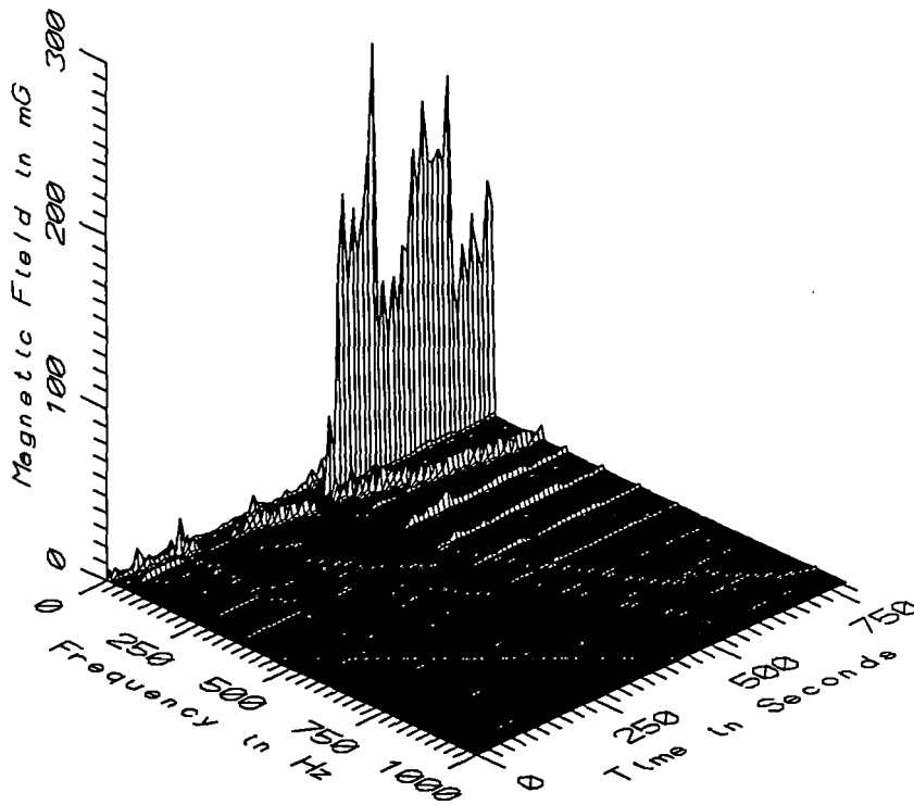
TGV005 - 110cm ABOVE FLOOR AGAINST ENGINEER'S CHAIR, PULL LOCOMOTIVE
