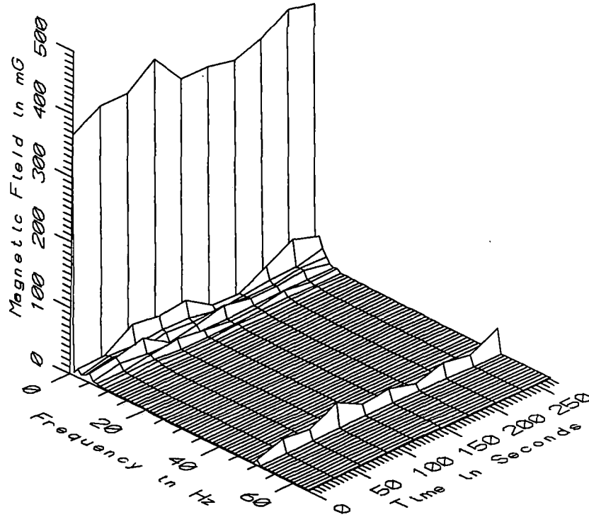
TGV004 - 160cm FROM WINDOW ABOVE SIDE SEAT AT FRONT OF COACH R1B
