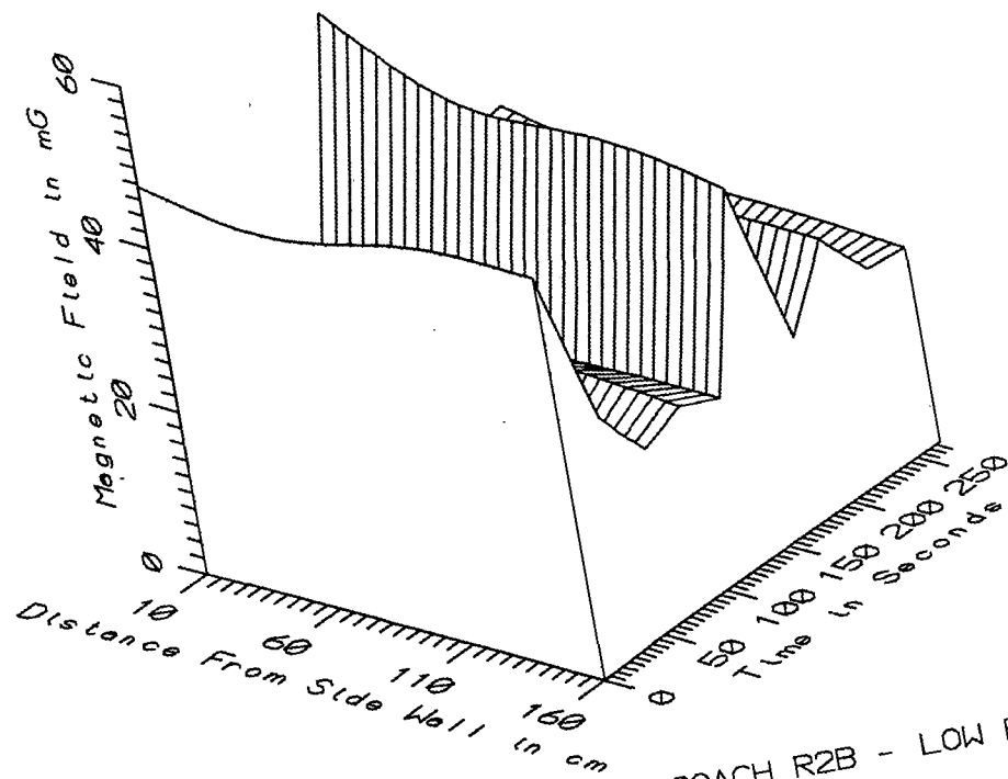
TGV013 - ABOVE SEATS 42 & 43 IN COACH R2B - STATIC
