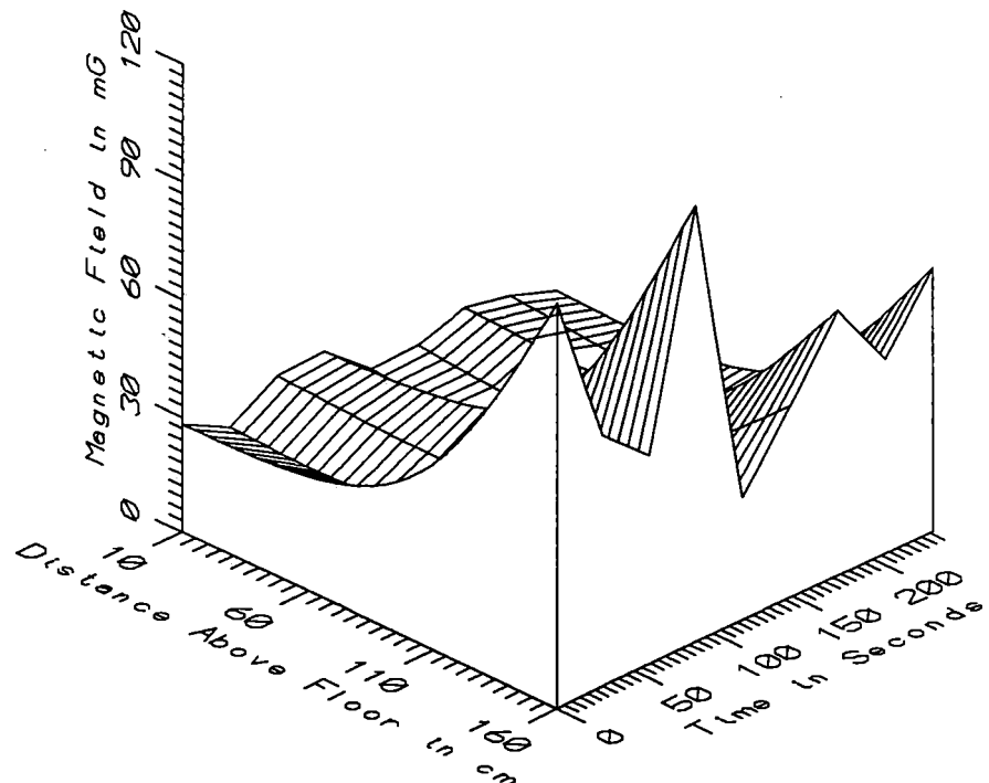
TGV002 - CENTER OF AISLE AT FRONT OF COACH R1B - ALL FREQ, 5-2560Hz
