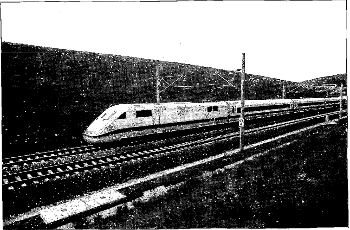
FIGURE 2.4-1. VIEW OF TYPICAL CATENARY SYSTEM SIMILAR TO THE ONE PROPOSED FOR THE NEC.
