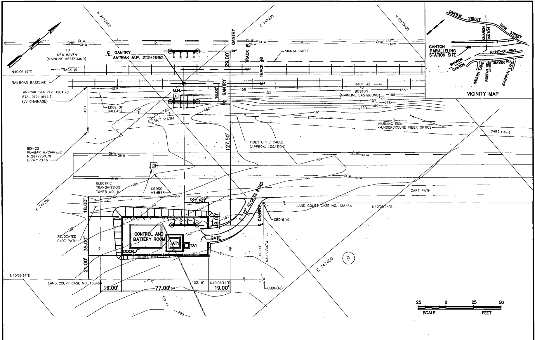
CANTON PARALLELING STATION M.P. 212.38 Figure A-24 Northeast Corridor Improvement Project Electrification – New Haven CT to Boston MA
