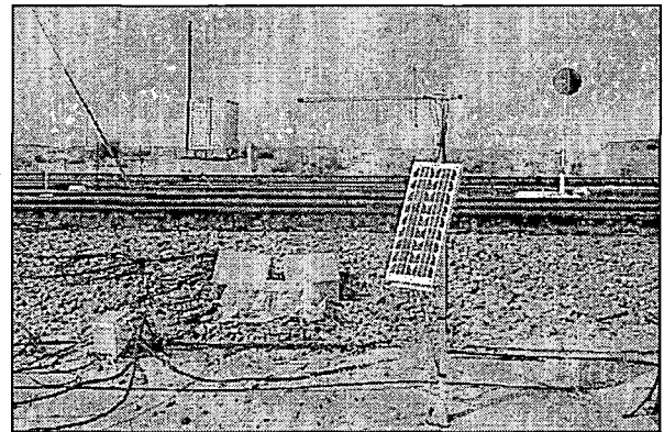
Figure 3. System 1 Solar Panel, Antenna, and Control Boxes
