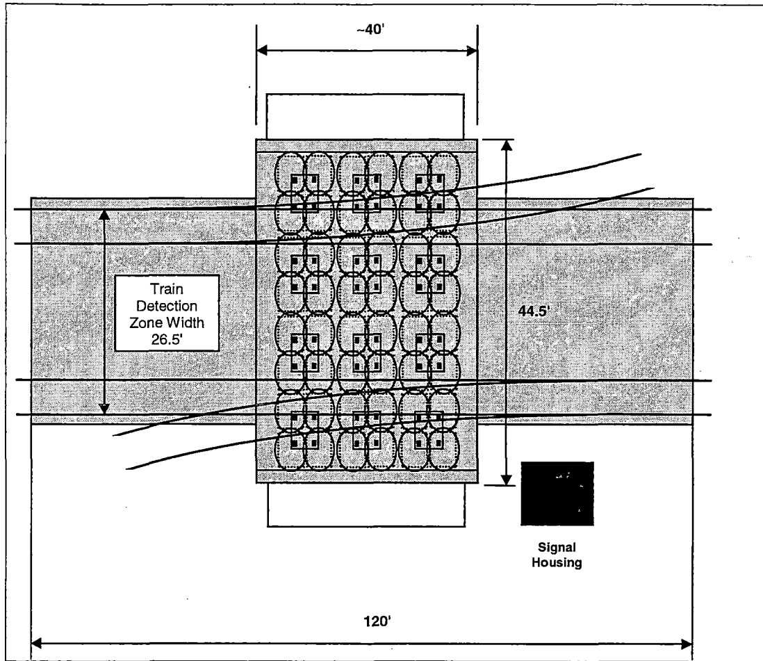
Figure 18. Top View of Coverage Pattern with 12 Detector Assemblies
