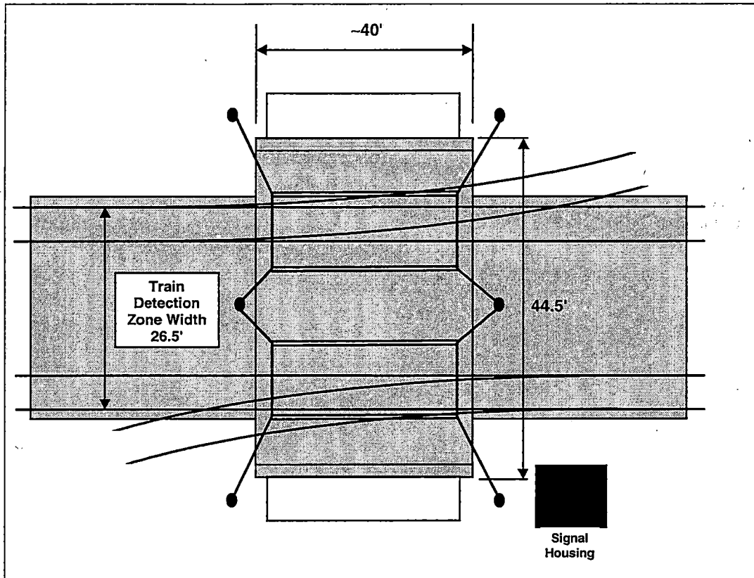
Figure 17. Schematic span Wire Installation for the Mounting of 12 Detector Assemblies
