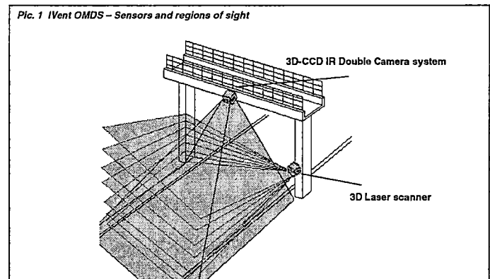
Figure 10. IVent OMDS, Sensors and Regions of Sight
