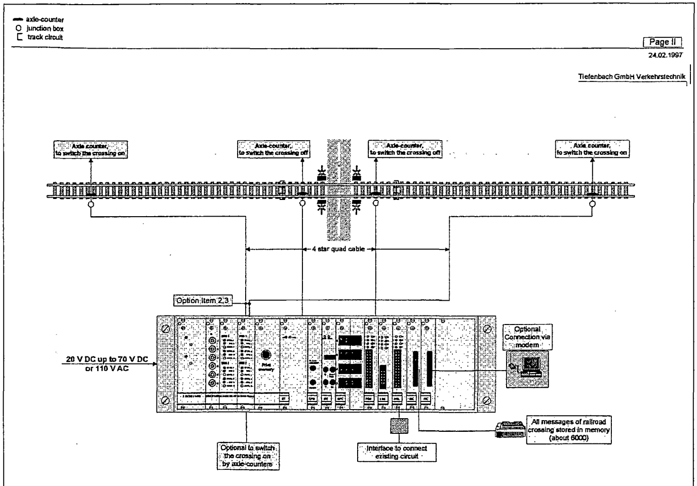
Figure 7. Description of Axle-Counter System
