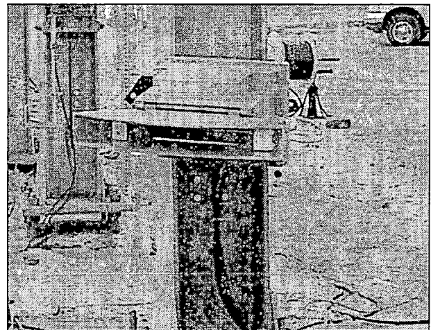
Figure 5. System 2 Vehicle/Obstacle Detection Sensor, Combined Low Power Laser and Video Imaging System
