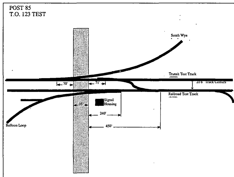
Figure 1: Overall site layout showing tracks, turnouts and road crossing.
