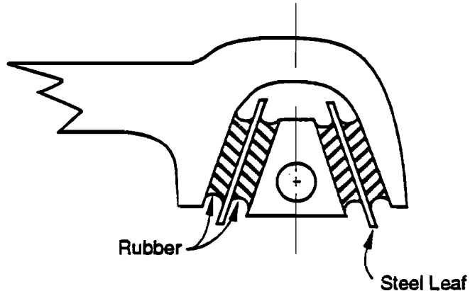
Figure 2.11b Rubber Chevron
