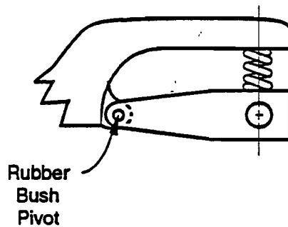
Figure 2.11d Radius Arm
