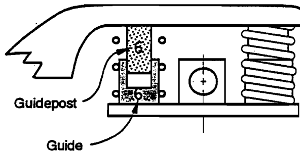
Figure 2.11f Guidepost
