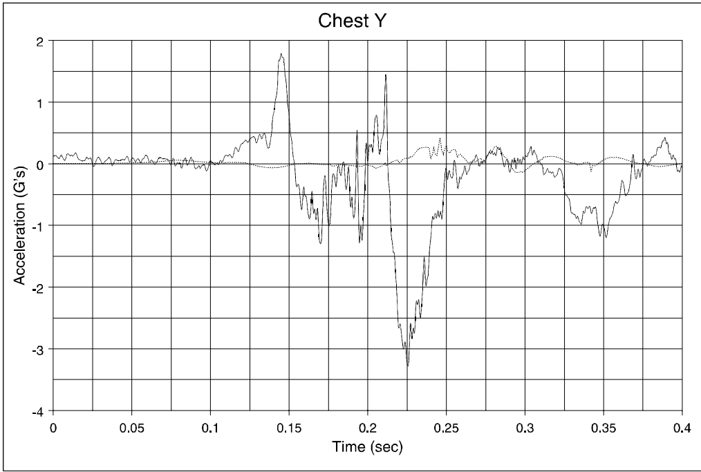
Figure F190. Walkover Seat, Type 2 Test, 50th-Percentile Hybrid III Male ATD, Center Seat; Chest Acceleration, y Direction
