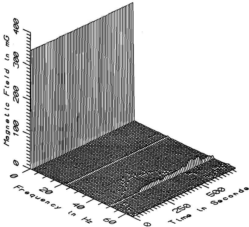
TGV034 - 110cm ABOVE FLOOR IN CONTROL HOUSE, GAULT ST. DENIS SUBSTATION
