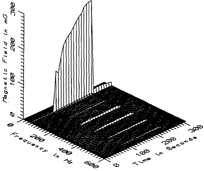
TGV029 - 110cm ABOVE OVERPASS BASE, ABOVE PARIS BOUND LINE. 120km MARKER
