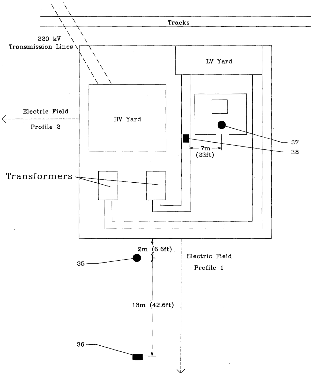
FIGURE 7-1. REPETITIVE WAVEFORM MEASUREMENT LOCATIONS AT THE GAULT ST. DENIS SUBSTATION, ALSO SHOWING THE ELECTRIC FIELD PROFILES
