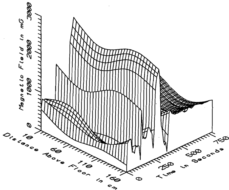
TGV005 - AGAINST ENGINEER'S CHAIR, PULL LOCOMOTIVE - STATIC
