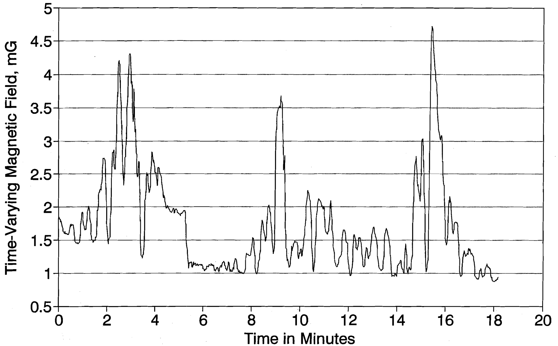
FIGURE 5-9. MAGNETIC FIELD LEVEL AS RECORDED BY THE DAT AT A POINT 22.5 m (74 ft) FROM CENTERLINE OF THE NEAREST TRACK, AS A FUNCTION OF TIME, AT AN OPEN SPACE ALONG THE WAYSIDE NEAR THE 104 km MARKER
