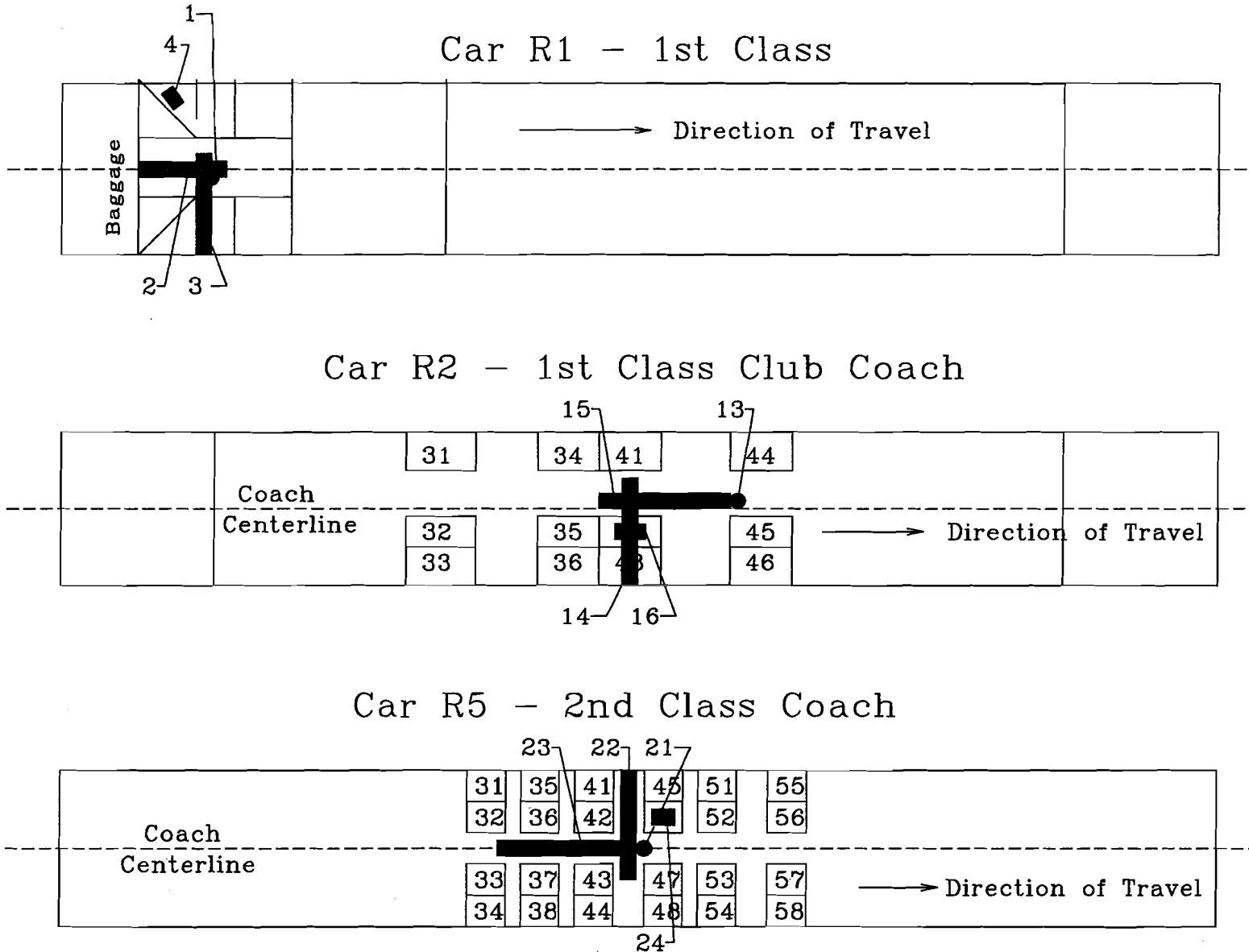
FIGURE 3-2. REPETITIVE WAVEFORM MEASUREMENT LOCATIONS IN CARS R1B-FIRST CLASS SALON, R2B-FIRST CLASS CLUB COACH AND R5B-SECOND CLASS COACH
