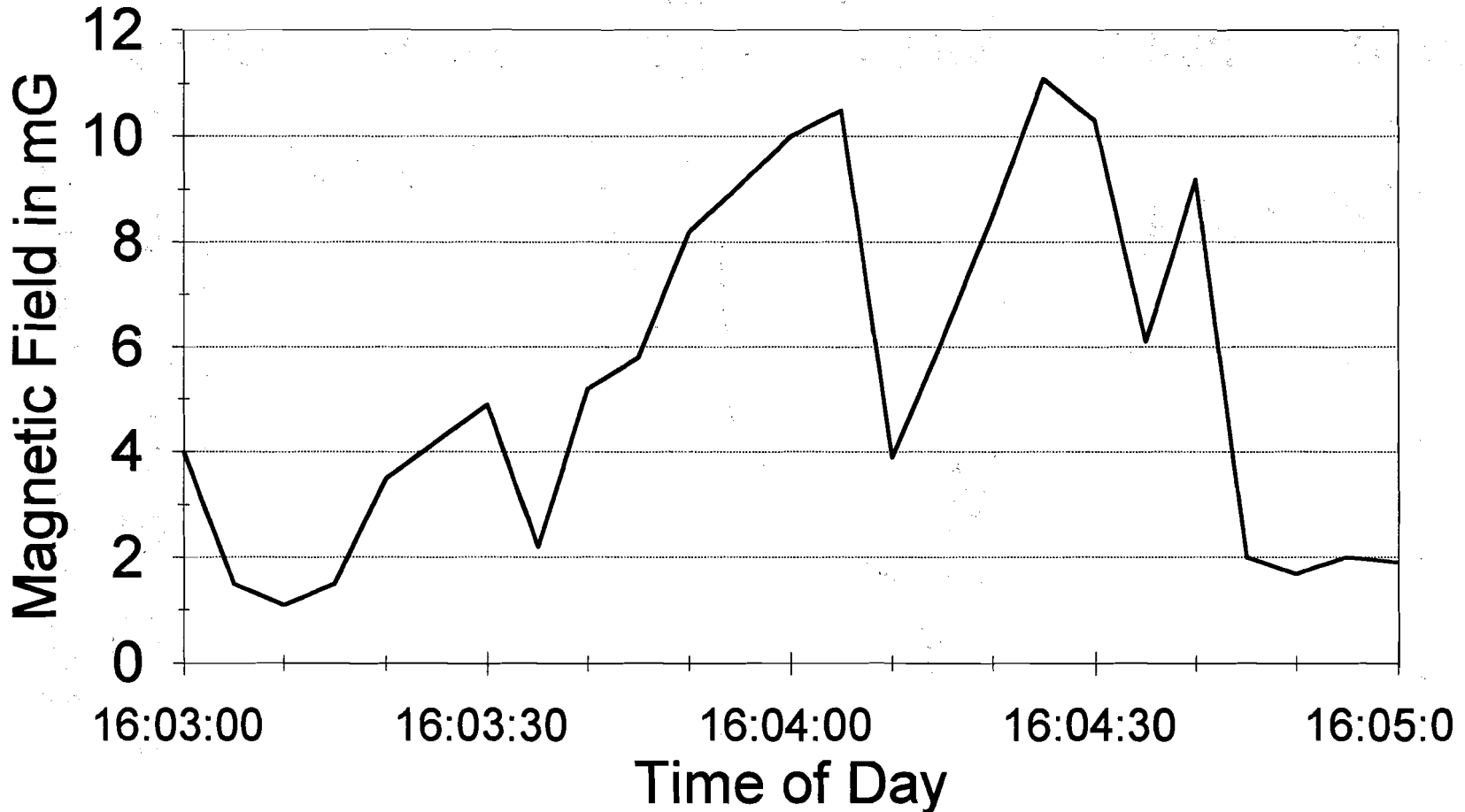
FIGURE 6-6. MAGNETIC FIELD LEVEL RECORDED ON THE PASSENGER PLATFORM AT VENDOME USING AN RMS RECORDER, WHILE A TRAIN FROM PARIS PASSED BY, AS A FUNCTION OF TIME
