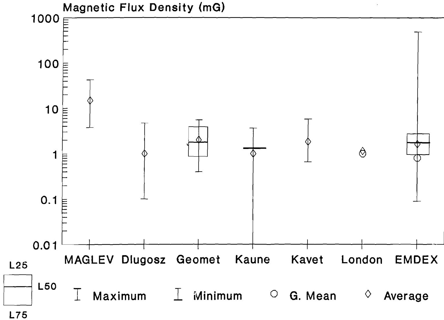
FIGURE 6-1. MAGNETIC FLUX DENSITIES ASSOCIATED WITH MAGLEV (TR-07, 50-60 Hz @ 12.7 cm) AND RESIDENTIAL EXPOSURES (see section 2.5 for study descriptions)
