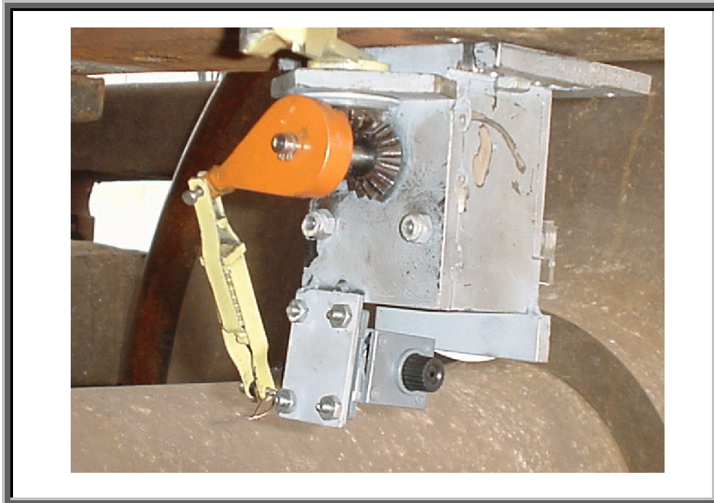
Figure 13. Rear view of mechanical system
