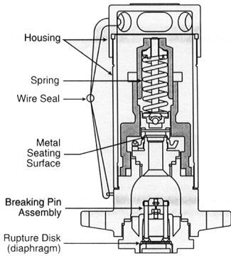
COMBINATION SAFETY RELIEF DEVICE
