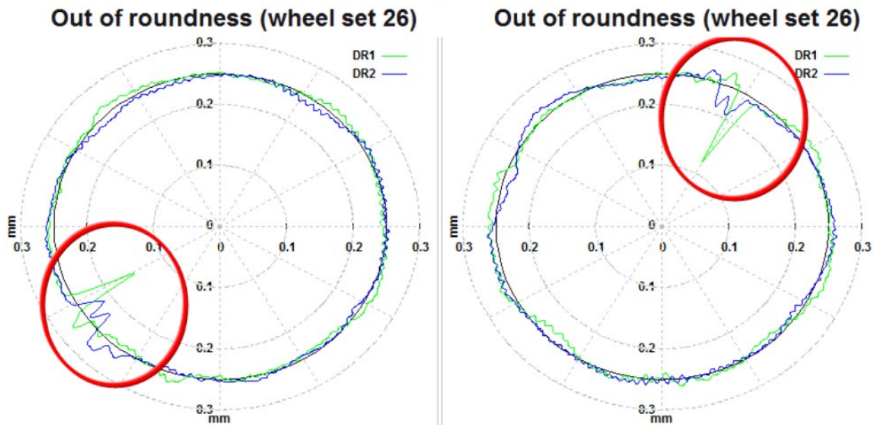
Figure 4-6. An example of wheel tread irregularity detection concept of MERMEC's WILD system using accelerometers and strain gages [9]
