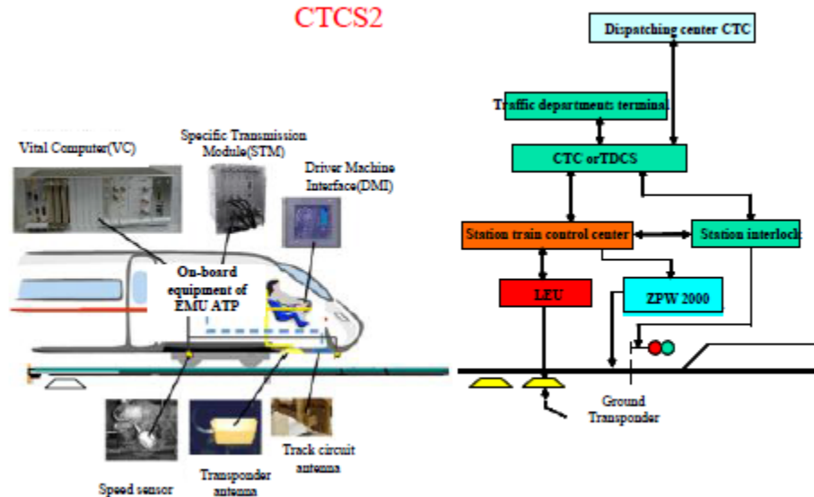
Figure A-2 CTSC2 System
