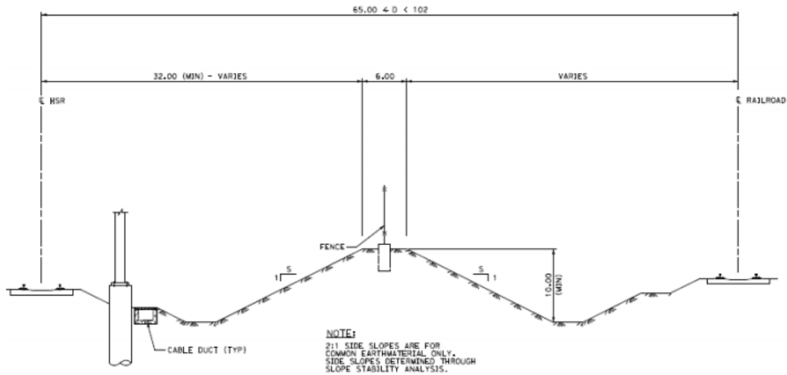
Figure 3.2 Earthwork barrier protection (Abtahi, 2013)
