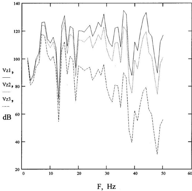
Figure 2.20 Effect of soil attenuation constant \gamma on ground vibration level (dB reference 10^{-9} m/s) generated by a train of five cars moving at three trans-Rayleigh speeds: 50 km/h (Vz1), 150 km/h (Vz2), and 250 km/h (Vz3). (Krylov, 1996)
