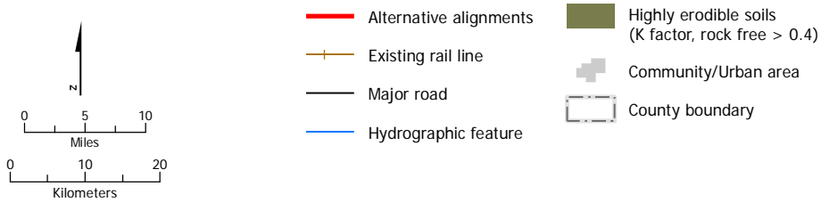
Figure 3.9-8 Erodible soils in the study area
