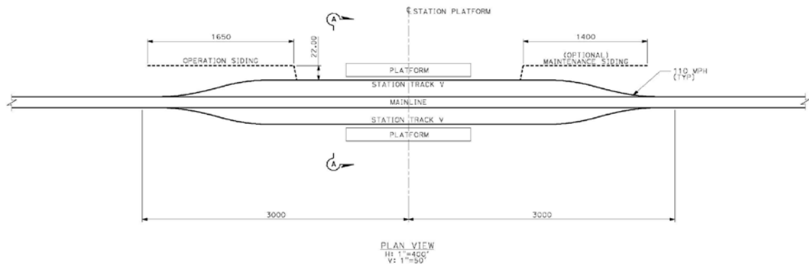
Figure 7 Intermediate Station Typical Configuration
