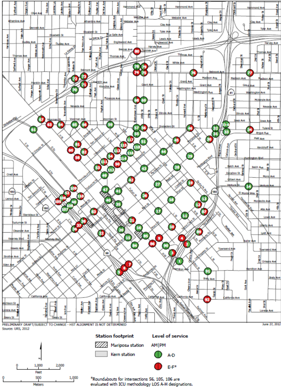
Figure 3.2-23b Future (2035) Plus Project intersection LOS in the Fresno Station area – Overpass Alternative
