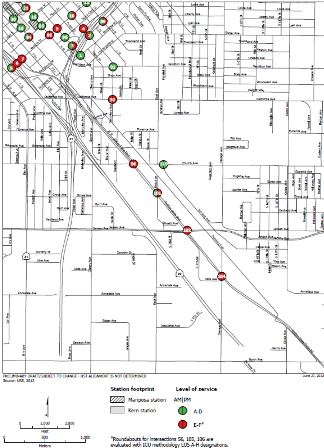
Figure 3.2-22c Future (2035) Plus Project intersection LOS in the Fresno Station area – Underpass Alternative
