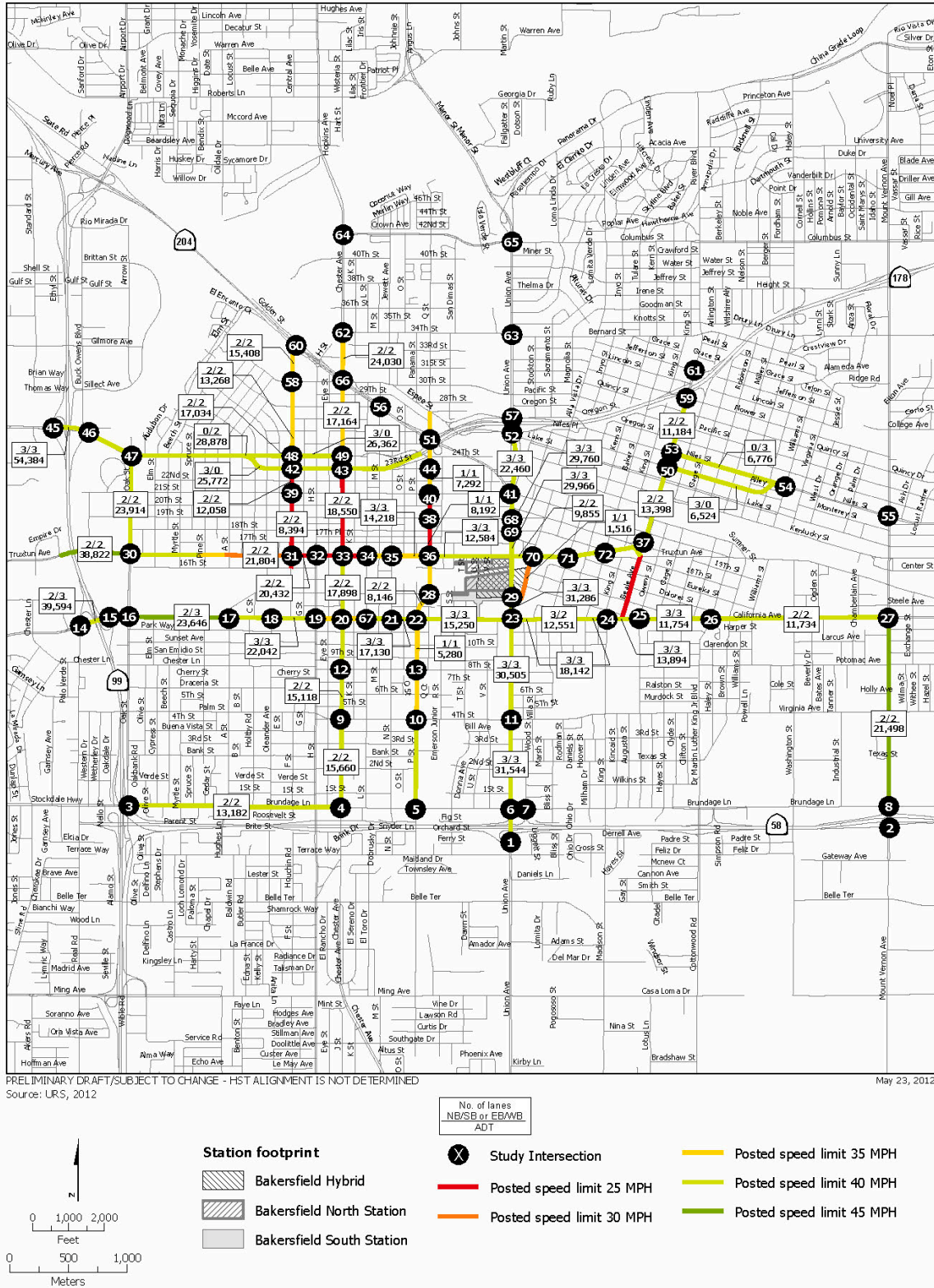
Figure 3.2-20 Average daily traffic, number of lanes, and speed—Bakersfield Station area
