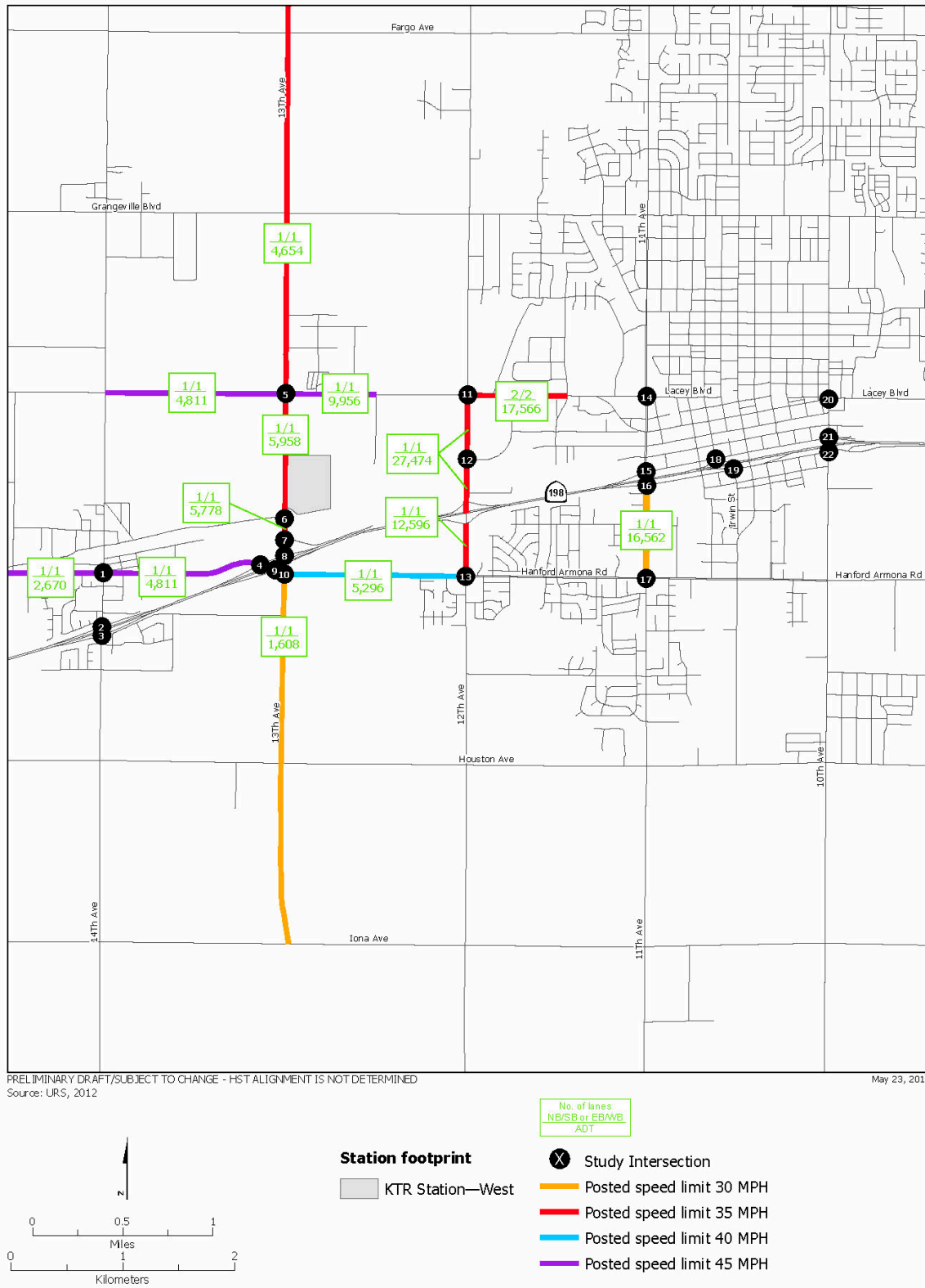
Figure 3.2-16 Average daily traffic, number of lanes, and speed: potential Kings/Tulare Regional Station—West
