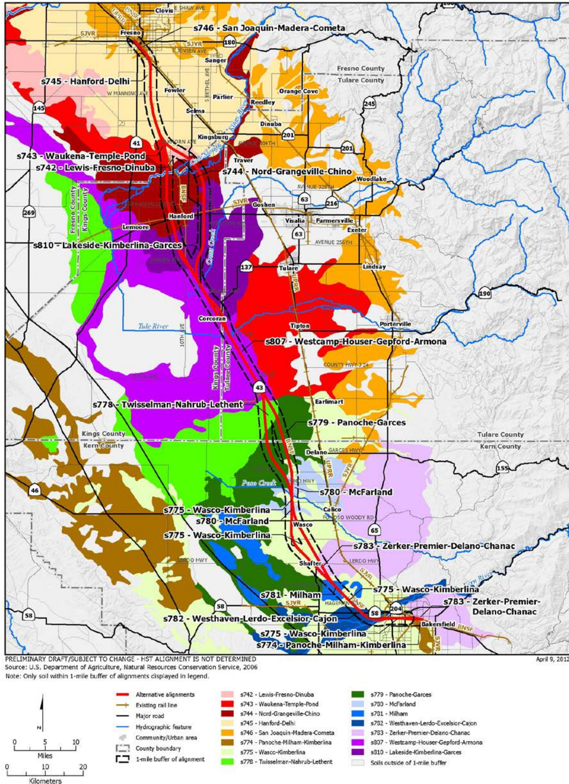
Figure 3.9-2 Soil associations within the study area
