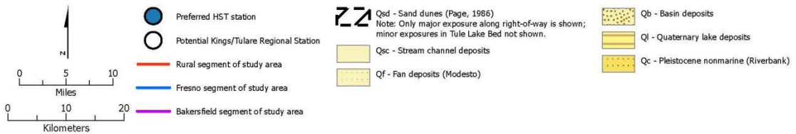
Figure 3.9-1 Surficial geology within the study area
