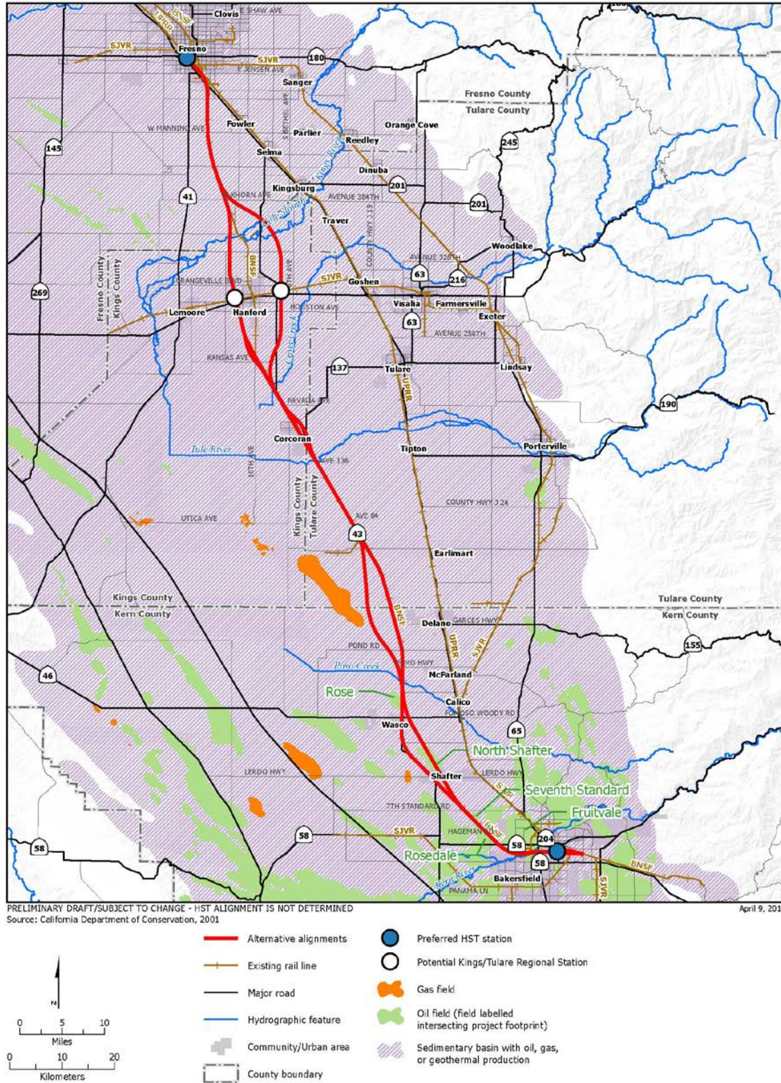
Figure 3.9-7 Oil, gas, and geothermal fields in the Fresno to Bakersfield Section
