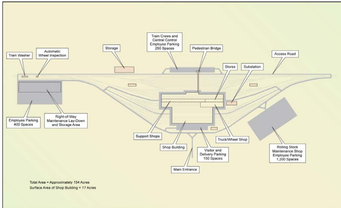
Figure 3.16-64 Conceptual HMF layout
