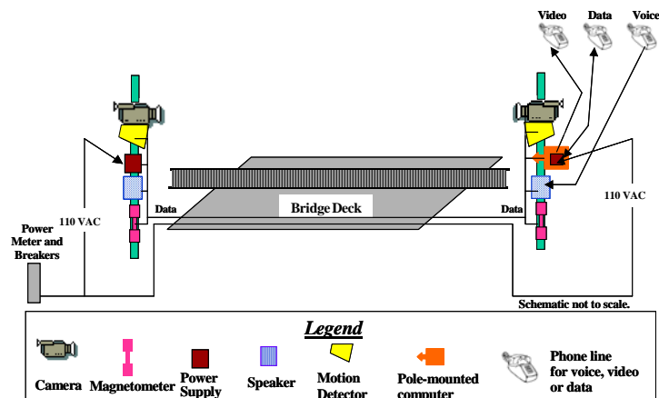
Figure 1. Illustration of the surveillance system technology
