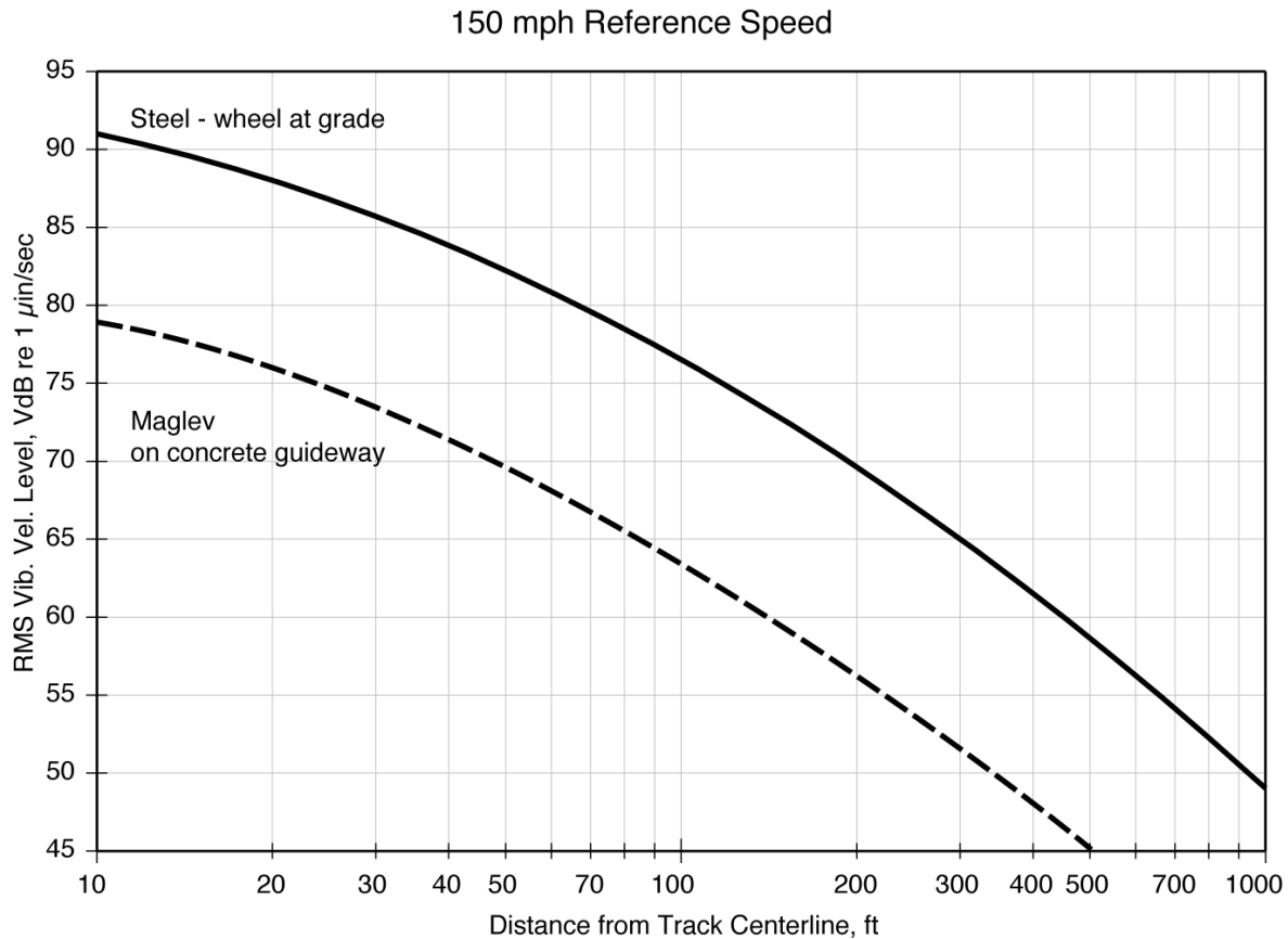
Figure 8-1 Generalized Ground-Borne Vibration Curve
