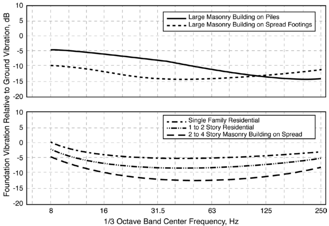
Figure 9-7 Approximate Foundation Response for Various Types of Buildings
