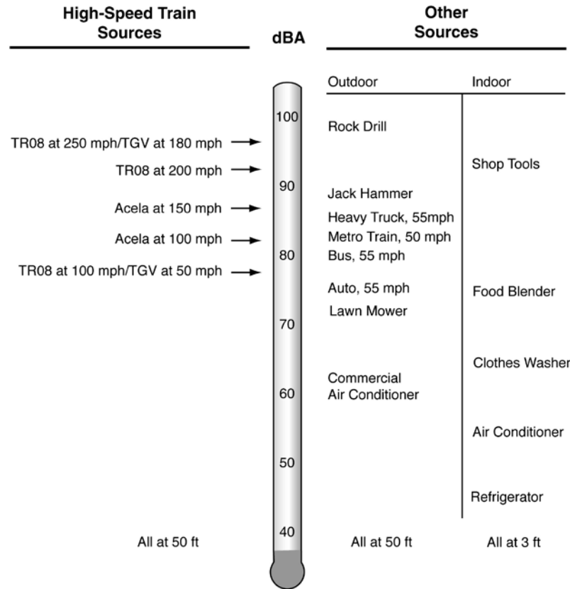
Figure 2-2 Typical A-Weighted Maximum Sound Levels
