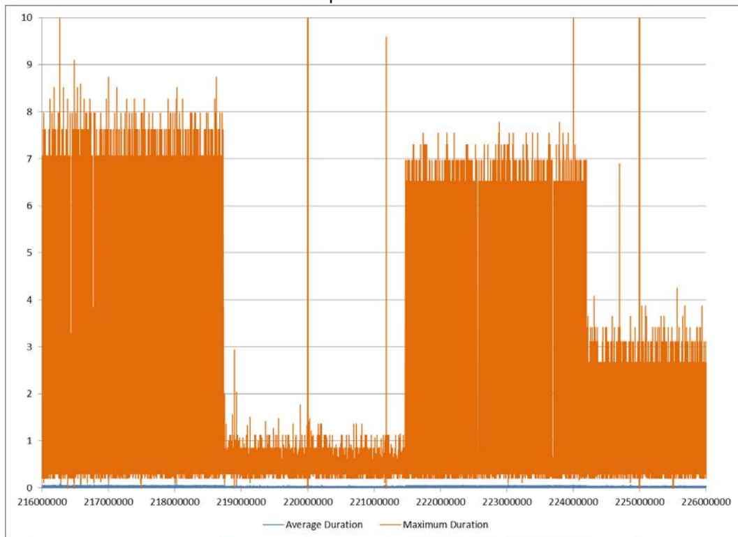
Duration Profile CSX 985 Notch 4 Figure 32
