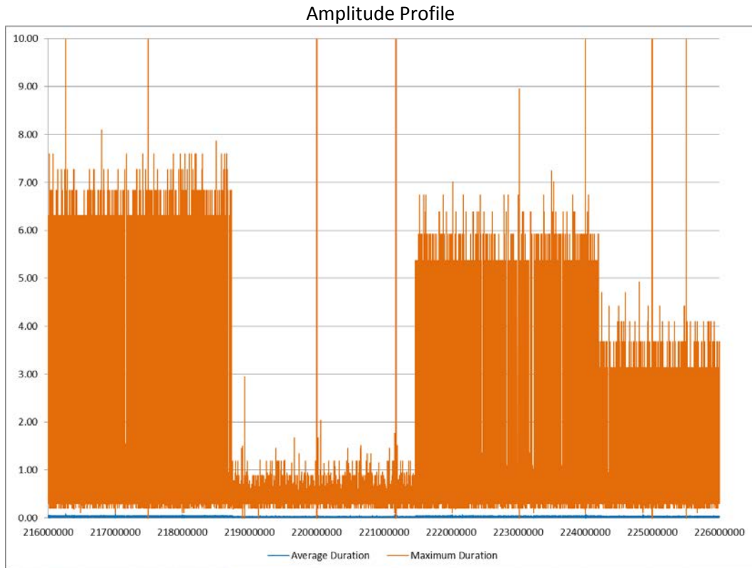
Duration Profile CSX 985 Engine Idle Figure 28
