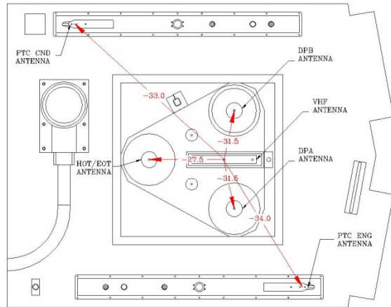
Transmit from single source Un-filtered
