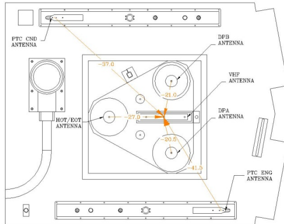
Receive from multiple sources Unfiltered
