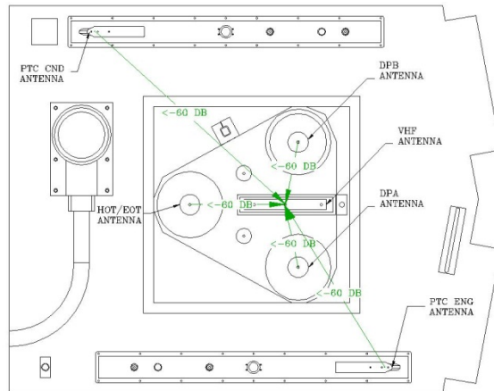
Receive from multiple sources Filtered
