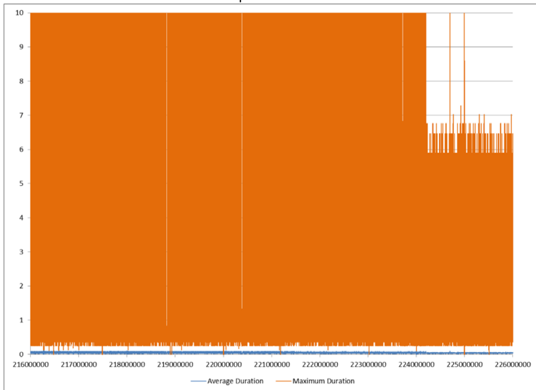
Duration Profile CSX 985 Notch 7 Figure 35
