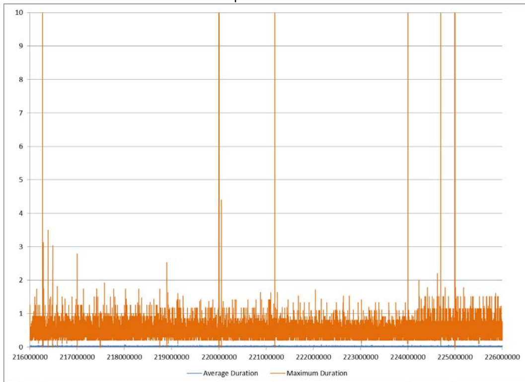
Duration Profile CSX 985 Notch 8 Figure 36
