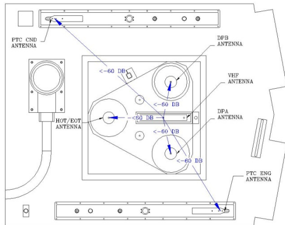
Transmit from single source Filtered
