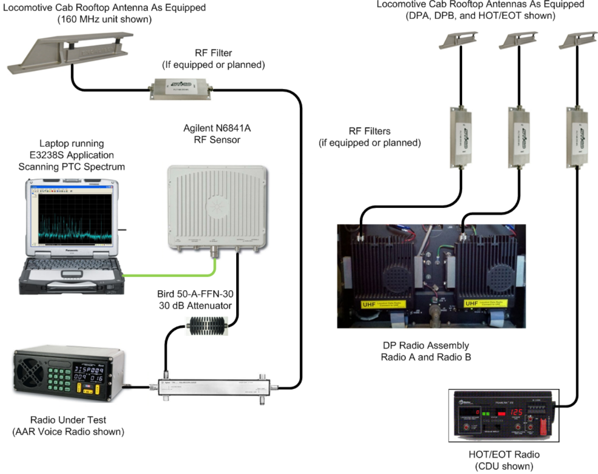
Transmit Intermodulation Testing Configuration Figure 22
