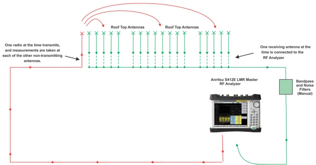
Antenna Isolation Testing Configuration Figure 14
