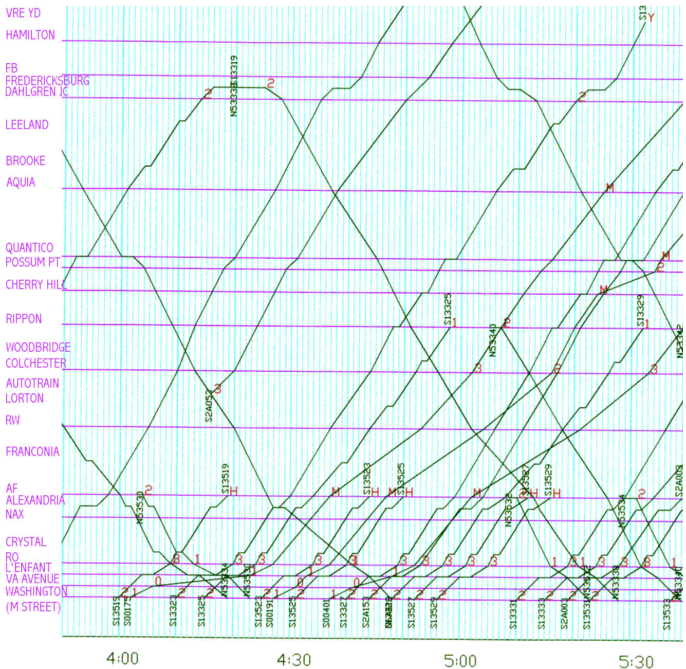
Figure C-1: Typical Simulation Stringline Plot
