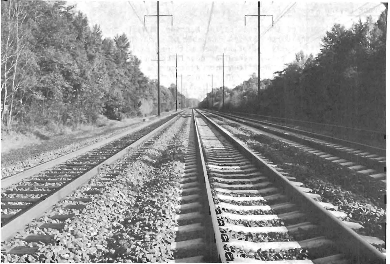
Typical concrete tie installation in multiple-track territory between New York and Washington.
